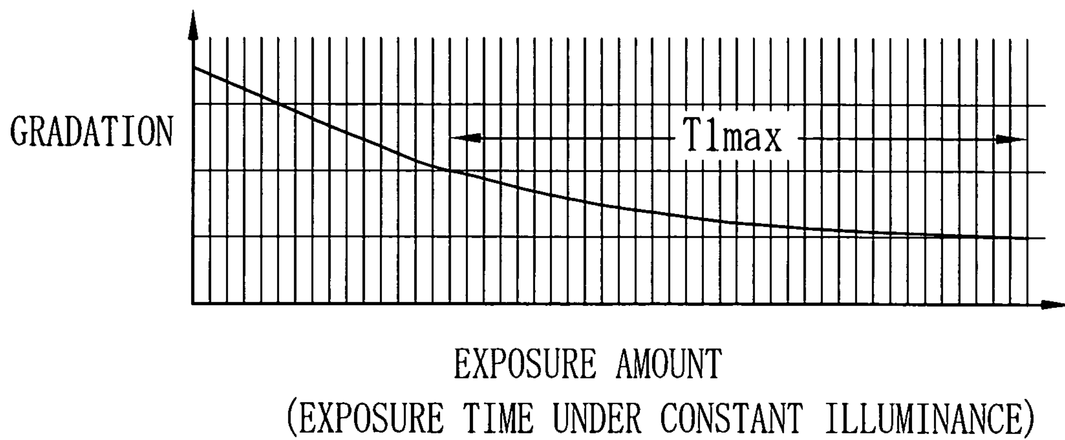
FIG. 11 (PRIOR ART)
