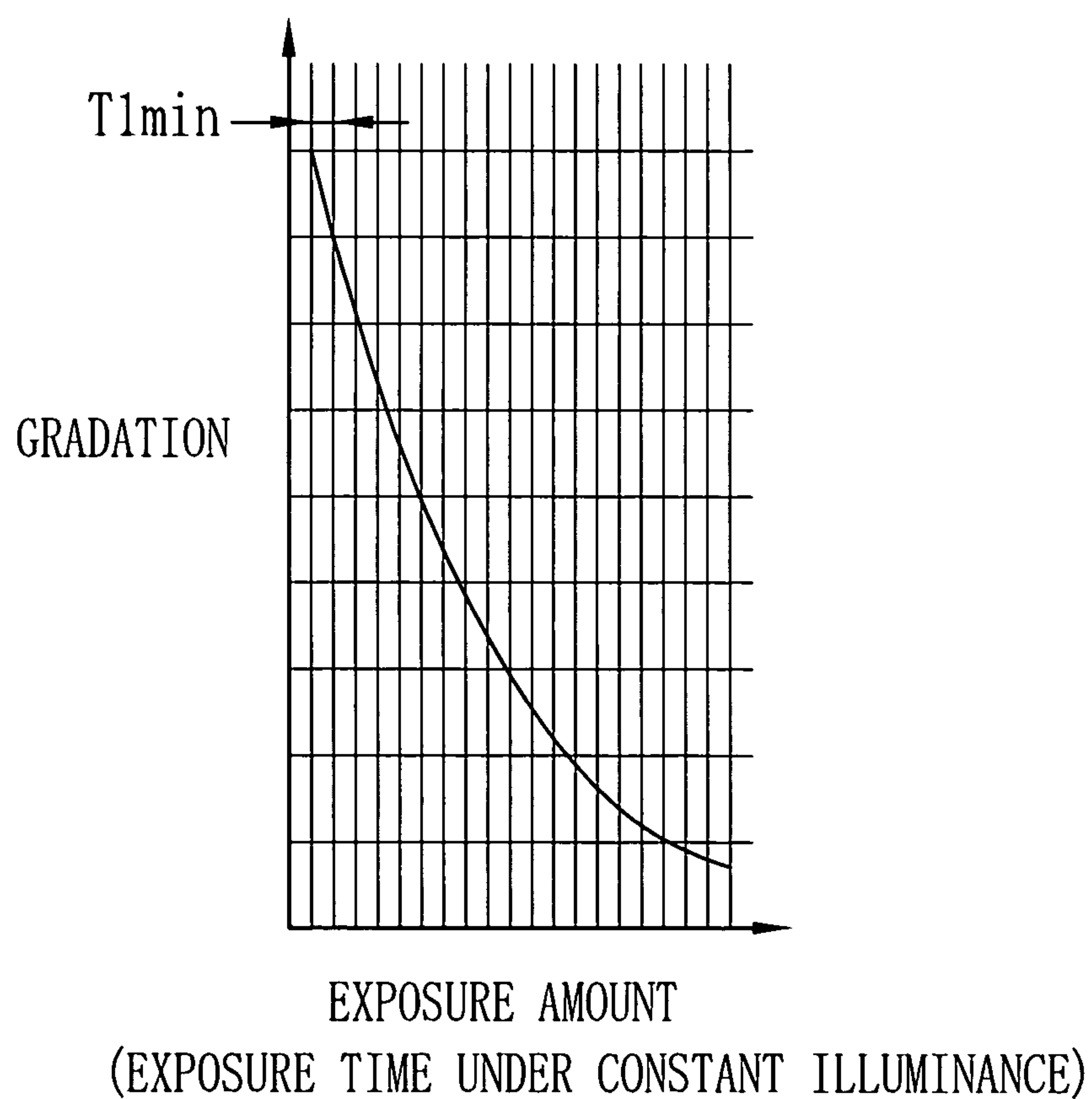
FIG. 12 (PRIOR ART)
