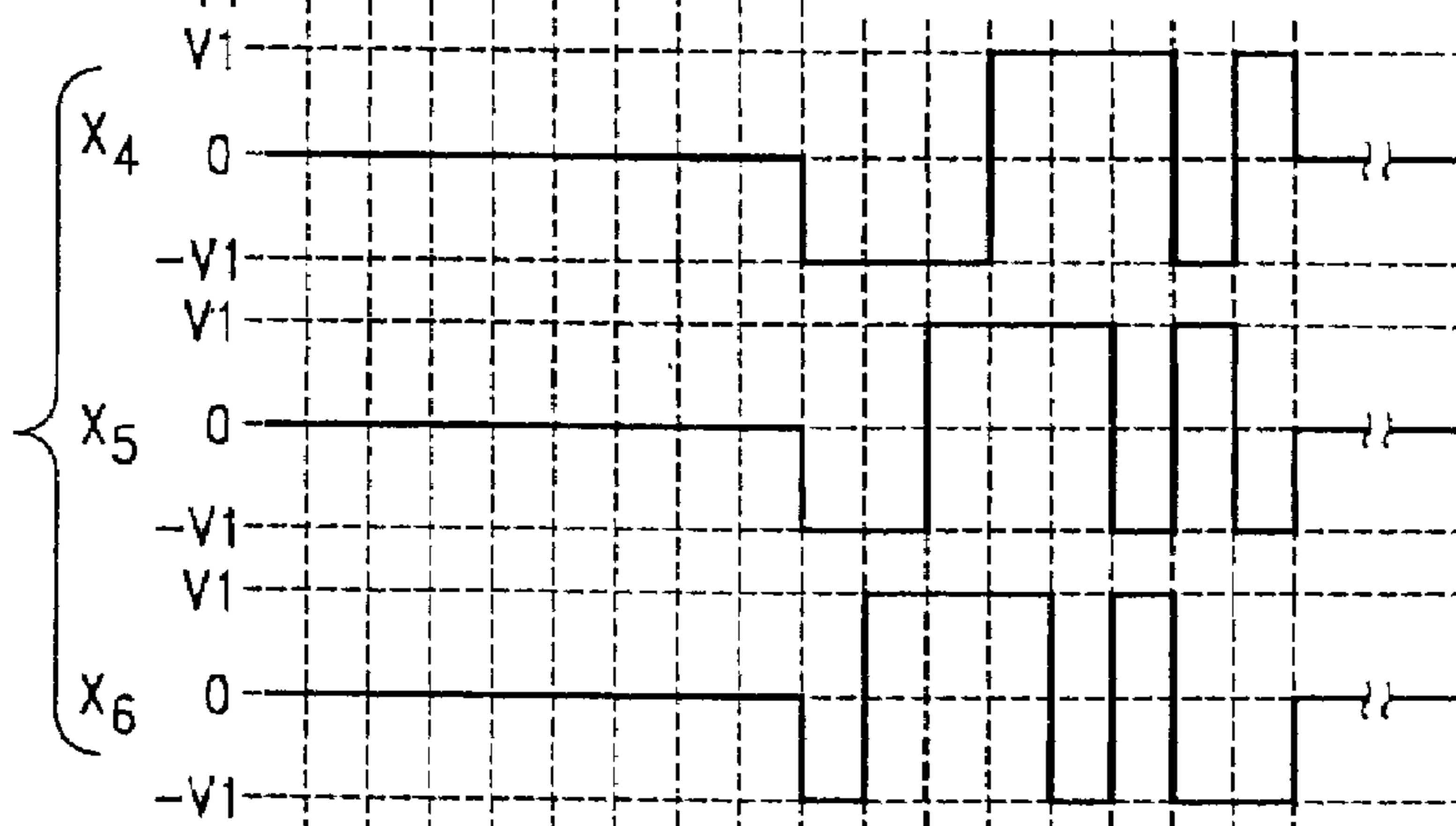
FIG.-25B (PRIOR ART)
