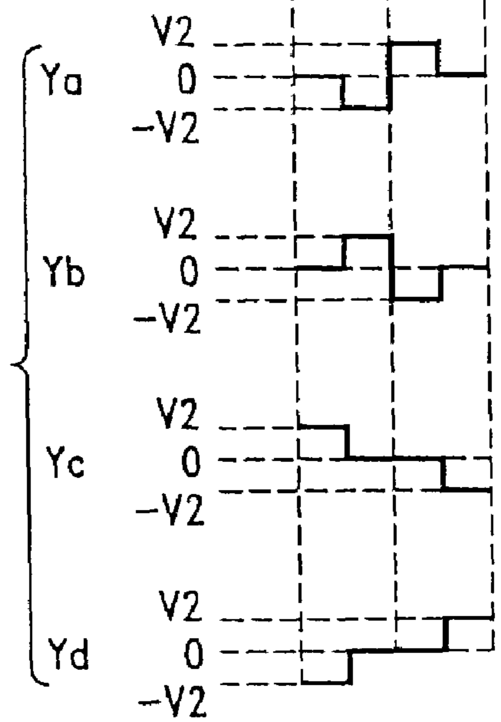
FIG.-24B (PRIOR ART)
