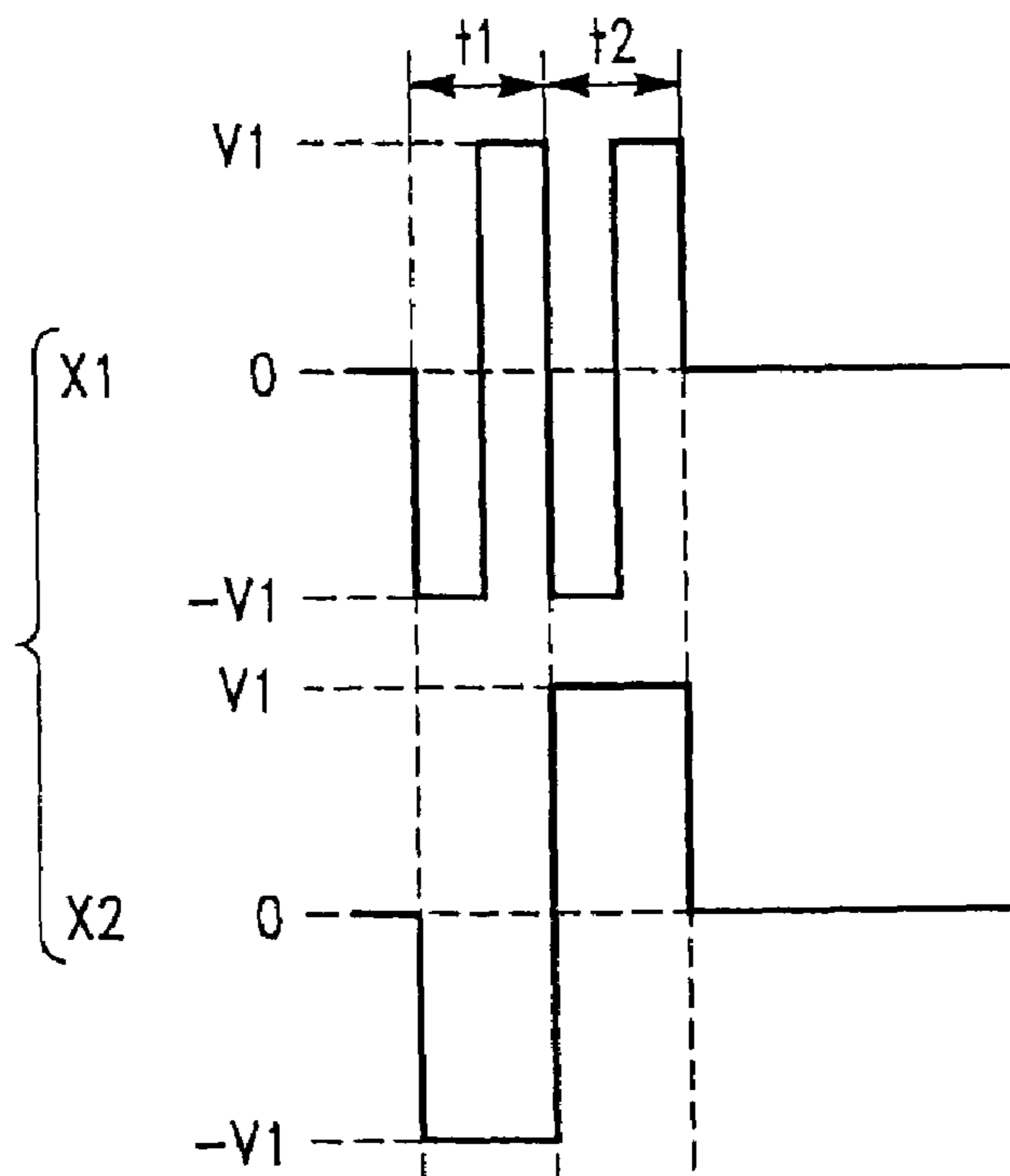
FIG.-24A (PRIOR ART)
