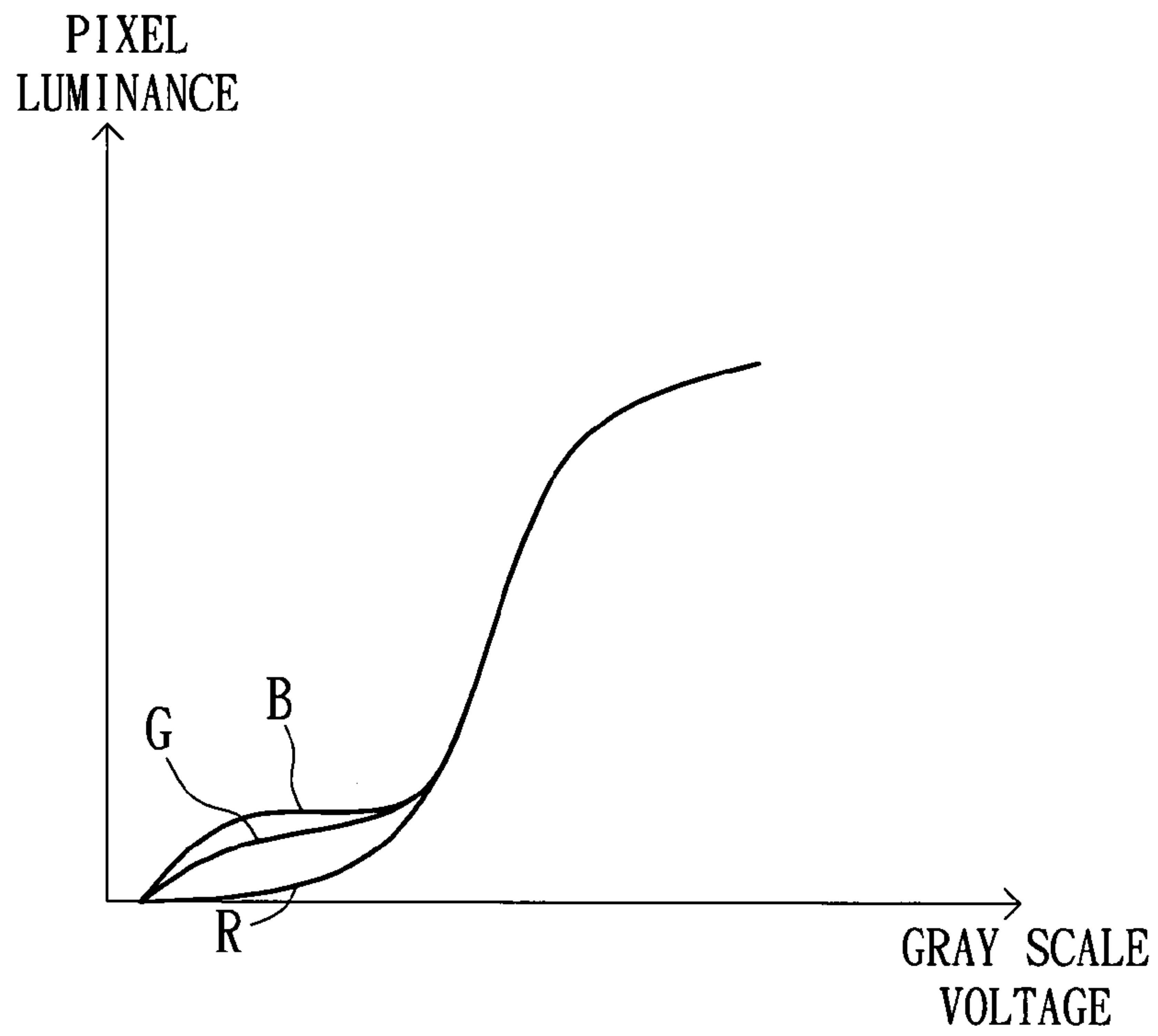
FIG. 4E(PRIOR ART)
