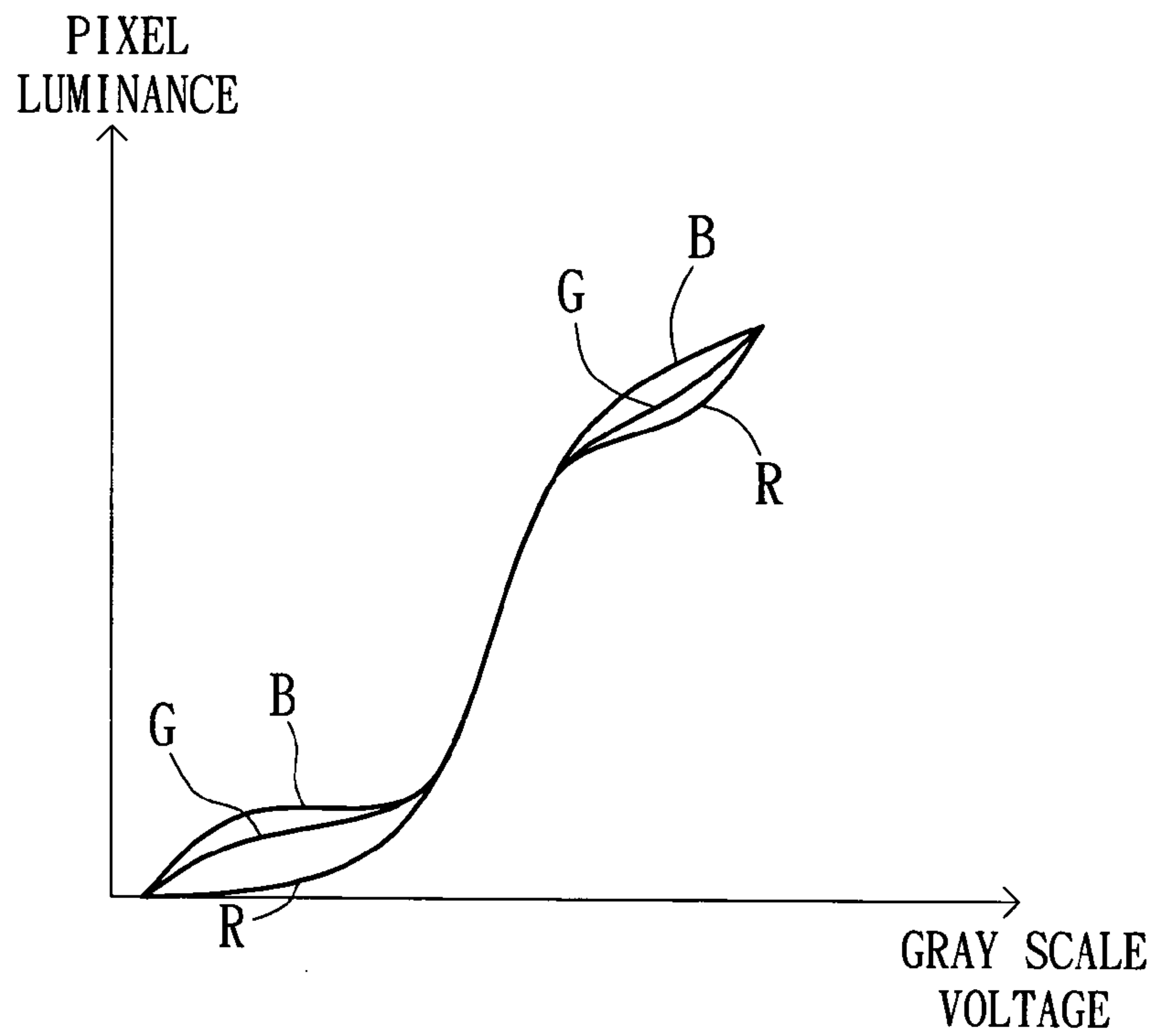
FIG. 4F(PRIOR ART)
