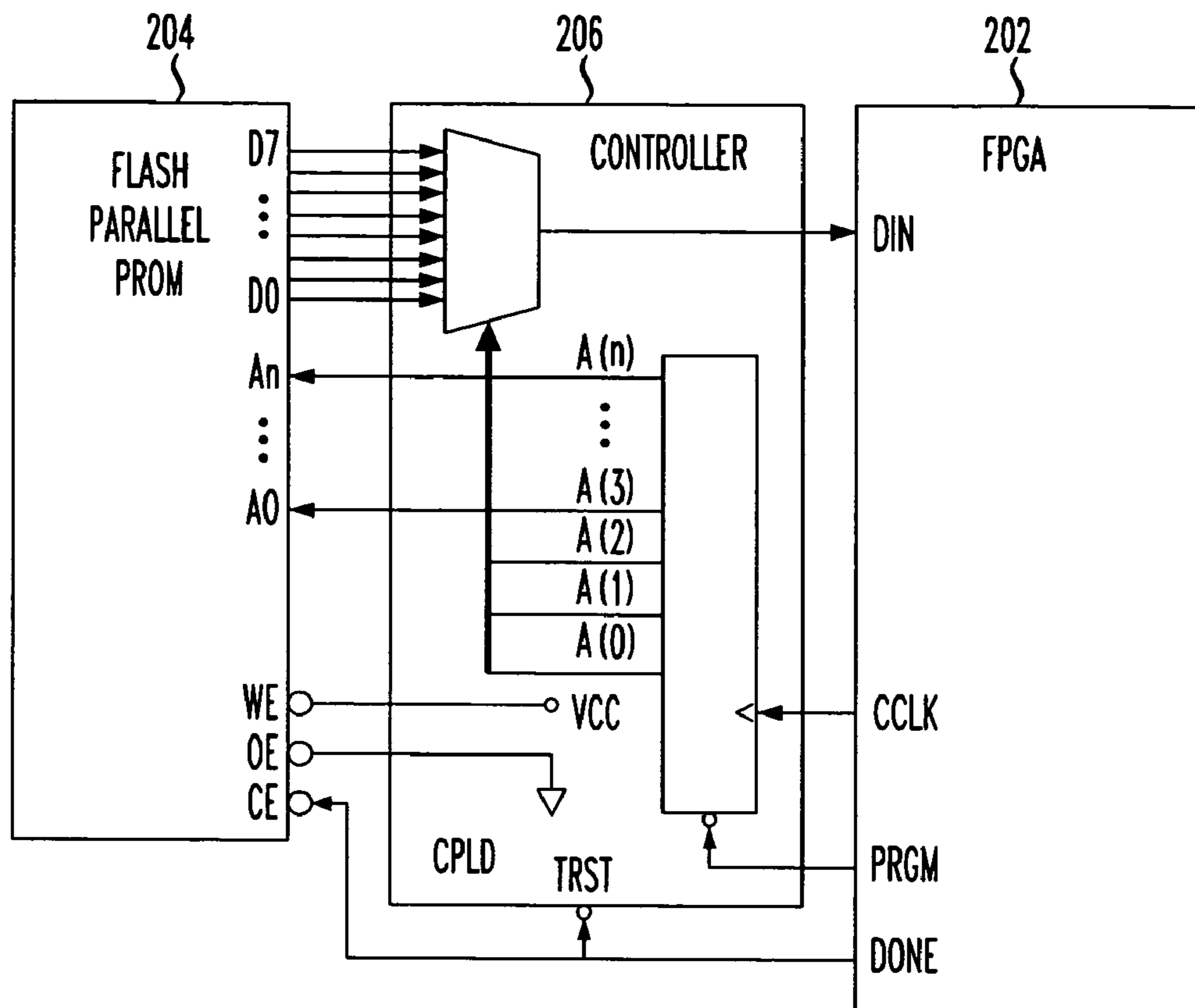
FIG. 2 (PRIOR ART)
