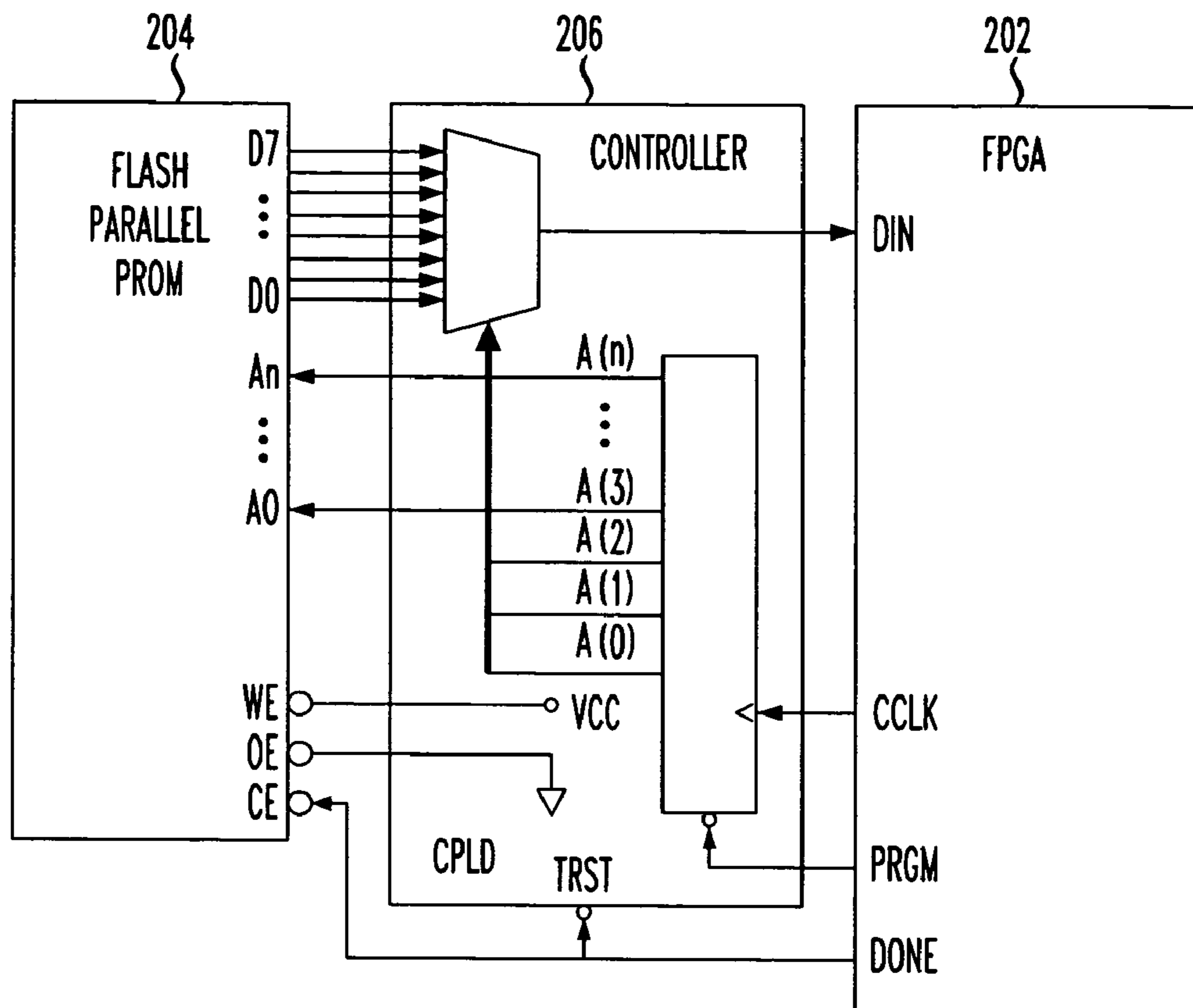
FIG. 2 (PRIOR ART)
