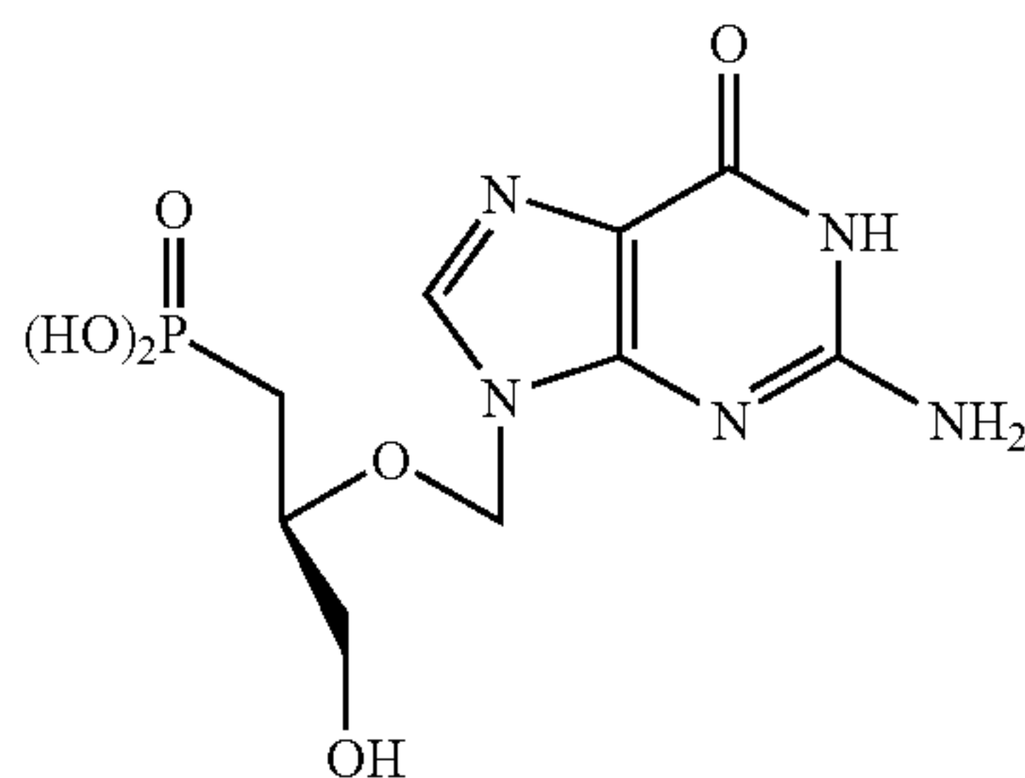
Ganciclovir phosphonate
