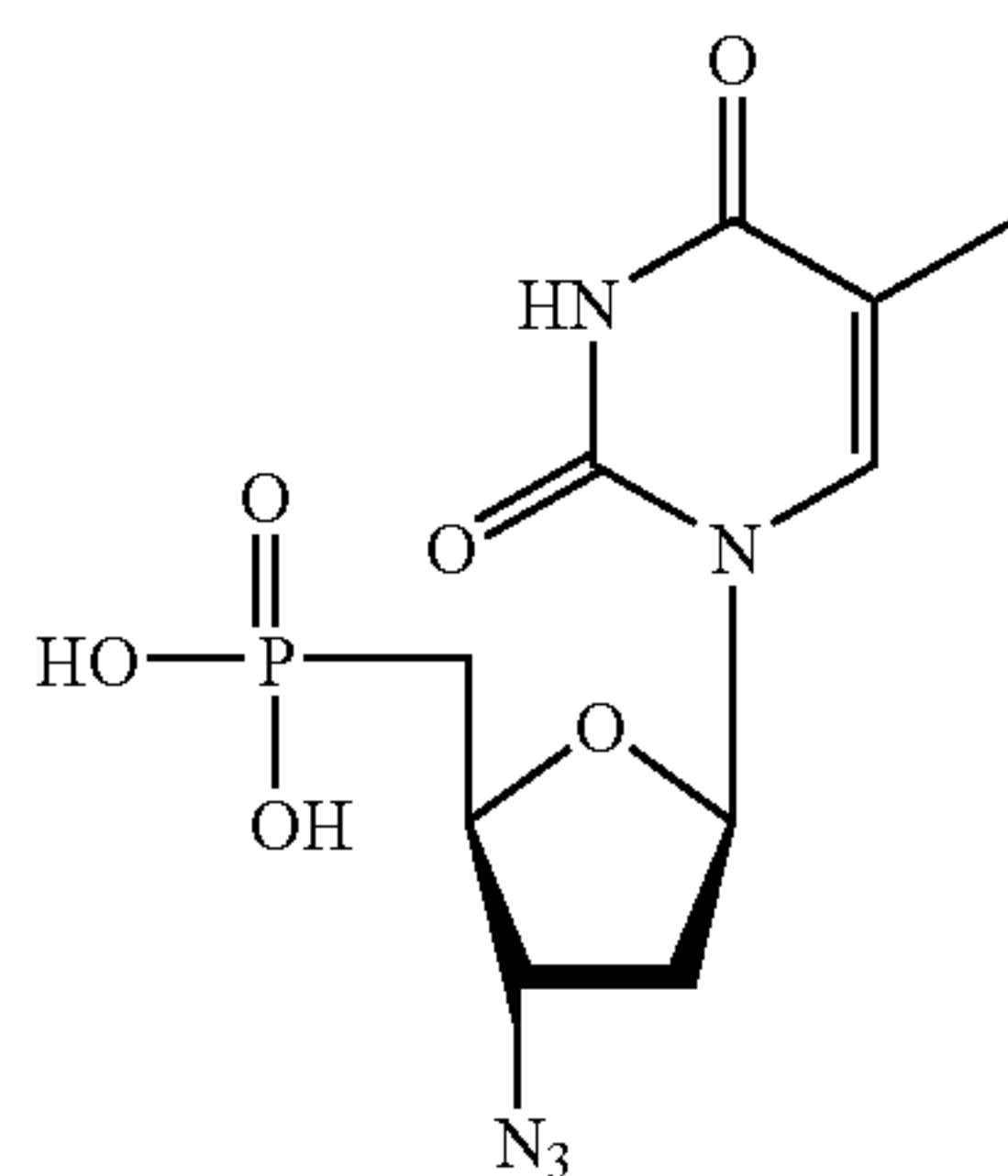
AZT 5'-phosphonate
