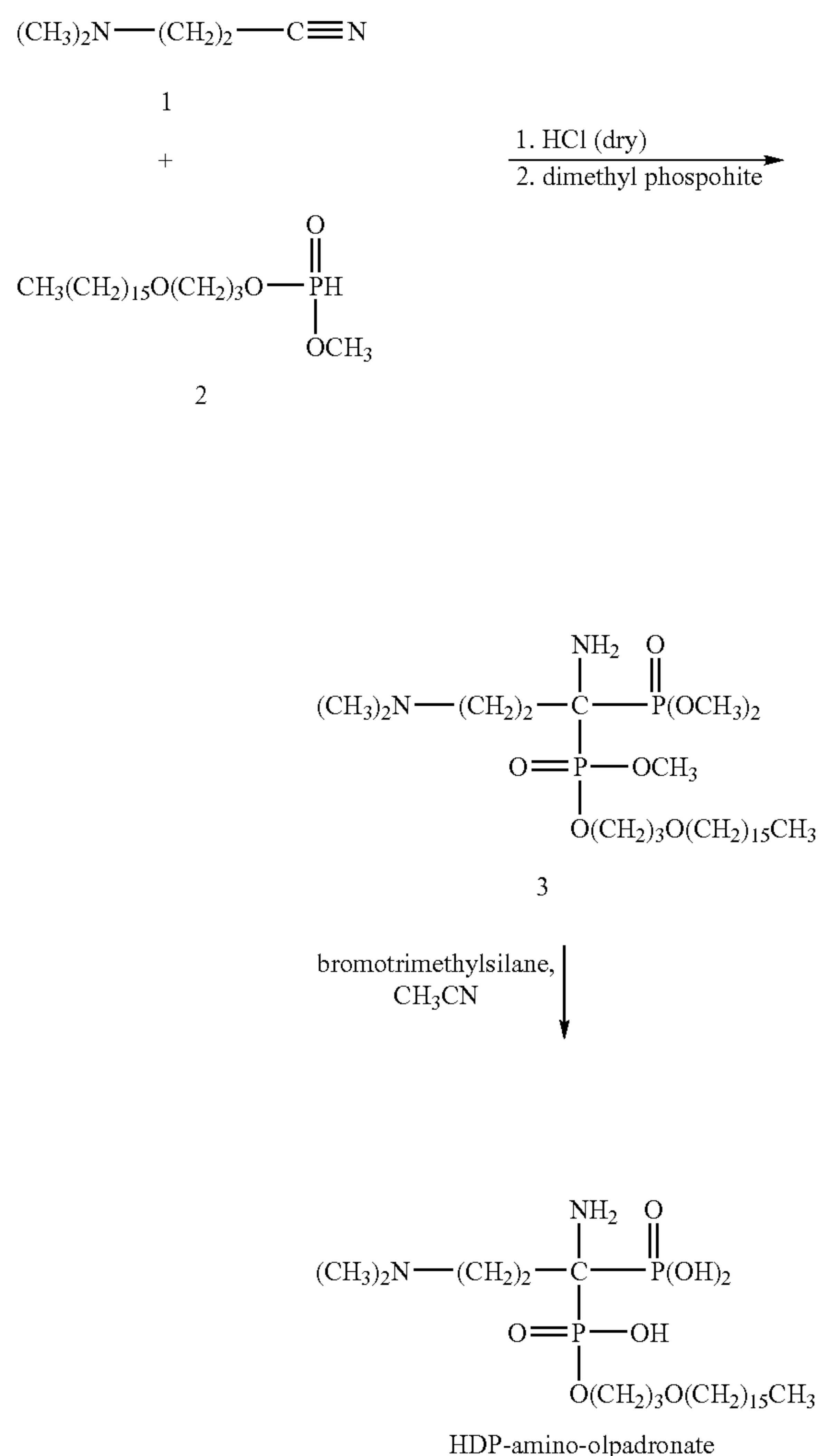
Scheme III
