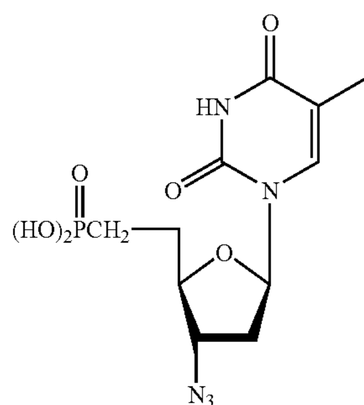
AZT 5'-methylene-phosphonate
