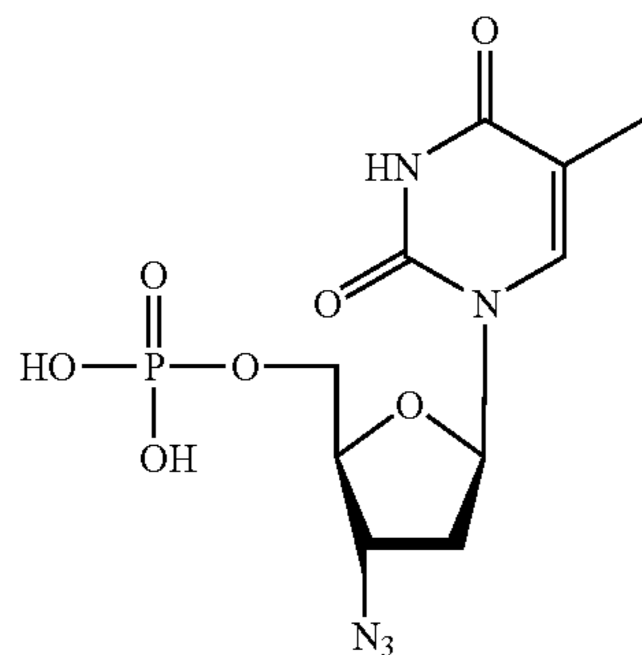
AZT 5'-phosphate
