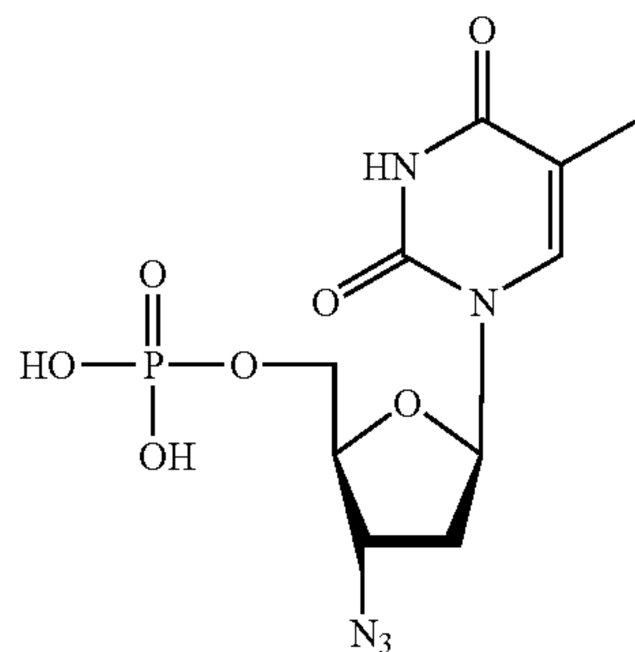
AZT 5'-phosphate
