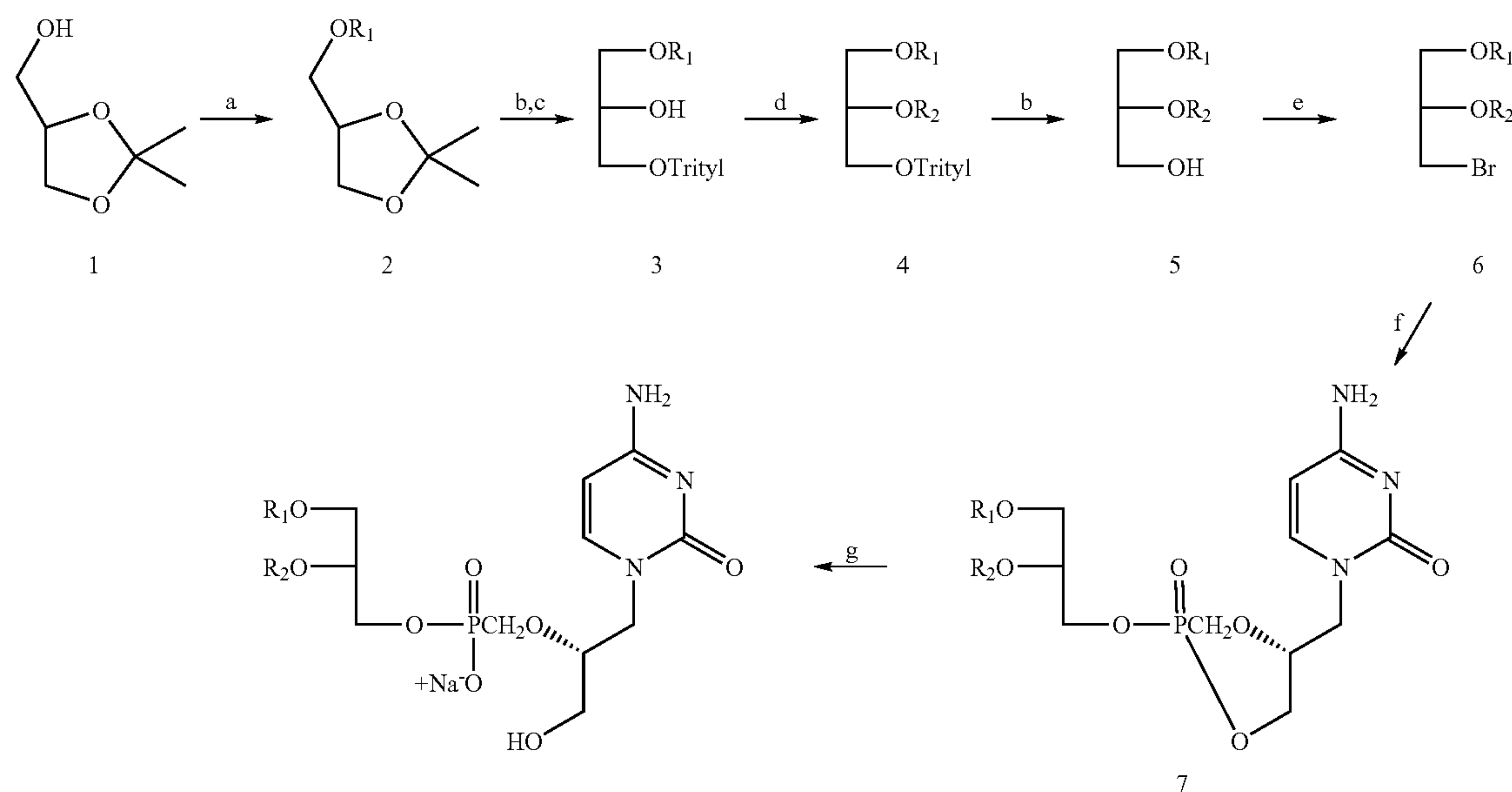
Scheme V
