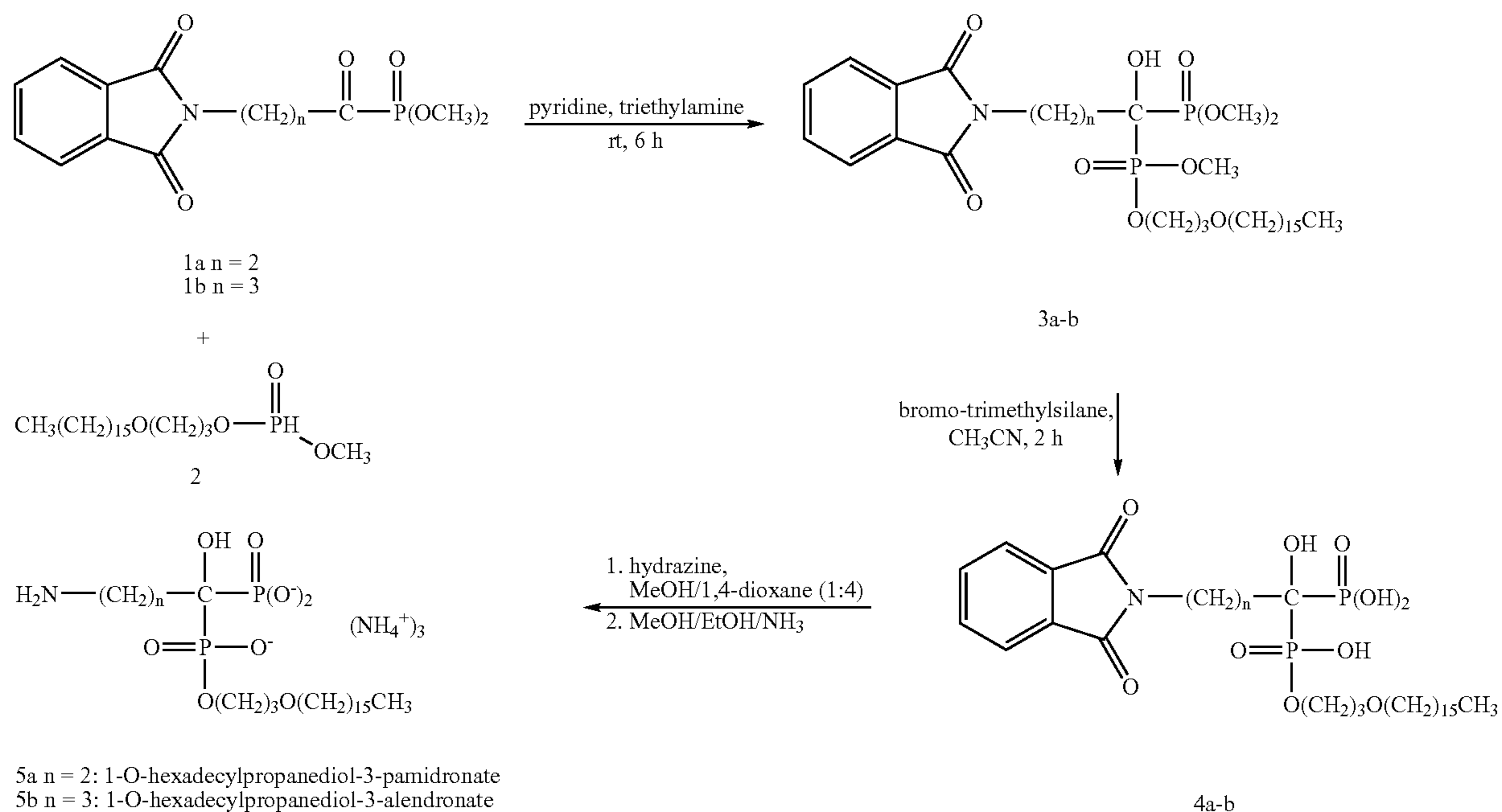
Scheme I
