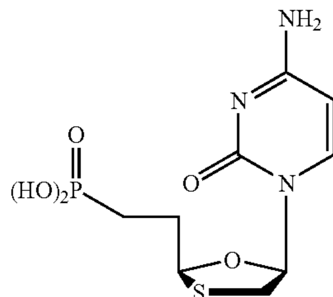
3'-thia-2',3'-dideoxycytidine-5'-phosphonic acid
