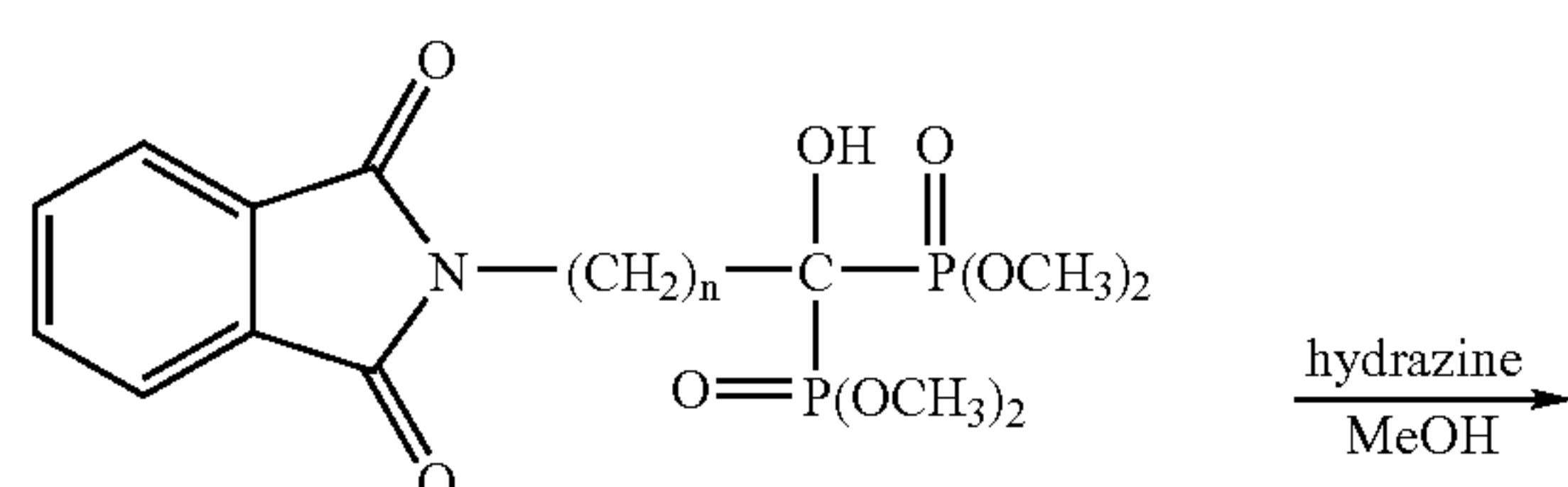
Scheme IV
