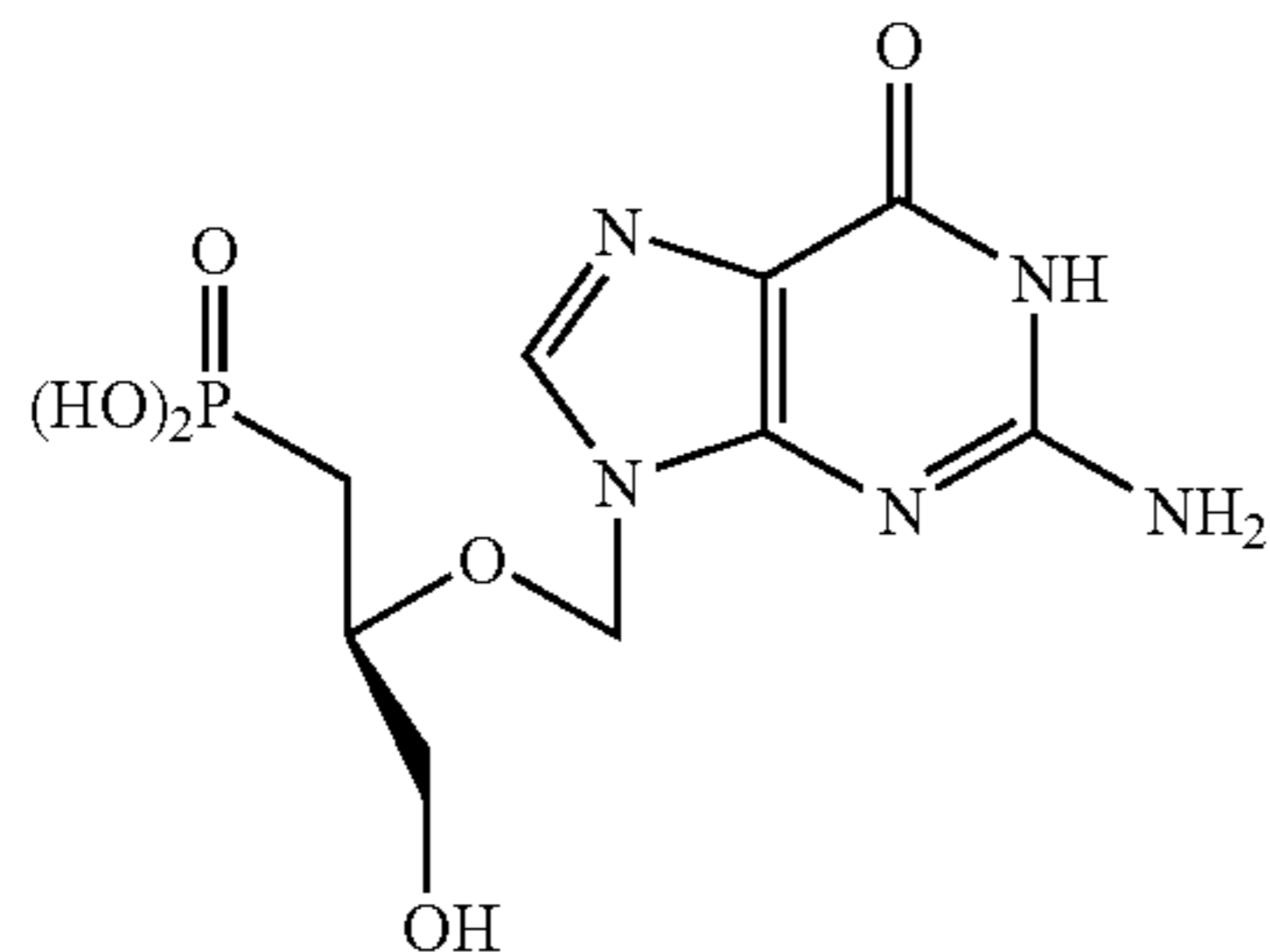
Ganciclovir phosphonate
