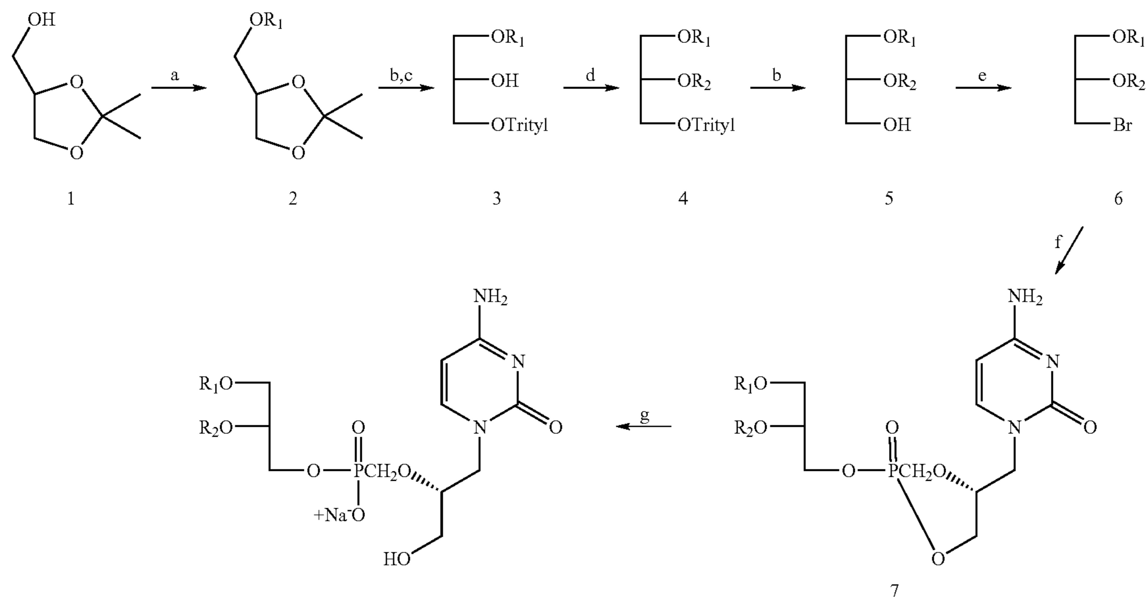
Scheme V
