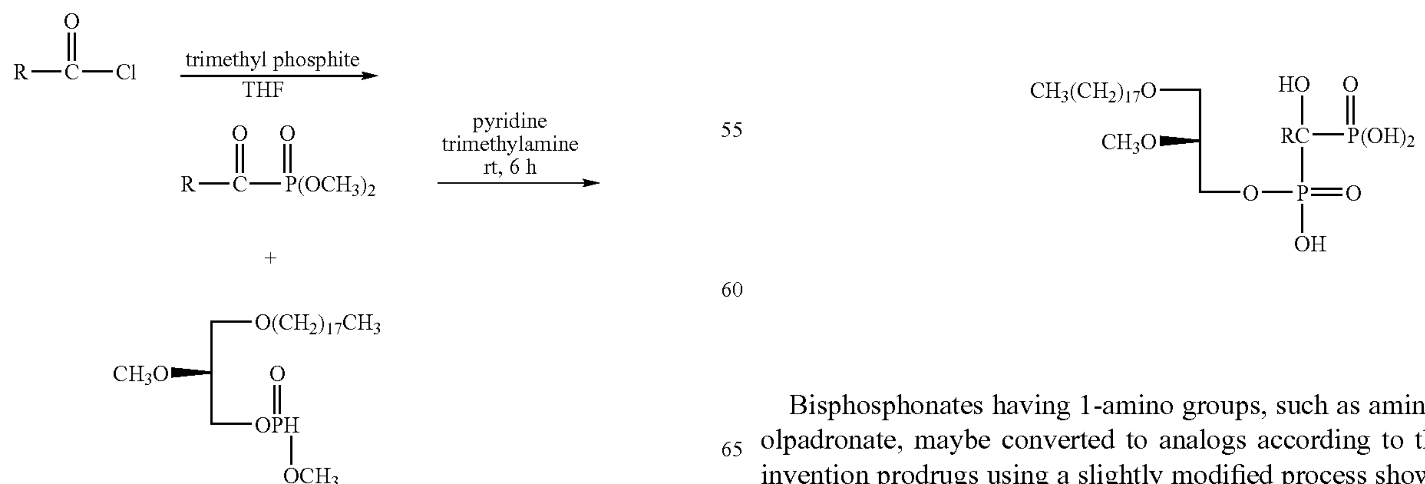
Scheme II
