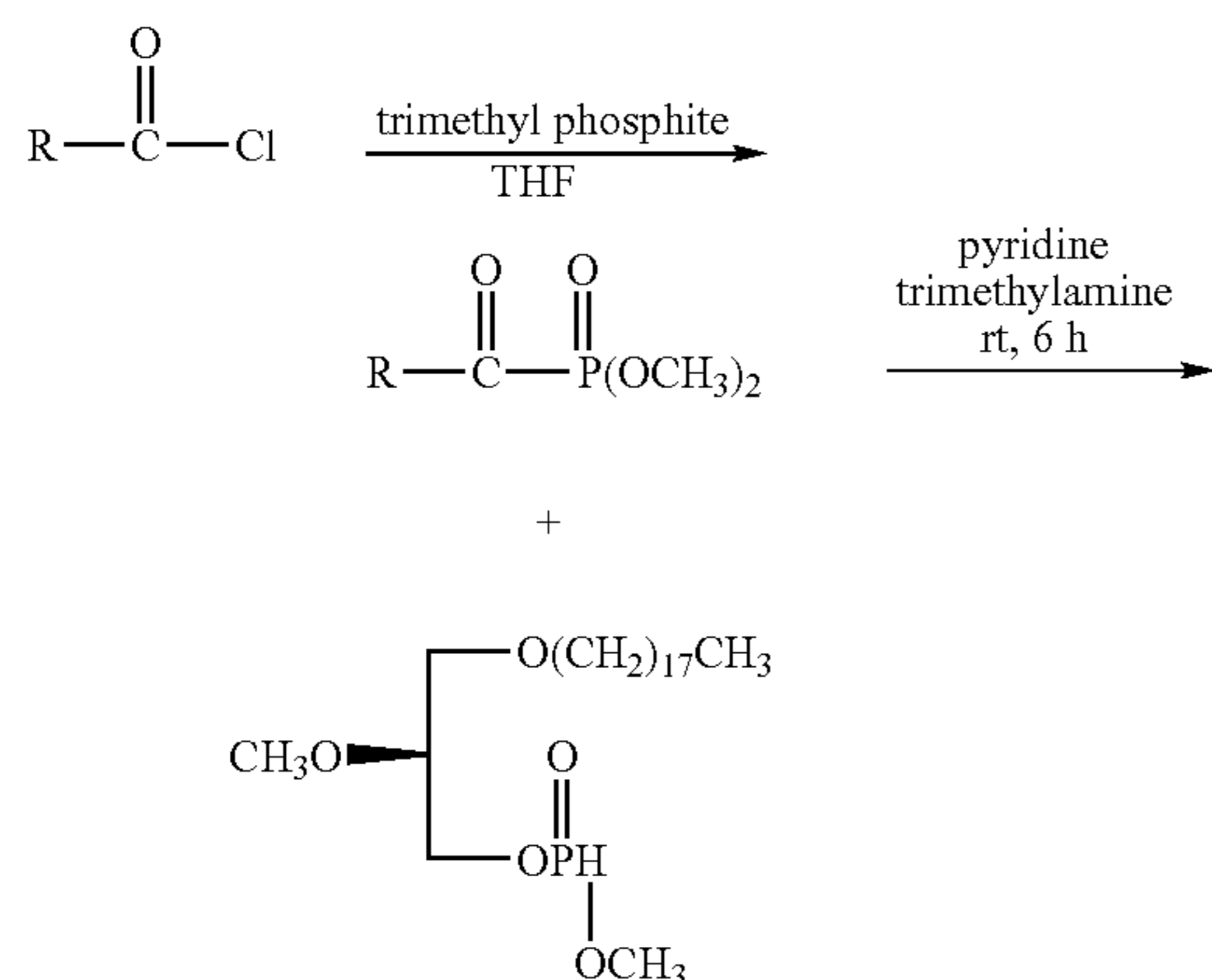
Scheme II
