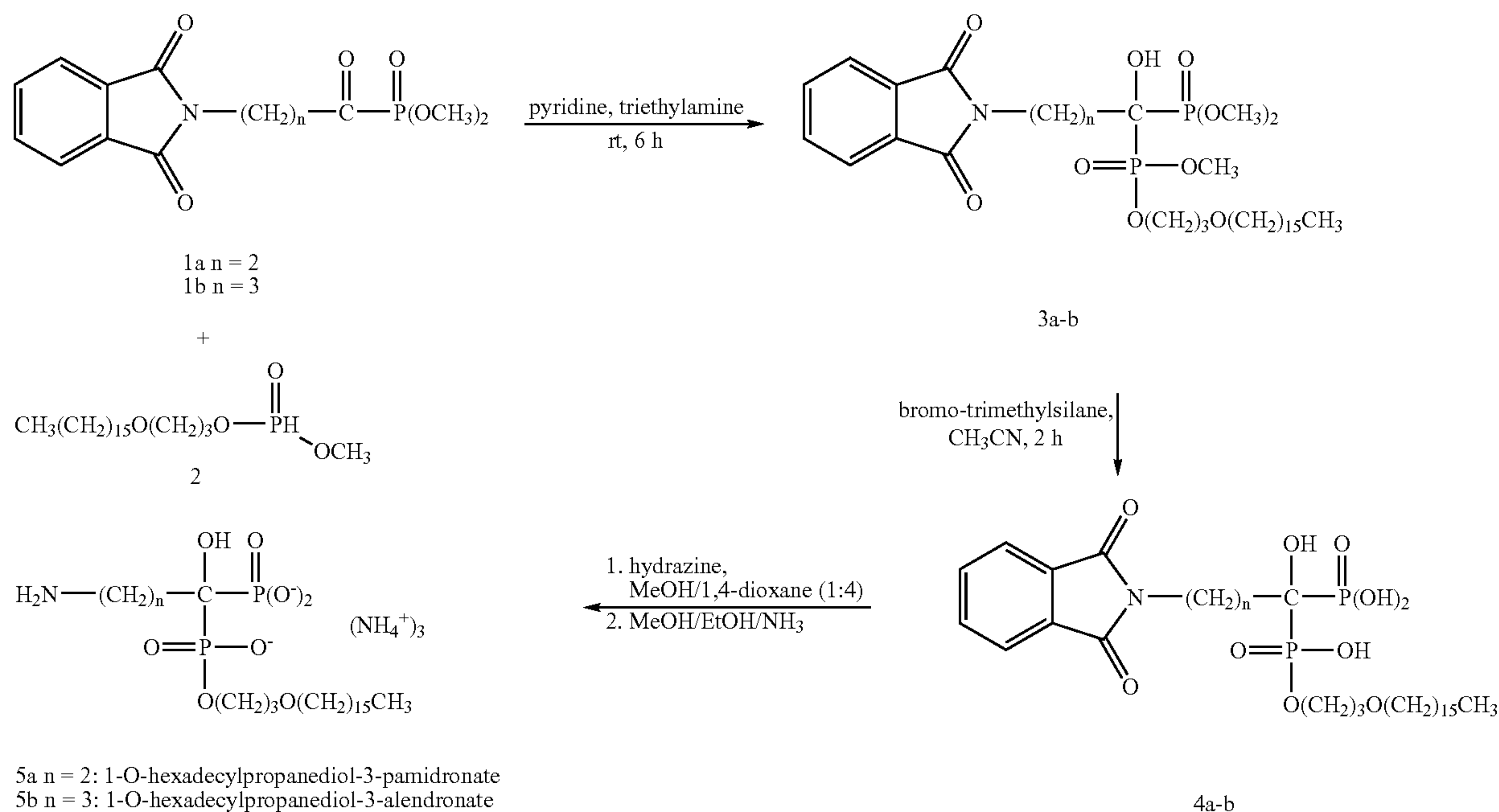
Scheme I
