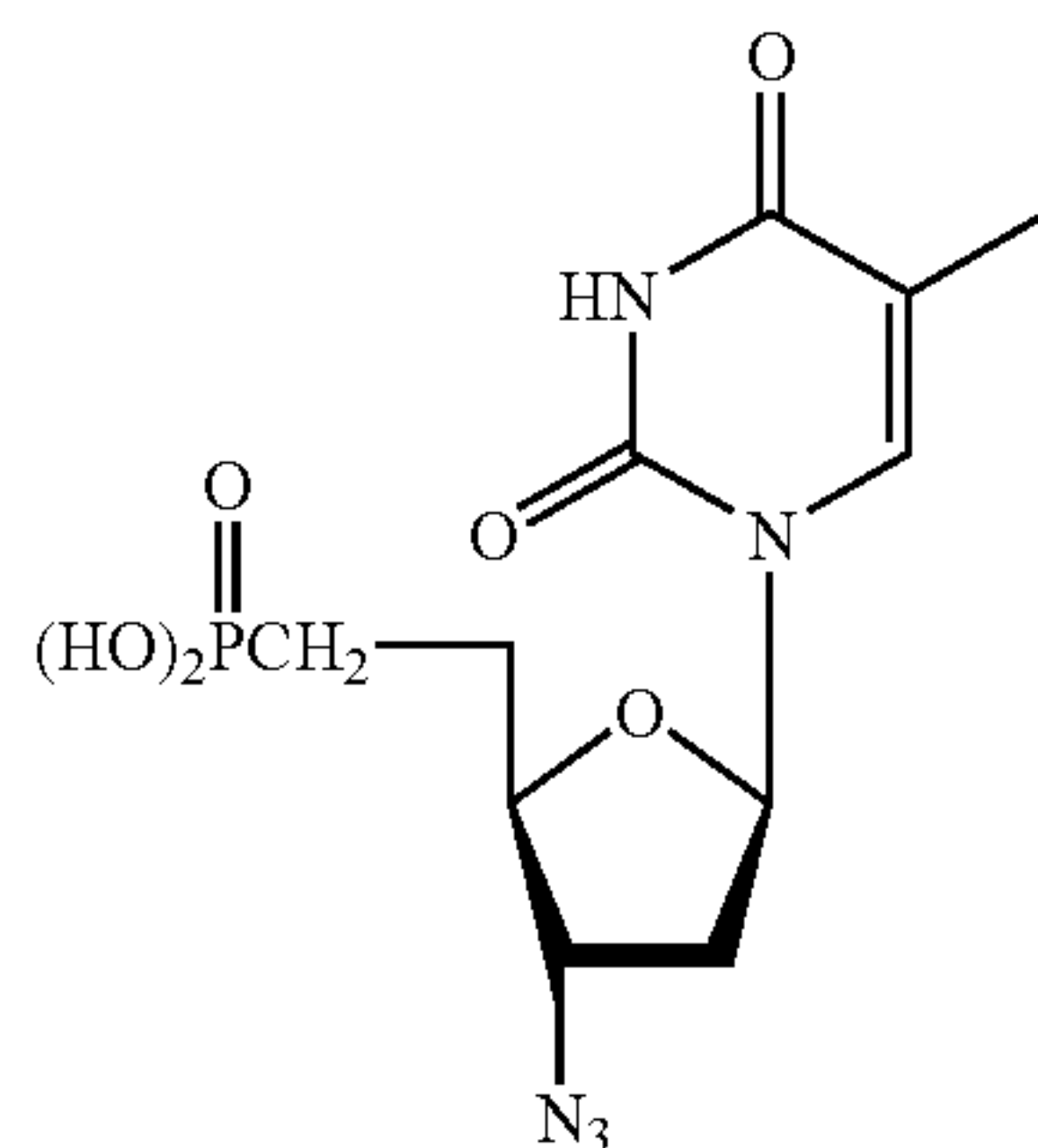
AZT 5'-methylene-phosphonate
