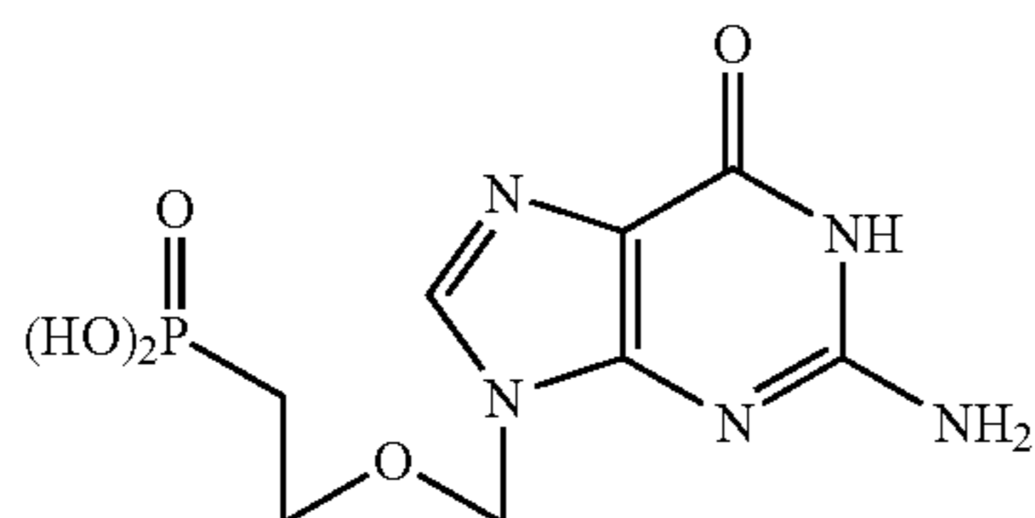
Acyclovir phosphonate
