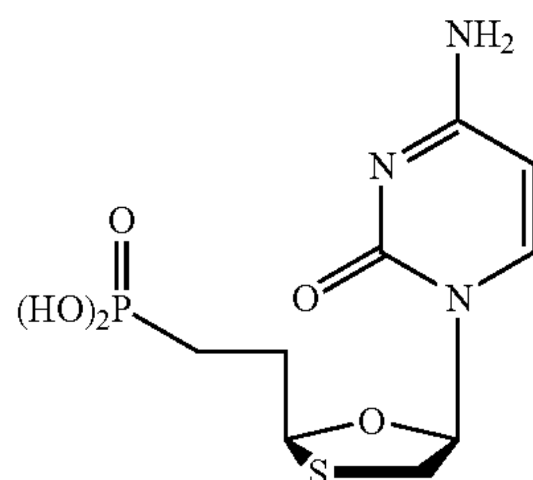
3'-thia-2',3'-dideoxycytidine-5'-phosphonic acid
