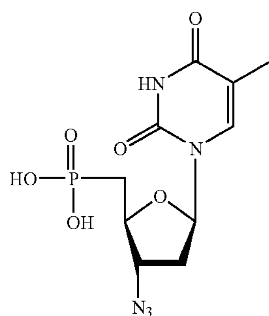
AZT 5'-phosphonate
