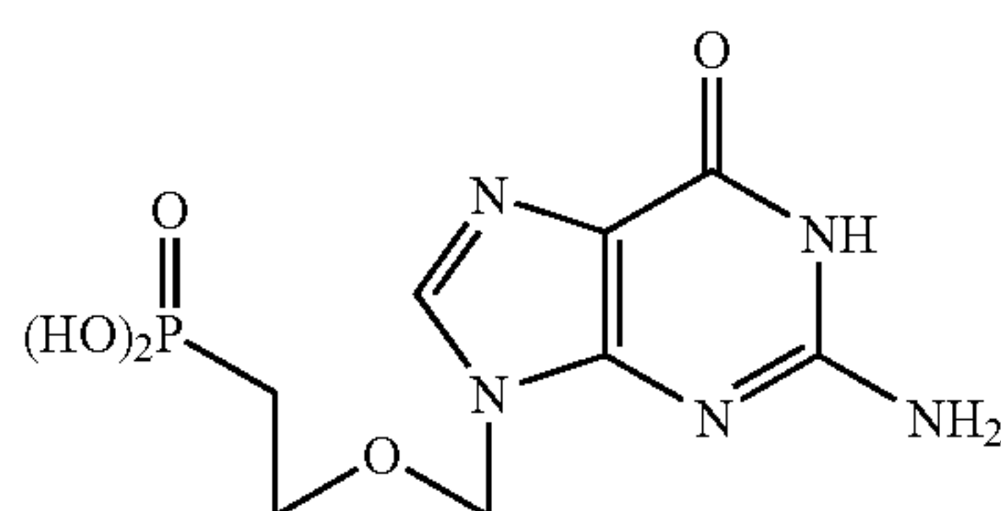
Acyclovir phosphonate
