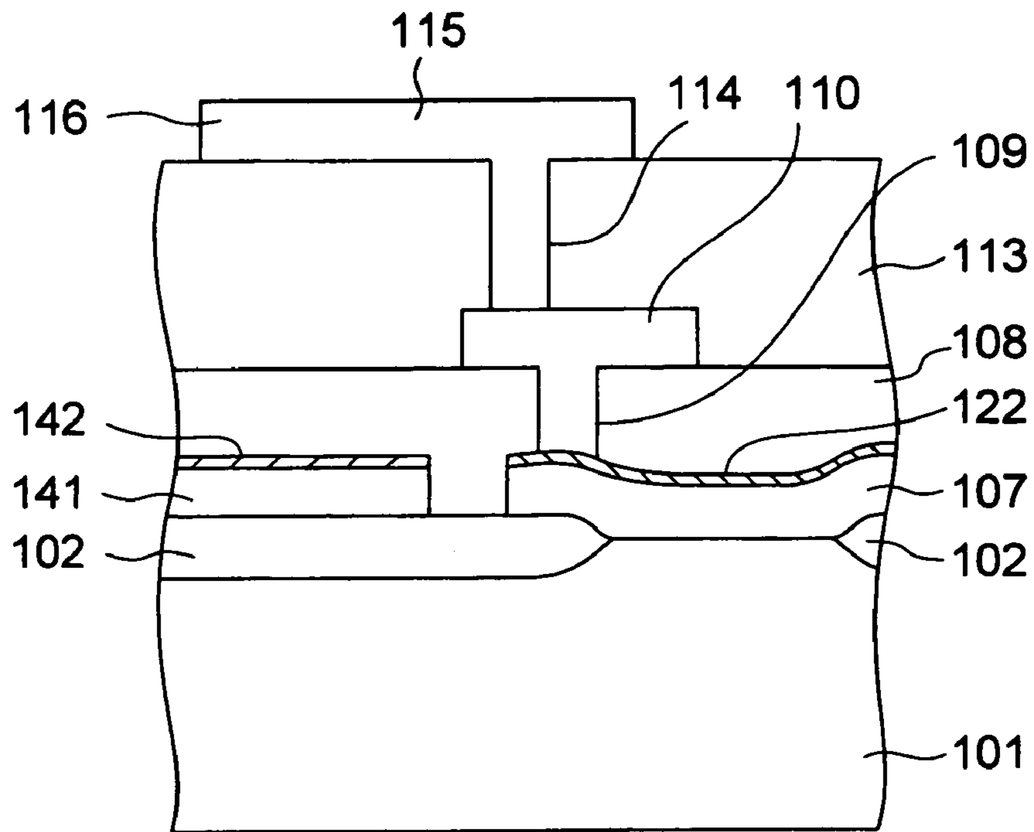
FIG. 6A c-c' SECTION
