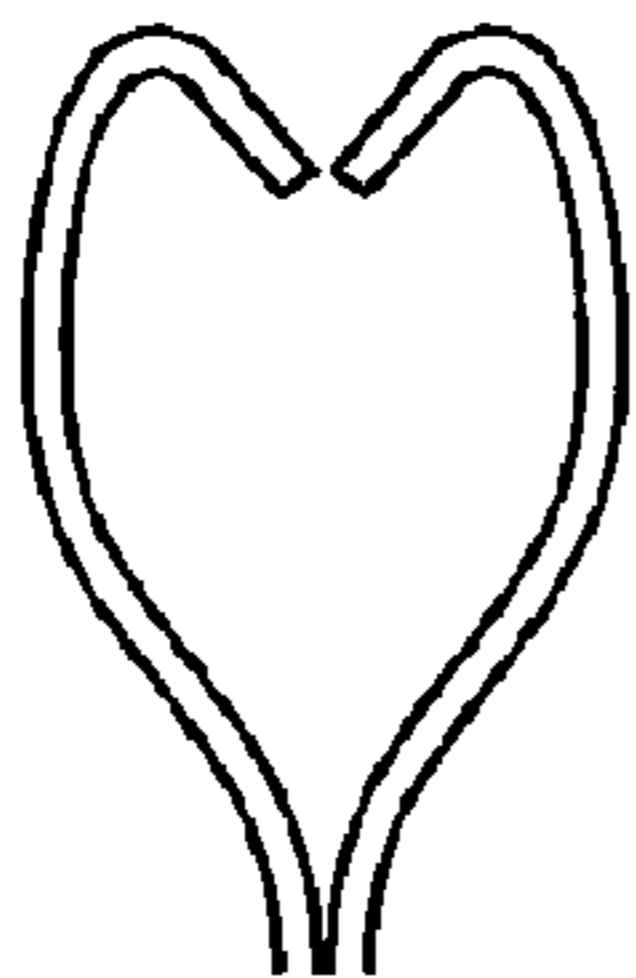
Parallel-Negative Angle
