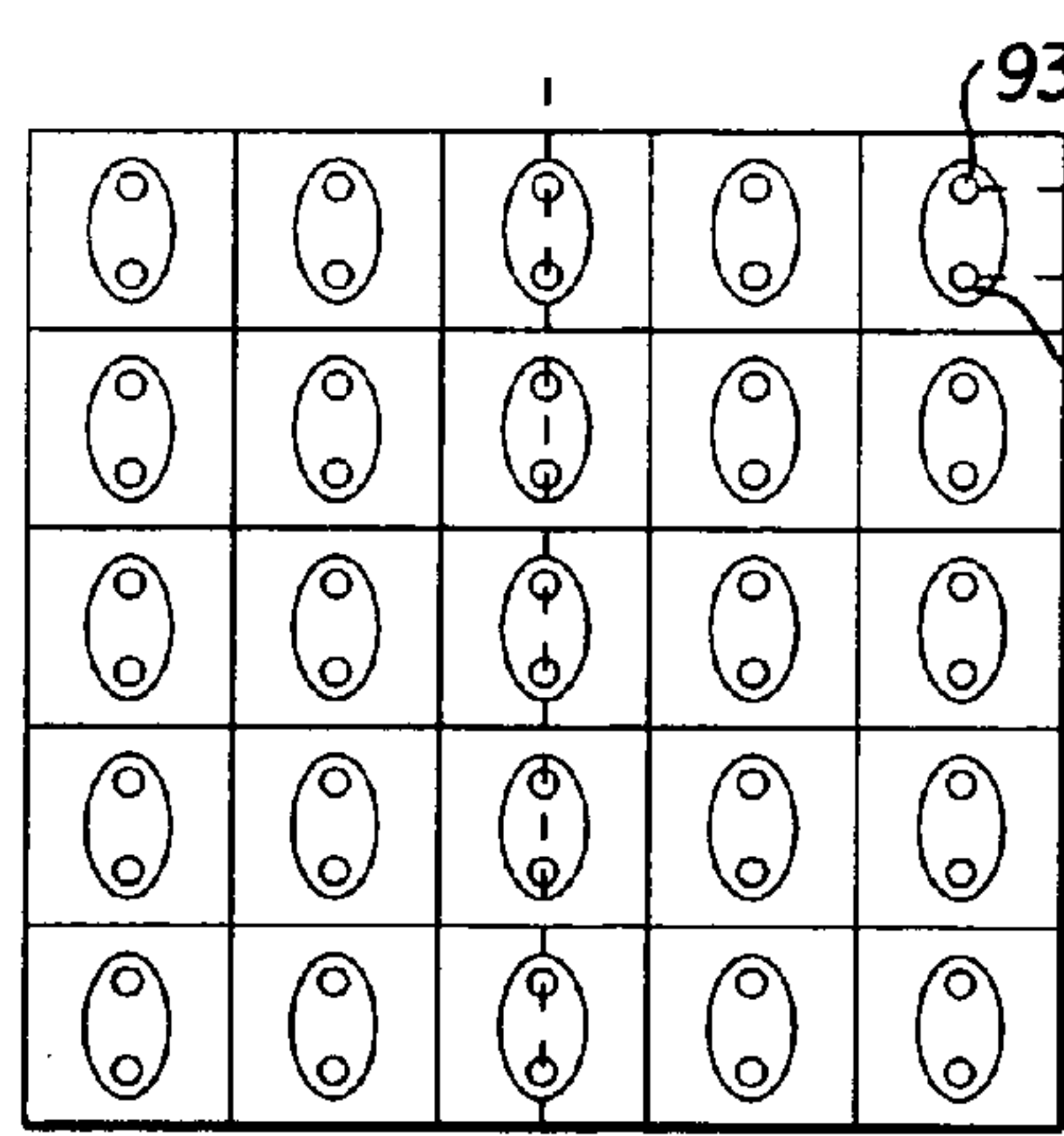
FIG. 9C (PRIOR ART)
