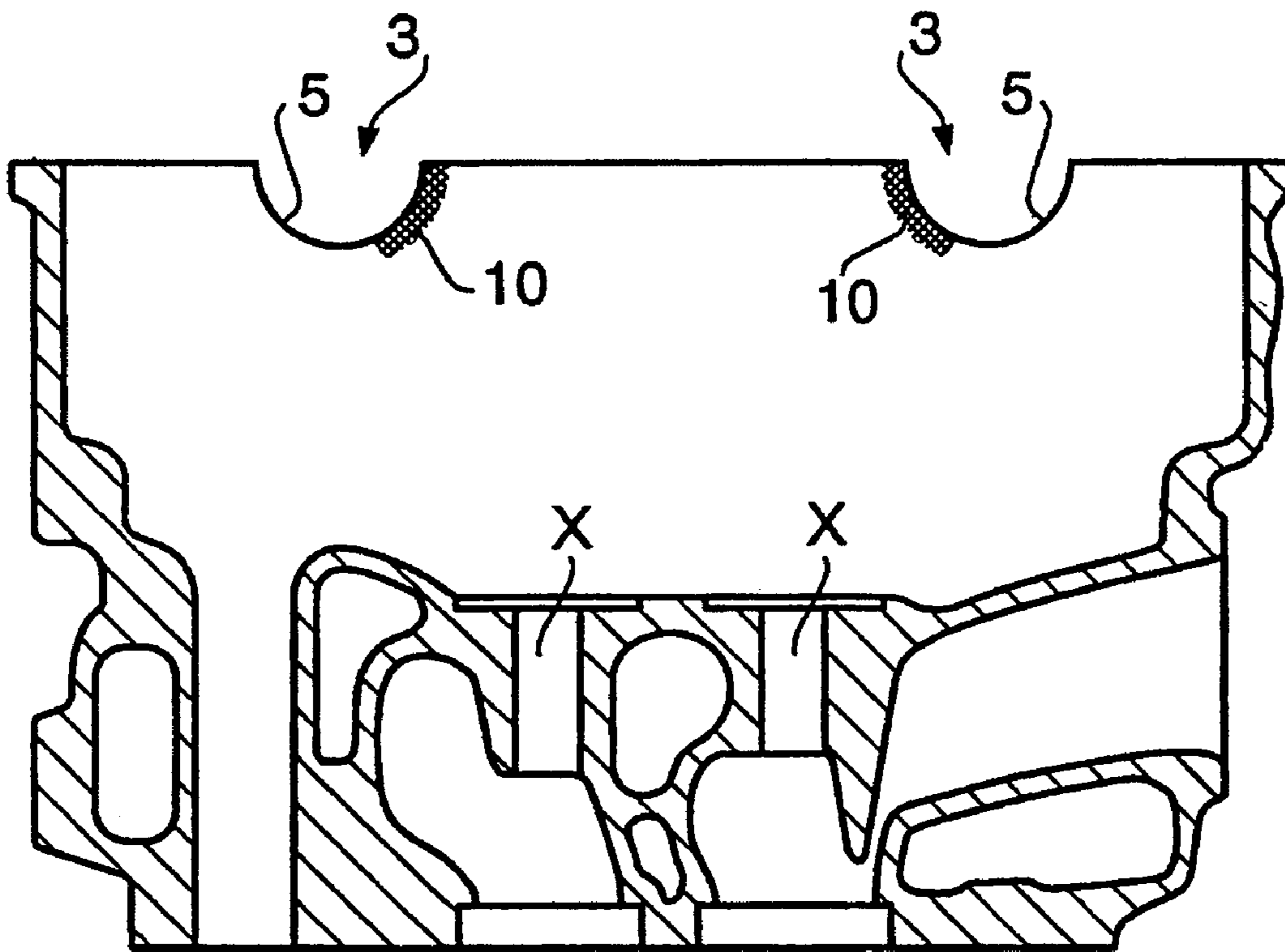
FIG. 7 Prior Art
