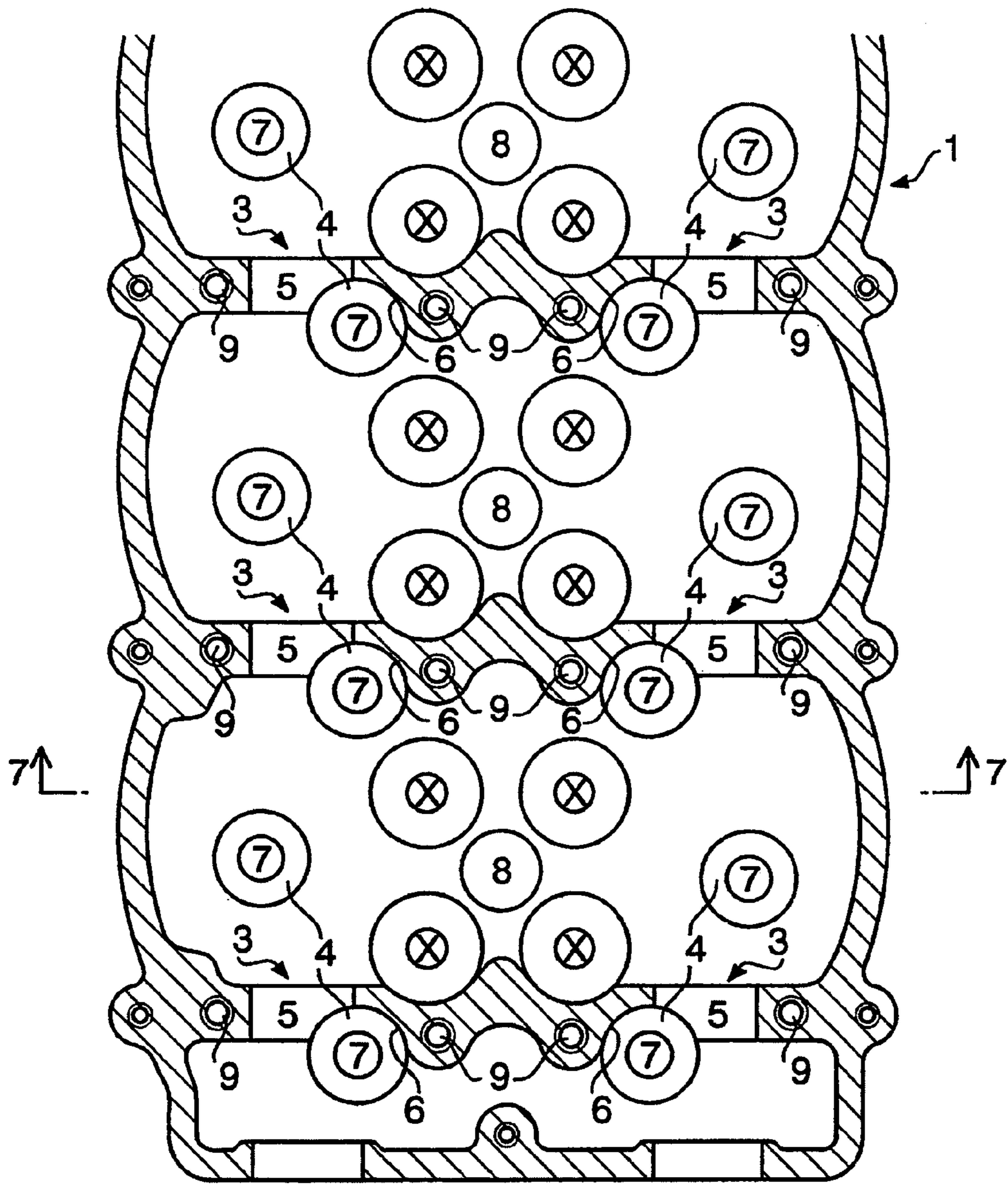
FIG. 6 Prior Art
