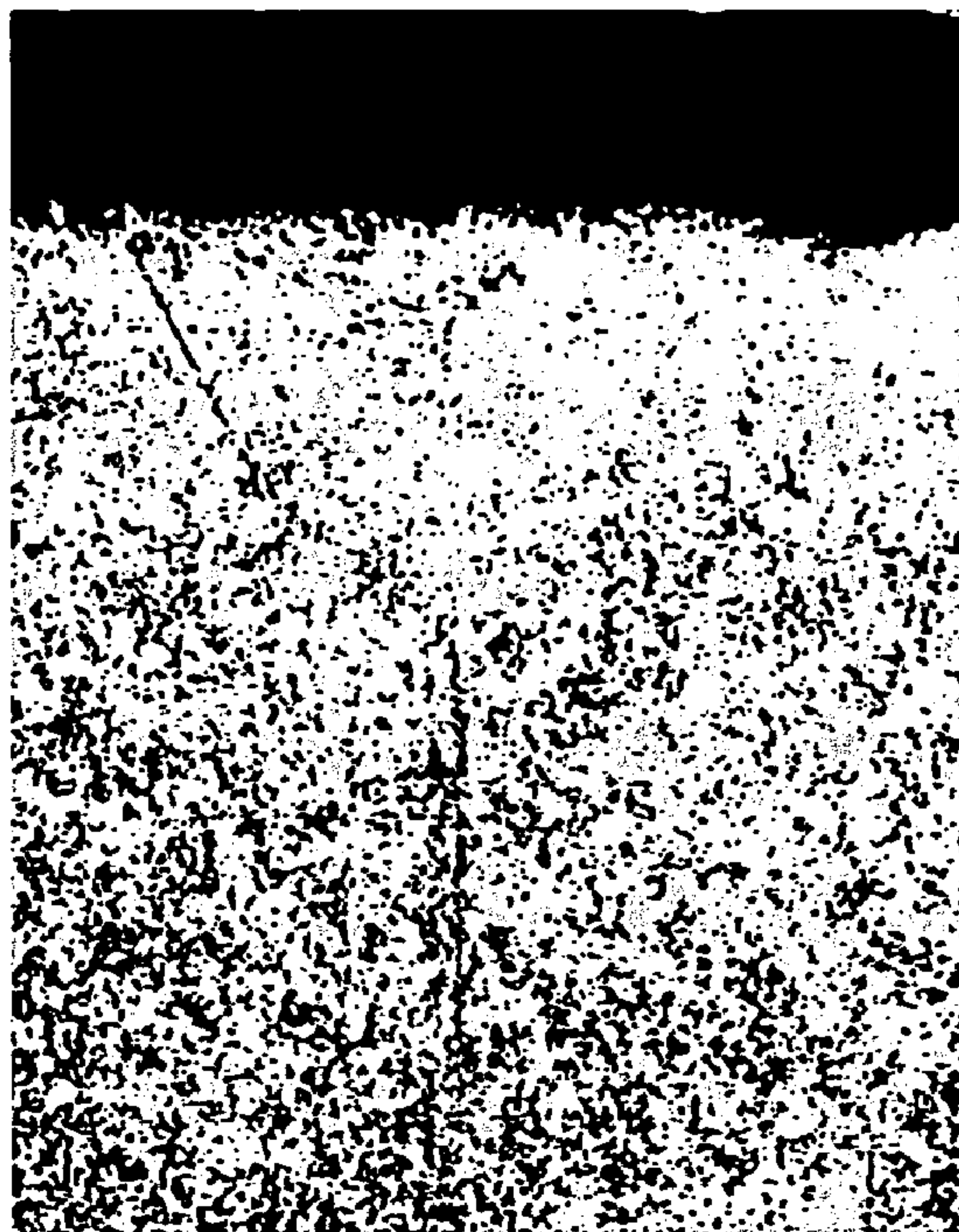
PRIOR TO SPHERODIZING ANNEALING SURFACE LAYER X 100
