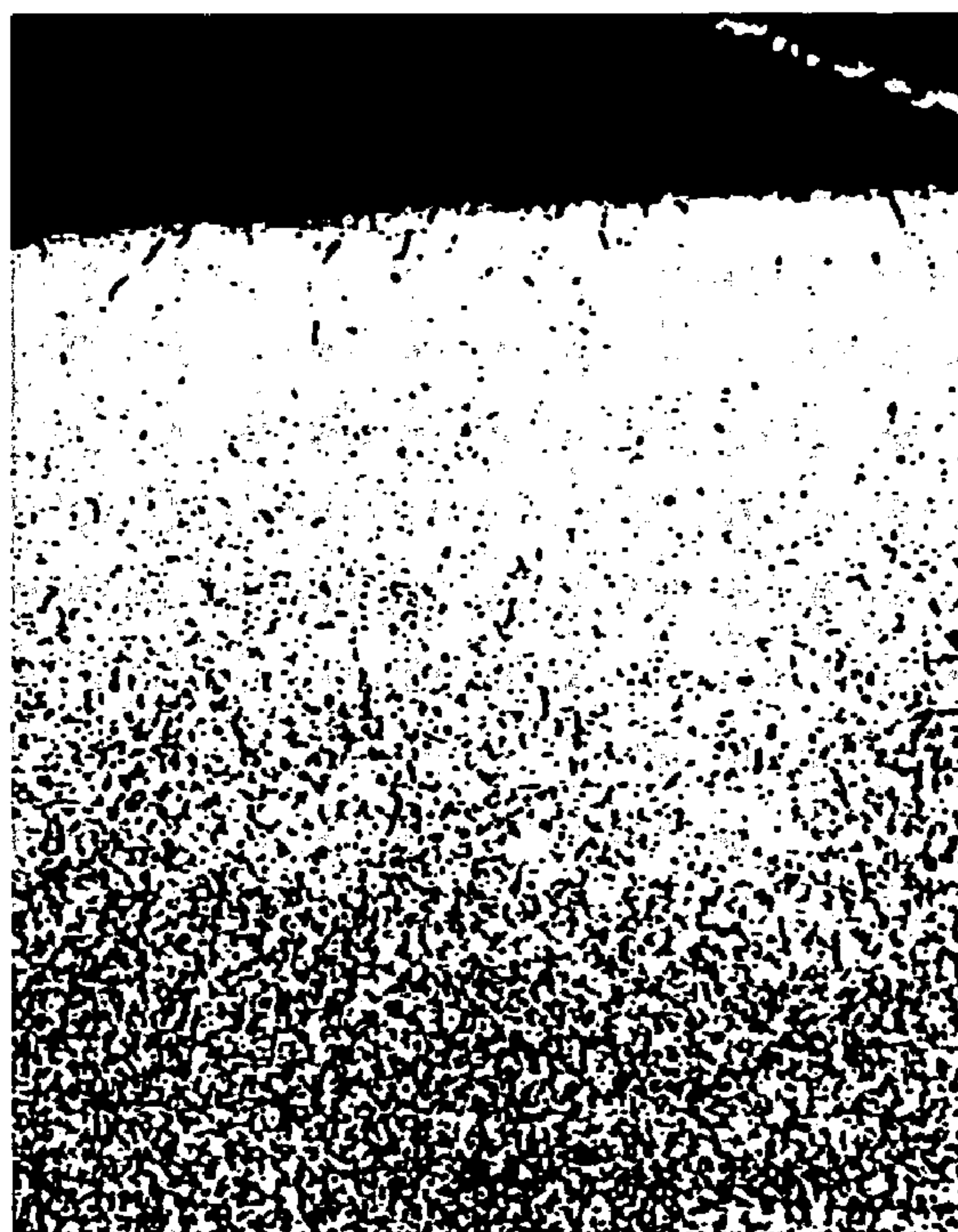
AFTER SPHERODIZING ANNEALING PATTERN 2 SURFACE LAYER X 100
