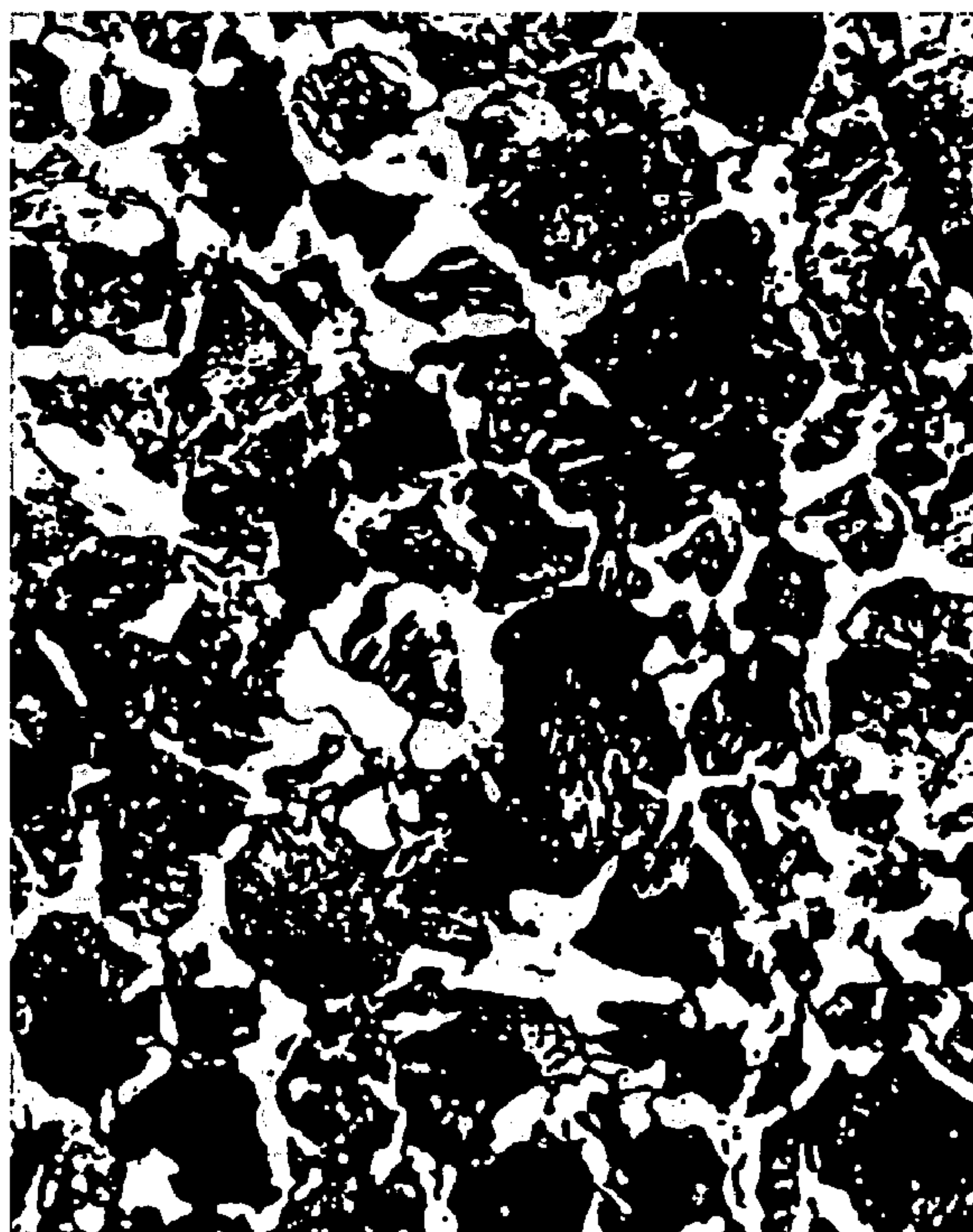
PRIOR TO SPHERODIZING ANNEALING CENTRAL PART X 400
