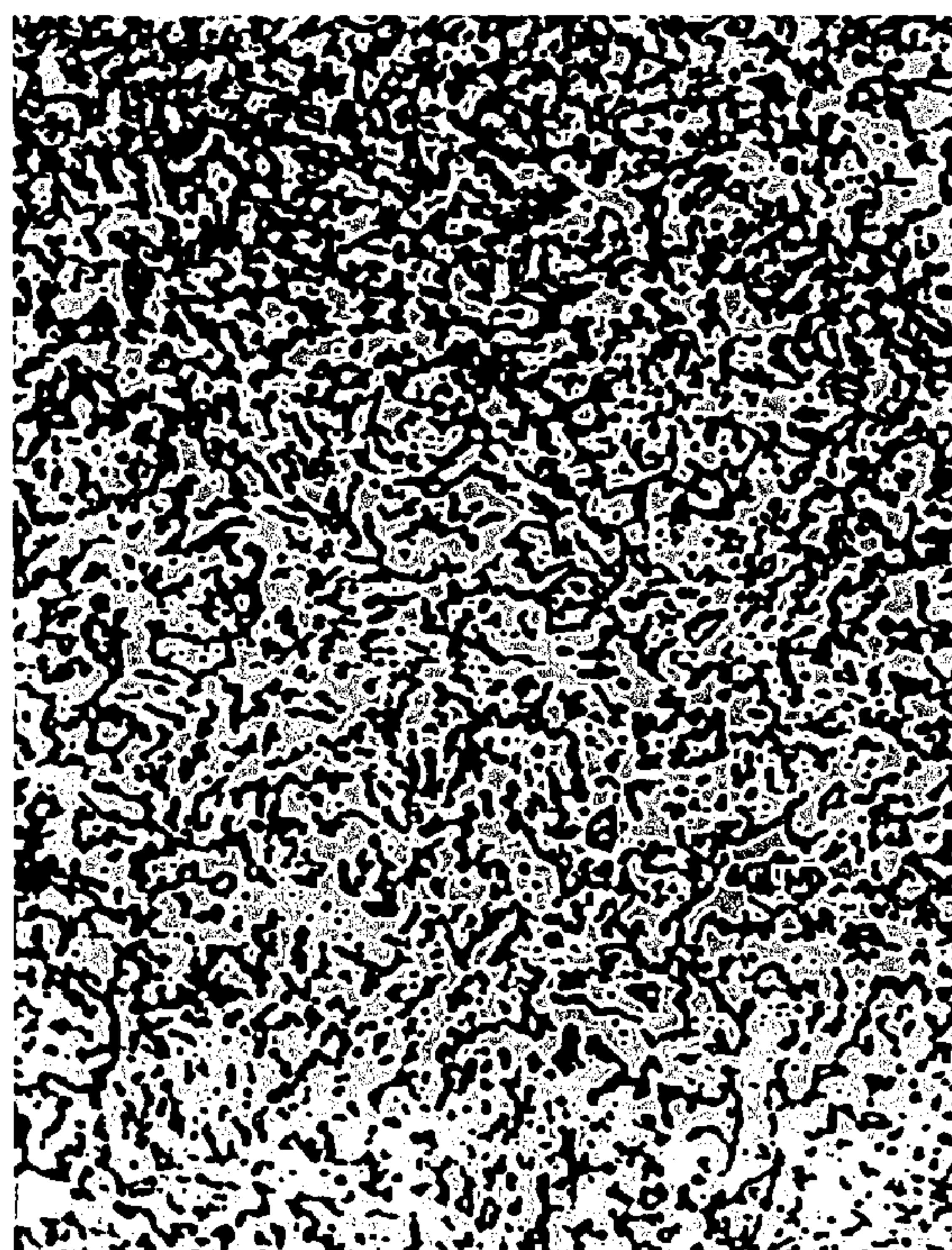
AFTER SPHERODIZING ANNEALING PATTERN 1 SURFACE LAYER X 400
