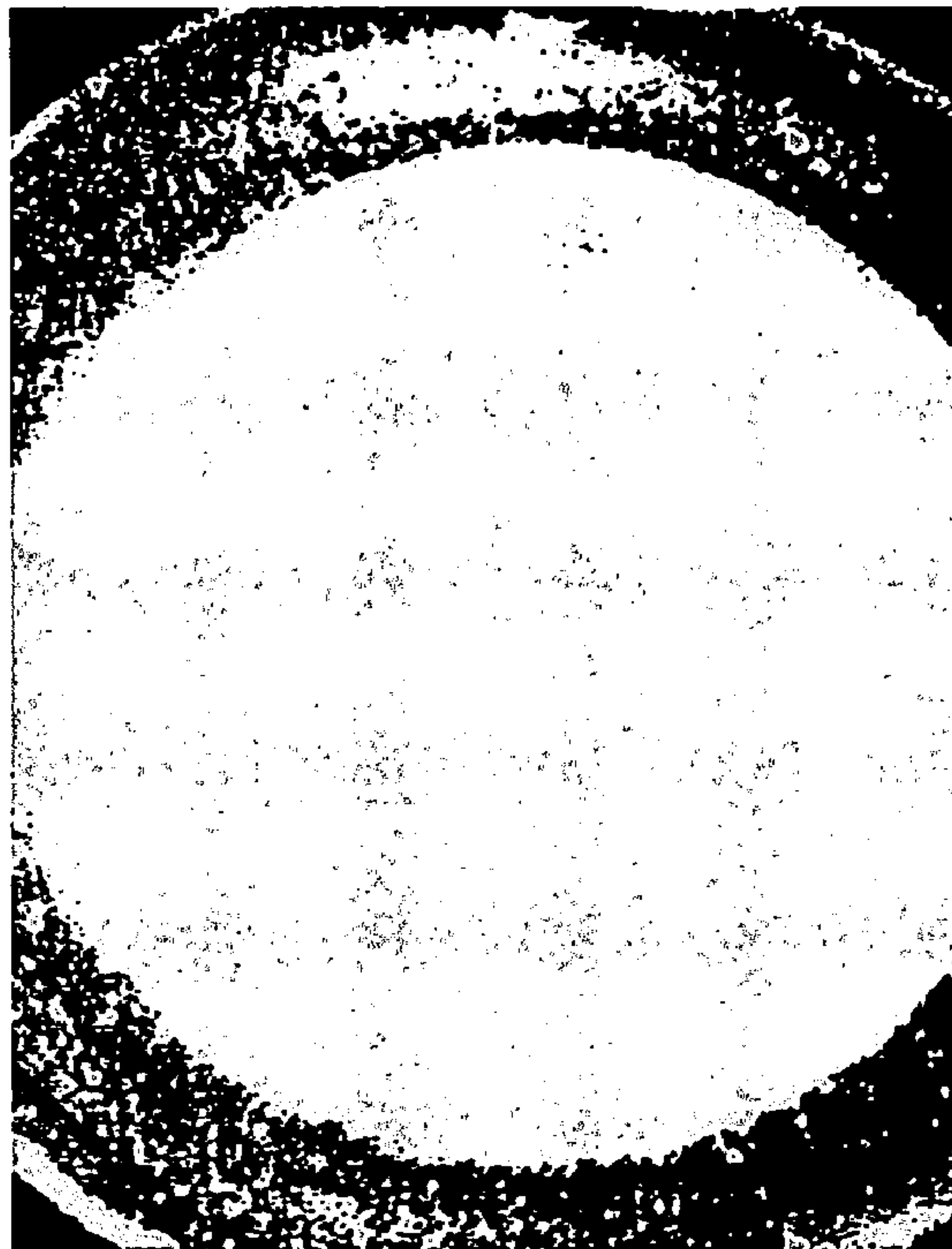
MARTENSITIC MATERIAL AFTER SPHERODIZING ANNEALING PATTERN 1 X2.1
