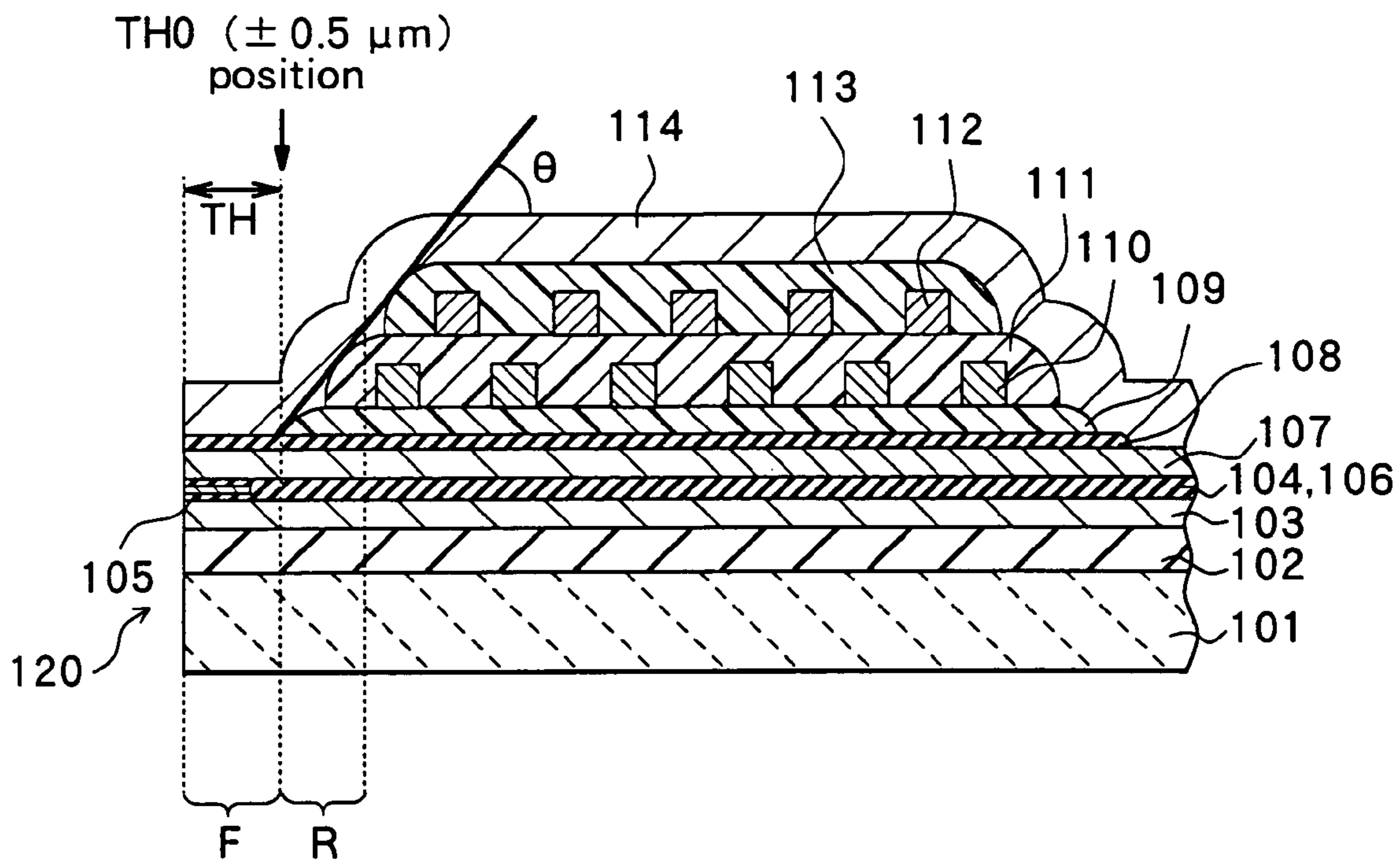
FIG.33 RELATED ART
