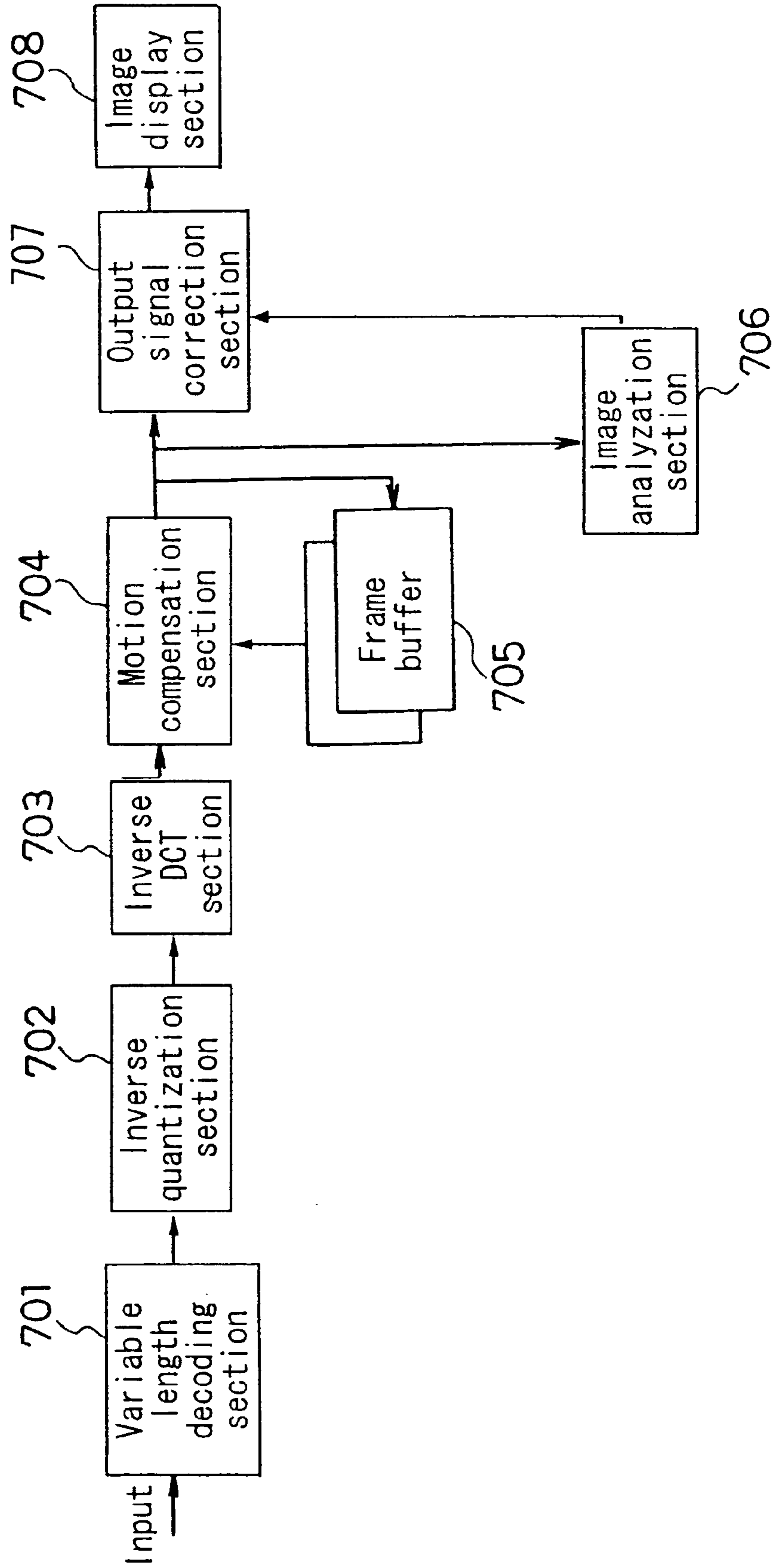
FIG. 7 (PRIOR ART)
