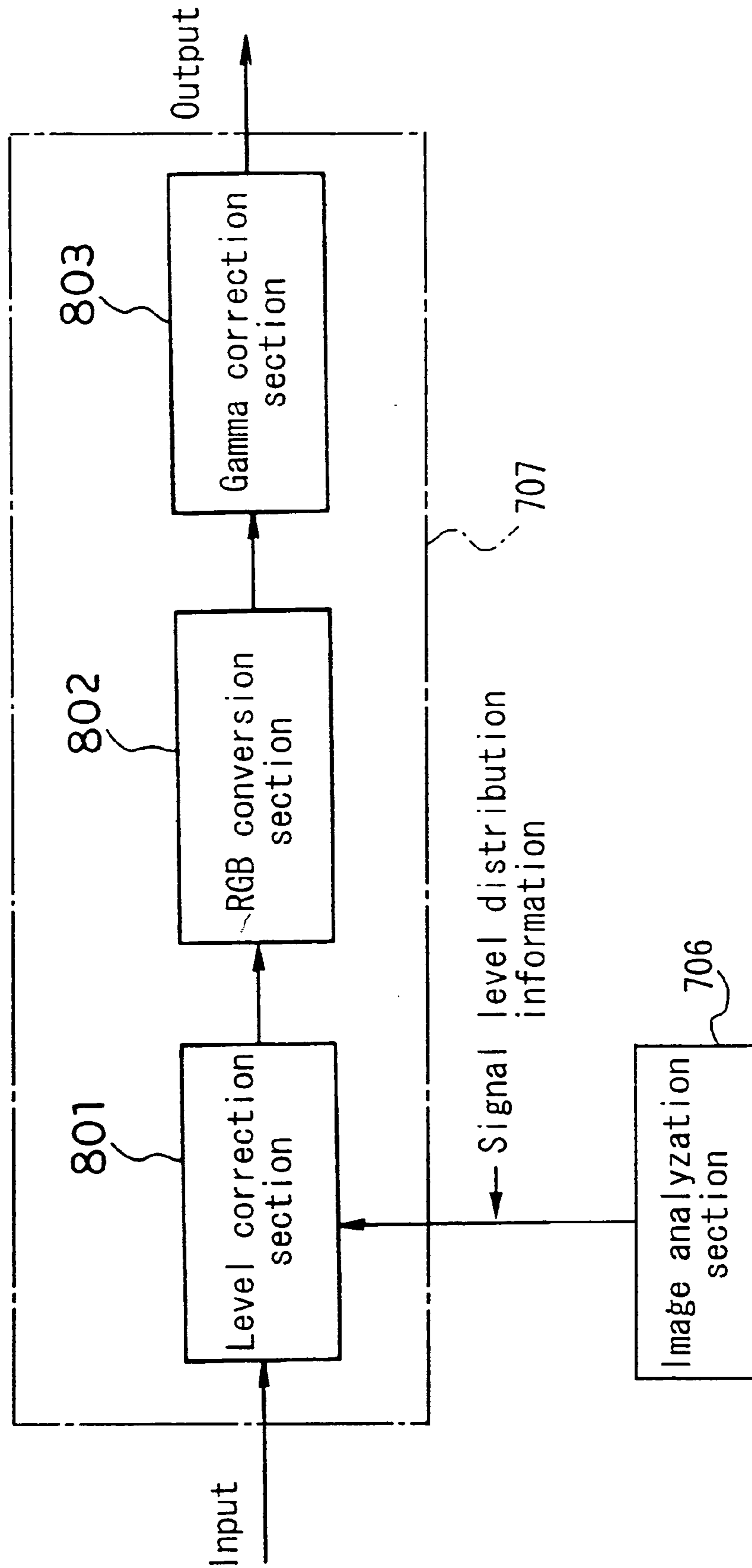
FIG. 8 (PRIOR ART)
