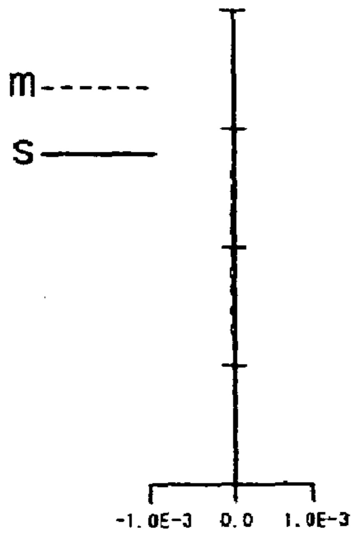
ASTIGMATISM
