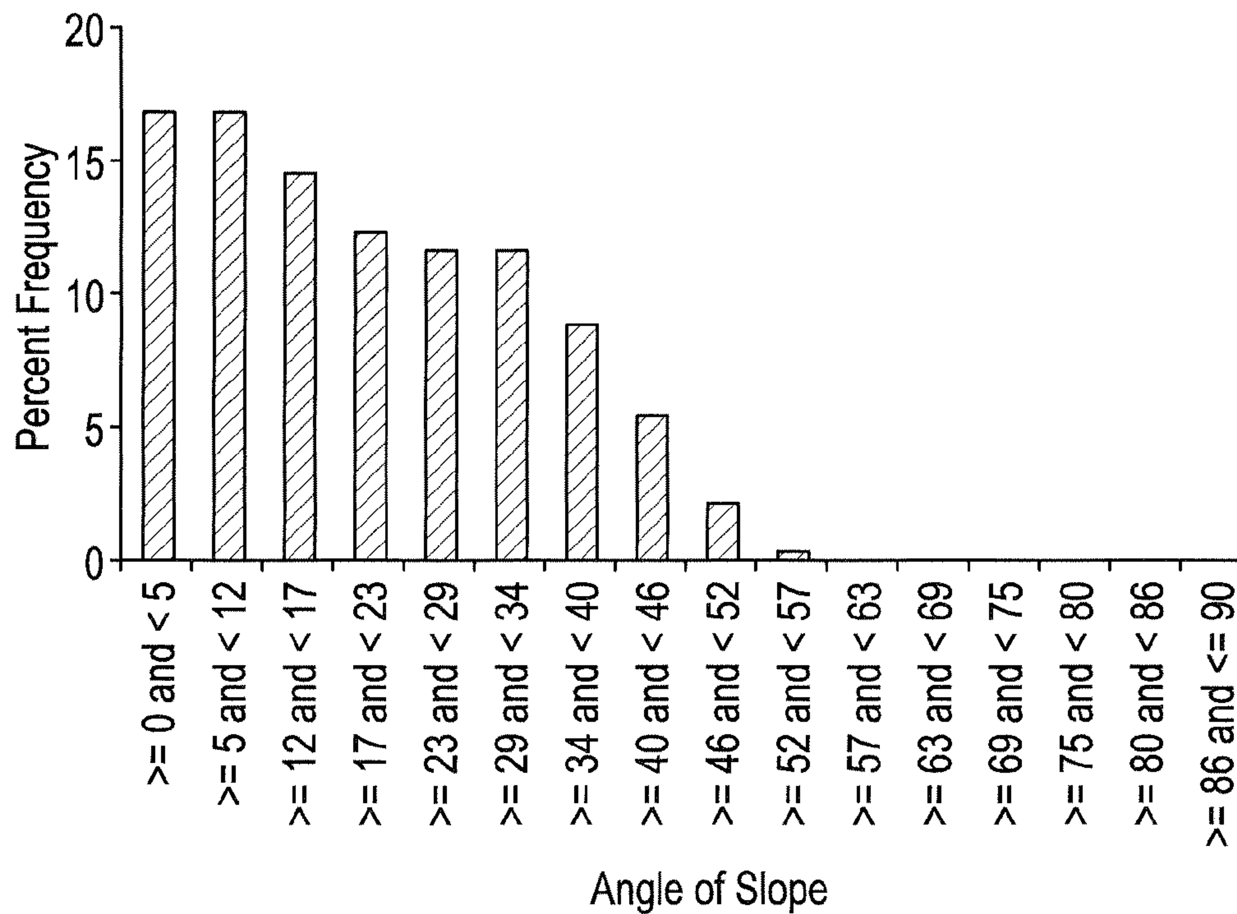
Polymer Film Front Surface Slope Distribution
