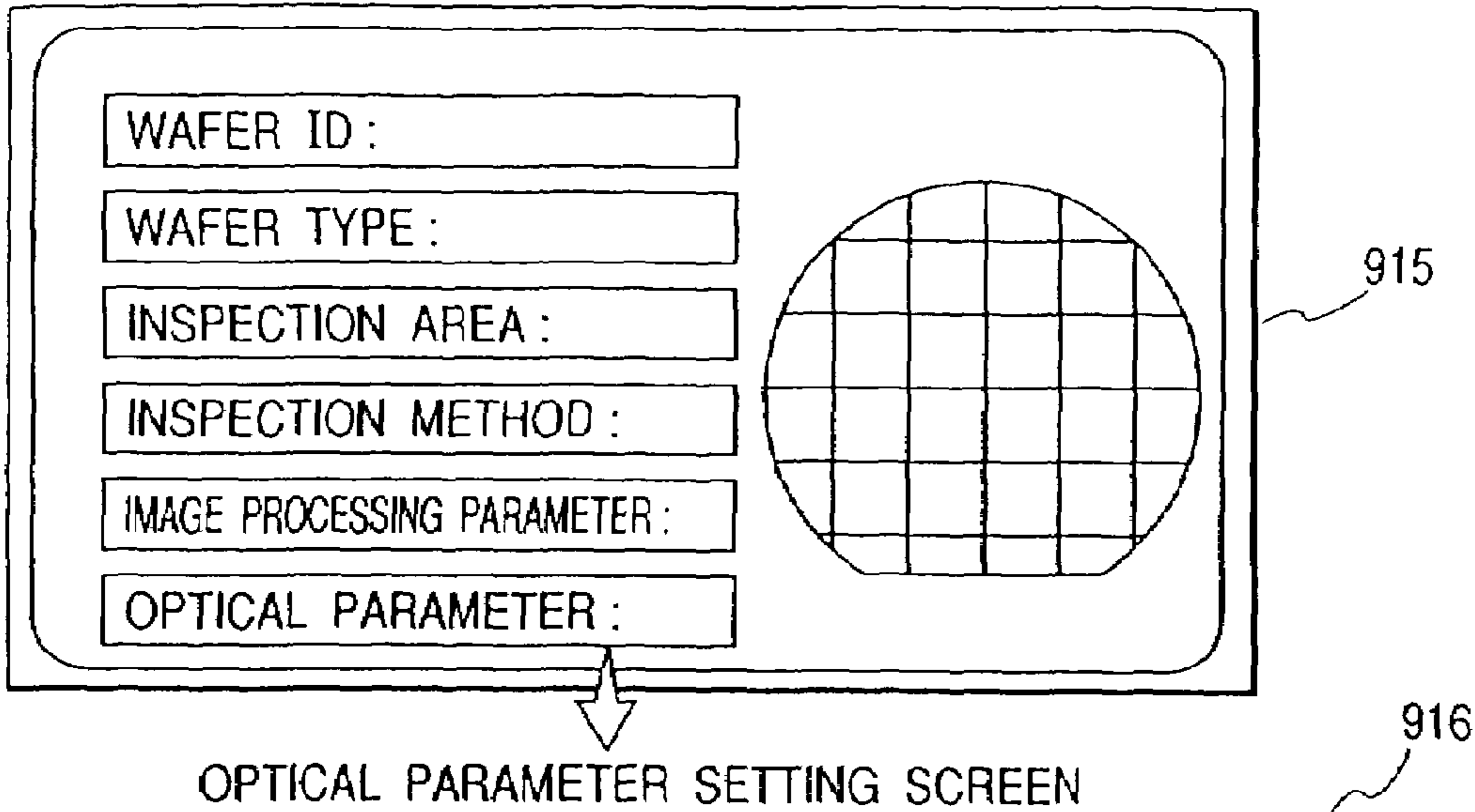
FIG. 6 RECIPE SCREEN
