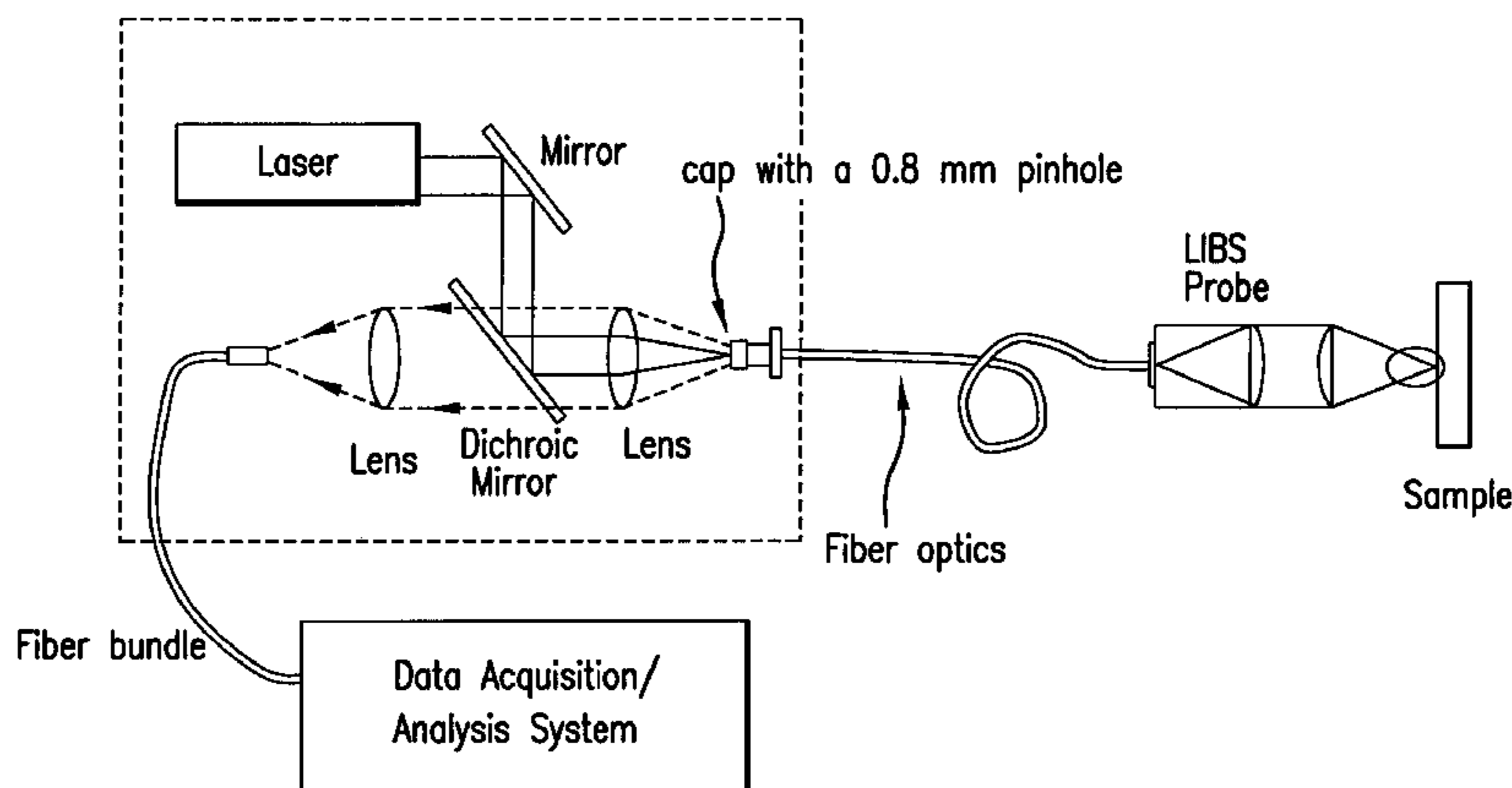
Diagram of LIBS setup.
