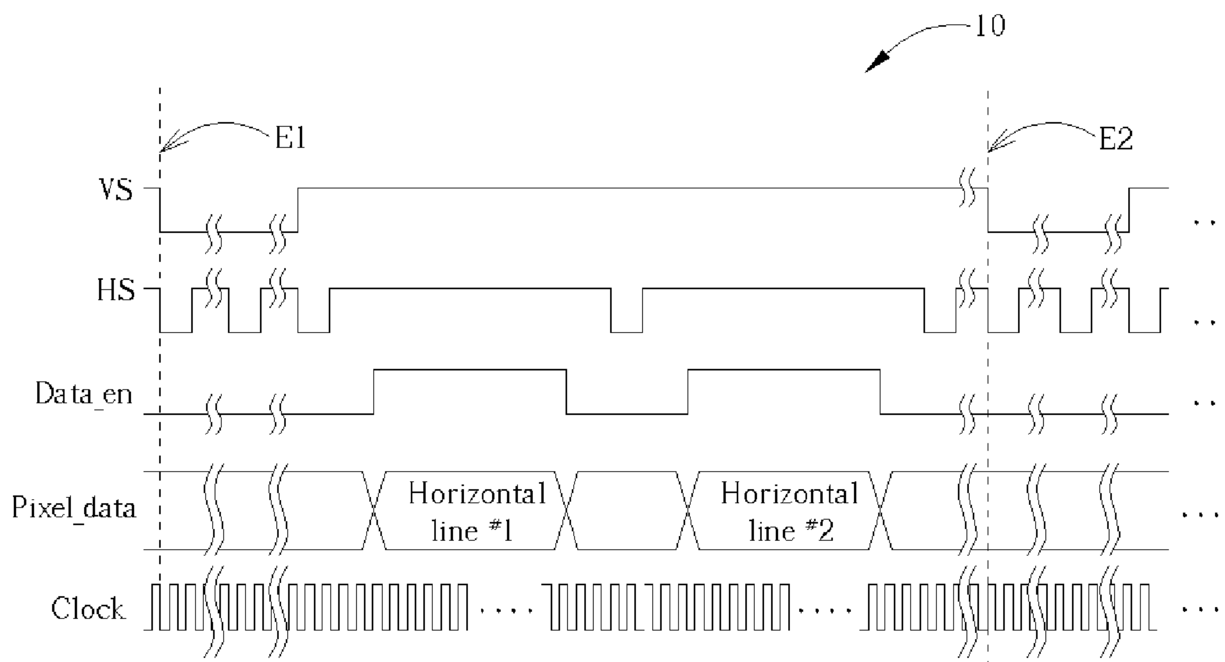
Fig. 1 Prior art
