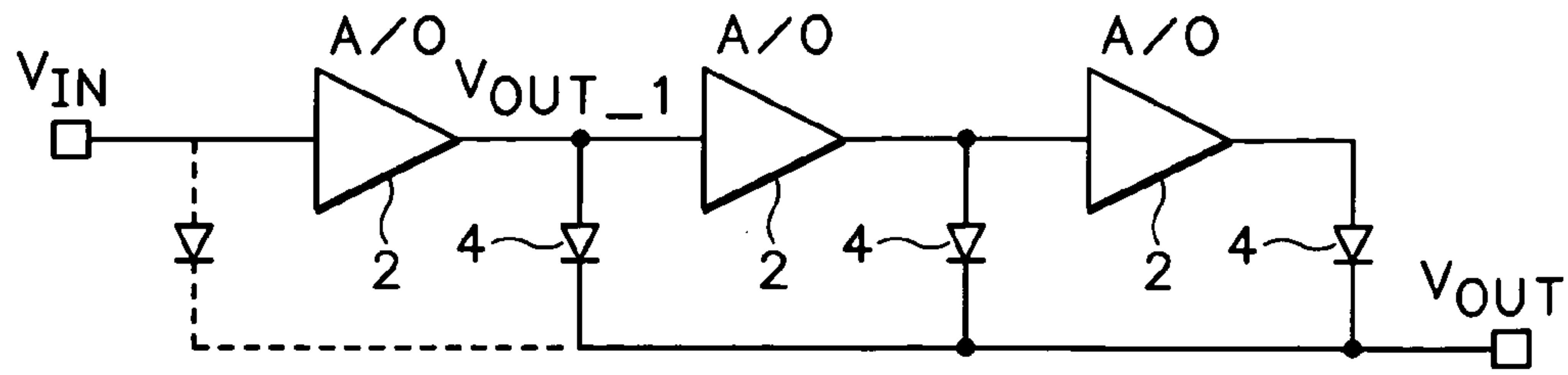
FIG.1 (PRIOR ART)
