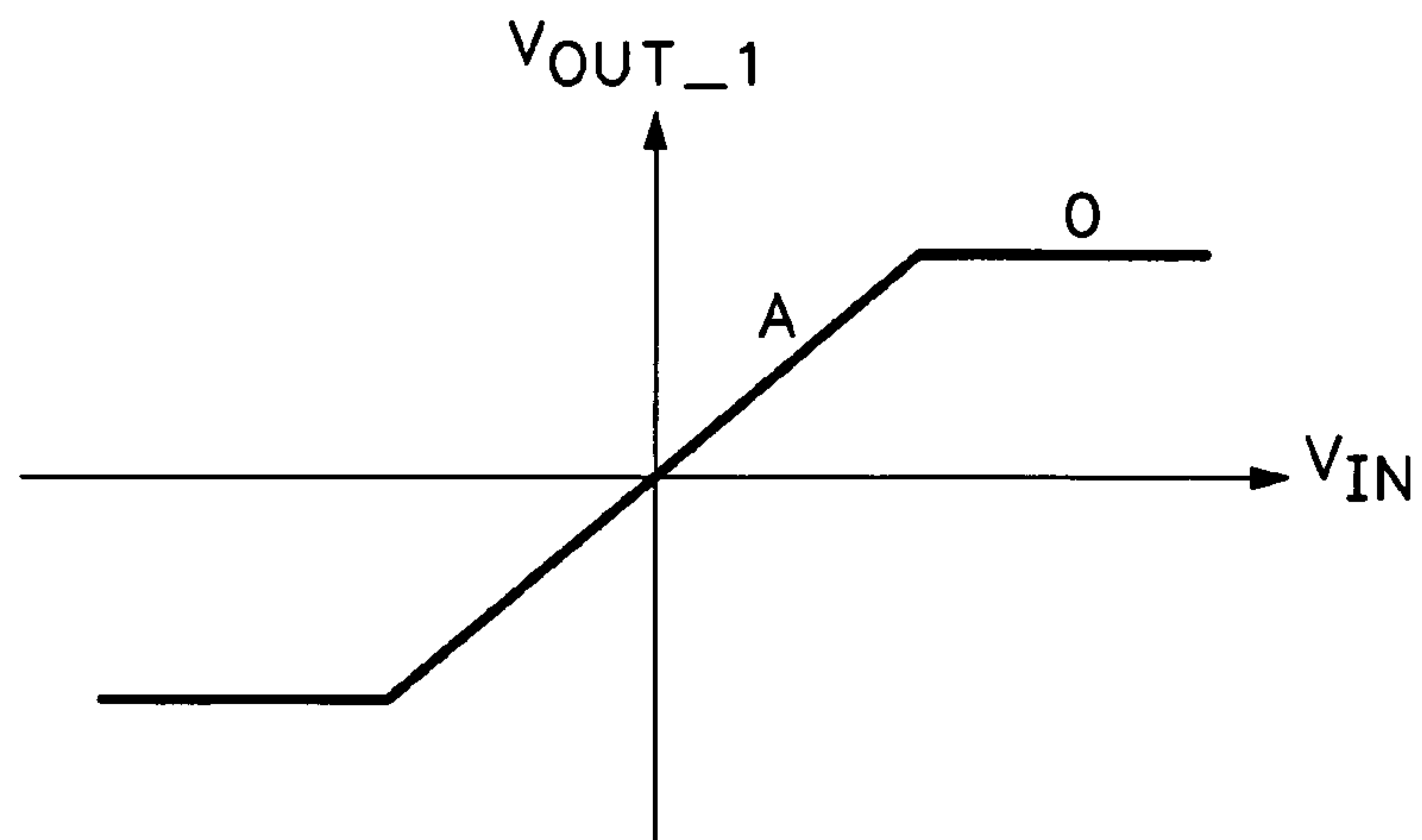
FIG.2 (PRIOR ART)
