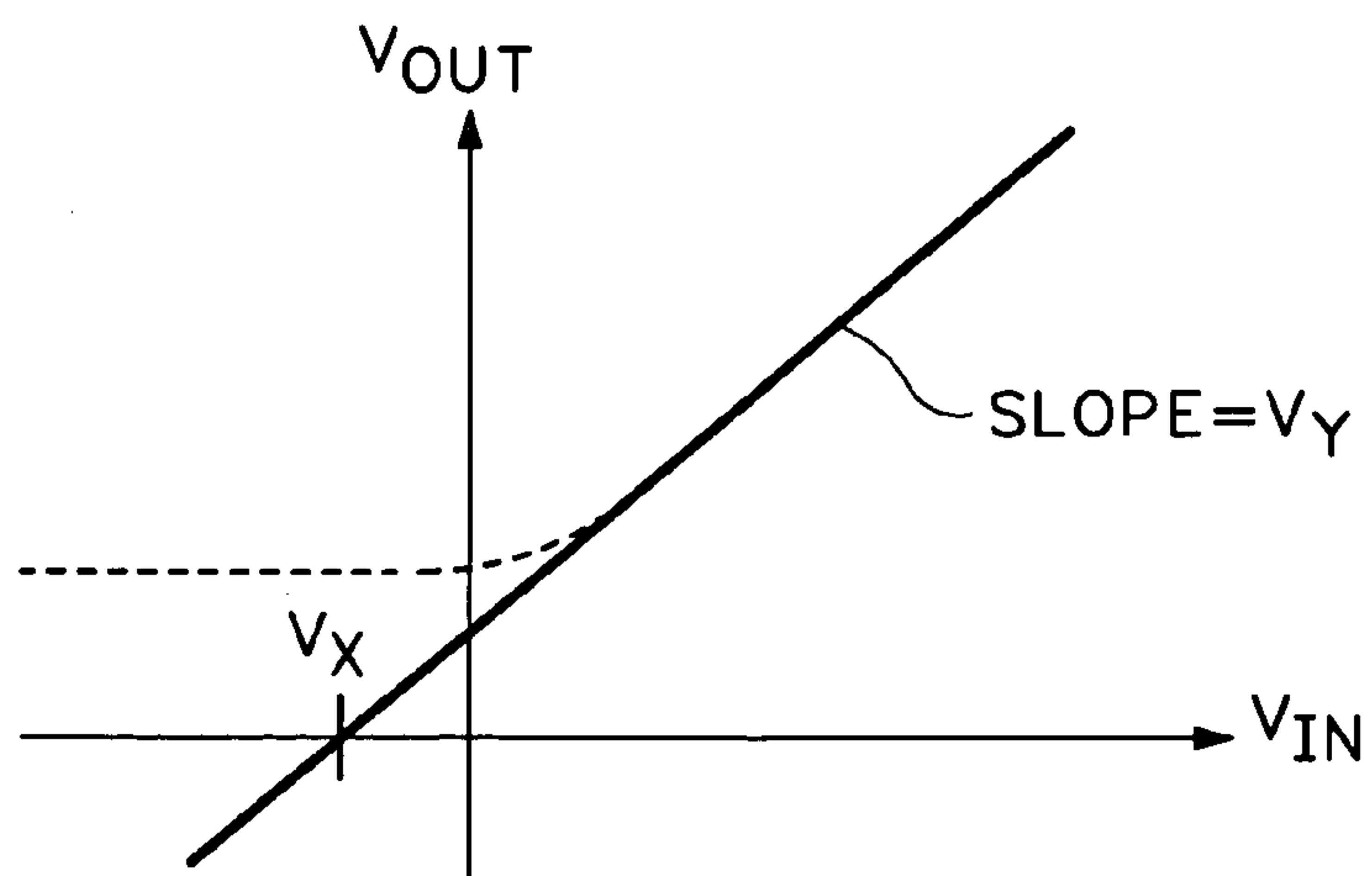
FIG.3 (PRIOR ART)
