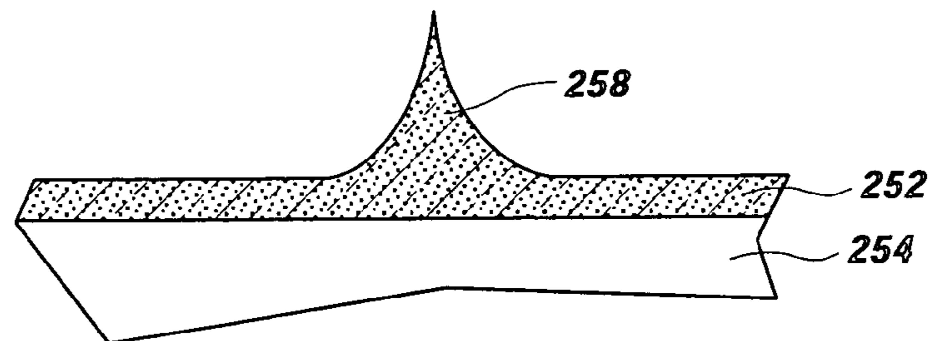
Fig. 21 (PRIOR ART)
