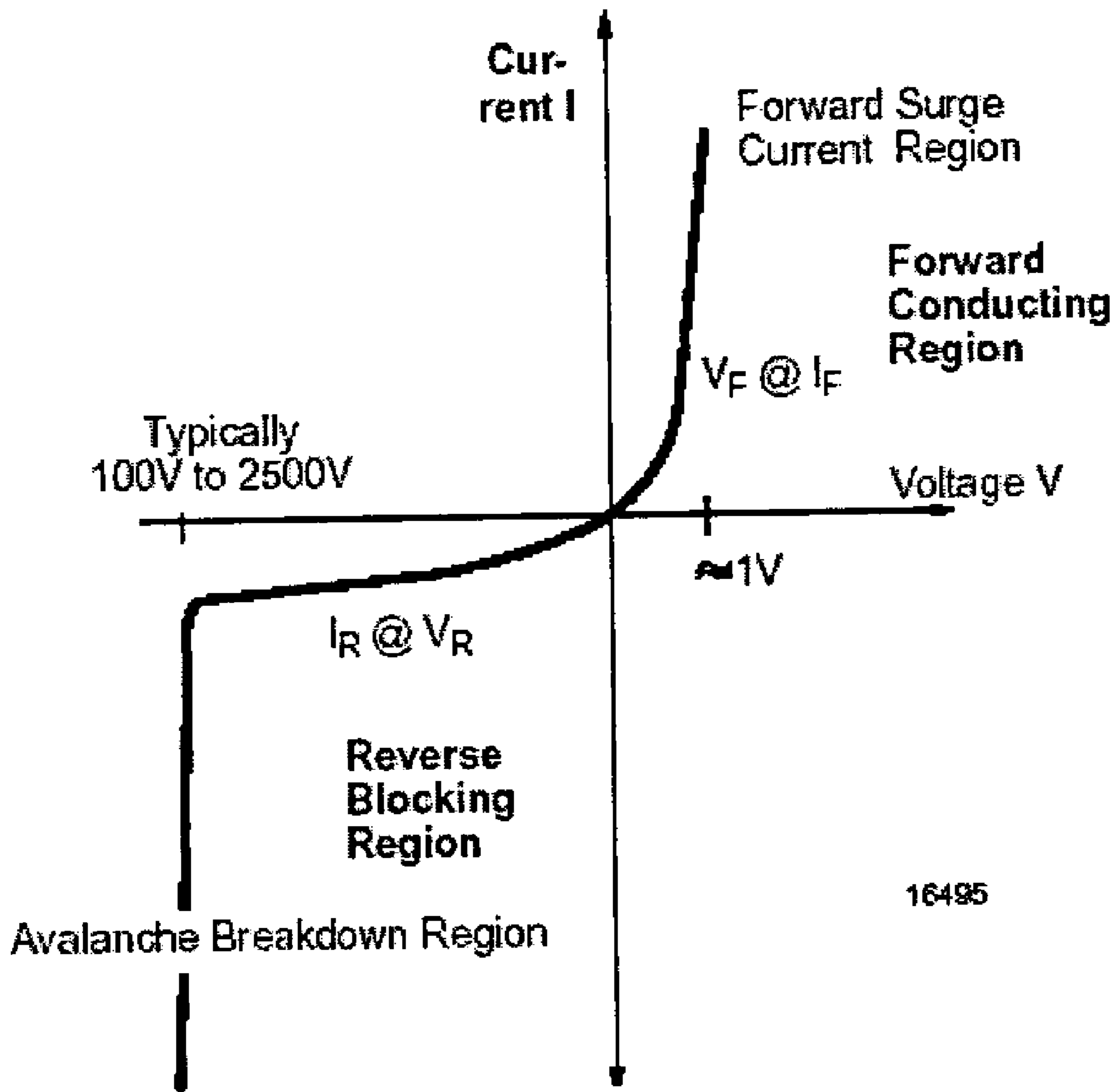
Figure 2: Typical Diode Current vs. Voltage Characteristics
