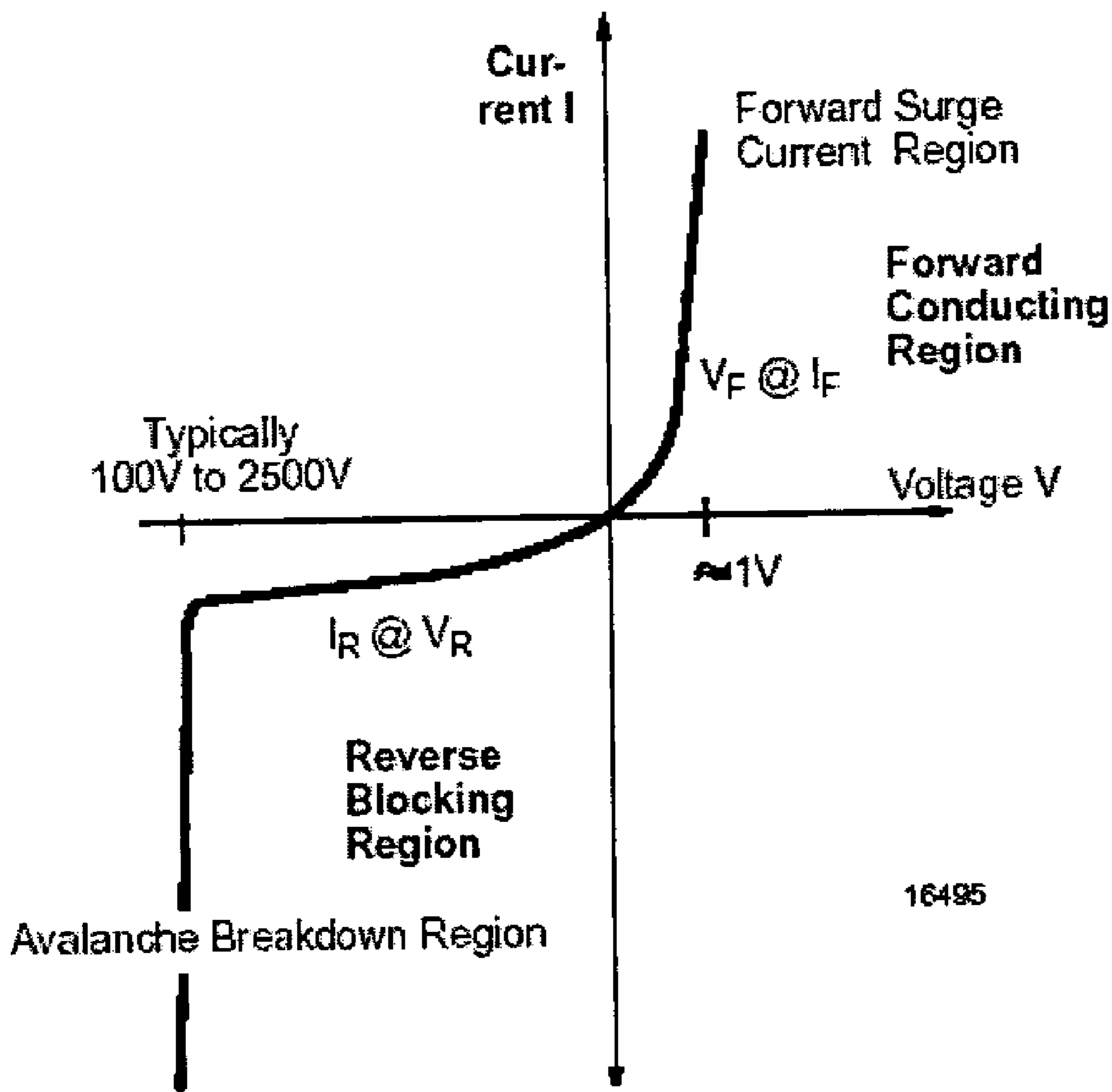
Figure 2: Typical Diode Current vs. Voltage Characteristics
