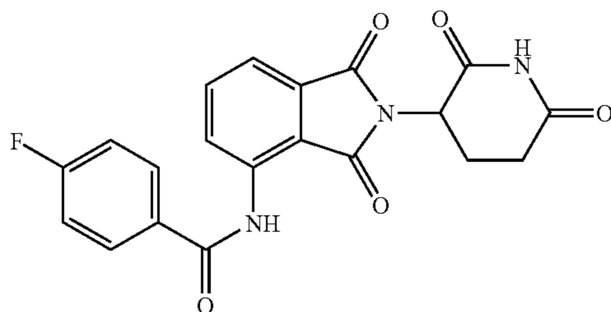
N-[2-(2,6-Dioxo-piperidin-3-yl)-1,3-dioxo-2,3-dihydro-1H-isoindol-4-yl]-4-fluoro-benzamide I-65
