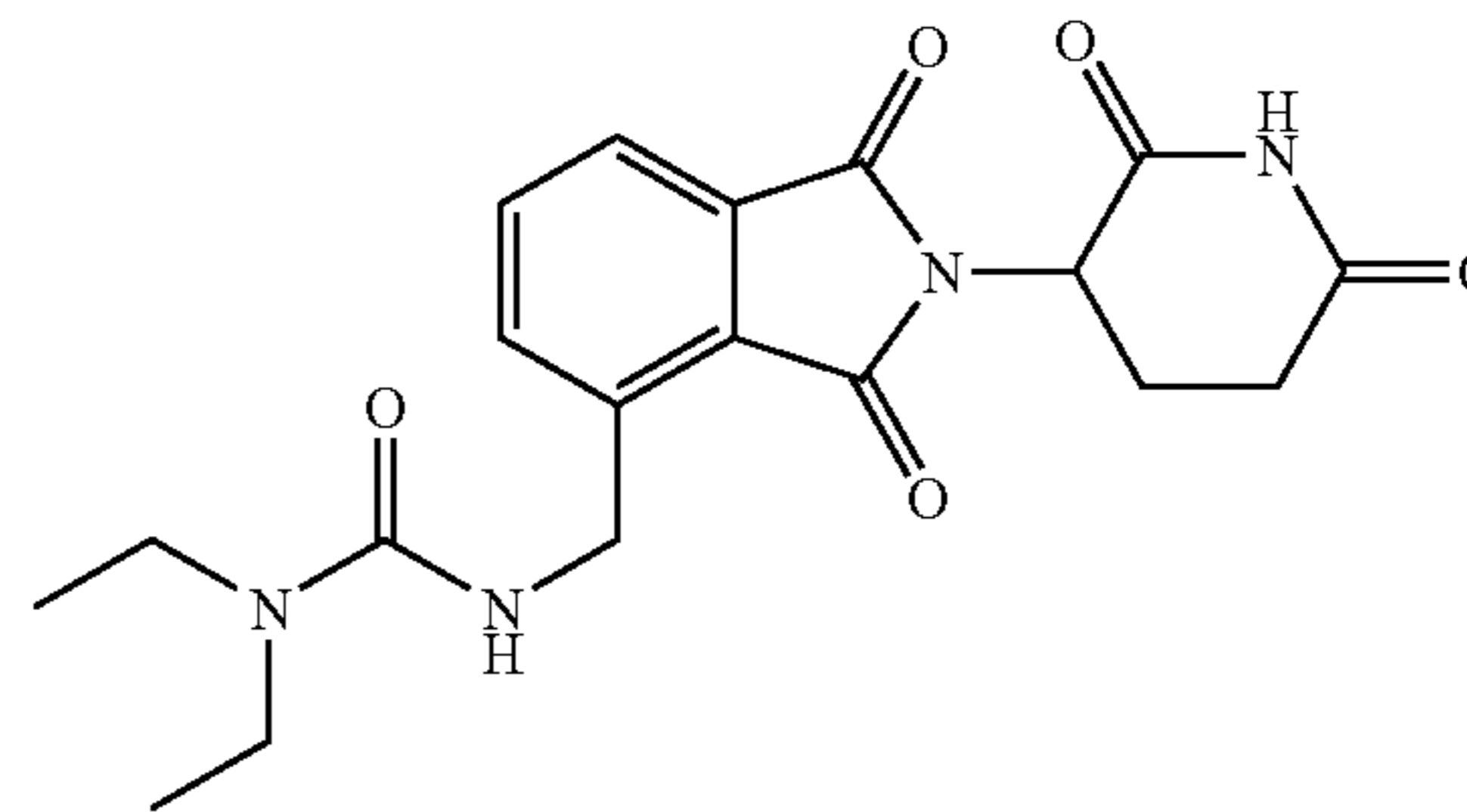
N-{[2-(2,6-Dioxo(3-piperidyl))-1,3-dioxoisindolin-4-yl]methyl}(diethylamino)carboxamide I-138
