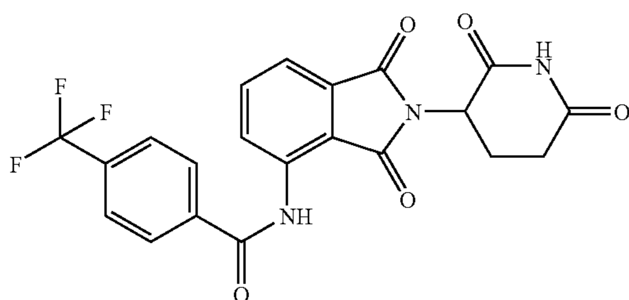
N-[2-(2,6-Dioxo-piperidin-3-yl)-1,3-dioxo-2,3-dihydro-1H-isoindol-4-yl]-4-trifluoromethyl-benzamide I-66
