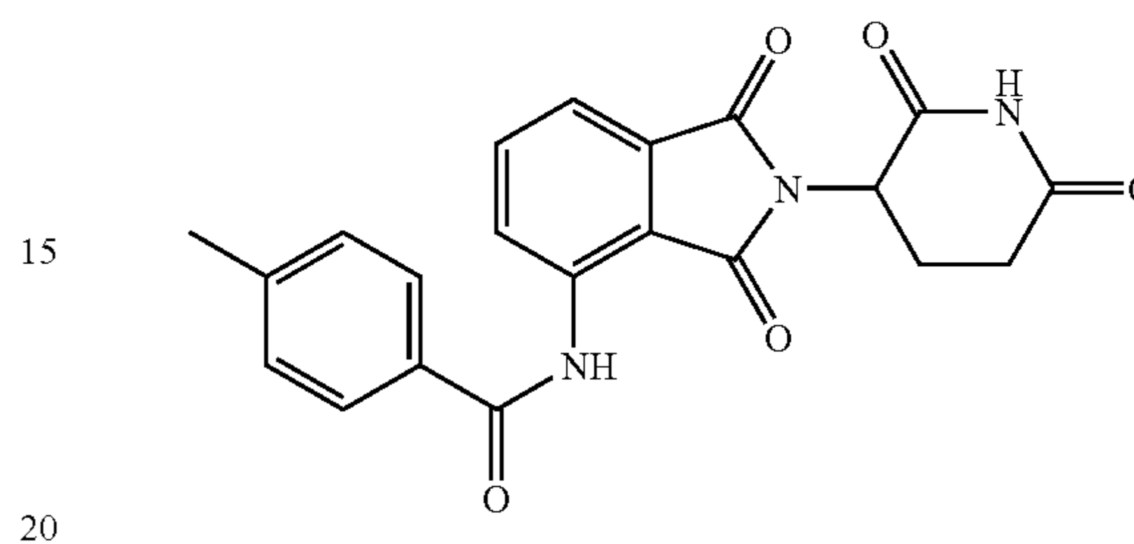
N-[2-(2,6-Dioxo-piperidin-3-yl)-1,3-dioxo-2,3-dihydro-1H-isoindol-4-yl]-4-methyl-benzamide I-67
