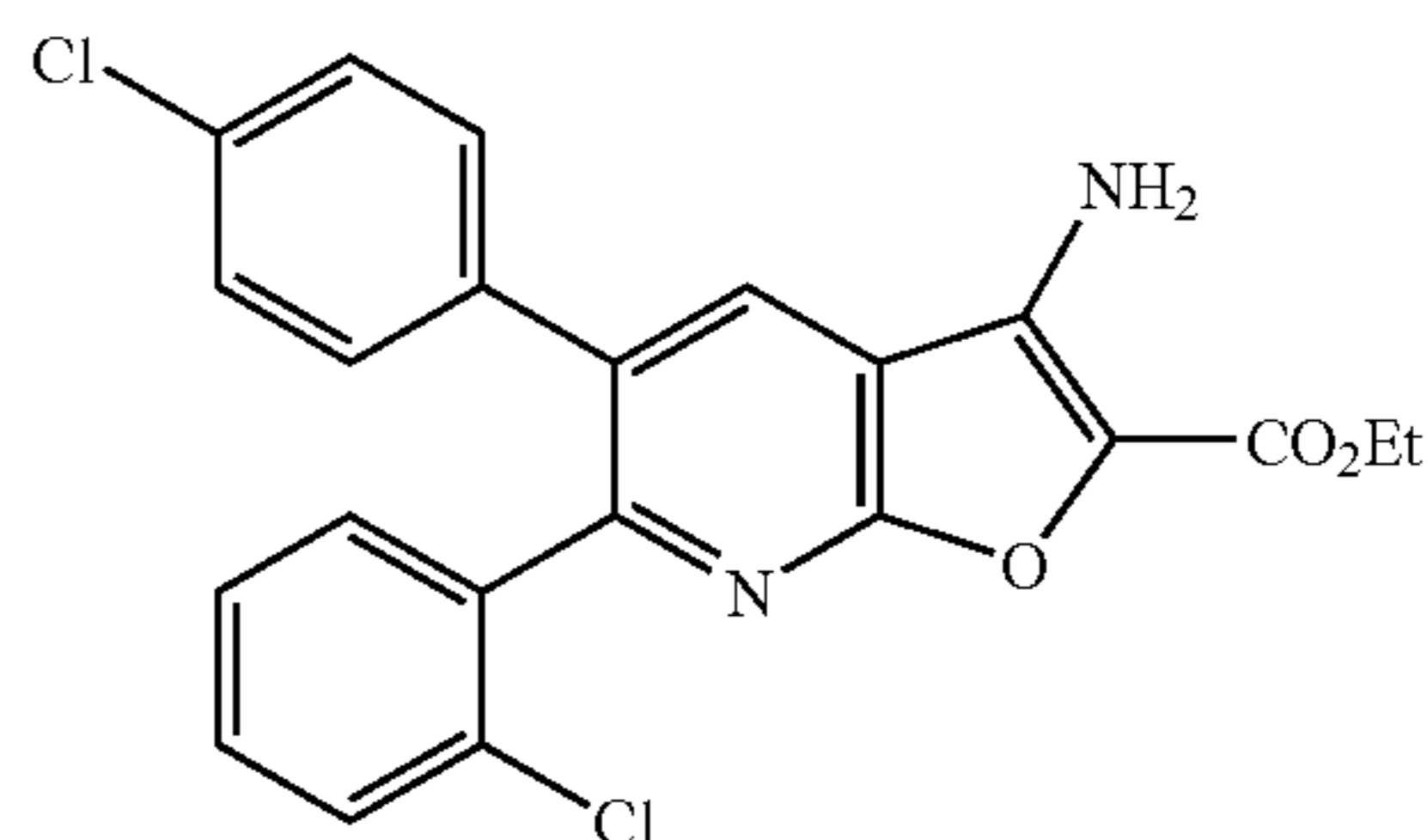
Ethyl 3-amino-6-(2-chlorophenyl)-5-(4-chlorophenyl)furo[2,3-b]pyridine-2-carboxylate
