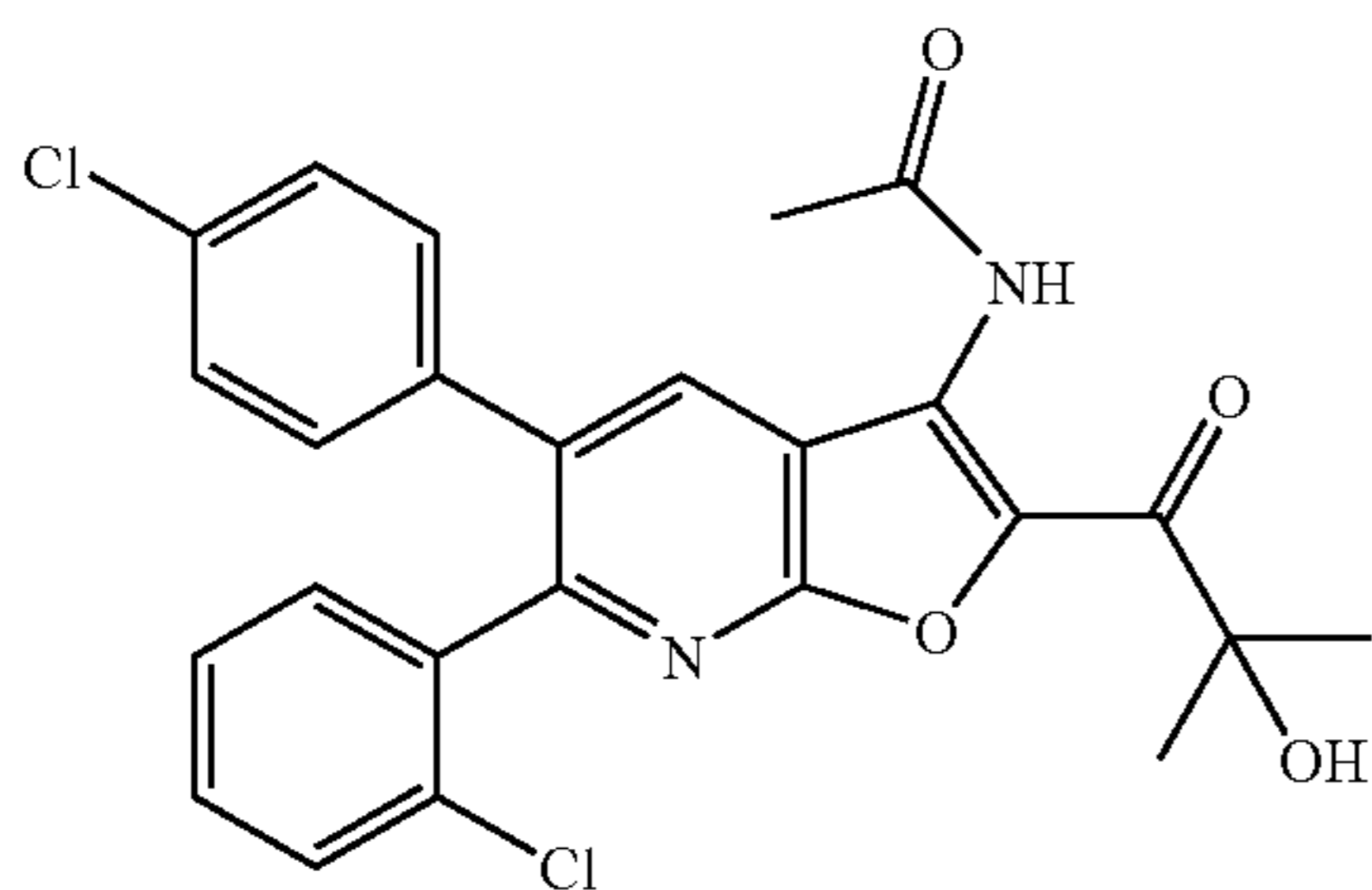
N-[6-(2-chlorophenyl)-5-(4-chlorophenyl)-2-(2-hydroxy-2-methylpropanoyl)furo[2,3-b]pyridin-3-yl]acetamide
