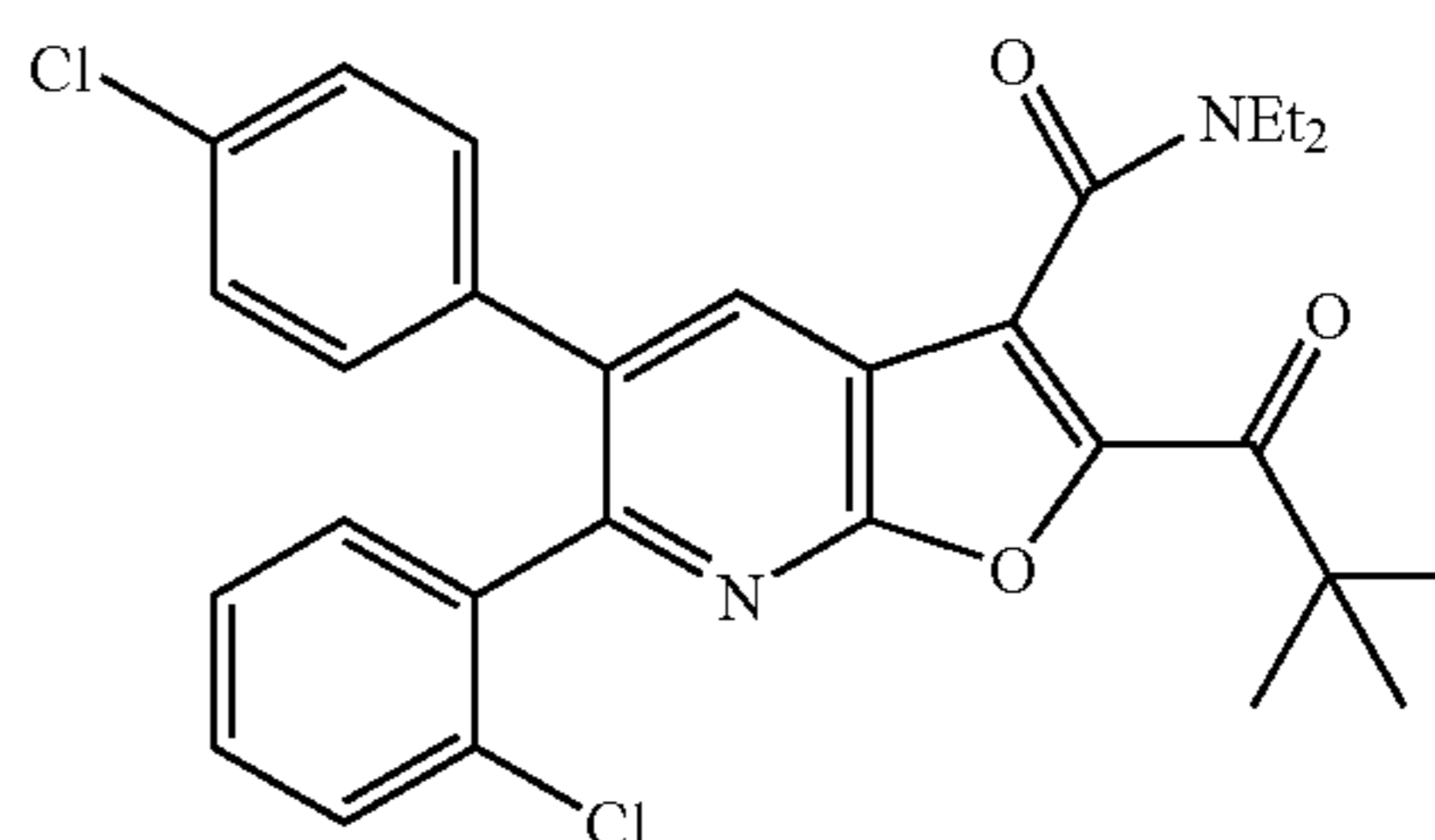
6-(2-Chlorophenyl)-5-(4-chlorophenyl)-2-(2,2-dimethylpropanoyl)-N,N-diethylfuro[2,3-b]pyridine-3-carboxamide
