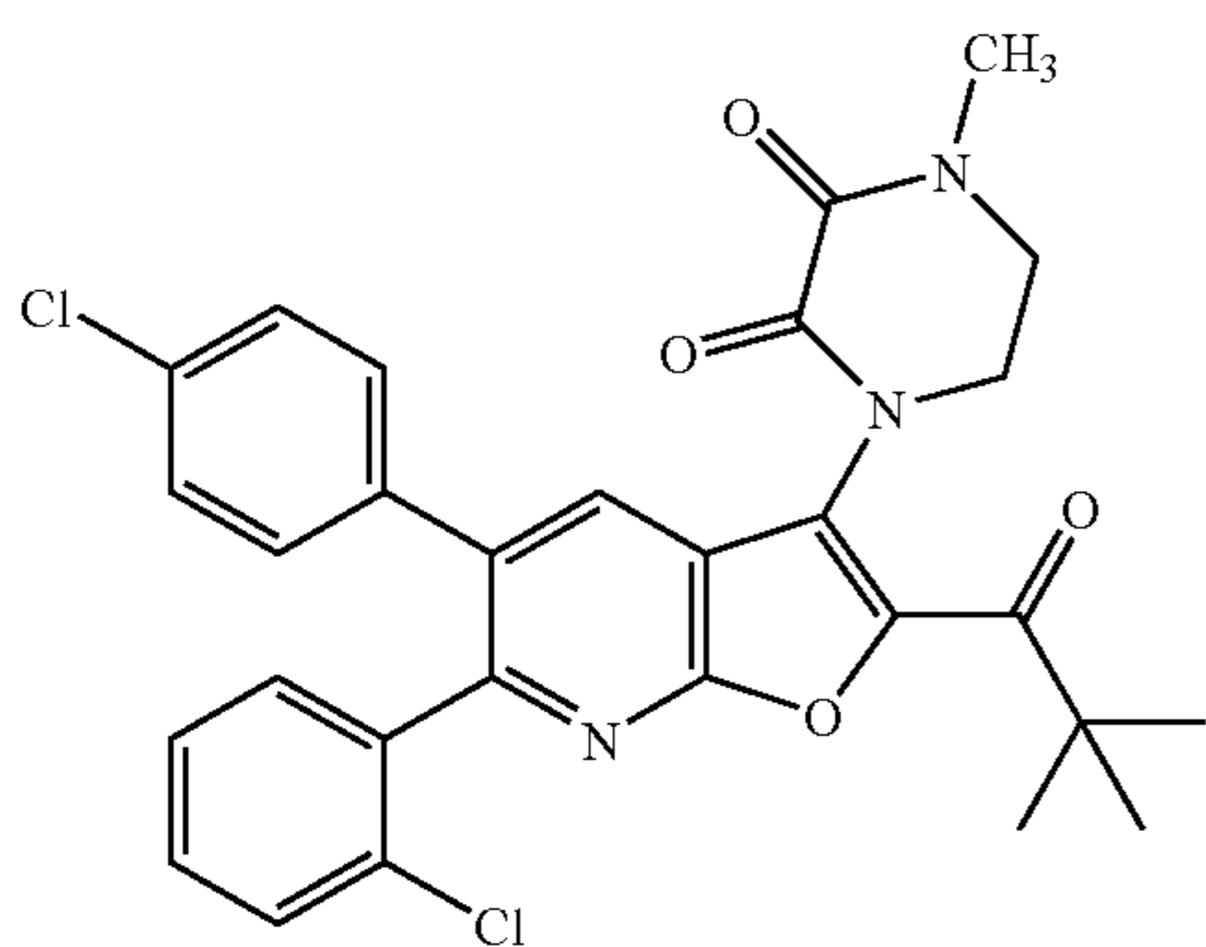
1-[6-(2-Chlorophenyl)-5-(4-chlorophenyl)-2-(2,2-dimethylpropanoyl)furo[2,3-b]pyridin-3-yl]-4-methylpiperazine-2,3-dione
