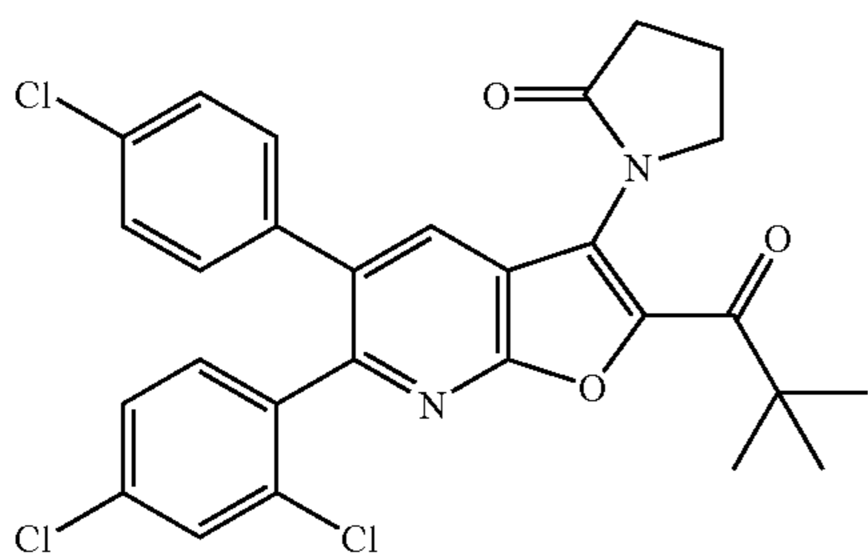
1-[5-(4-Chlorophenyl)-6-(2,4-dichlorophenyl)-2-(2-dimethylpropanoyl)furo[2,3-b]pyridin-3-yl]pyrrolidin-2-one
