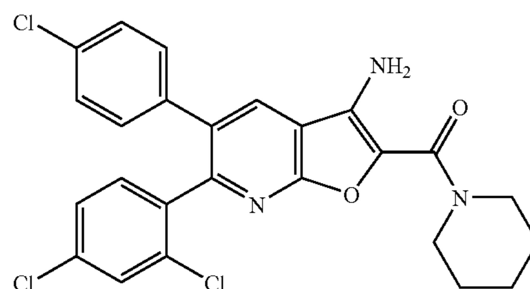
5-(4-Chlorophenyl)-6-(2,4-dichlorophenyl)-2-(piperidin-1-ylcarbonyl)furo[2,3-b]pyridin-3-amine
