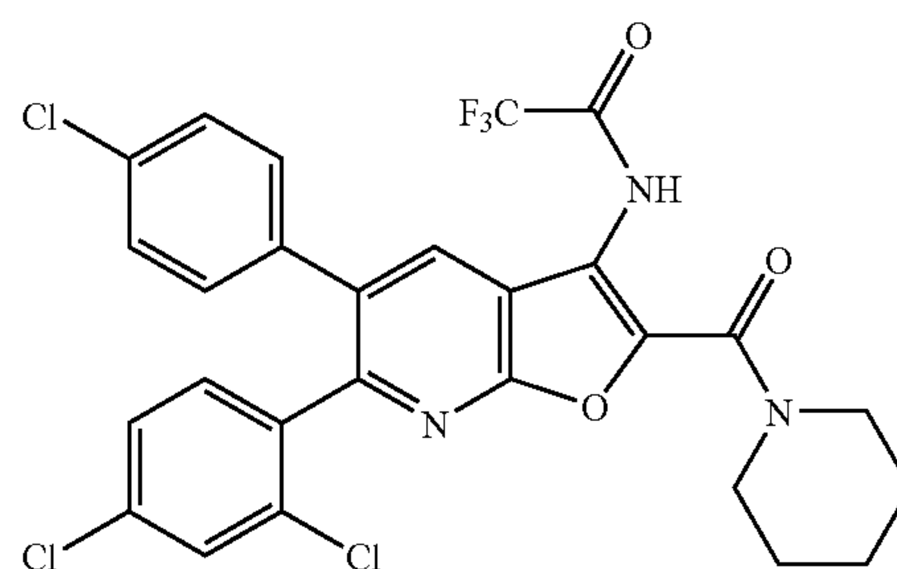
N-[5-(4-chlorophenyl)-6-(2,4-dichlorophenyl)-2-(piperidin-1-ylcarbonyl)furo[2,3-b]pyridin-3-yl]-2,2,2-trifluoroacetamide
