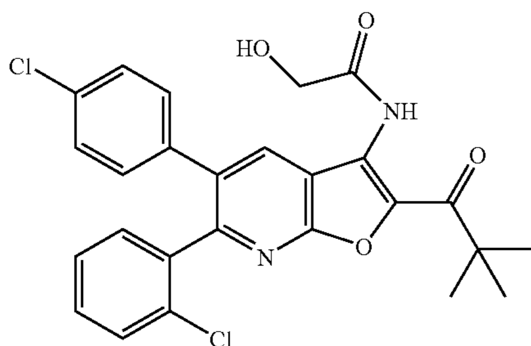
N-[6-(2-chlorophenyl)-5-(4-chlorophenyl)-2-(2,2-dimethylpropanoyl)furo[2,3-b]-pyridin-3-yl]-2-hydroxyacetamide
