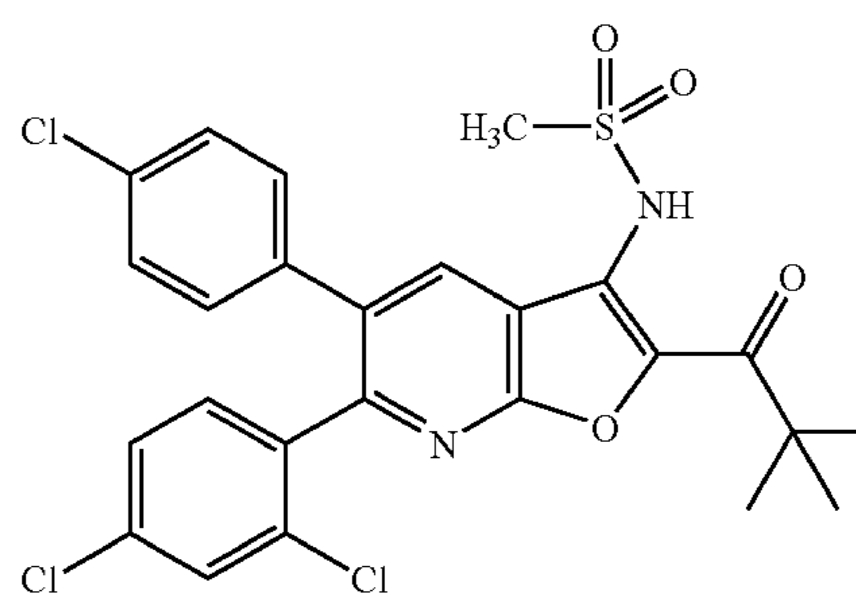
N-[5-(4-Chlorophenyl)-6-(2,4-dichlorophenyl)-2-(2,2-dimethylpropanoyl)furo[2,3-b]pyridin-3-yl]methanesulfonamide
