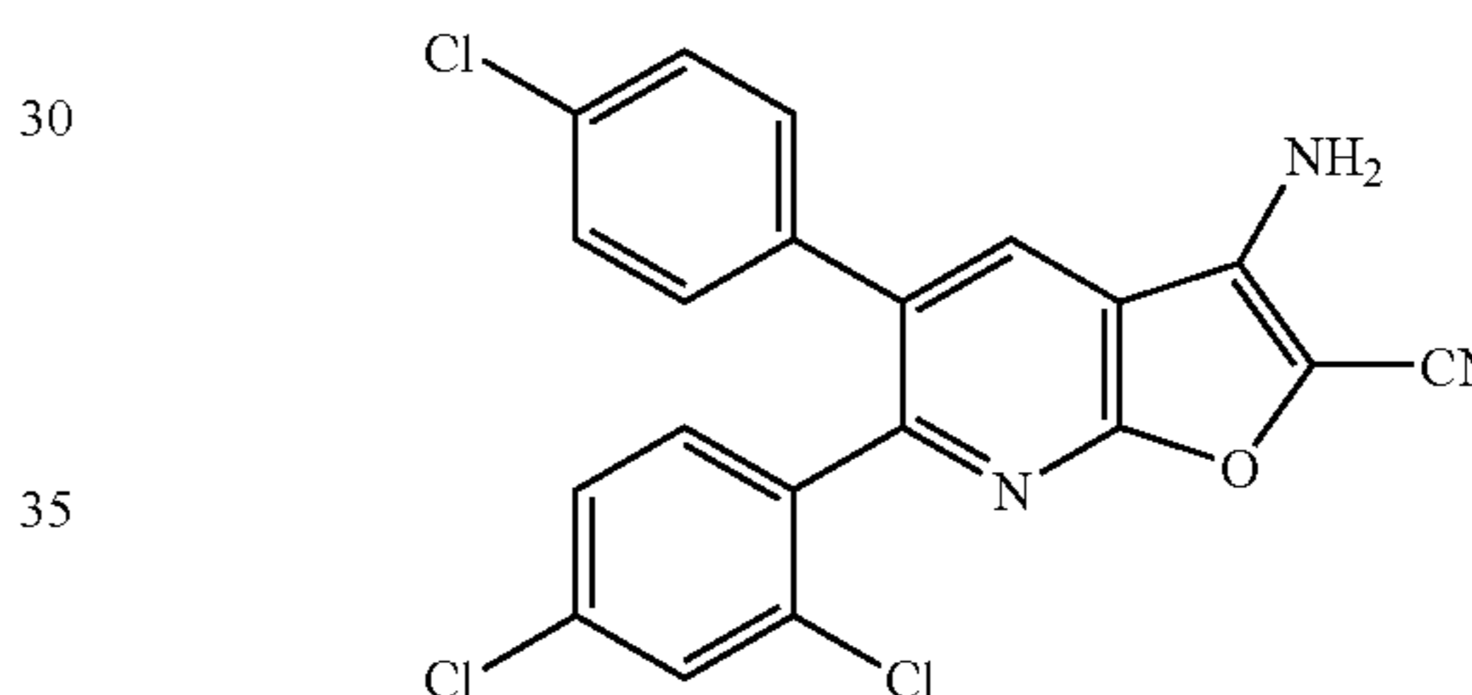
3-Amino-5-(4-chlorophenyl)-6-(2,4-dichlorophenyl)furo[2,3-b]pyridine-2-carbonitrile
