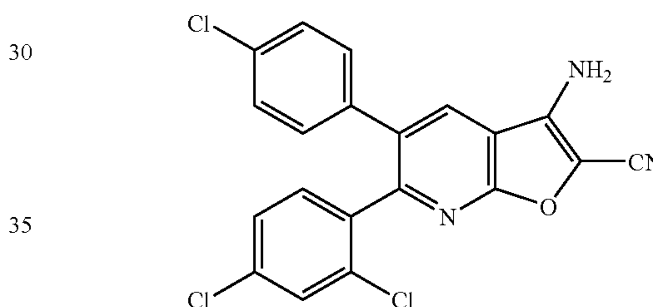
3-Amino-5-(4-chlorophenyl)-6-(2,4-dichlorophenyl)furo[2,3-b]pyridine-2-carbonitrile
