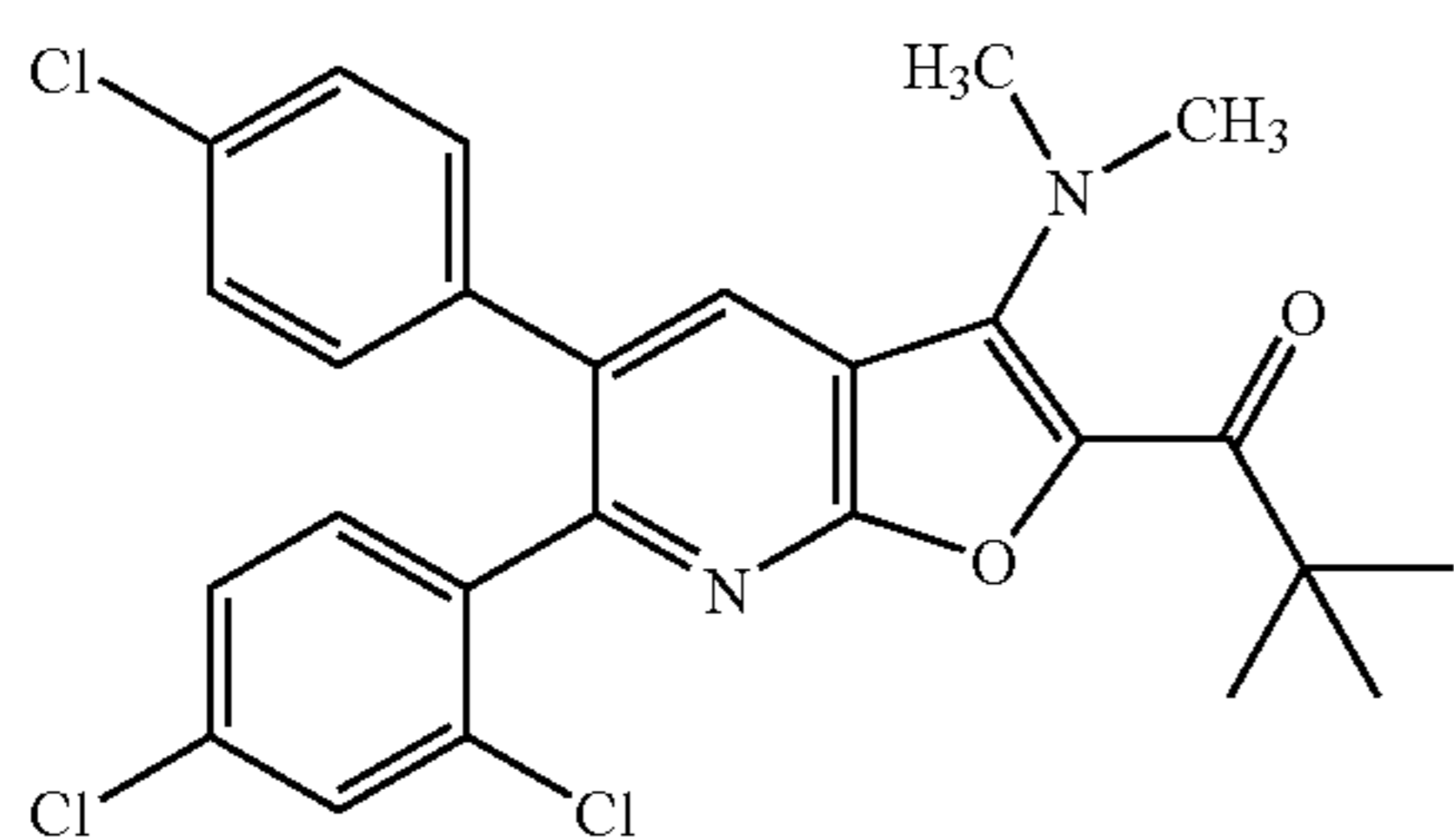
1-[5-(4-Chlorophenyl)-6-(2,4-dichlorophenyl)-3-(dimethylamino)furo[2,3-b]pyridin-2-yl]-2,2-dimethylpropan-1-one
