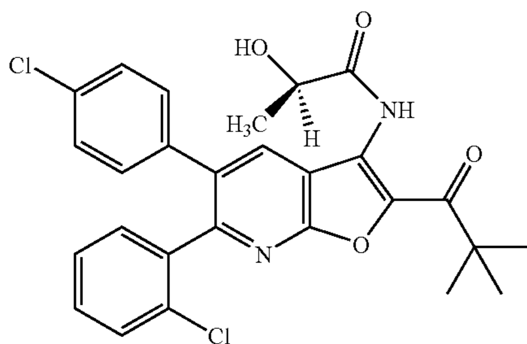
(2S)-N-[6-(2-chlorophenyl)-5-(4-chlorophenyl)-2-(2,2-dimethylpropanoyl)furo[2,3-b]pyridin-3-yl]-2-hydroxypropanamide
