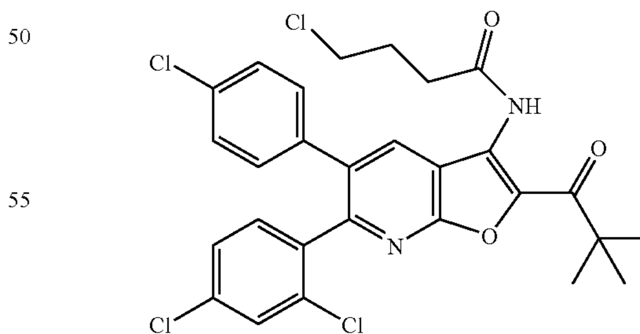
4-Chloro-N-[5-(4-chlorophenyl)-6-(2,4-dichlorophenyl)-2-(2,2-dimethylpropanoyl)furo[2,3-b]pyridin-3-yl]butanamide
