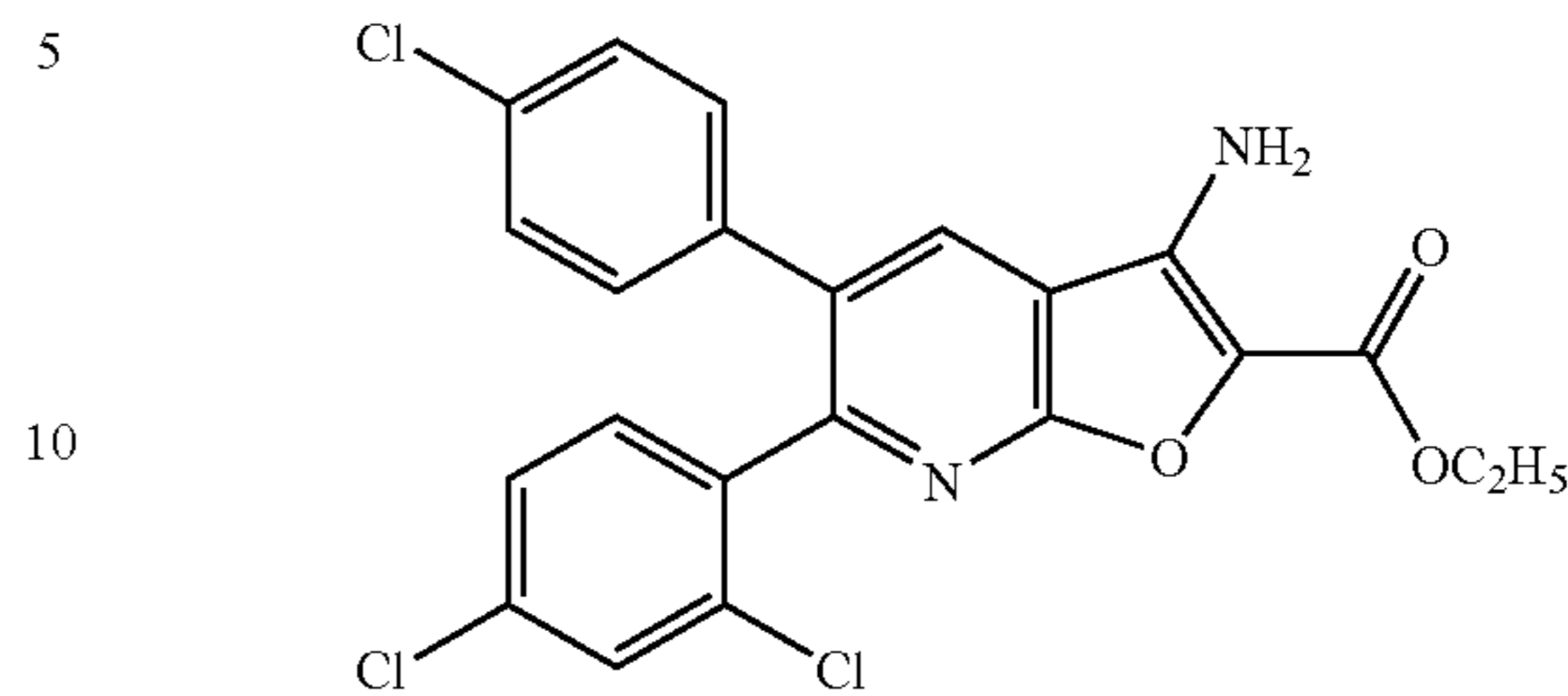
Ethyl 3-amino-5-(4-chlorophenyl)-6-(2,4-dichlorophenyl)furo[2,3-b]pyridine-2-carboxylate
