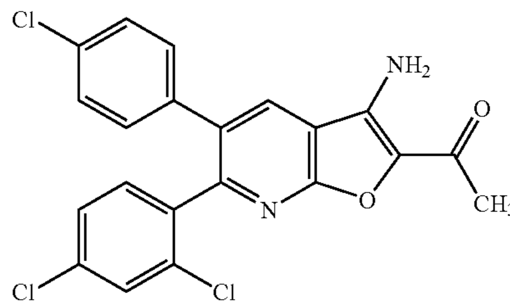
1-[3-Amino-5-(4-chlorophenyl)-6-(2,4-dichlorophenyl)furo[2,3-b]pyridin-2-yl]ethanone
