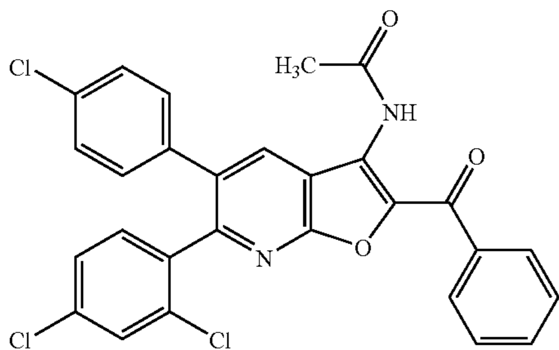
N-[2-Benzol-5-(4-chlorophenyl)-6-(2,4-dichlorophenyl)furo[2,3-b]pyridin-3-yl]acetamide
