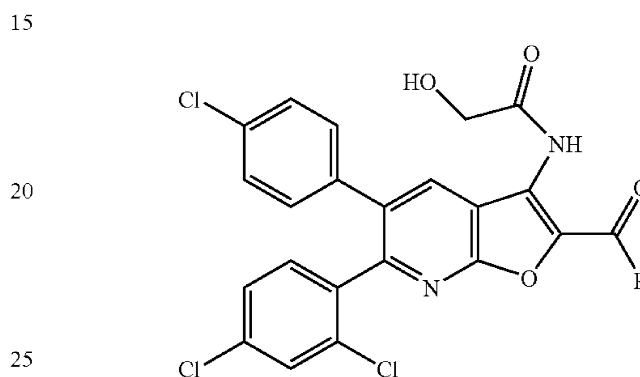
1-[3-Amino-5-(4-chlorophenyl)-6-(2,4-dichlorophenyl)furo[2,3-b]pyridin-2-yl]-2-methylpropan-1-one
