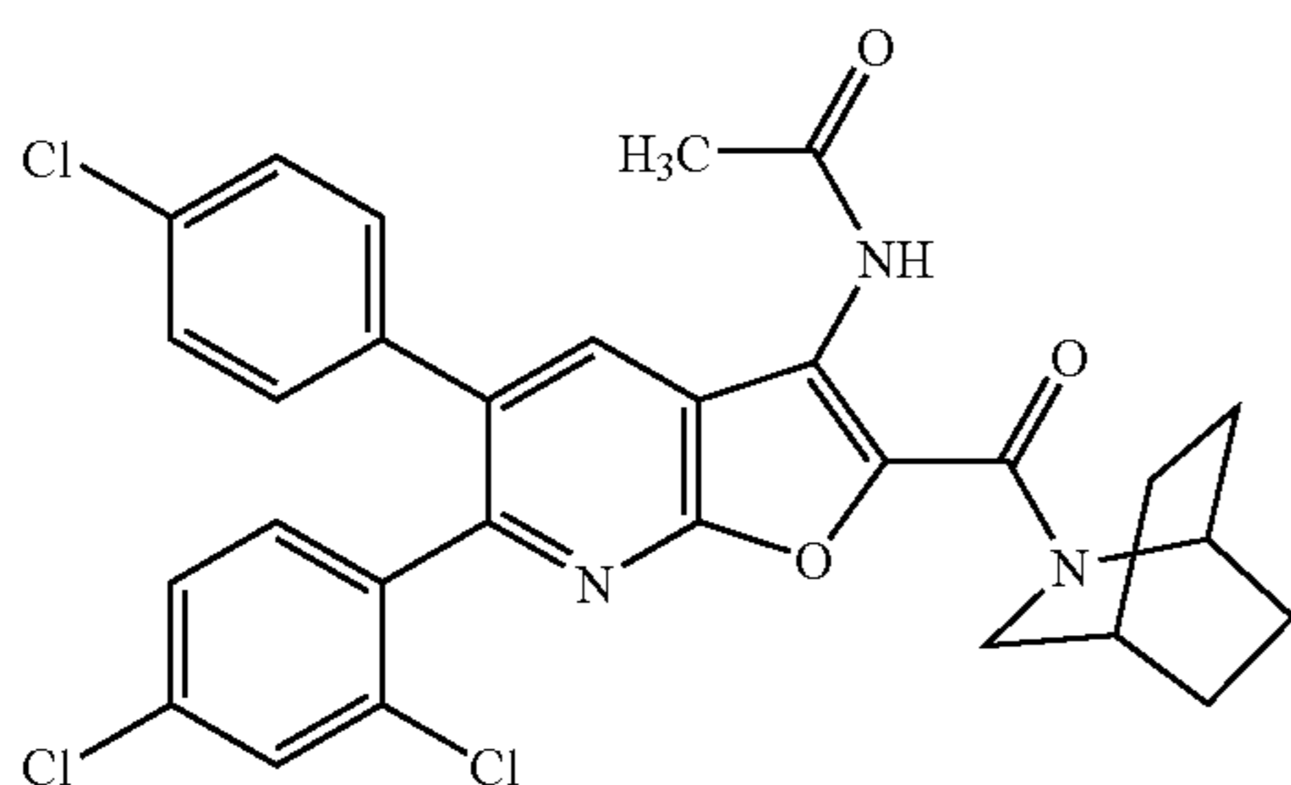
N-[2-(2-Azabicyclo[2.2.2]oct-2-ylcarbonyl)-5-(4-chlorophenyl)-6-(2,4-dichlorophenyl)furo[2,3-b]pyridin-3-yl]acetamide
