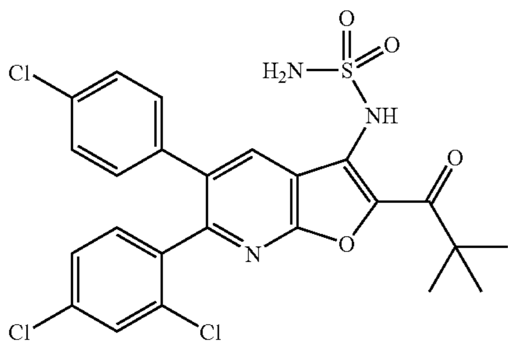
N-[5-(4-Chlorophenyl)-6-(2,4-dichlorophenyl)-2-(2,2-dimethylpropanoyl)furo[2,3-b]pyridin-3-yl]methanesulfonamide
