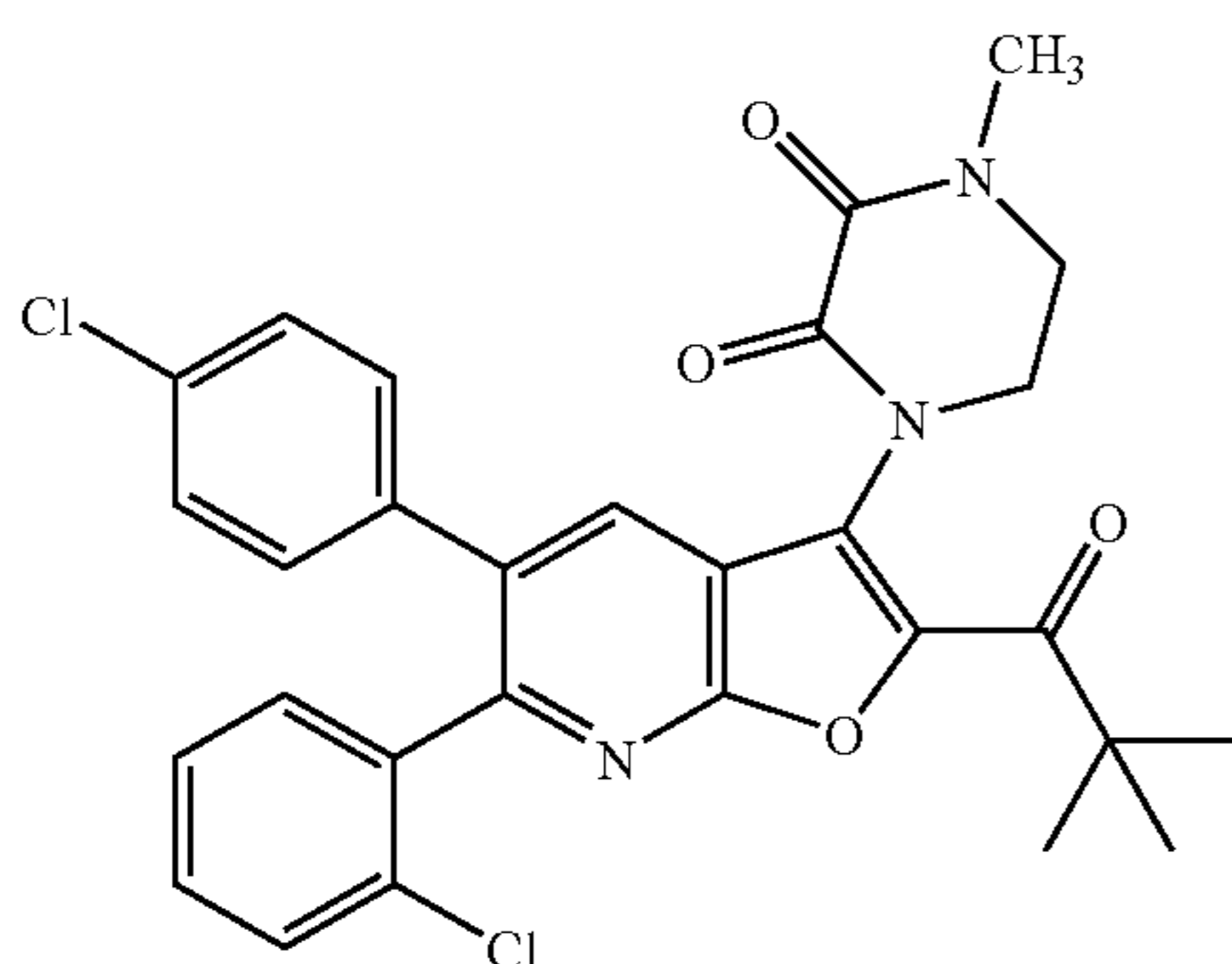
1-[6-(2-Chlorophenyl)-5-(4-chlorophenyl)-2-(2,2-dimethylpropanoyl)furo[2,3-b]pyridin-3-yl]-4-methylpiperazine-2,3-dione
