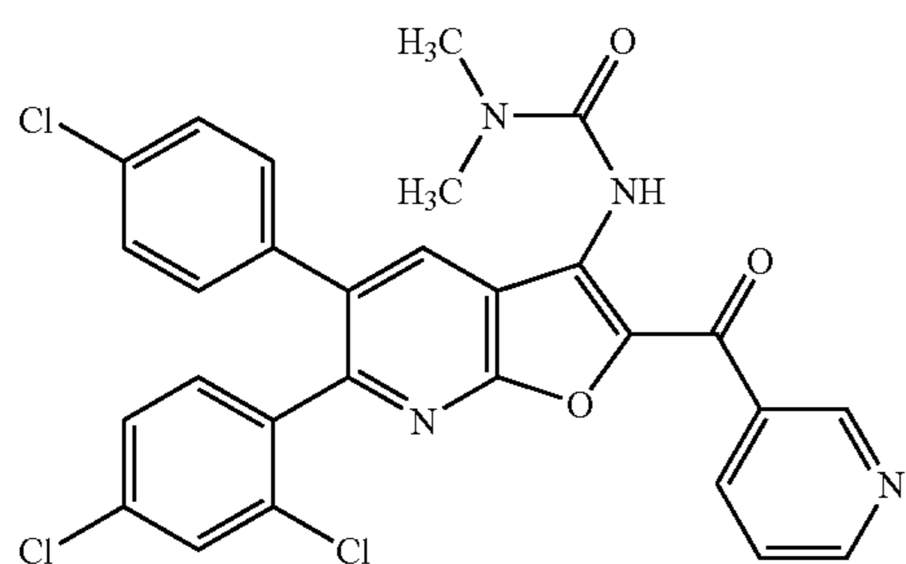
N'-[5-(4-Chlorophenyl)-6-(2,4-dichlorophenyl)-2-(pyridin-3-ylcarbonyl)furo[2,3-b]pyridin-3-yl]-N,N-dimethylurea
