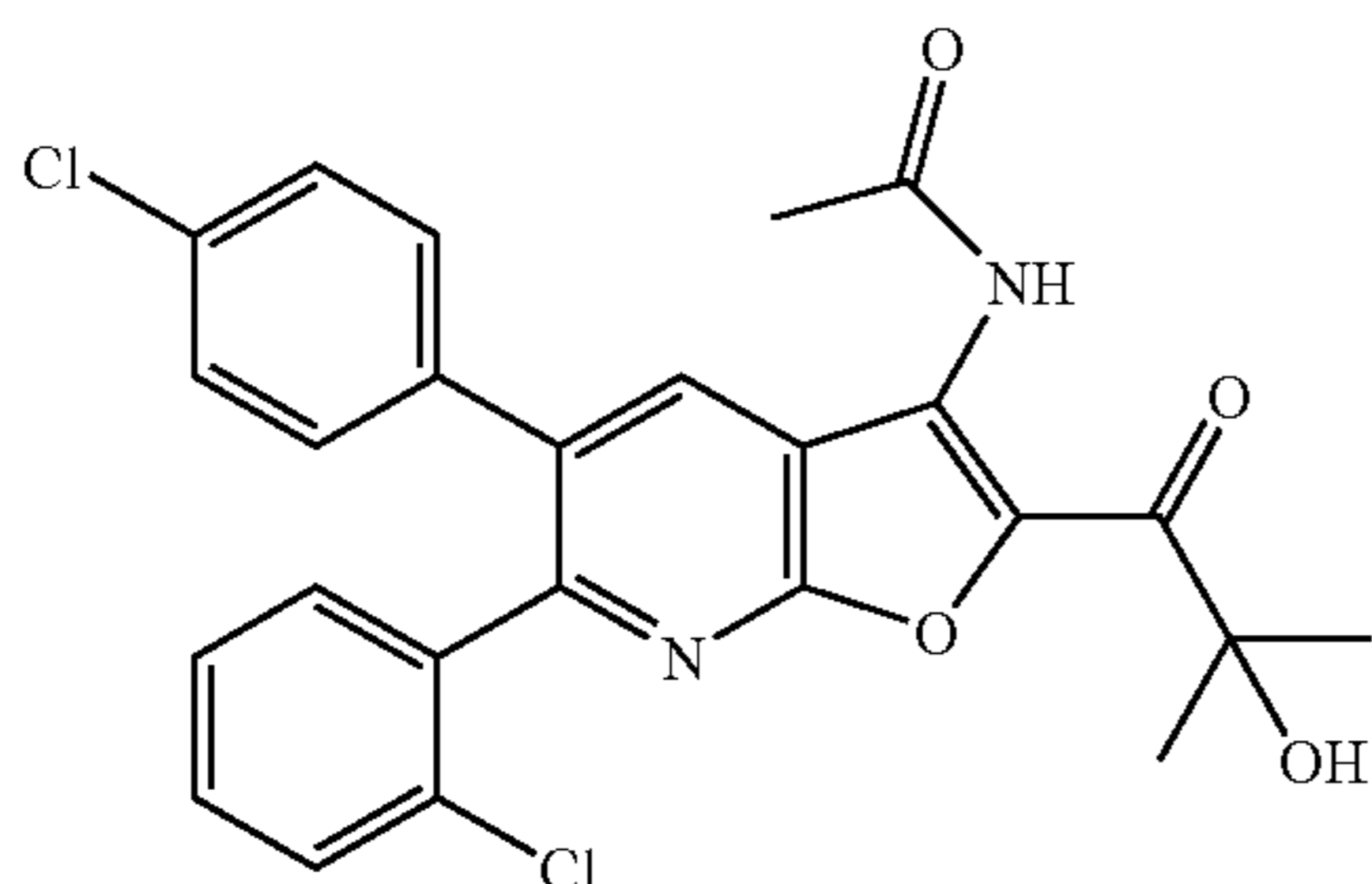
N-[6-(2-chlorophenyl)-5-(4-chlorophenyl)-2-(2-hydroxy-2-methylpropanoyl)furo[2,3-b]pyridin-3-yl]acetamide
