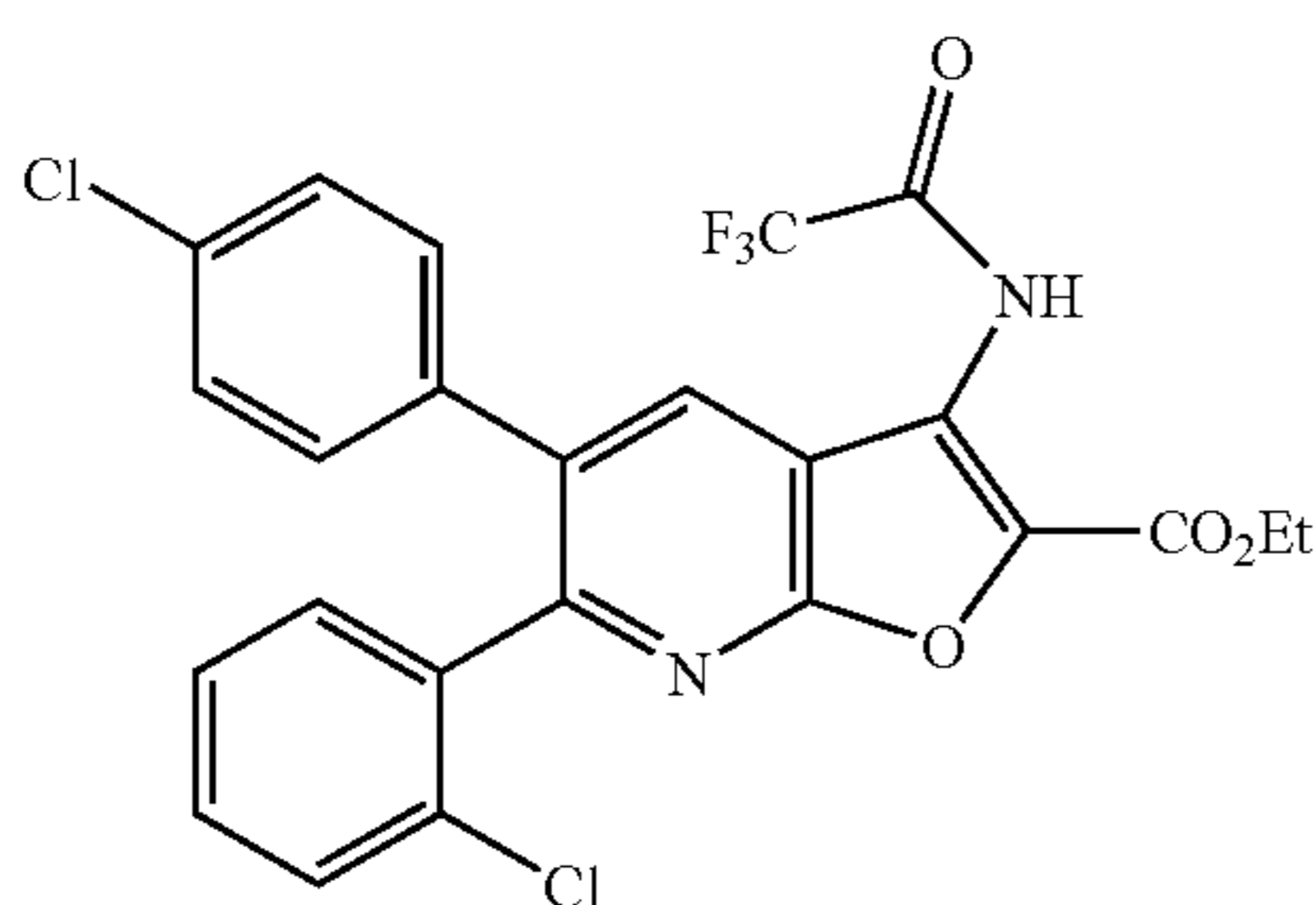
Ethyl 6-(2-chlorophenyl)-5-(4-chlorophenyl)-3-[(trifluoroacetyl)amino]furo[2,3-b]pyridine-2-carboxylate
