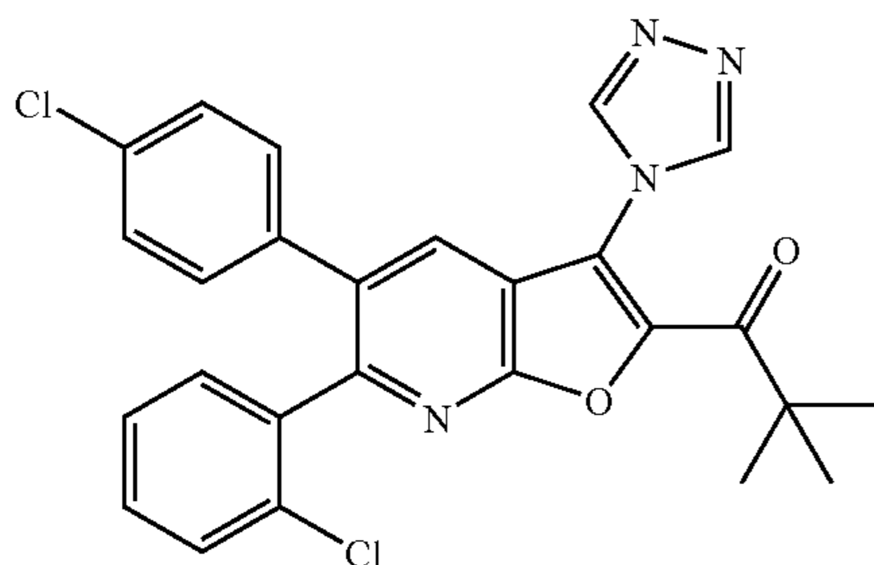
1-[6-(2-Chlorophenyl)-5-(4-chlorophenyl)-3-(4H-1,2,4-triazol-4-yl)furo[2,3-b]pyridin-2-yl]-2,2-dimethylpropan-1-one
