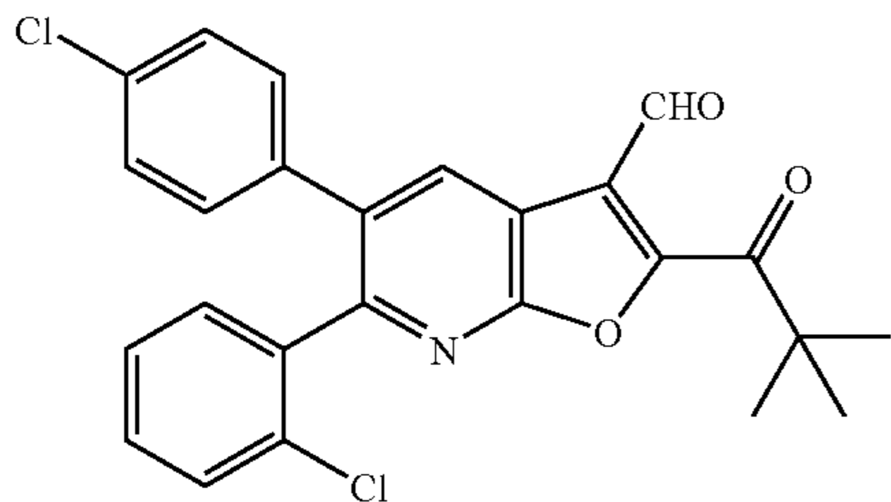
6-(2-Chlorophenyl)-5-(4-chlorophenyl)-2-(2,2-dimethylpropanoyl)furo[2,3-b]pyridine-3-carbaldehyde
