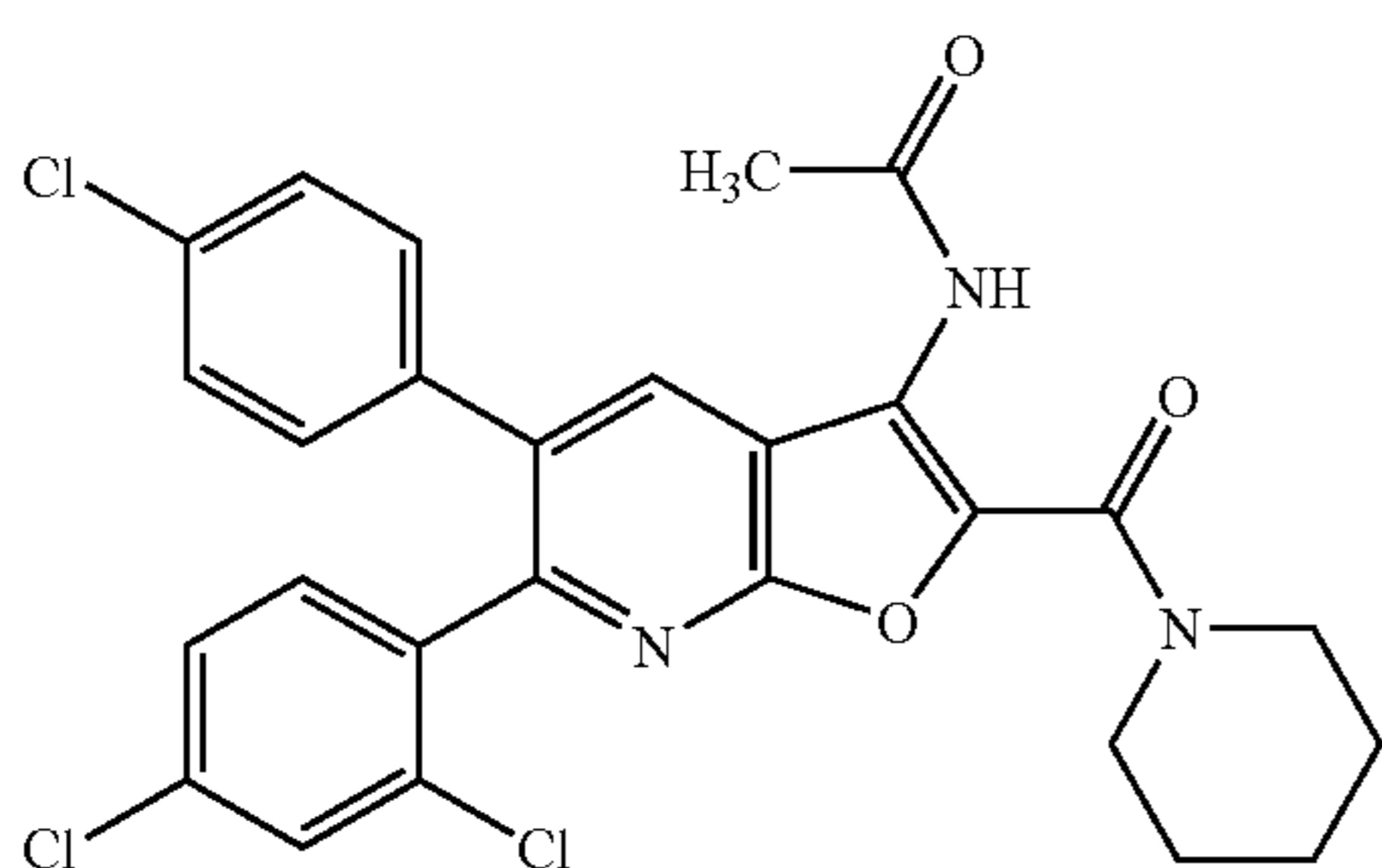
N-[5-(4-Chlorophenyl)-6-(2,4-dichlorophenyl)-2-(piperidin-1-ylcarbonyl)furo[2,3-b]pyridin-3-yl]acetamide
