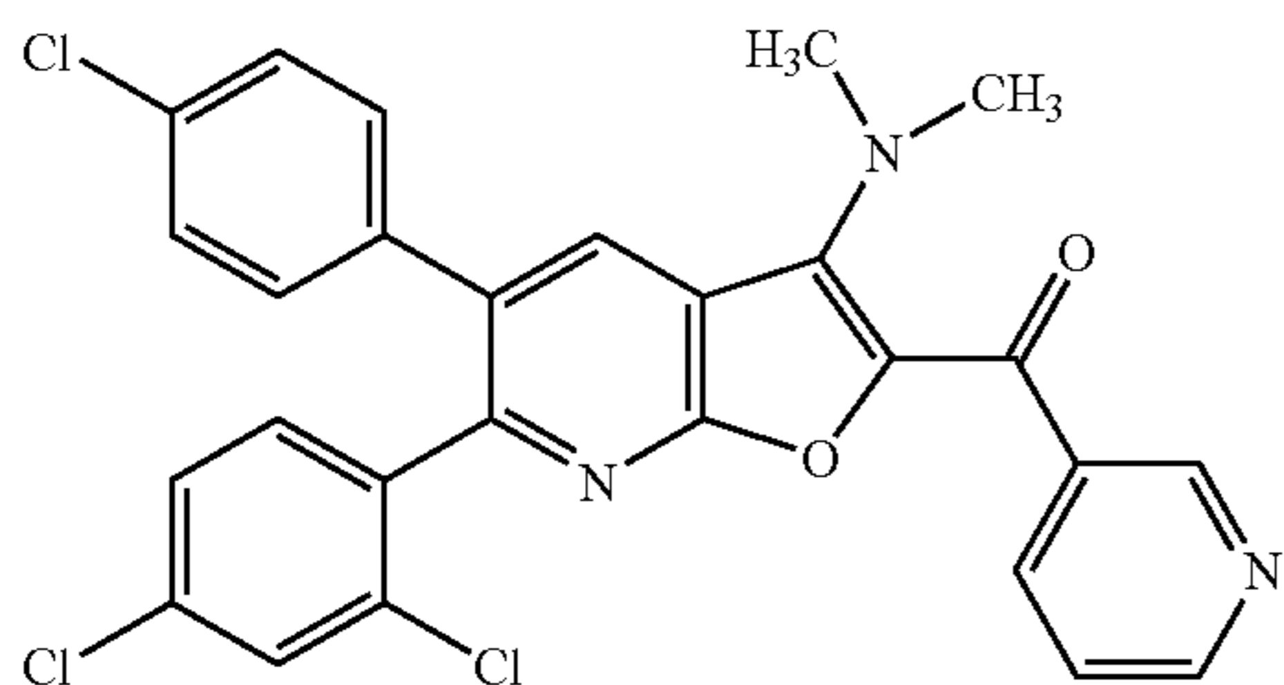
[5-(4-Chlorophenyl)-6-(2,4-dichlorophenyl)-3-(diethylamino)furo[2,3-b]pyridin-2-yl](pyridin-3-yl)methanone
