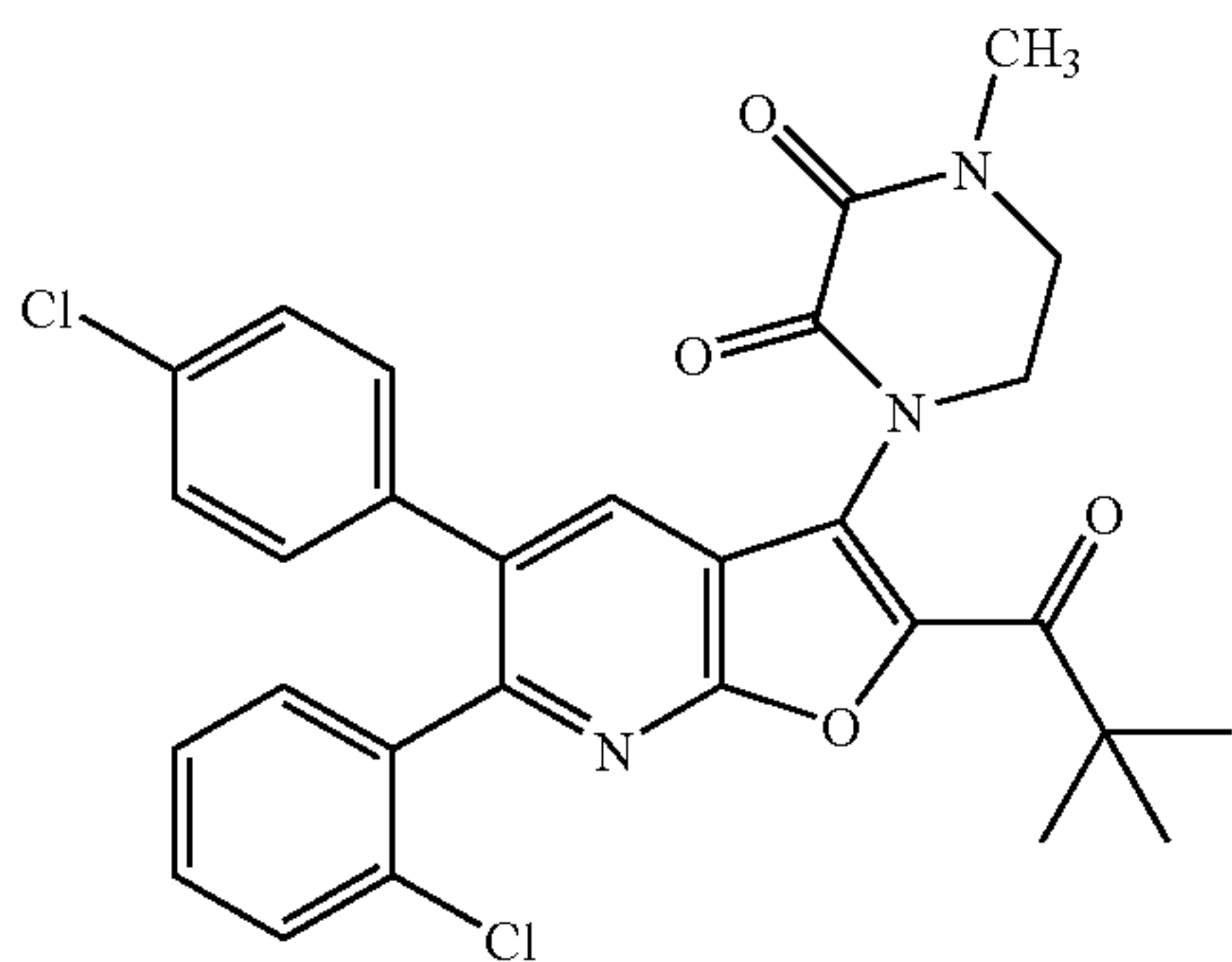
1-[6-(2-Chlorophenyl)-5-(4-chlorophenyl)-2-(2,2-dimethylpropanoyl)furo[2,3-b]pyridin-3-yl]-4-methylpiperazine-2,3-dione
