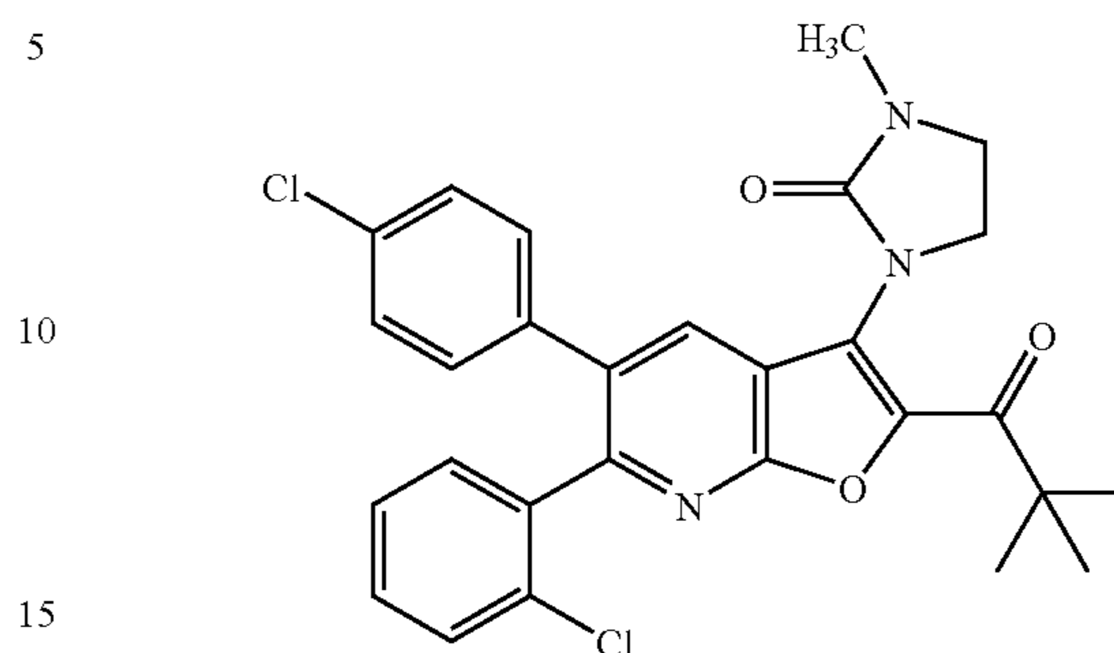
1-[6-(2-Chlorophenyl)-5-(4-chlorophenyl)-2-(2,2-dimethylpropanoyl)furo[2,3-b]pyridin-3-yl]-3-methylimidazolidin-2-one
