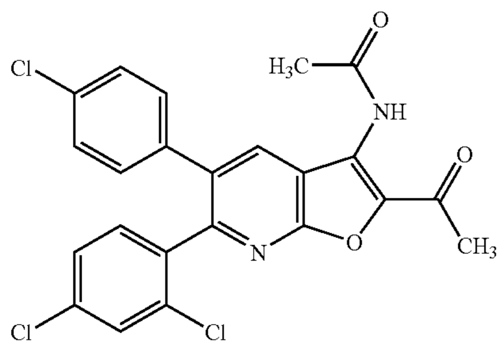
N-[2-Acetyl-5-(4-chlorophenyl)-6-(2,4-dichlorophenyl)furo[2,3-b]pyridin-3-yl]acetamide
