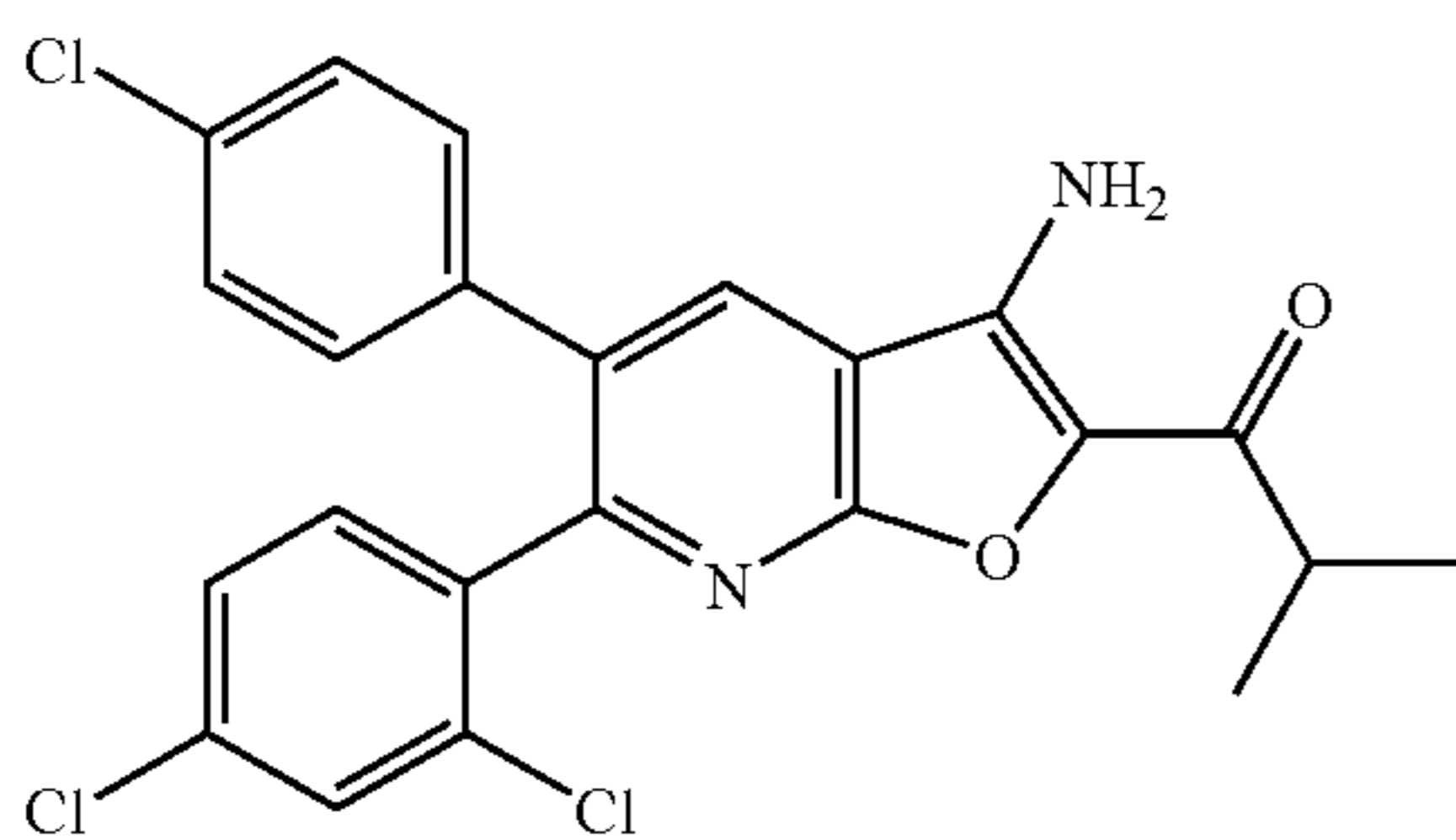
1-[3-Amino-5-(4-chlorophenyl)-6-(2,4-dichlorophenyl)furo[2,3-b]pyridin-2-yl]-2-methylpropan-1-one
