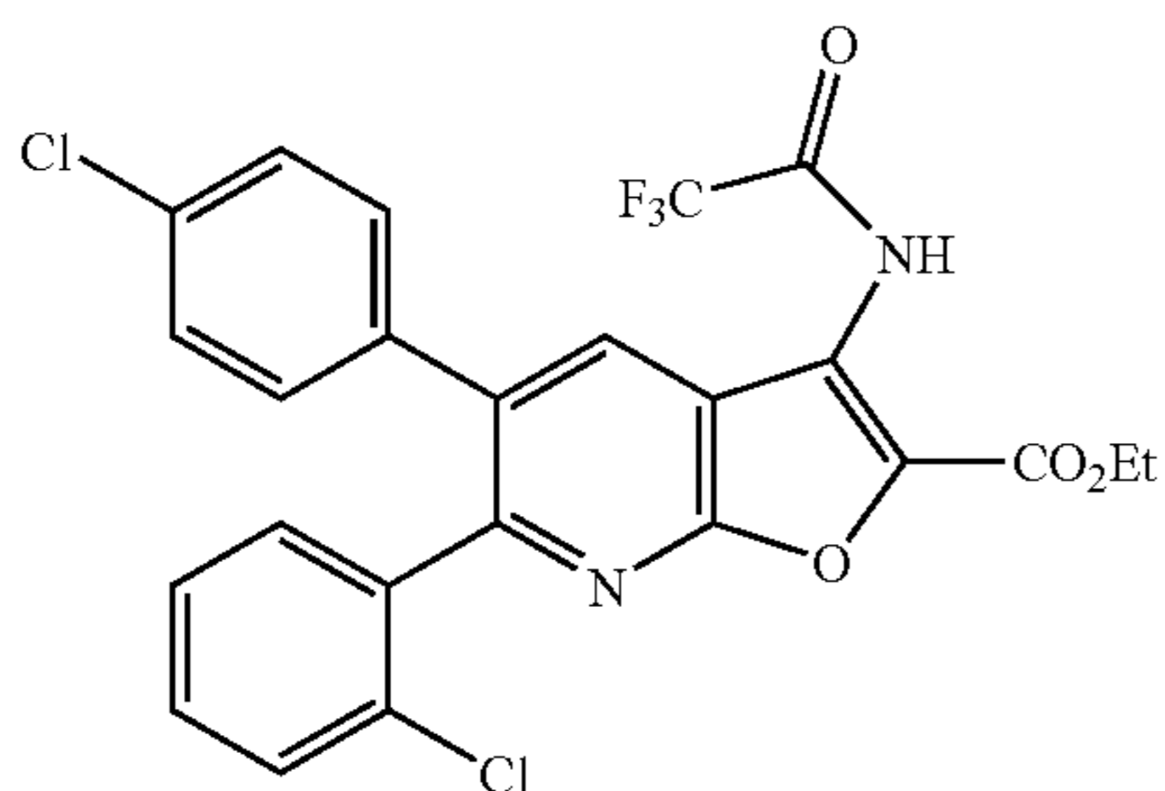
Ethyl 6-(2-chlorophenyl)-5-(4-chlorophenyl)-3-[(trifluoroacetyl)amino]furo[2,3-b]pyridine-2-carboxylate
