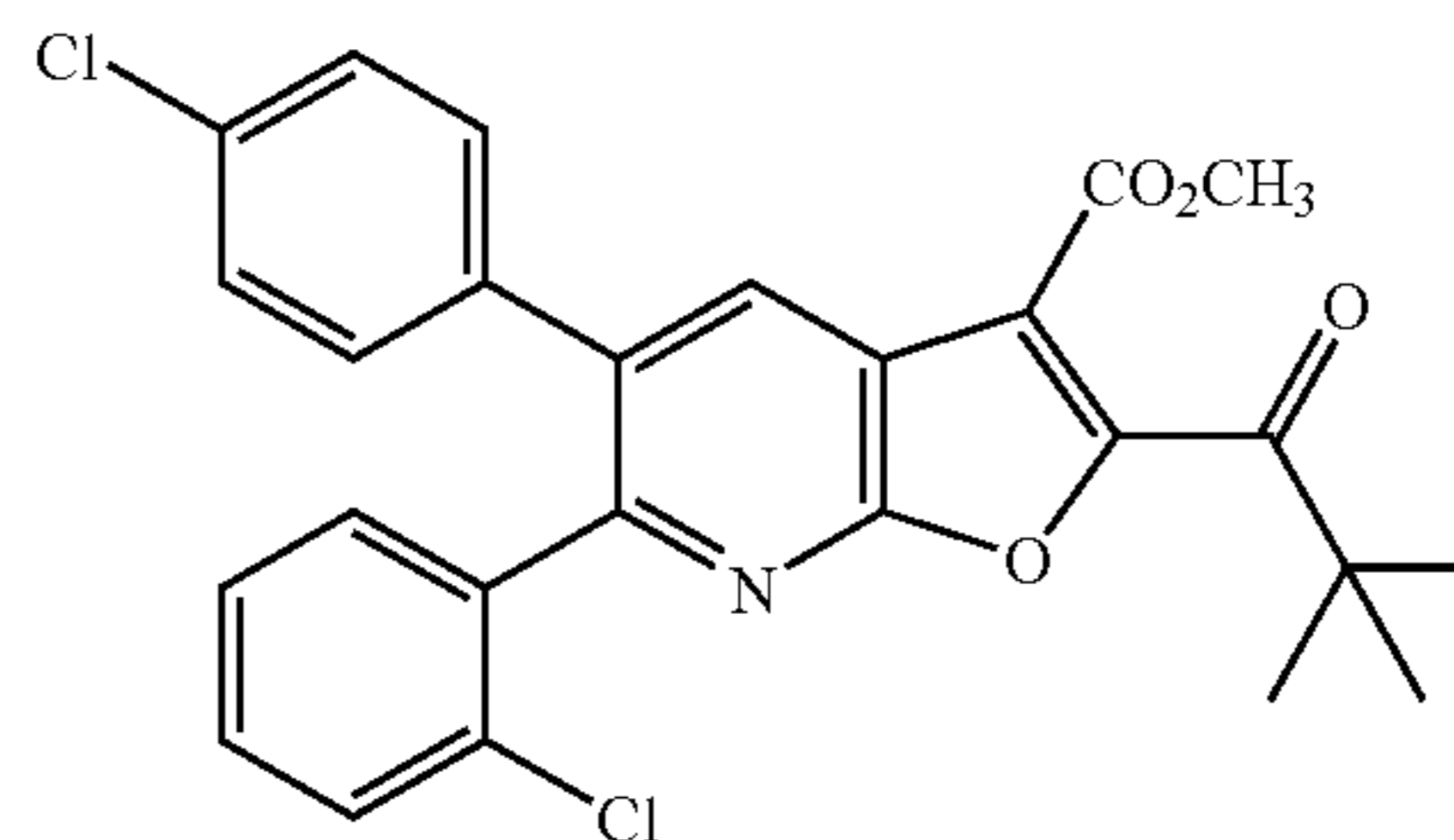
Methyl 6-(2-chlorophenyl)-5-(4-chlorophenyl)-2-(2,2-dimethylpropanoyl)furo[2,3-b]pyridine-3-carboxylate
