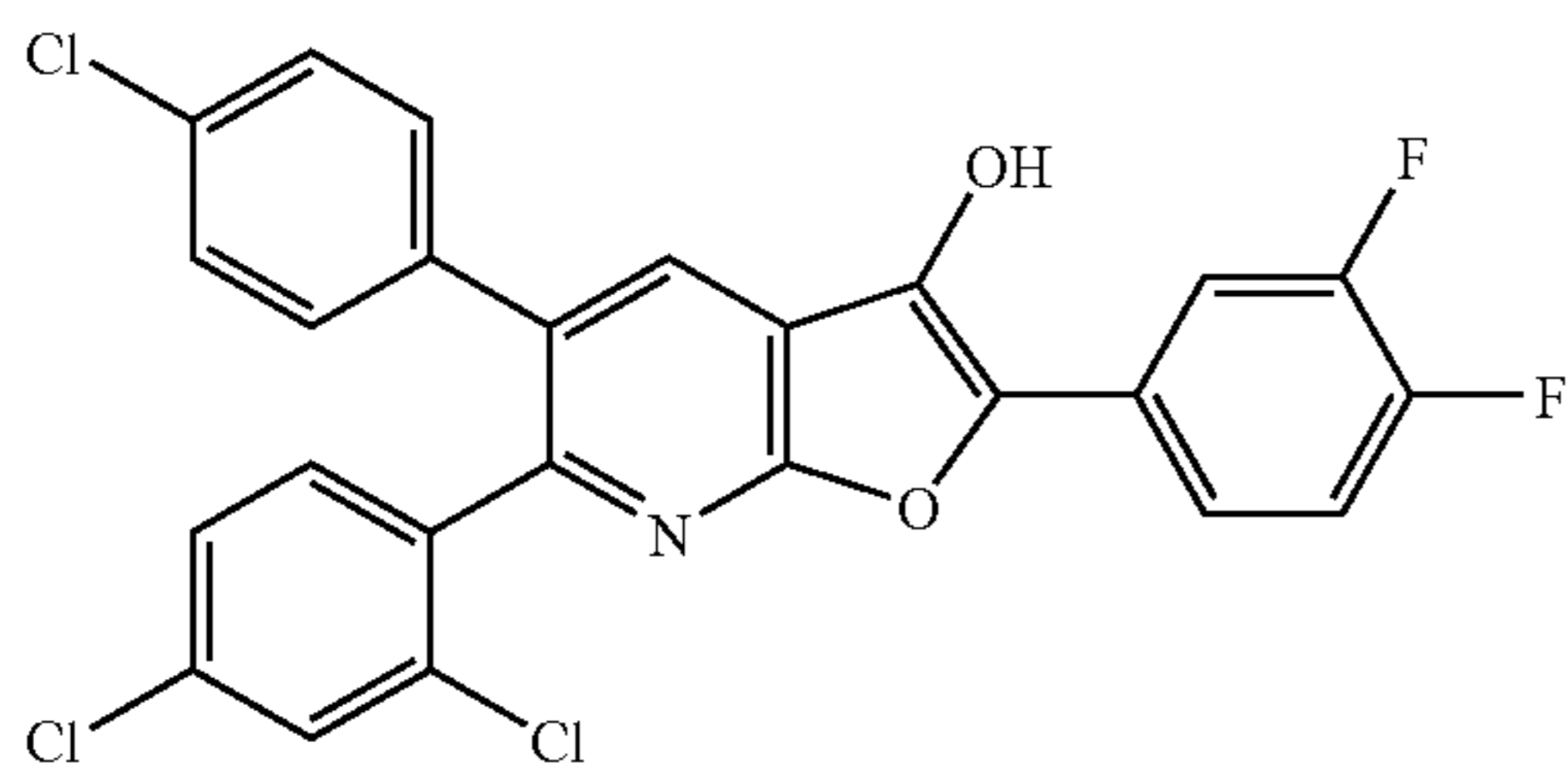
5-(4-Chlorophenyl)-6-(2,4-dichlorophenyl)-2-(3,4-difluorophenyl)furo[2,3-b]pyridin-3-ol
