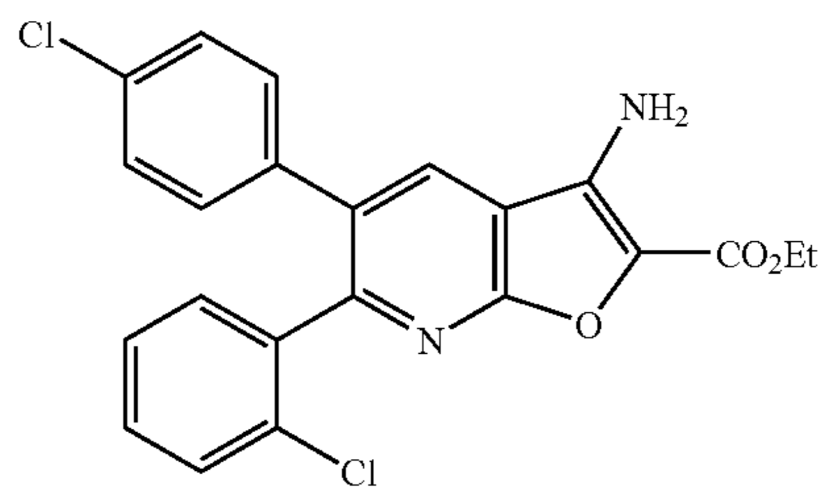
Ethyl 3-amino-6-(2-chlorophenyl)-5-(4-chlorophenyl)furo[2,3-b]pyridine-2-carboxylate
