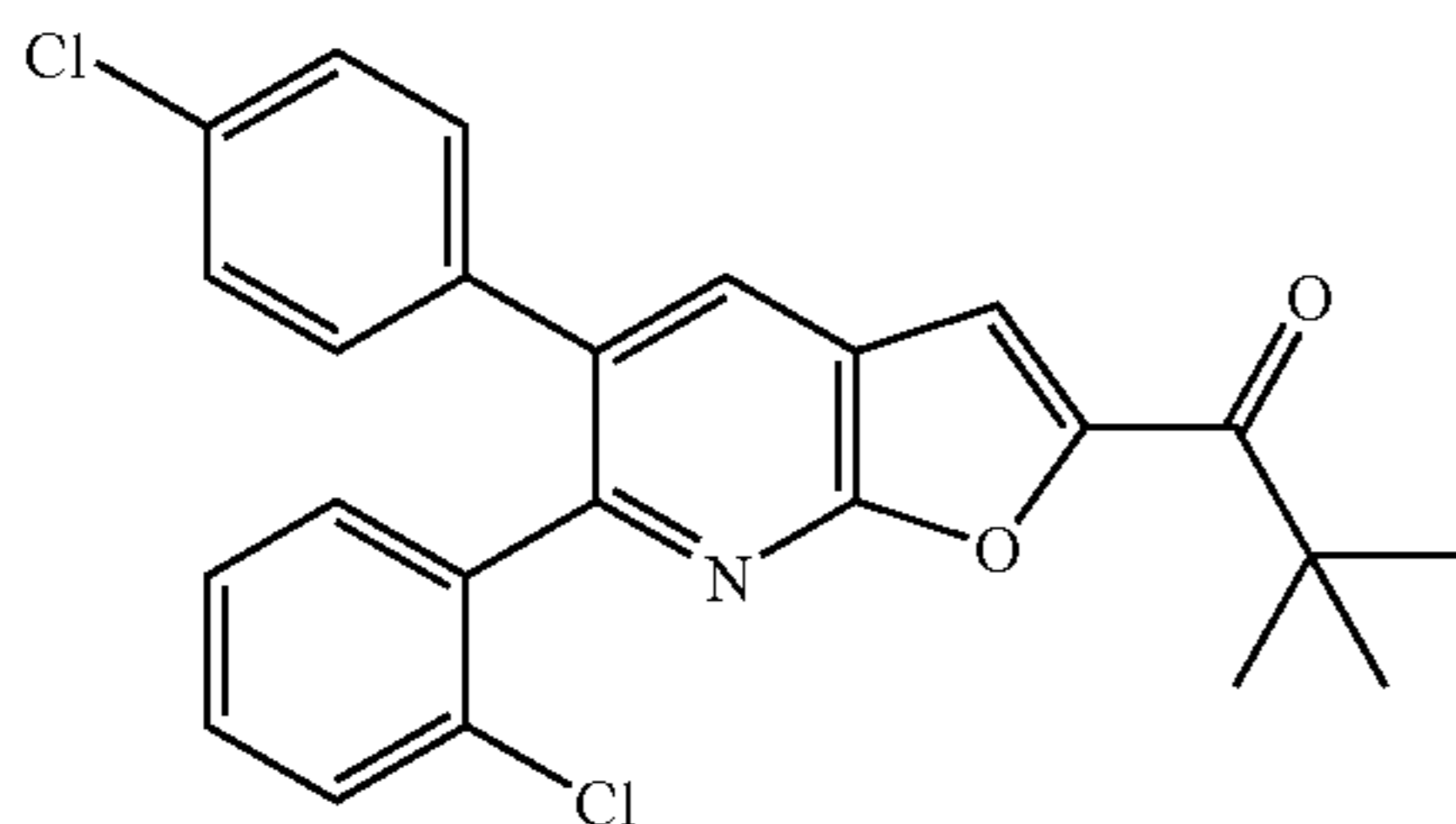
1-[6-(2-Chlorophenyl)-5-(4-chlorophenyl)furo[2,3-b]pyridin-2-yl]-2,2-dimethylpropan-1-one
