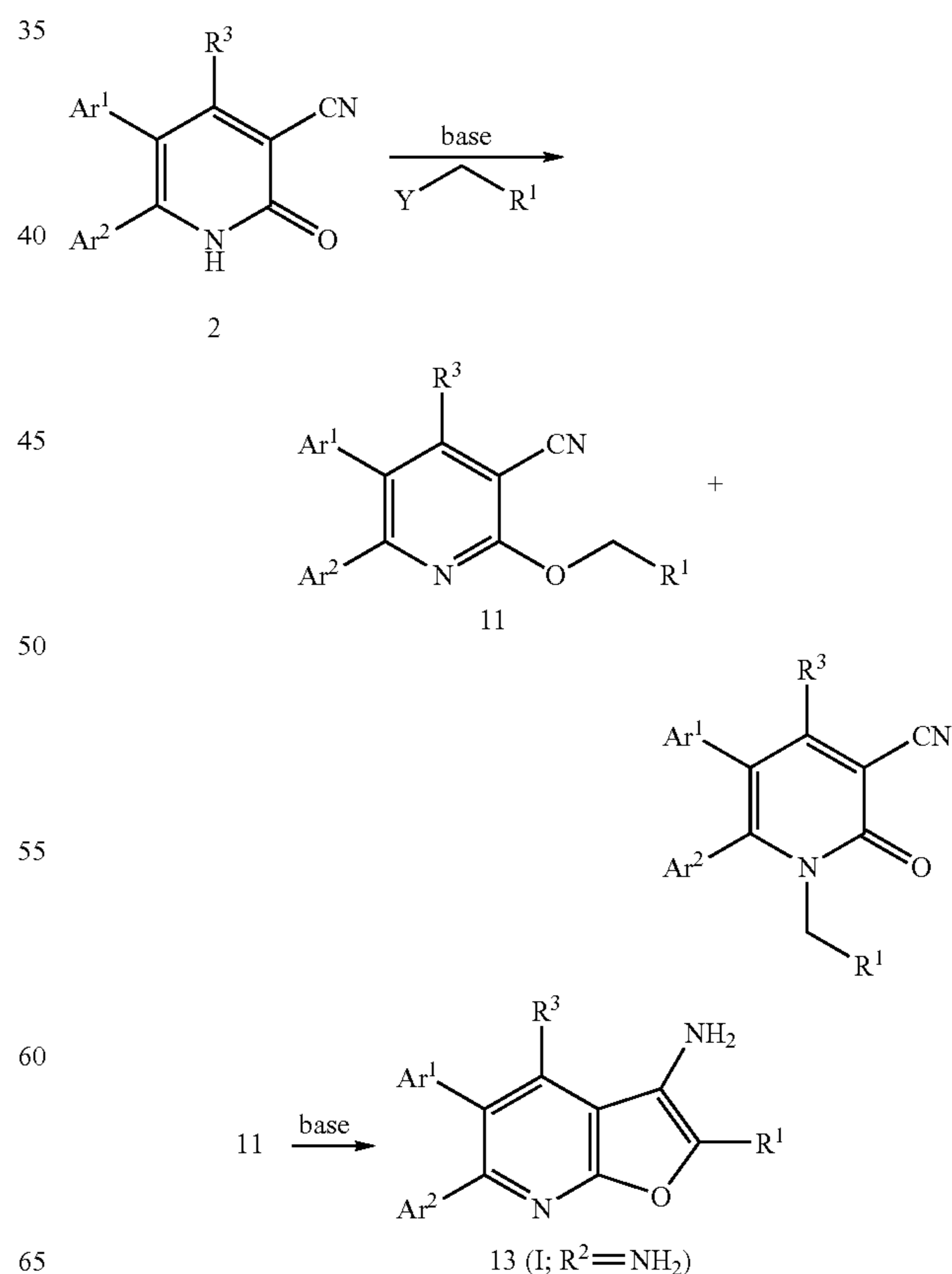
Scheme 4
