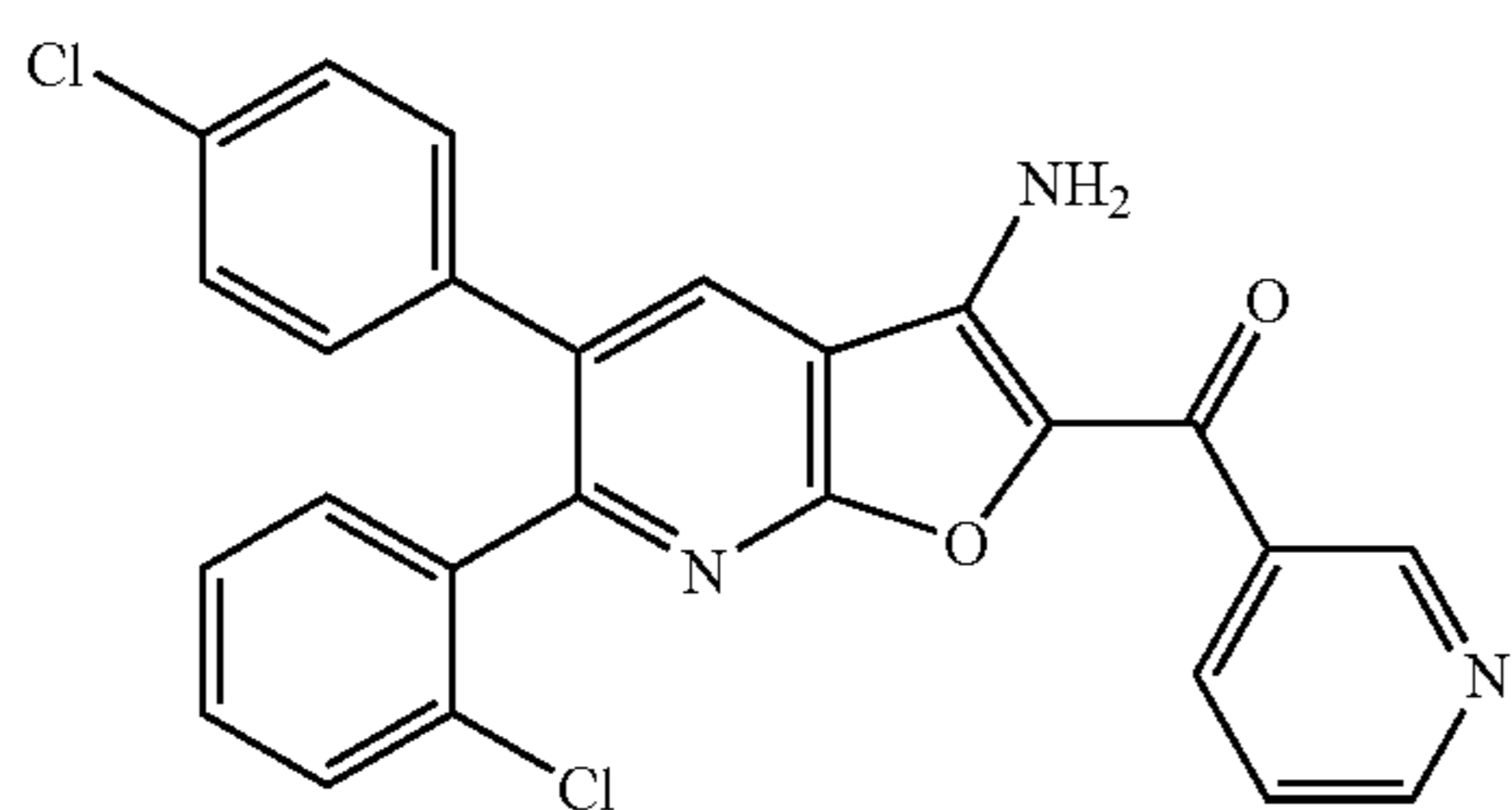
[3-Amino-6-(2-chlorophenyl)-5-(4-chlorophenyl)furo[2,3-b]pyridin-2-yl](pyridin-3-yl)methanone
