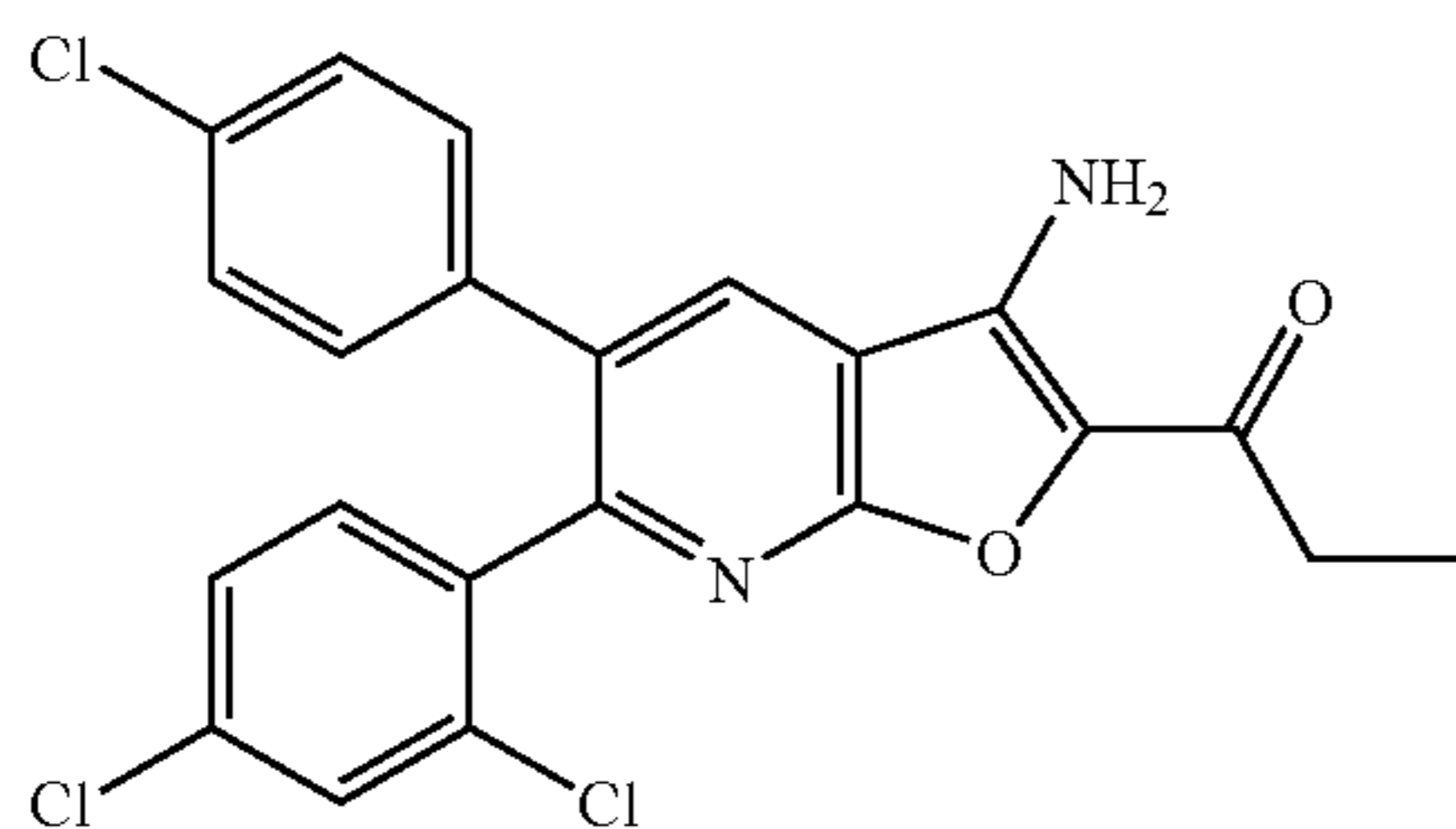
1-[3-Amino-5-(4-chlorophenyl)-6-(2,4-dichlorophenyl)furo[2,3-b]pyridin-2-yl]propan-1-one
