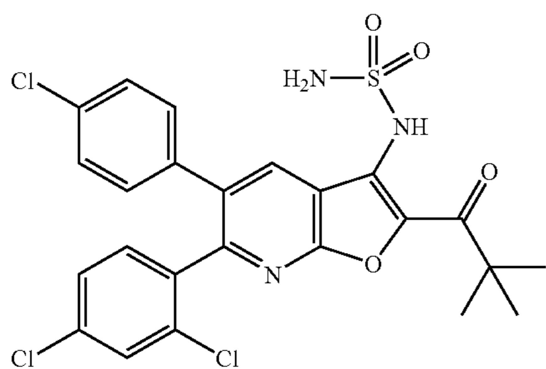
N-[5-(4-Chlorophenyl)-6-(2,4-dichlorophenyl)-2-(2,2-dimethylpropanoyl)furo[2,3-b]pyridin-3-yl]methanesulfonamide
