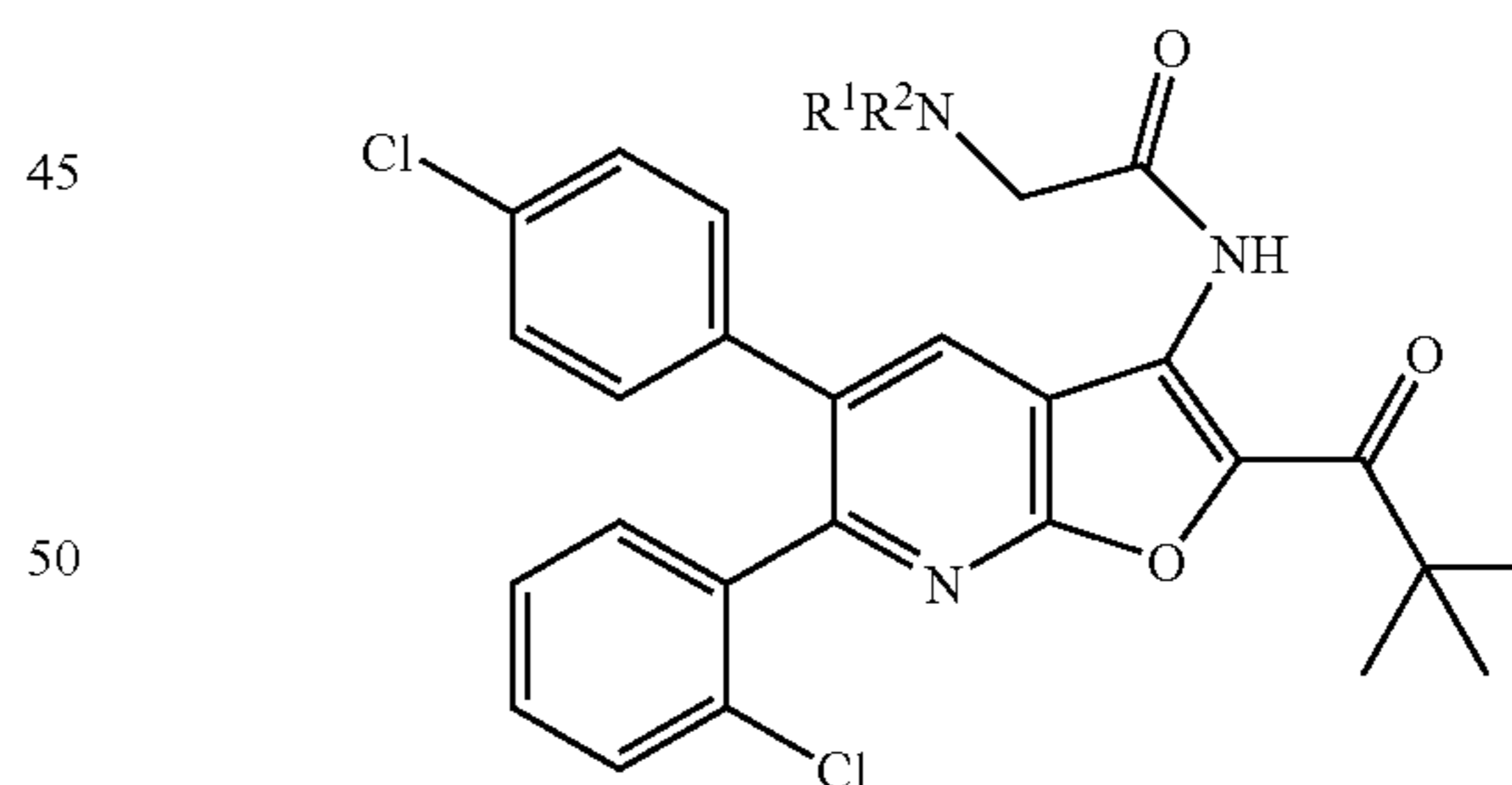
N-[6-(2-chlorophenyl)-5-(4-chlorophenyl)-2-(2,2-dimethylpropanoyl)furo[2,3-b]-pyridin-3-yl]-2-hydroxyacetamide
