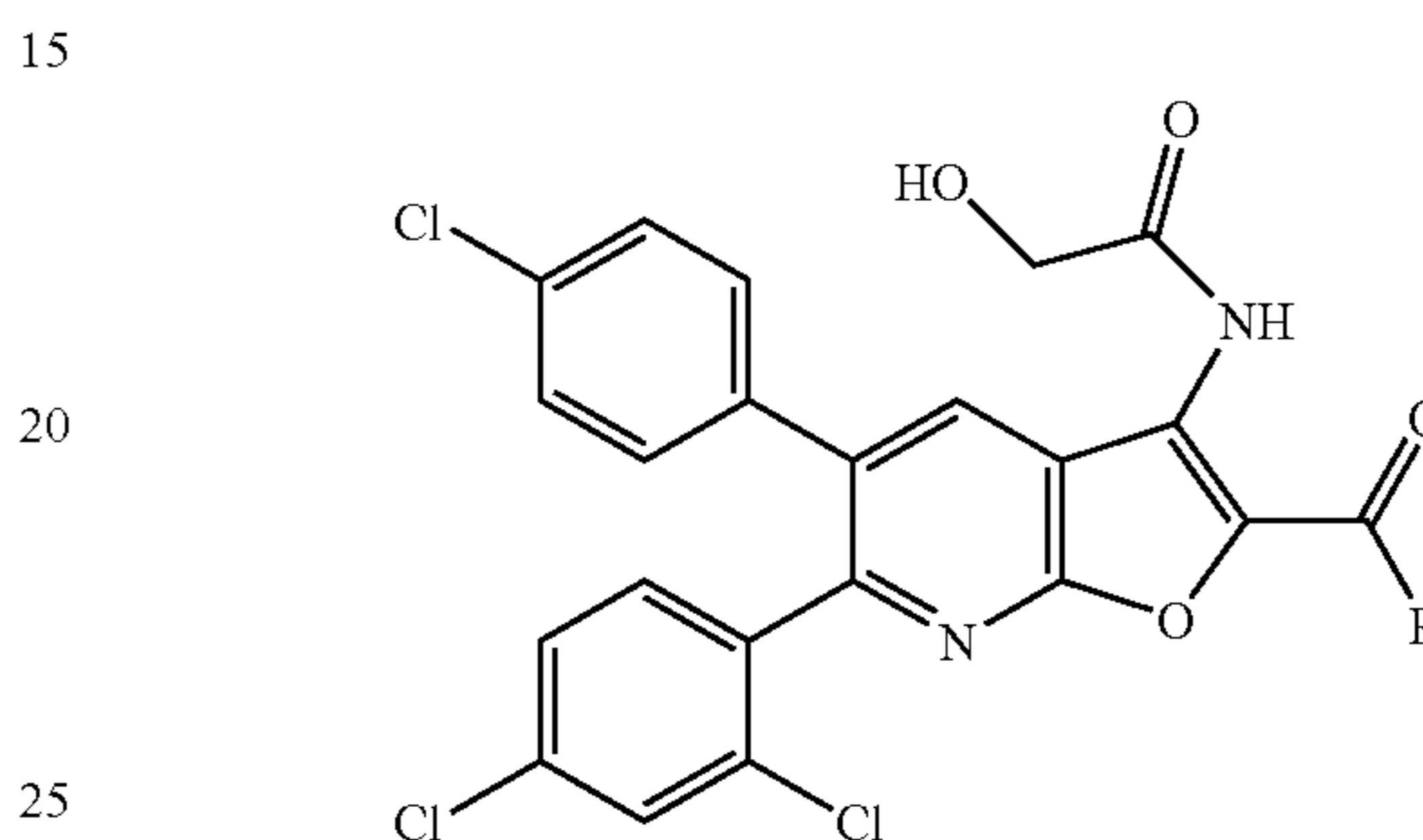
1-[3-Amino-5-(4-chlorophenyl)-6-(2,4-dichlorophenyl)furo[2,3-b]pyridin-2-yl]-2-methylpropan-1-one
