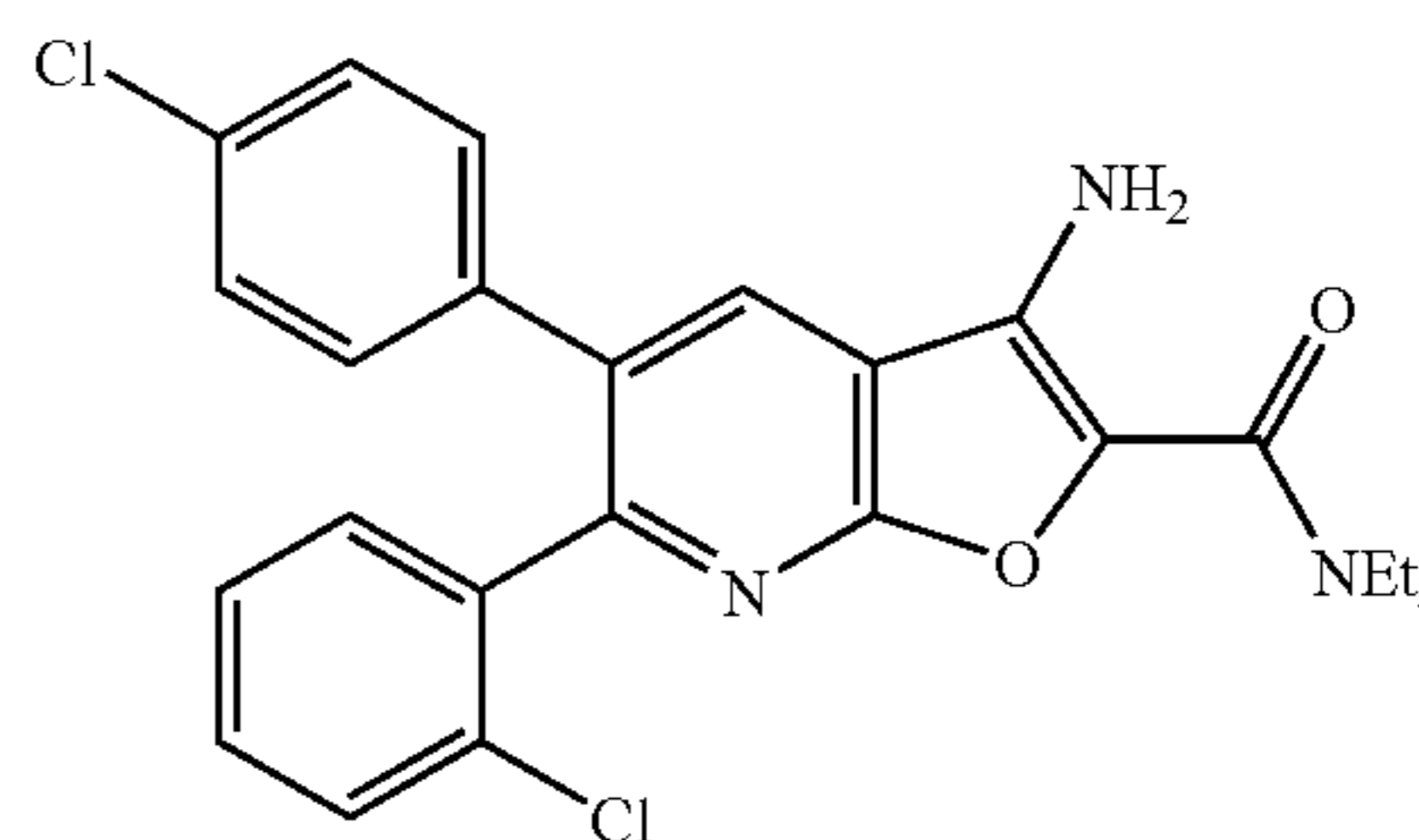
3-Amino-6-(2-chlorophenyl)-5-(4-chlorophenyl)-N,N-diethylfuro[2,3-b]pyridine-2-carboxamide
