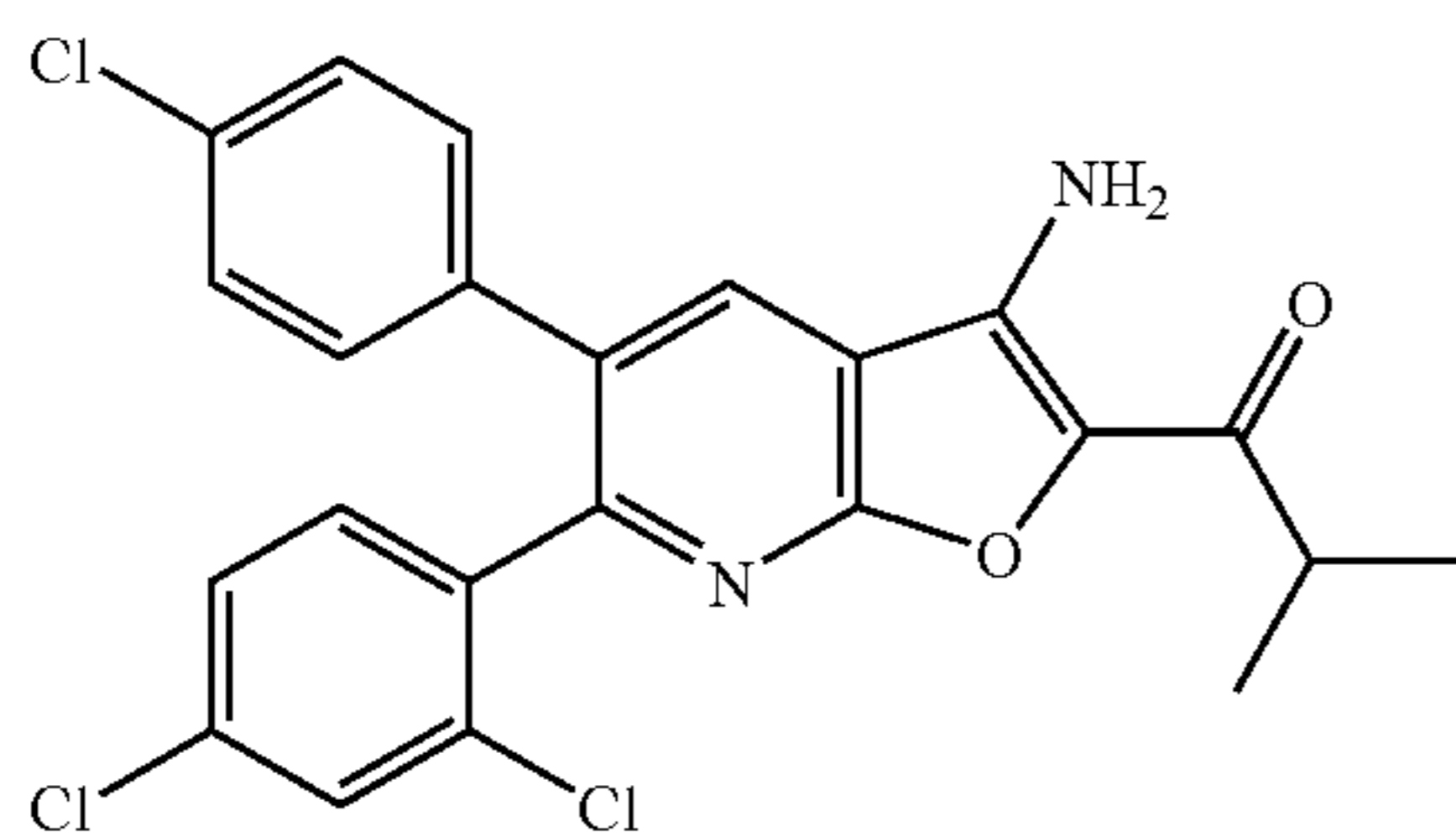
1-[3-Amino-5-(4-chlorophenyl)-6-(2,4-dichlorophenyl)furo[2,3-b]pyridin-2-yl]-2-methylpropan-1-one
