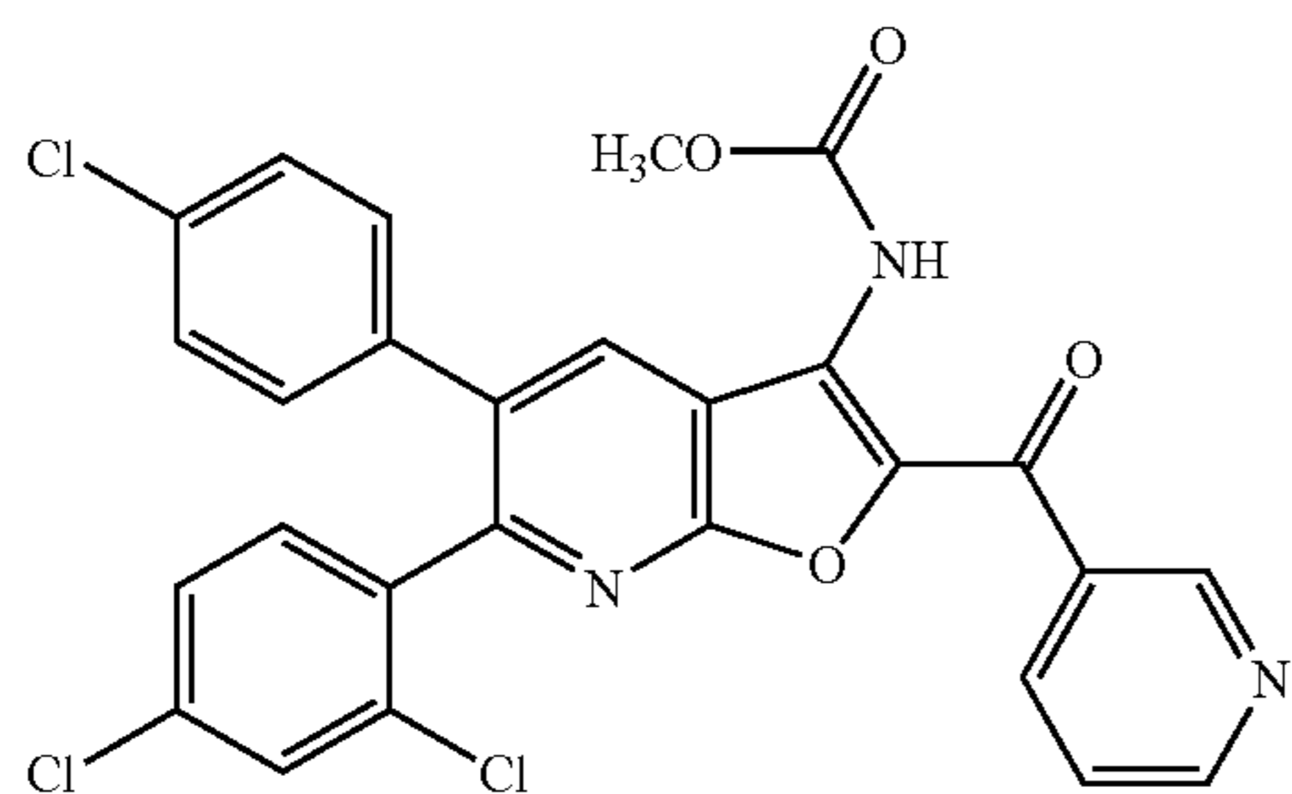
Methyl 5-(4-chlorophenyl)-6-(2,4-dichlorophenyl)-2-(pyridin-3-ylcarbonyl)furo[2,3-b]pyridin-3-ylcarbamate
