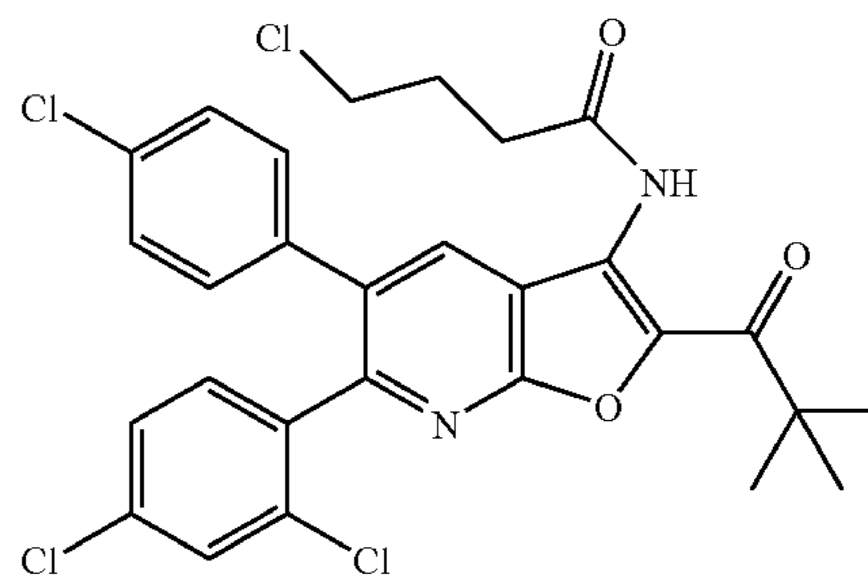
4-Chloro-N-[5-(4-chlorophenyl)-6-(2,4-dichlorophenyl)-2-(2,2-dimethylpropanoyl)furo[2,3-b]pyridin-3-yl]butanamide
