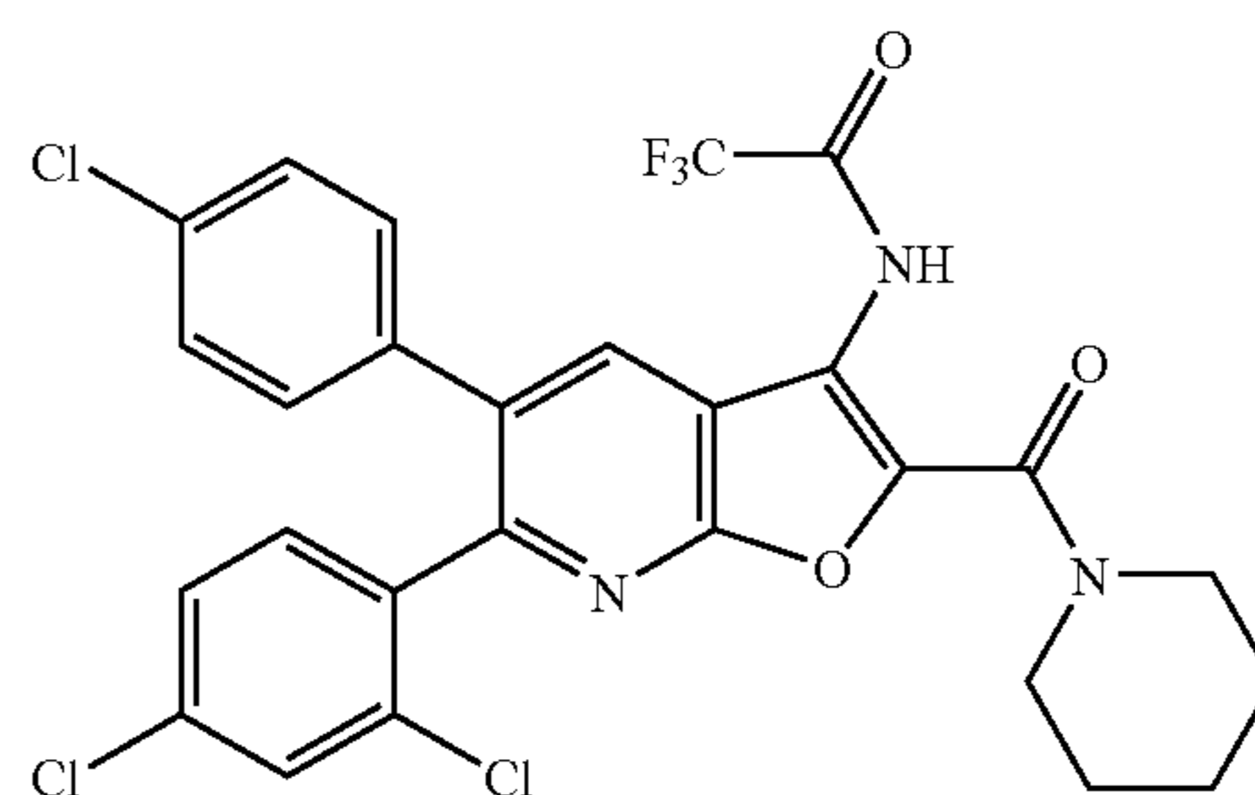
N-[5-(4-chlorophenyl)-6-(2,4-dichlorophenyl)-2-(piperidin-1-ylcarbonyl)furo[2,3-b]pyridin-3-yl]-2,2,2-trifluoroacetamide
