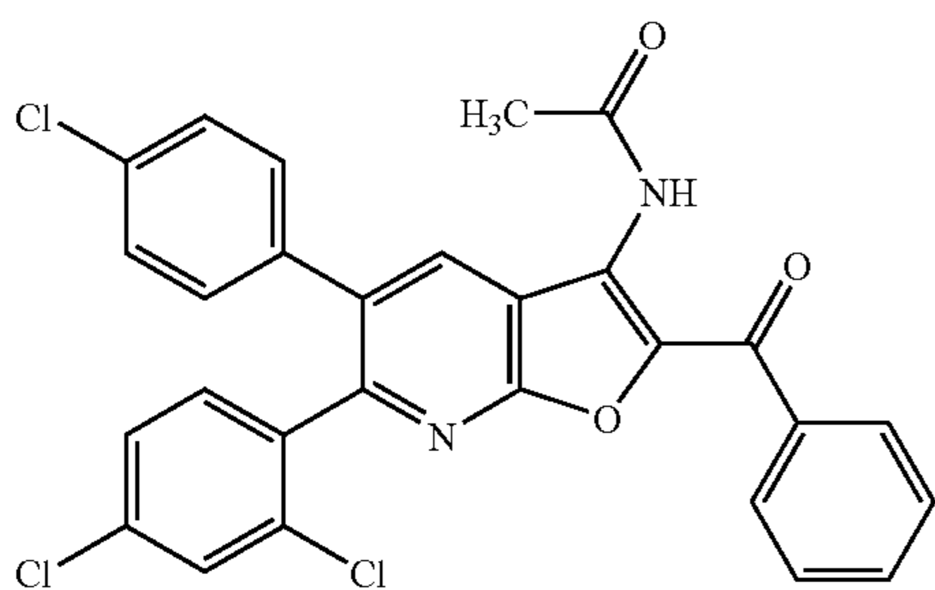
N-[2-Benzol-5-(4-chlorophenyl)-6-(2,4-dichlorophenyl)furo[2,3-b]pyridin-3-yl]acetamide
