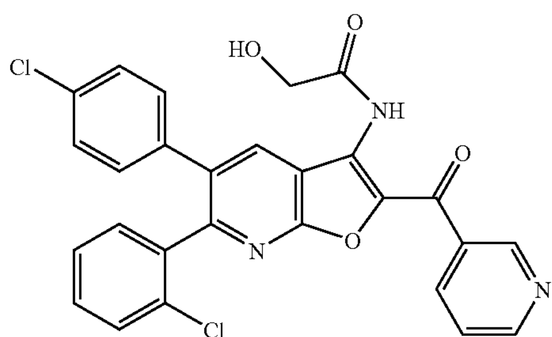
N-[6-(2-chlorophenyl)-5-(4-chlorophenyl)-2-(pyridin-3-ylcarbonyl)furo[2,3-b]pyridin-3-yl]-2-hydroxyacetamide
