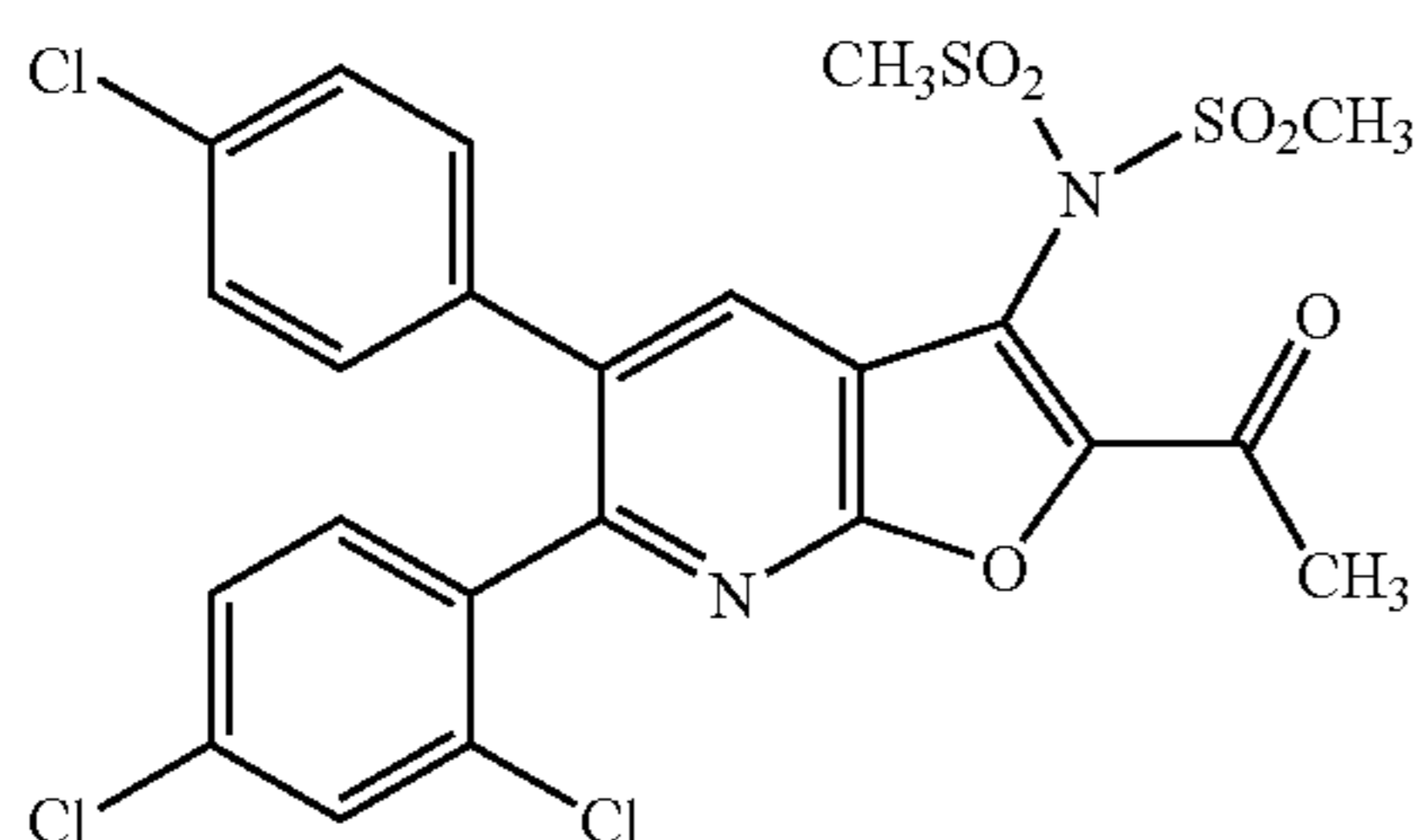
N-[2-Acetyl-5-(4-chlorophenyl)-6-(2,4-dichlorophenyl)furo[2,3-b]pyridin-3-yl]-N-(methylsulfonyl)methanesulfonamide
