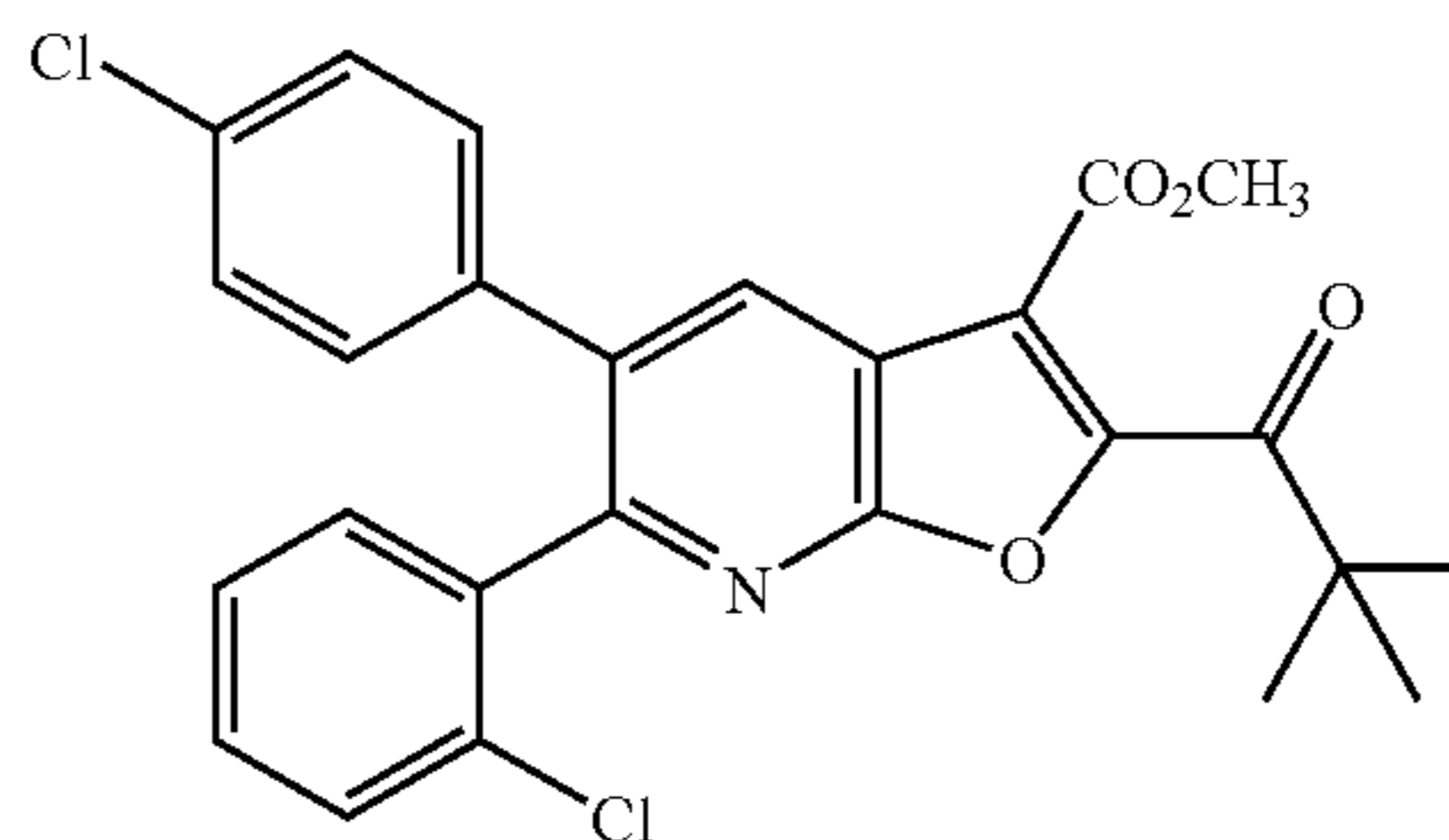
Methyl 6-(2-chlorophenyl)-5-(4-chlorophenyl)-2-(2,2-dimethylpropanoyl)furo[2,3-b]pyridine-3-carboxylate
