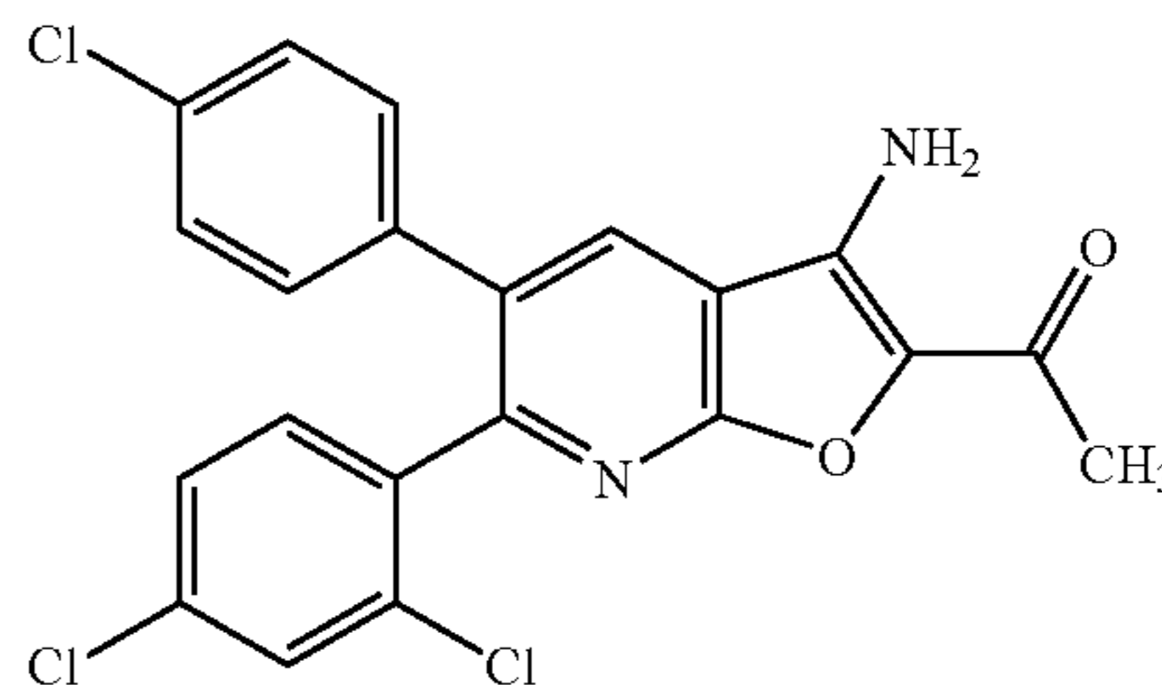
1-[3-Amino-5-(4-chlorophenyl)-6-(2,4-dichlorophenyl)furo[2,3-b]pyridin-2-yl]ethanone
