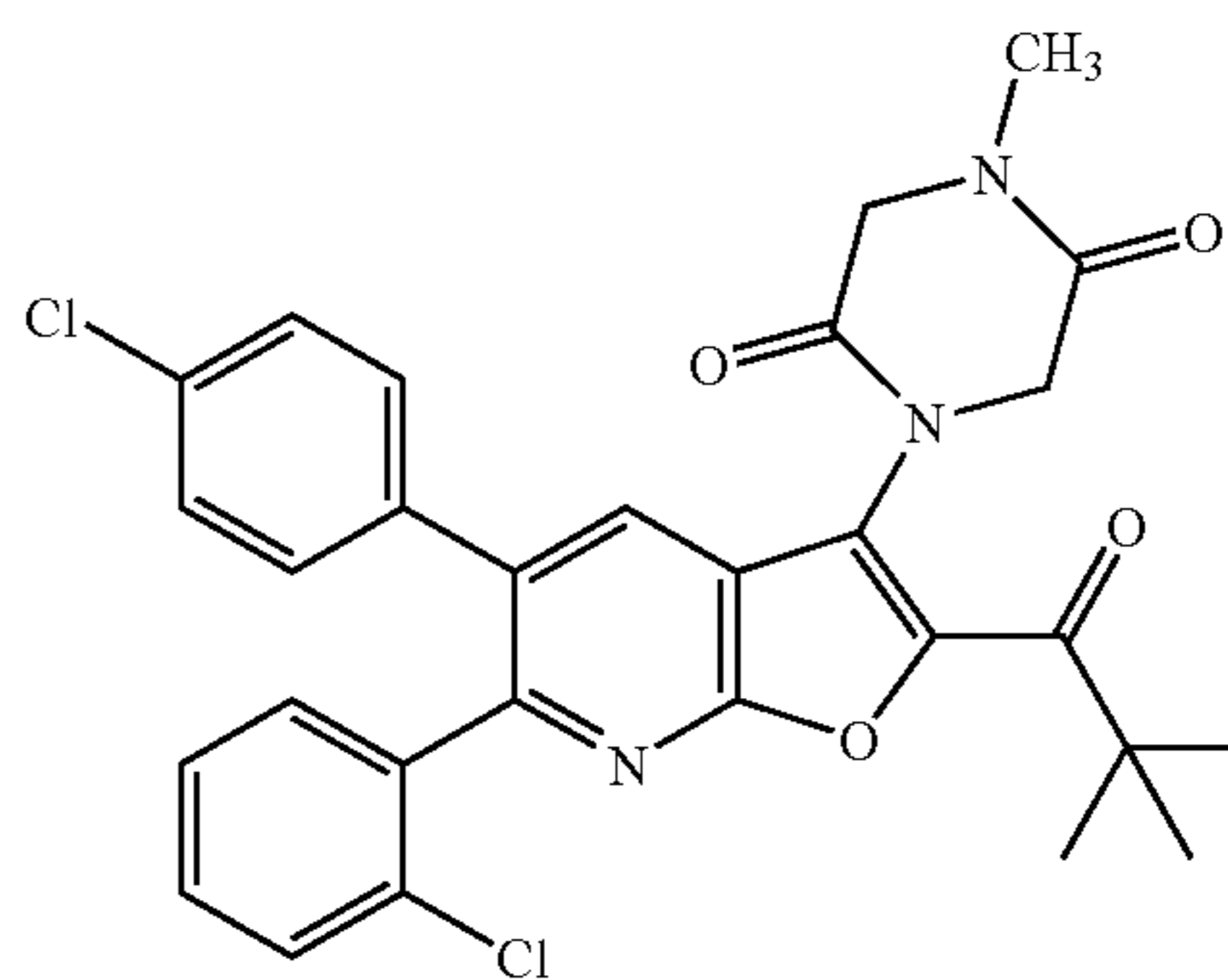
1-[6-(2-Chlorophenyl)-5-(4-chlorophenyl)-2-(2,2-dimethylpropanoyl)furo[2,3-b]pyridin-3-yl]-4-methylpiperazine-2,5-dione
