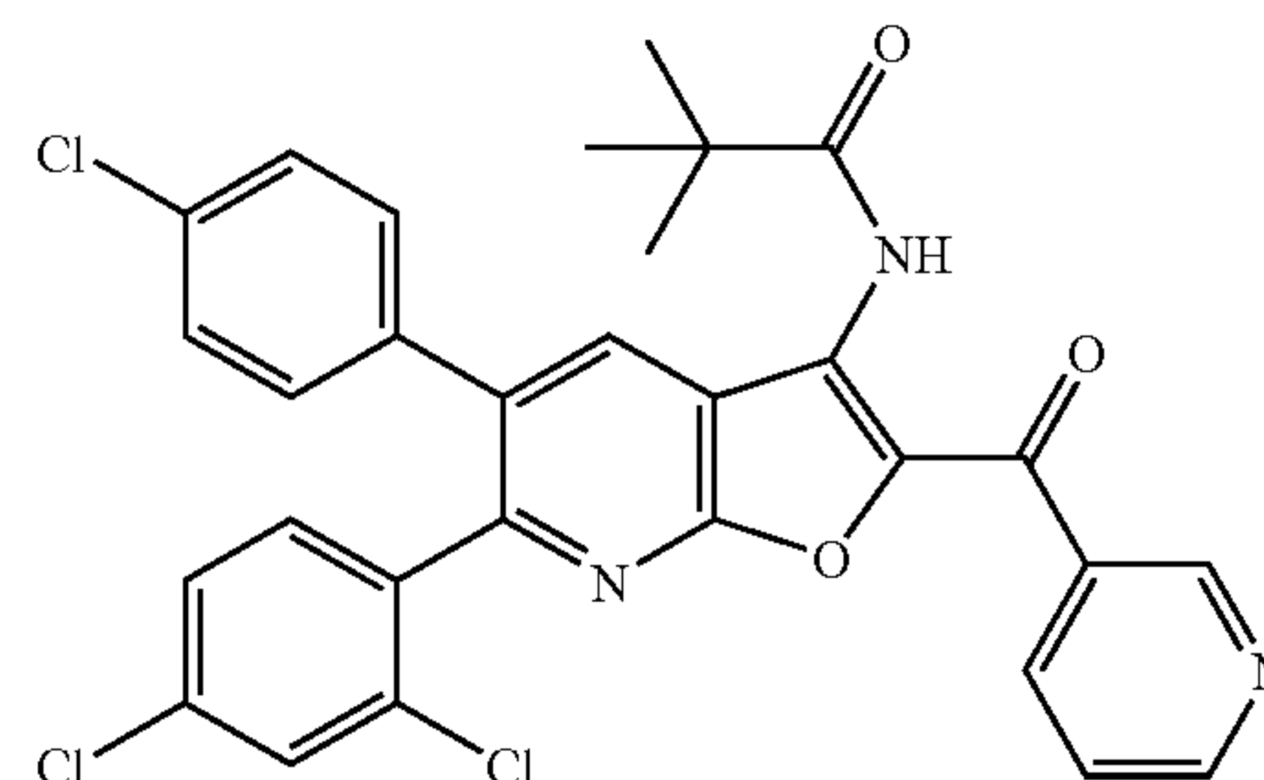
N-[5-(4-Chlorophenyl)-6-(2,4-dichlorophenyl)-2-(pyridin-3-ylcarbonyl)furo[2,3-b]pyridin-3-yl]-2,2-dimethylpropanamide
