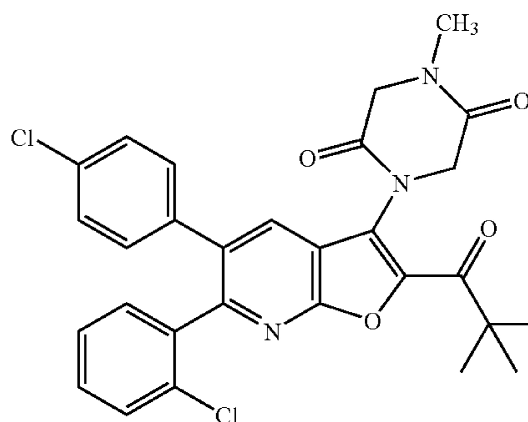
1-[6-(2-Chlorophenyl)-5-(4-chlorophenyl)-2-(2,2-dimethylpropanoyl)furo[2,3-b]pyridin-3-yl]-4-methylpiperazine-2,5-dione
