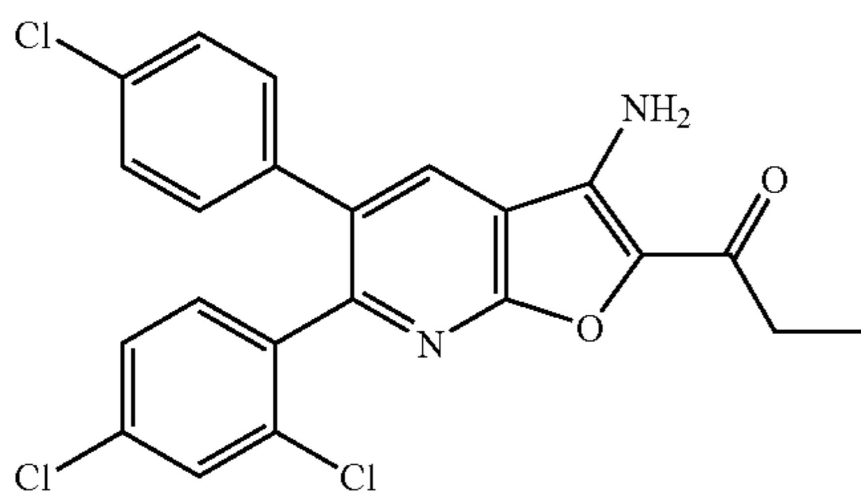
1-[3-Amino-5-(4-chlorophenyl)-6-(2,4-dichlorophenyl)furo[2,3-b]pyridin-2-yl]propan-1-one
