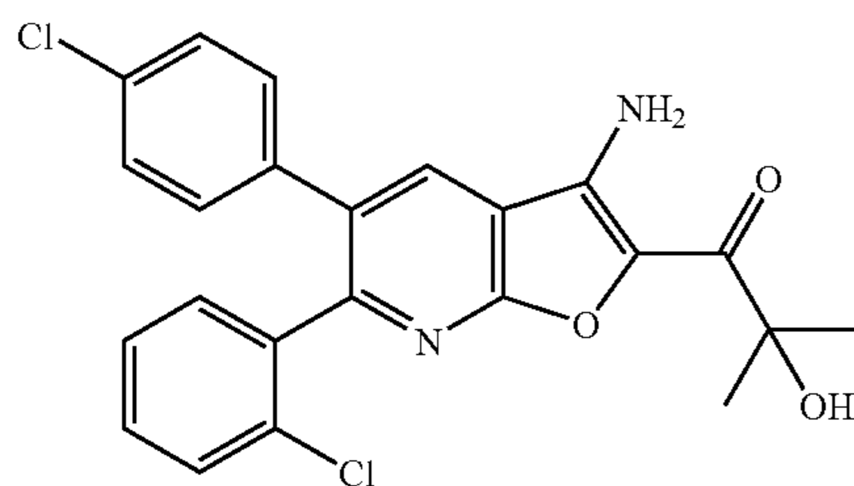
1-[3-Amino-6-(2-chlorophenyl)-5-(4-chlorophenyl)furo[2,3-b]pyridin-2-yl]-2-hydroxy-2-methylpropan-1-one
