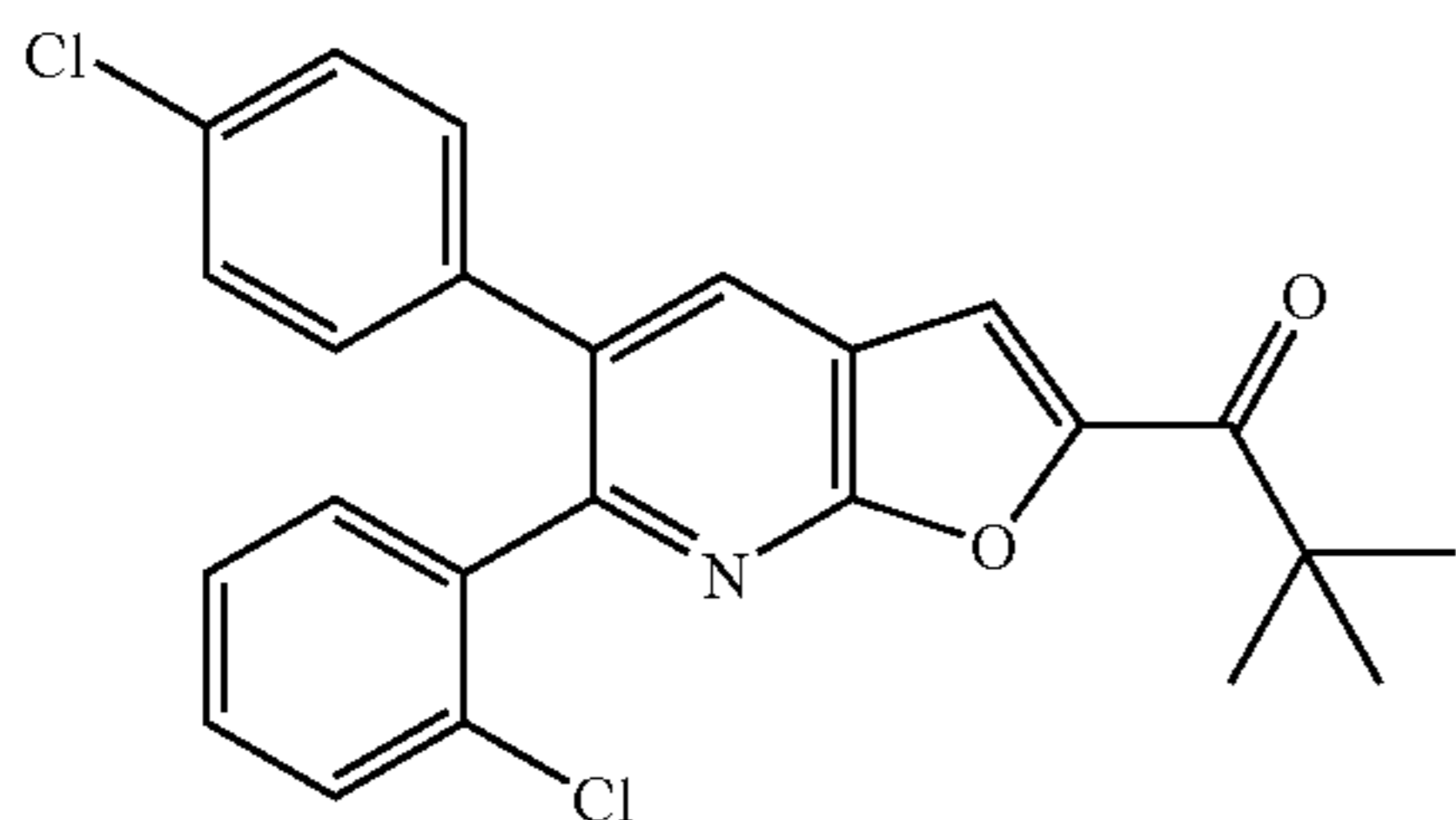
1-[6-(2-Chlorophenyl)-5-(4-chlorophenyl)furo[2,3-b]pyridin-2-yl]-2,2-dimethylpropan-1-one
