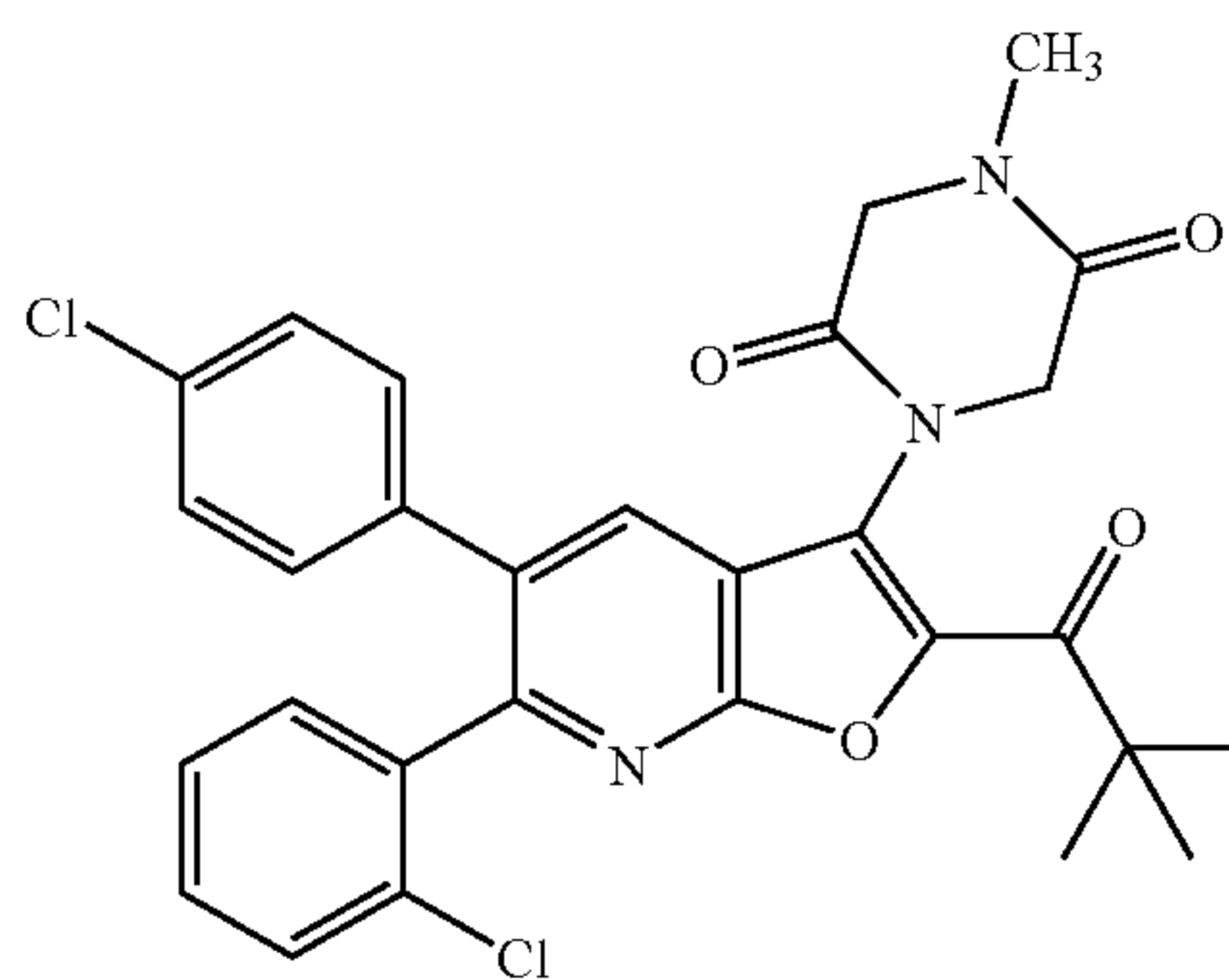
1-[6-(2-Chlorophenyl)-5-(4-chlorophenyl)-2-(2,2-dimethylpropanoyl)furo[2,3-b]pyridin-3-yl]-4-methylpiperazine-2,5-dione
