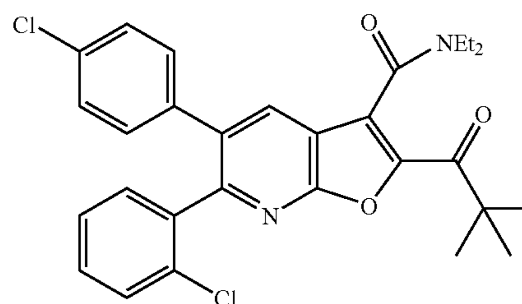
6-(2-Chlorophenyl)-5-(4-chlorophenyl)-2-(2,2-dimethylpropanoyl)-N,N-diethylfuro[2,3-b]pyridine-3-carboxamide
