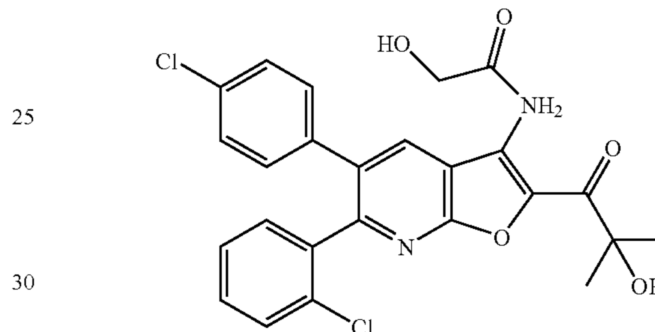
N-[6-(2-Chlorophenyl)-5-(4-chlorophenyl)-2-(2-hydroxy-2-methylpropanoyl)furo[2,3-b]pyridin-3-yl]-2-hydroxyacetamide
