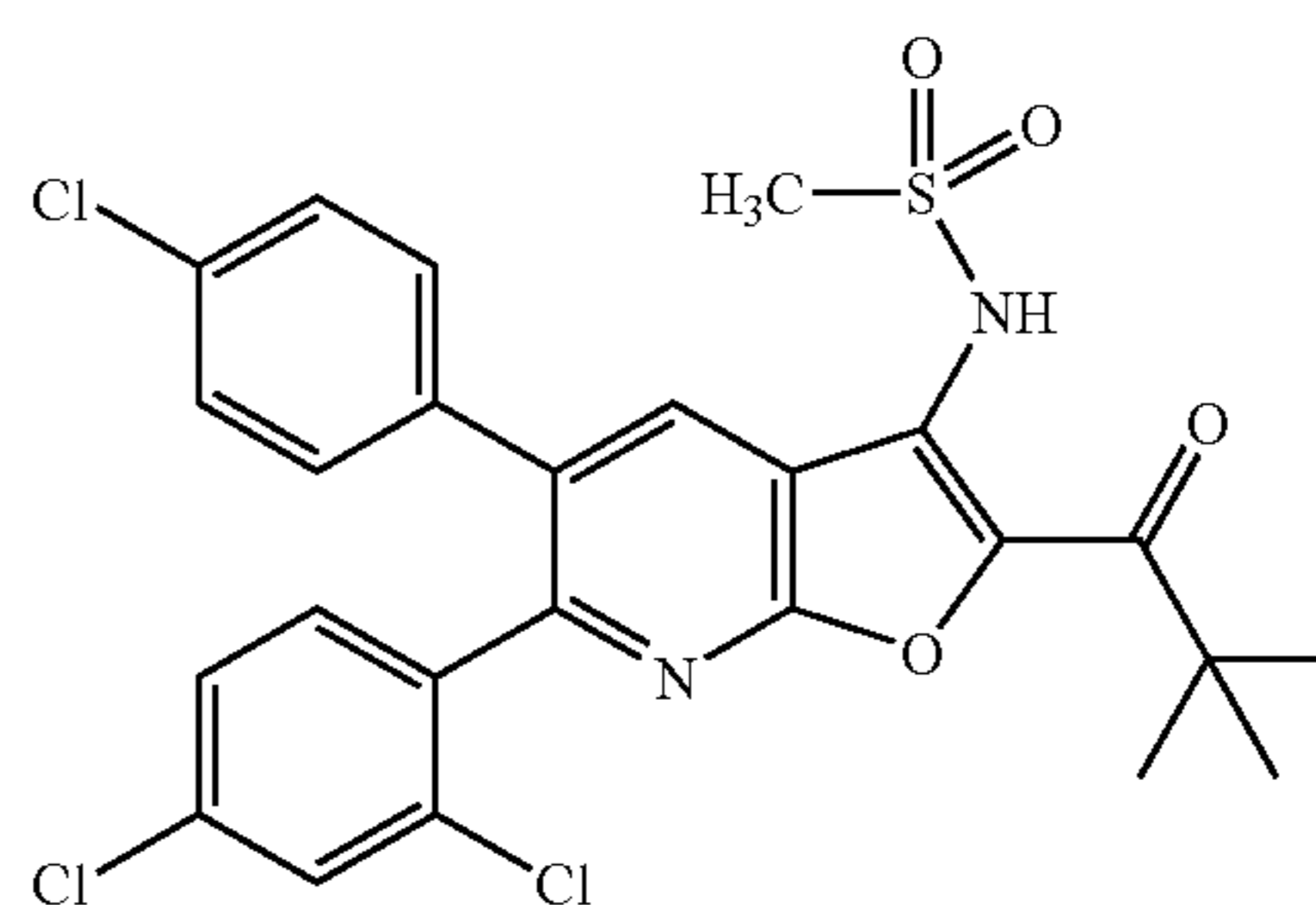
N-[5-(4-Chlorophenyl)-6-(2,4-dichlorophenyl)-2-(2,2-dimethylpropanoyl)furo[2,3-b]pyridin-3-yl]methanesulfonamide
