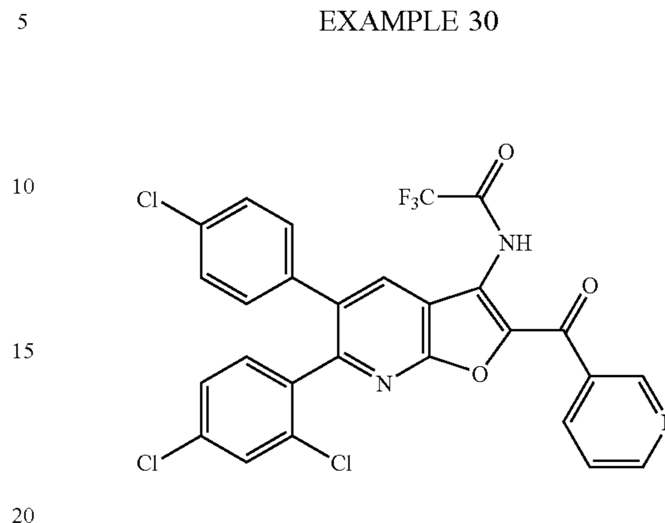
N-[5-(4-Chlorophenyl)-6-(2,4-dichlorophenyl)-2-(pyridin-3-ylcarbonyl)furo[2,3-b]pyridin-3-yl]-2,2,2-trifluoroacetamide
