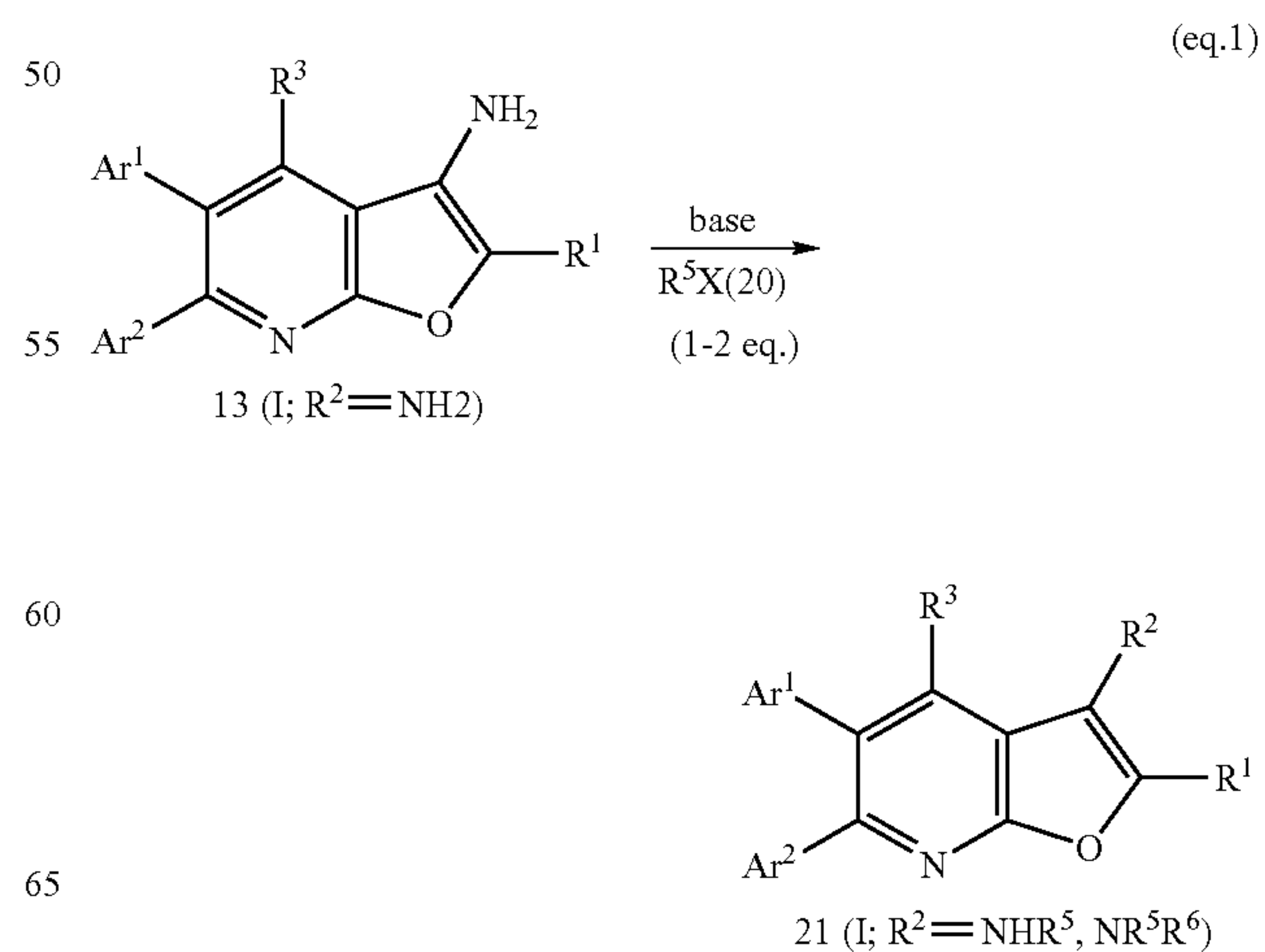
Scheme 7
