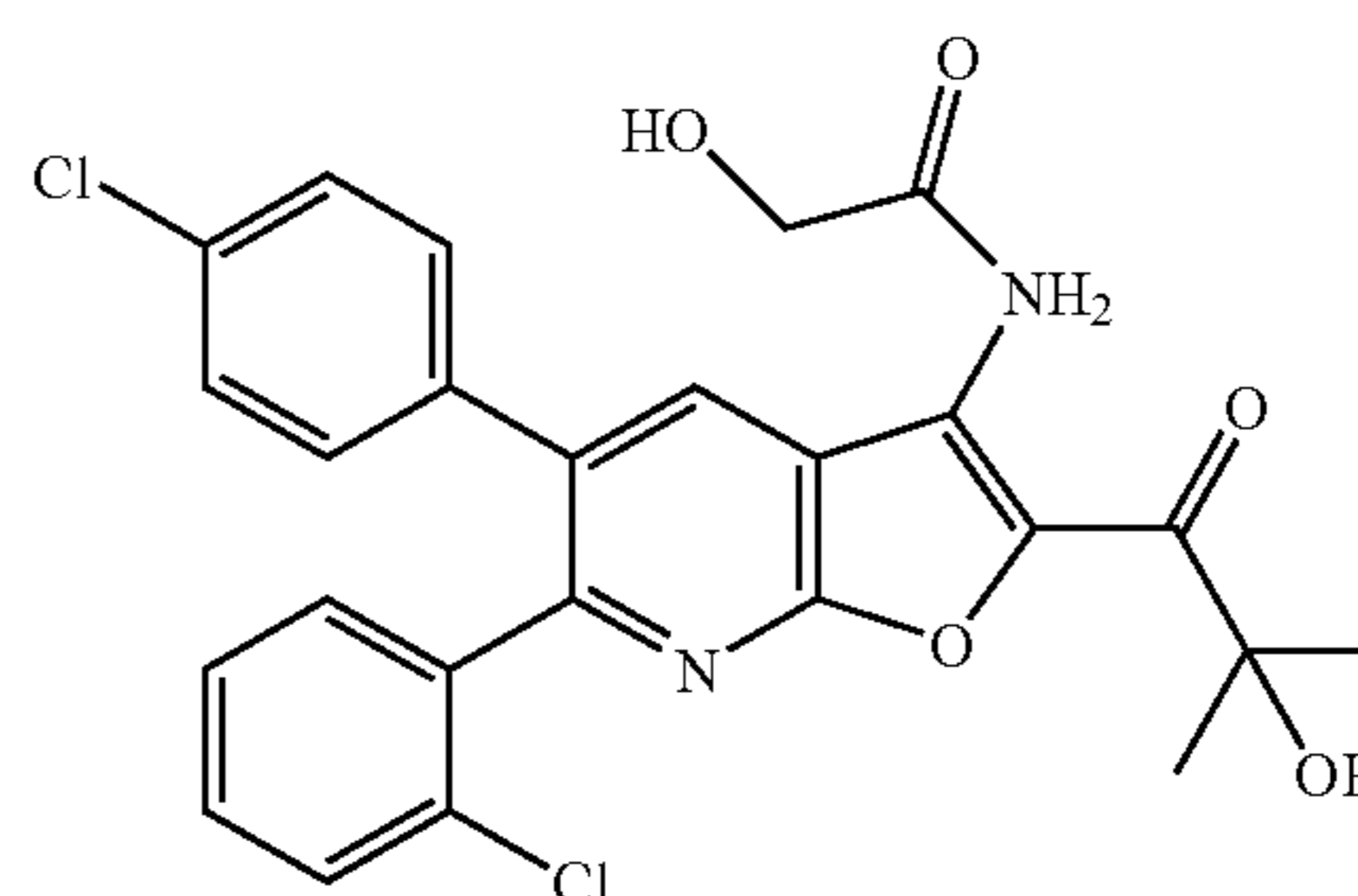
N-[6-(2-Chlorophenyl)-5-(4-chlorophenyl)-2-(2-hydroxy-2-methylpropanoyl)furo[2,3-b]pyridin-3-yl]-2-hydroxyacetamide
