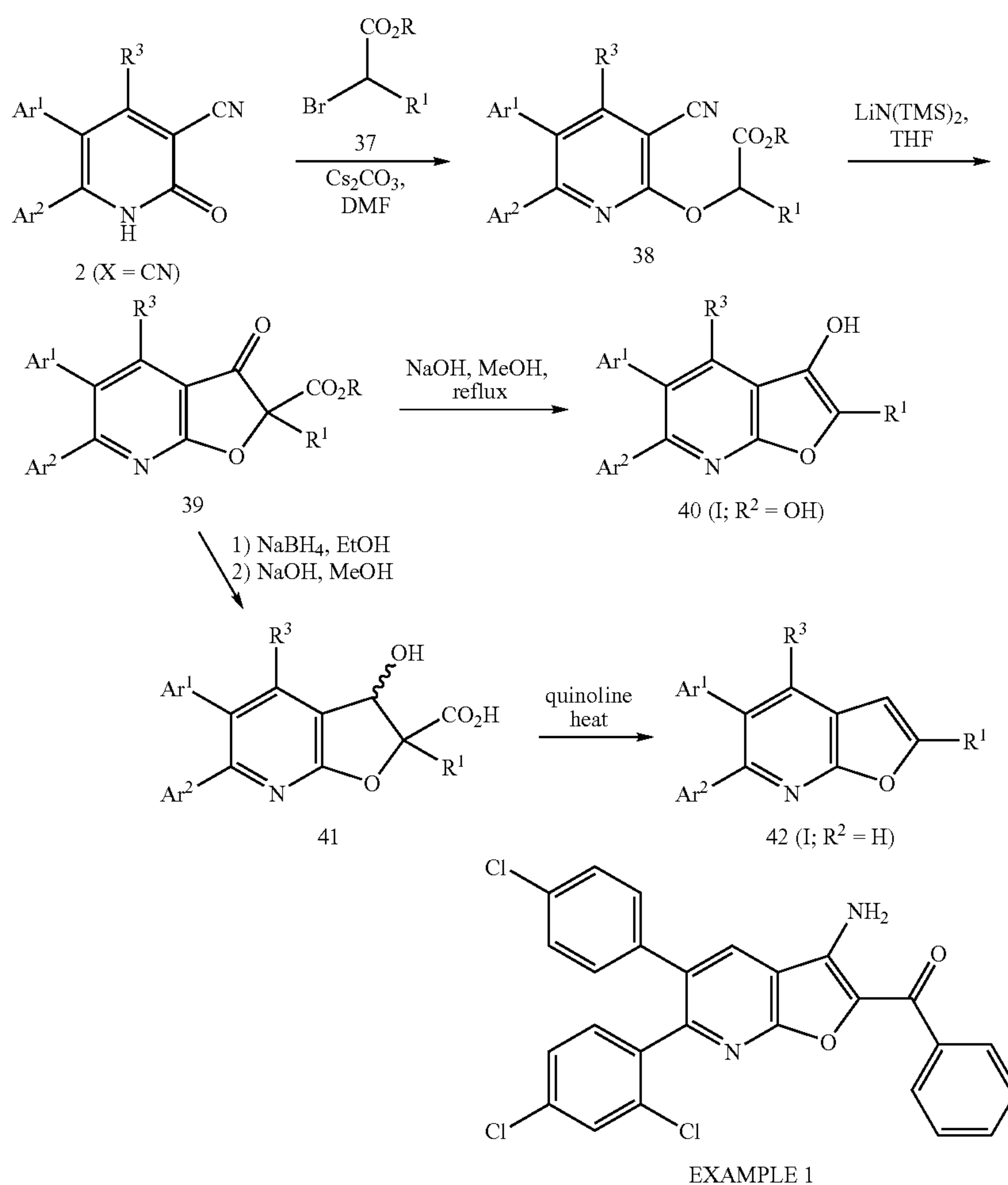
Scheme 12
