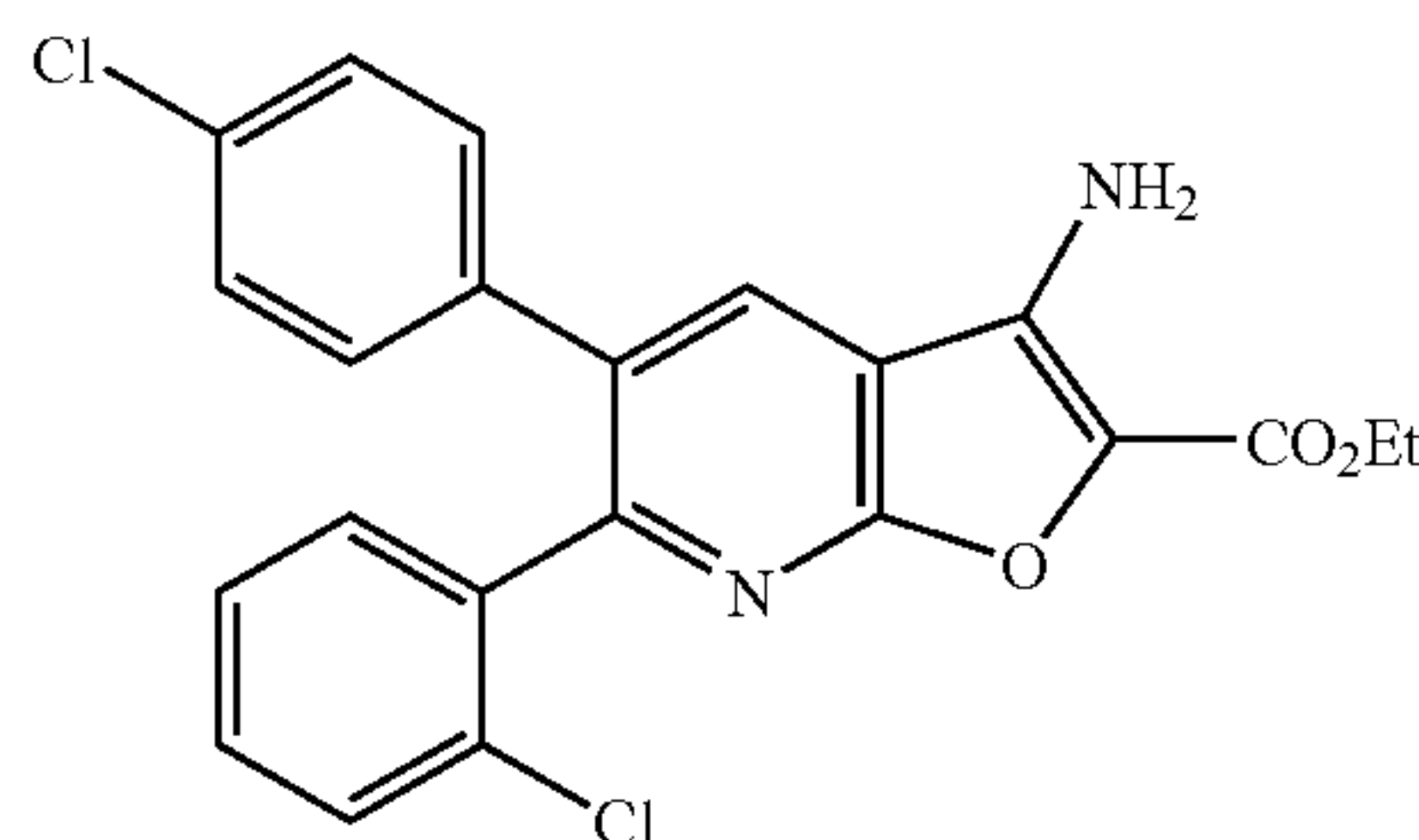
Ethyl 3-amino-6-(2-chlorophenyl)-5-(4-chlorophenyl)furo[2,3-b]pyridine-2-carboxylate
