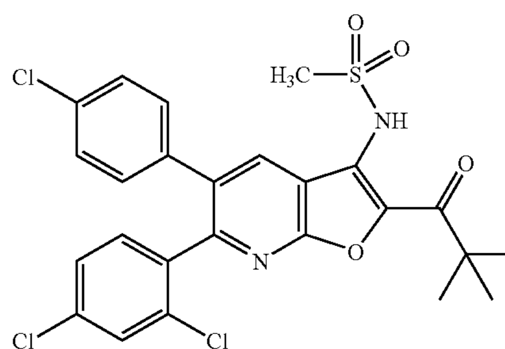
N-[5-(4-Chlorophenyl)-6-(2,4-dichlorophenyl)-2-(2,2-dimethylpropanoyl)furo[2,3-b]pyridin-3-yl]methanesulfonamide
