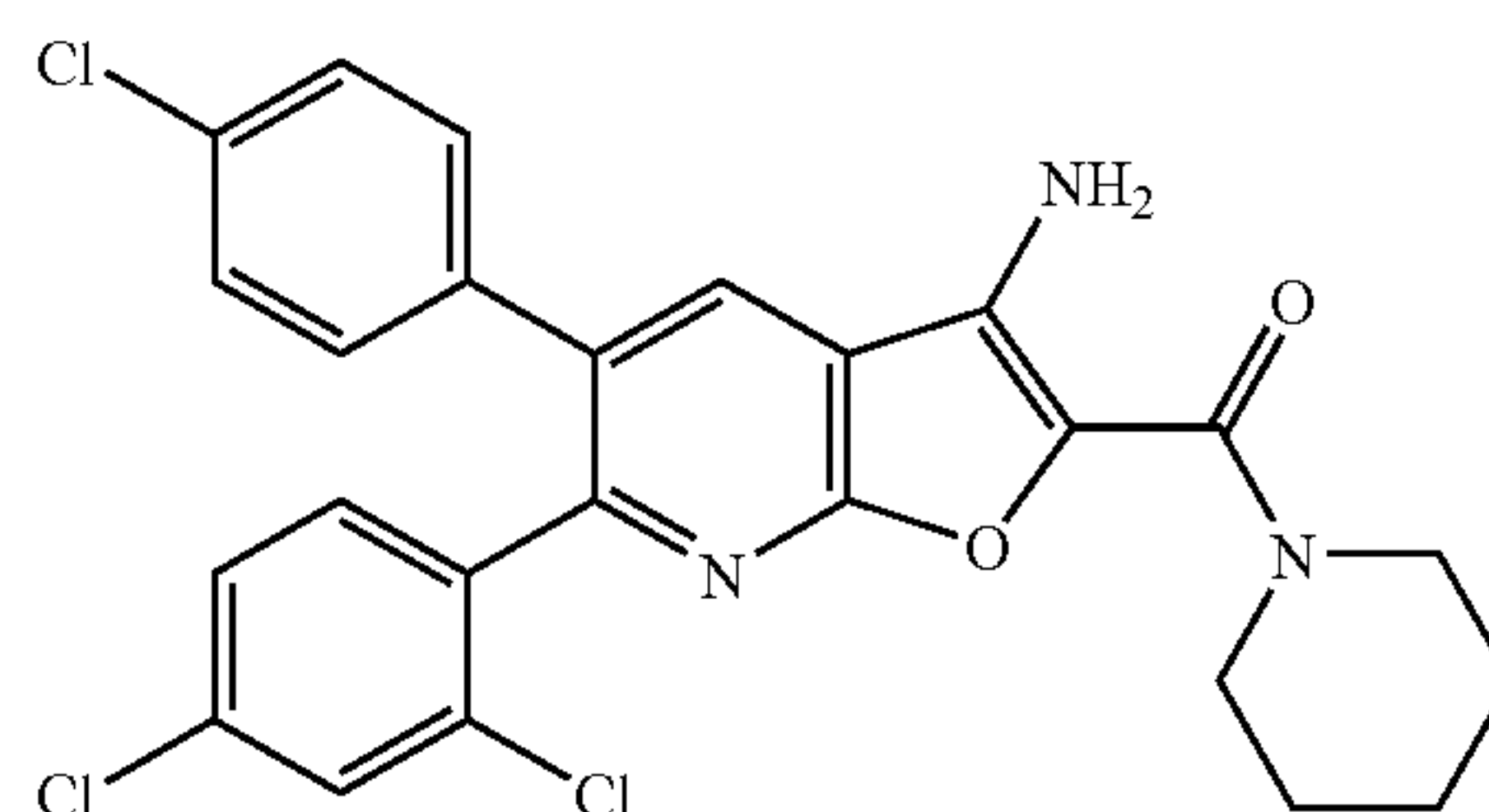
5-(4-Chlorophenyl)-6-(2,4-dichlorophenyl)-2-(piperidin-1-ylcarbonyl)furo[2,3-b]pyridin-3-amine
