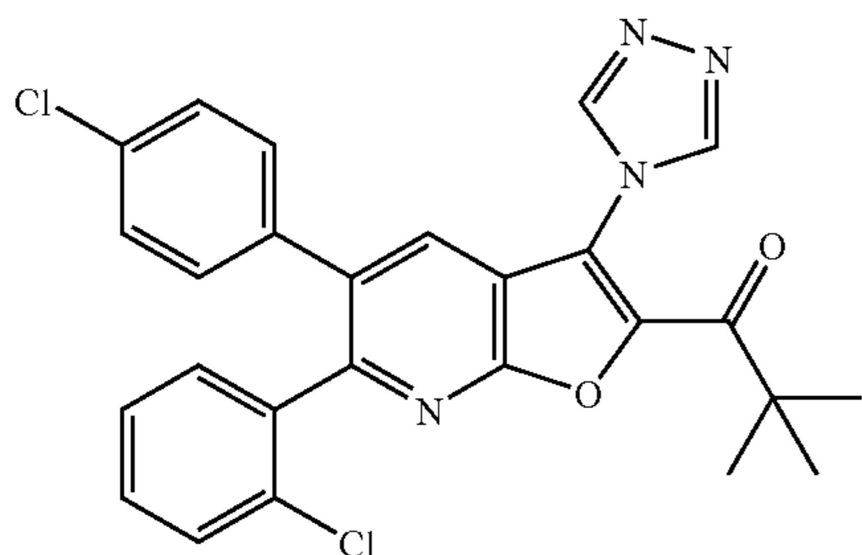
1-[6-(2-Chlorophenyl)-5-(4-chlorophenyl)-3-(4H-1,2,4-triazol-4-yl)furo[2,3-b]pyridin-2-yl]-2,2-dimethylpropan-1-one
