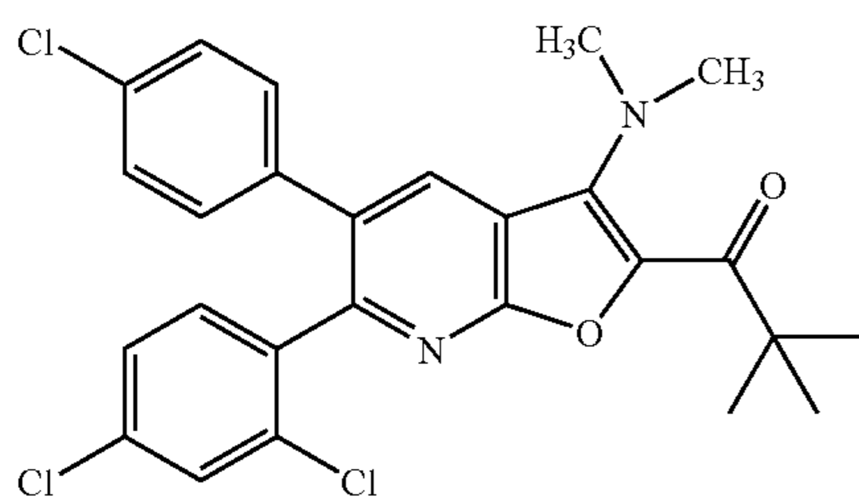
1-[5-(4-Chlorophenyl)-6-(2,4-dichlorophenyl)-3-(dimethylamino)furo[2,3-b]pyridin-2-yl]-2,2-dimethylpropan-1-one
