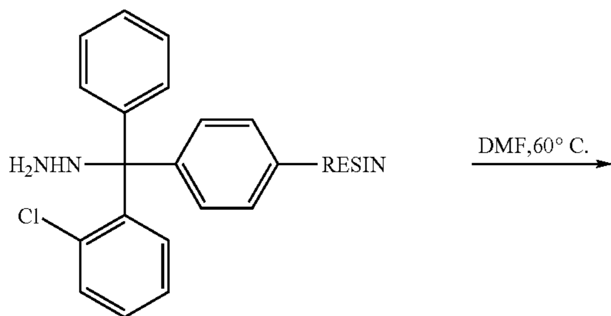
Hydrazine-2-chlorotriptyl resin
