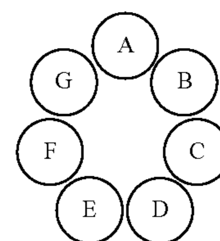
\beta -cyclodextrin
