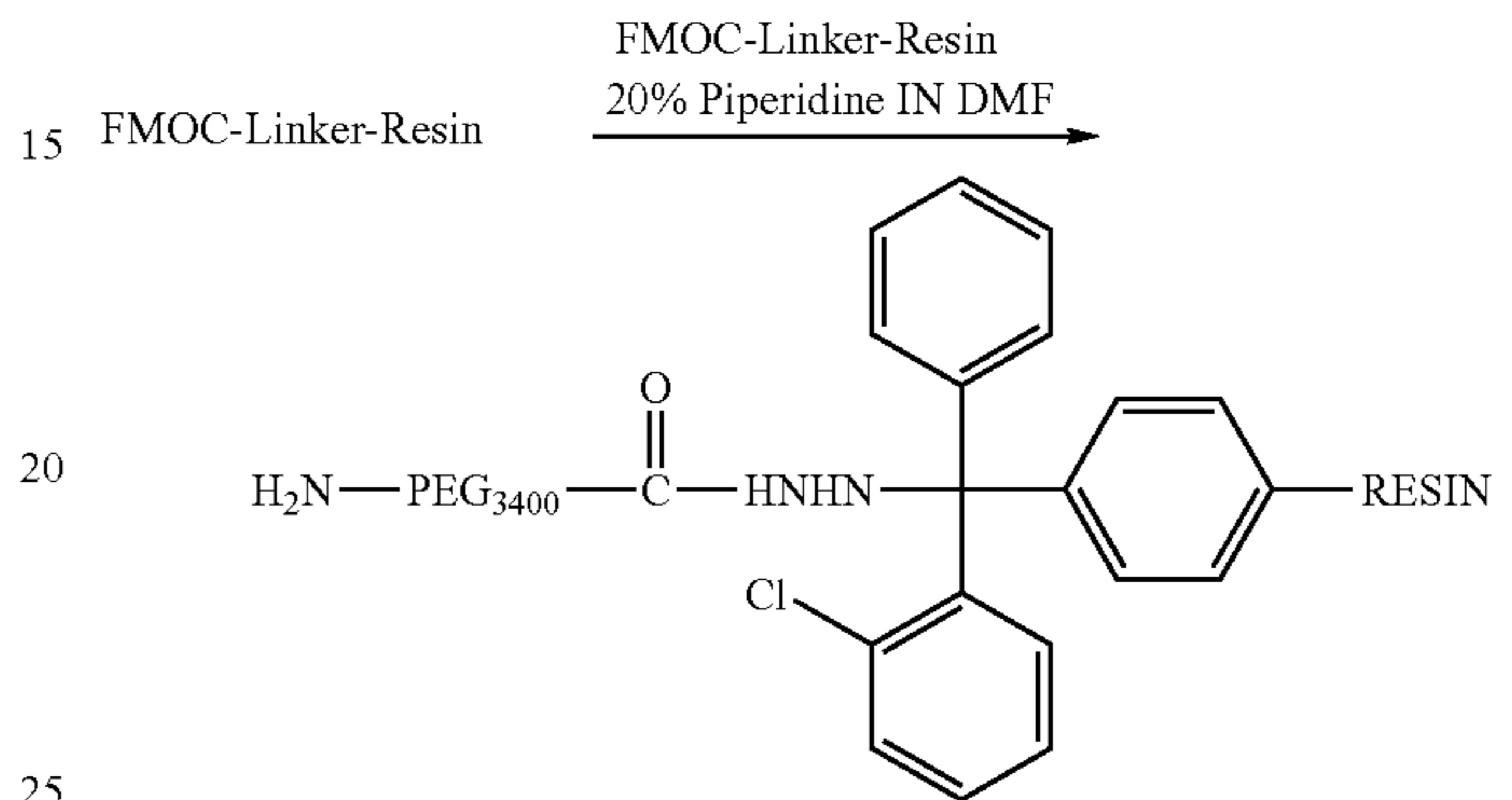
Linker-Resin
