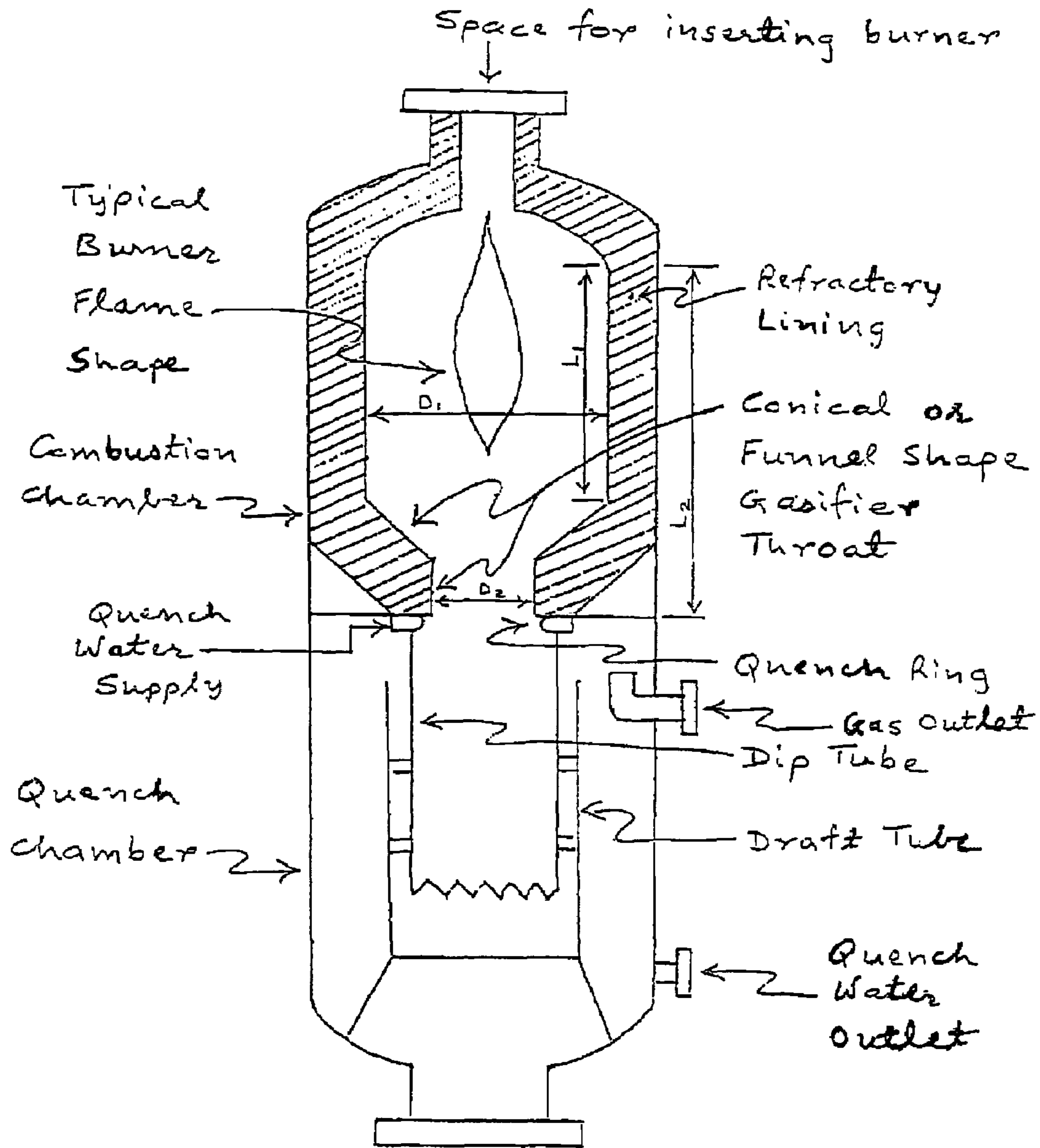
Figure 1 (Prior Art)
