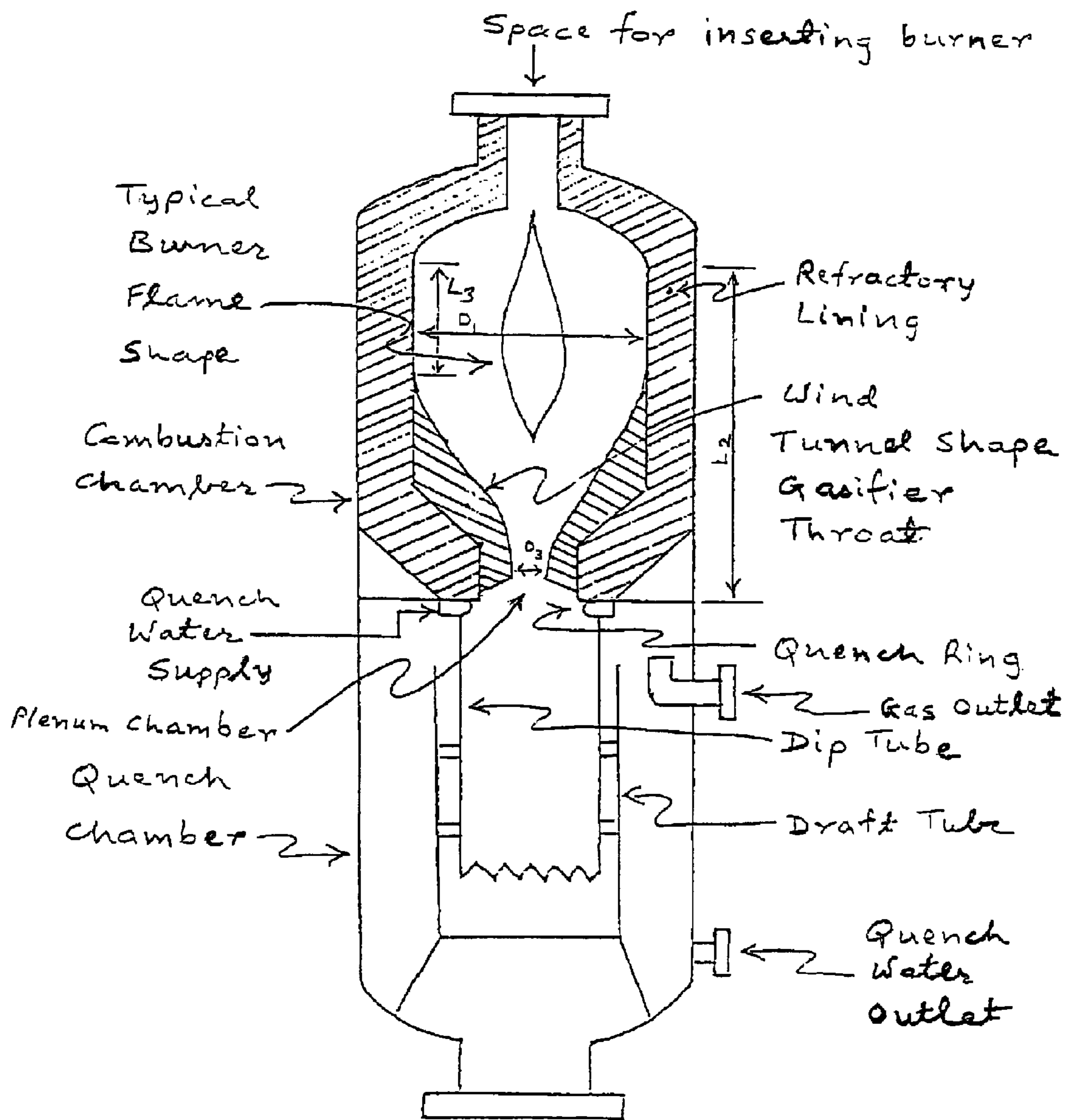
Figure 2 (Prior Art)
