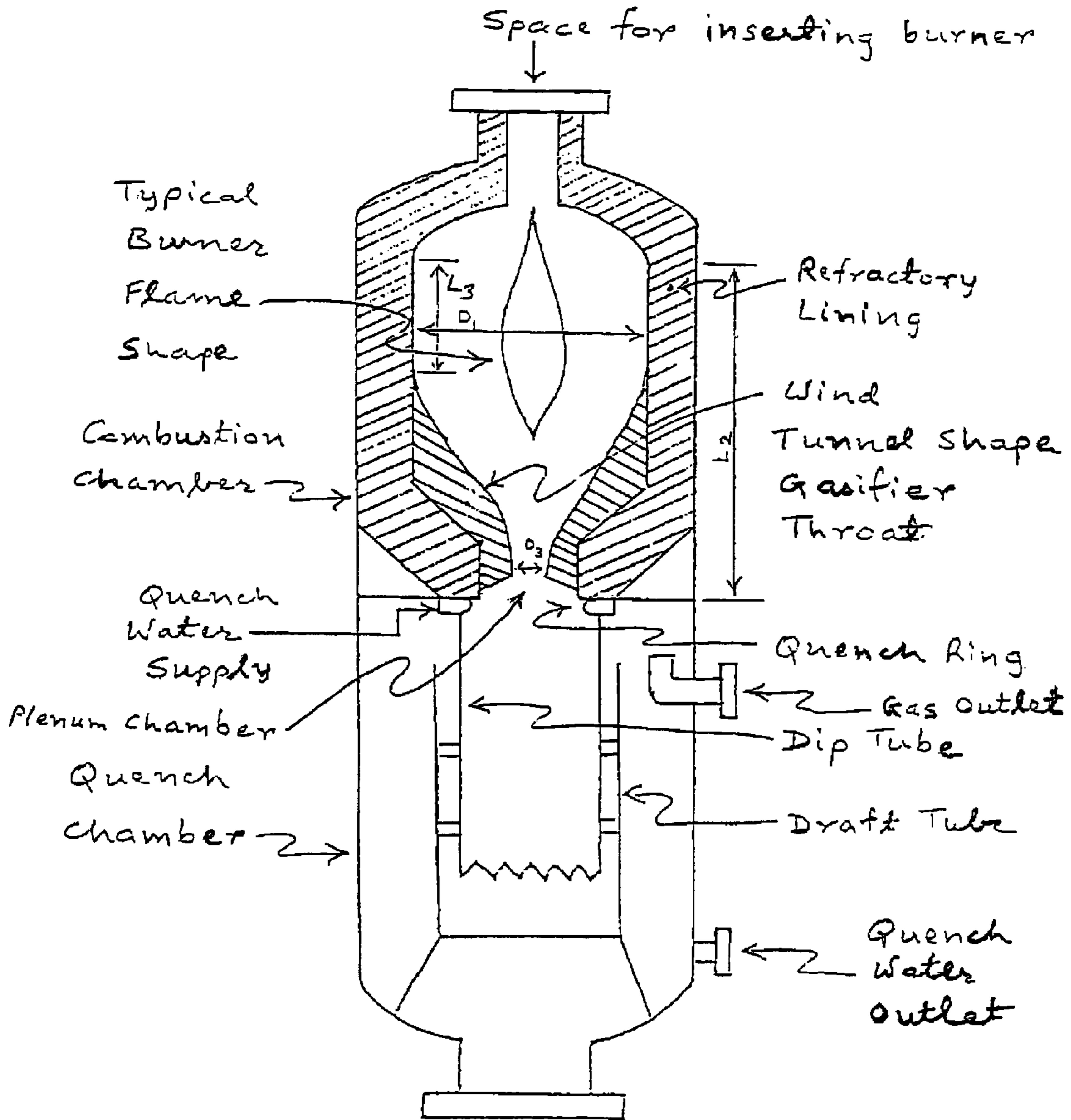
Figure 2 (Prior Art)
