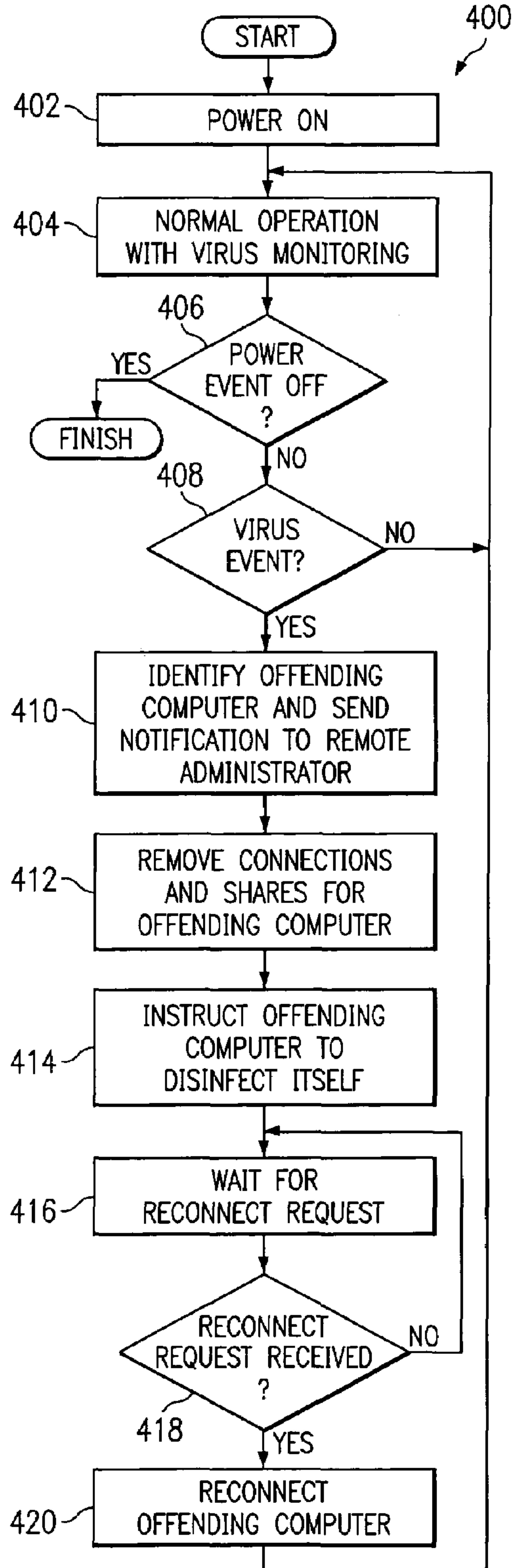
FIG. 4 SERVER OPERATION
