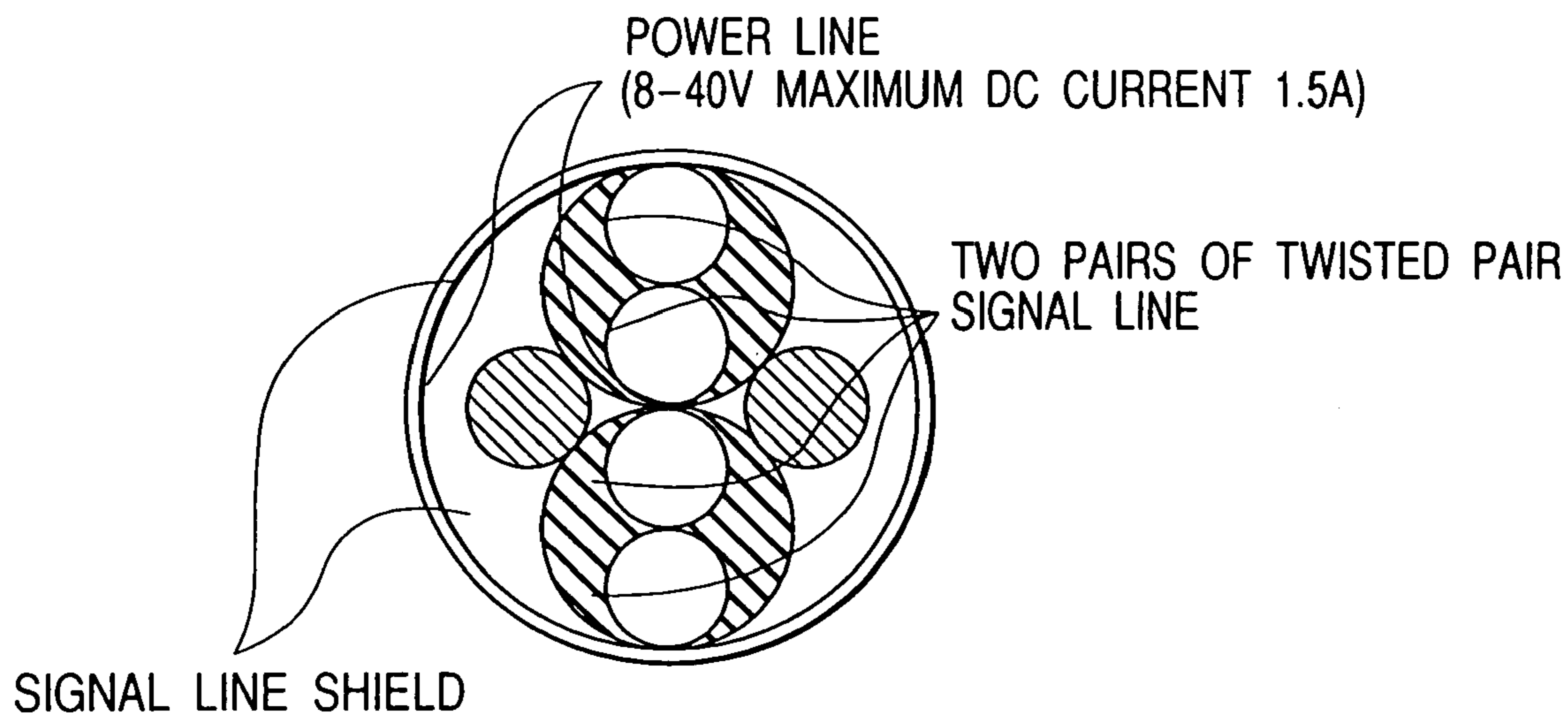
(CABLE CROSS SECTION DIAGRAM)
