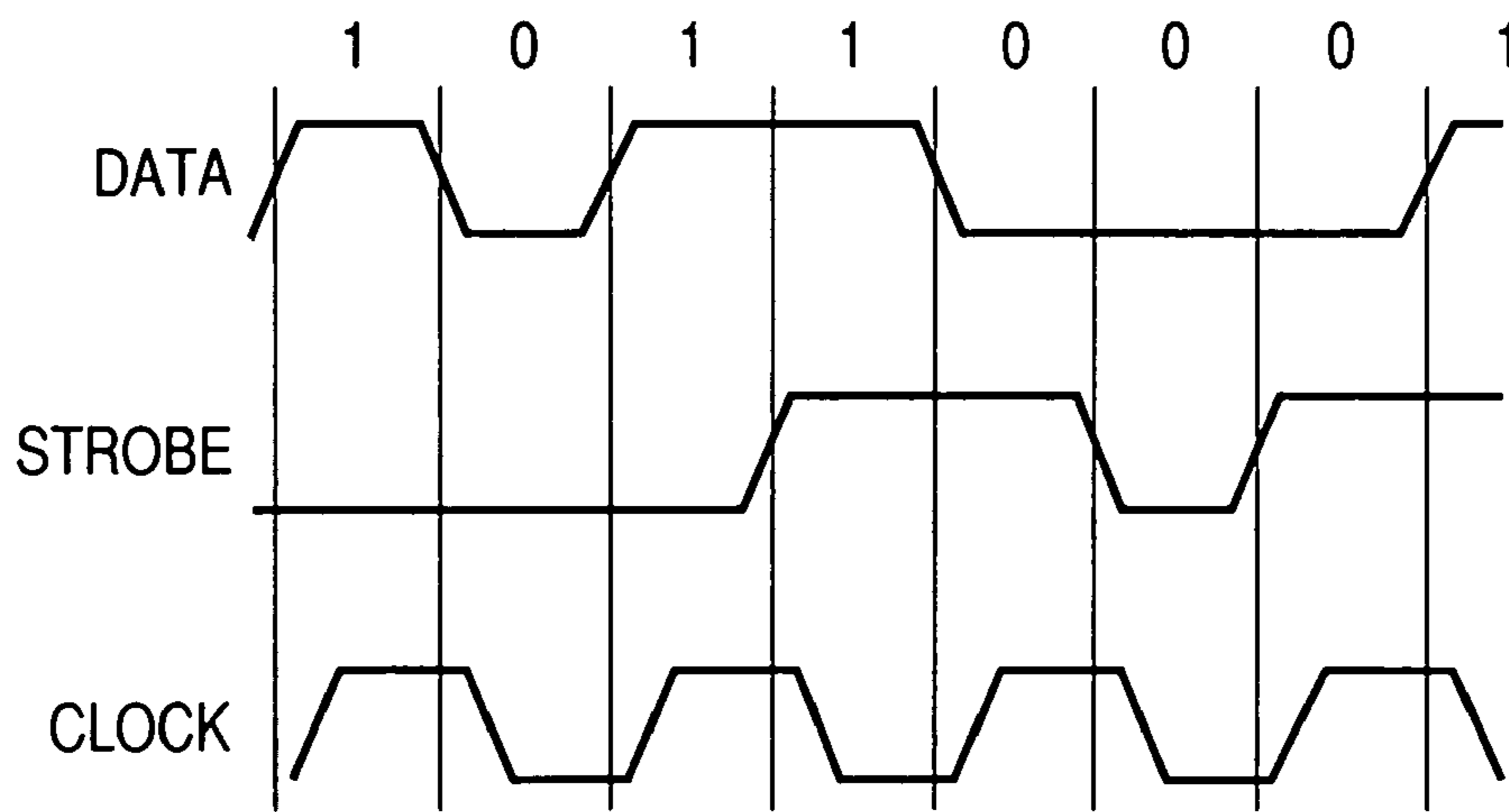
(EXCLUSIVE OR SIGNAL OF DATA AND STROBE)
