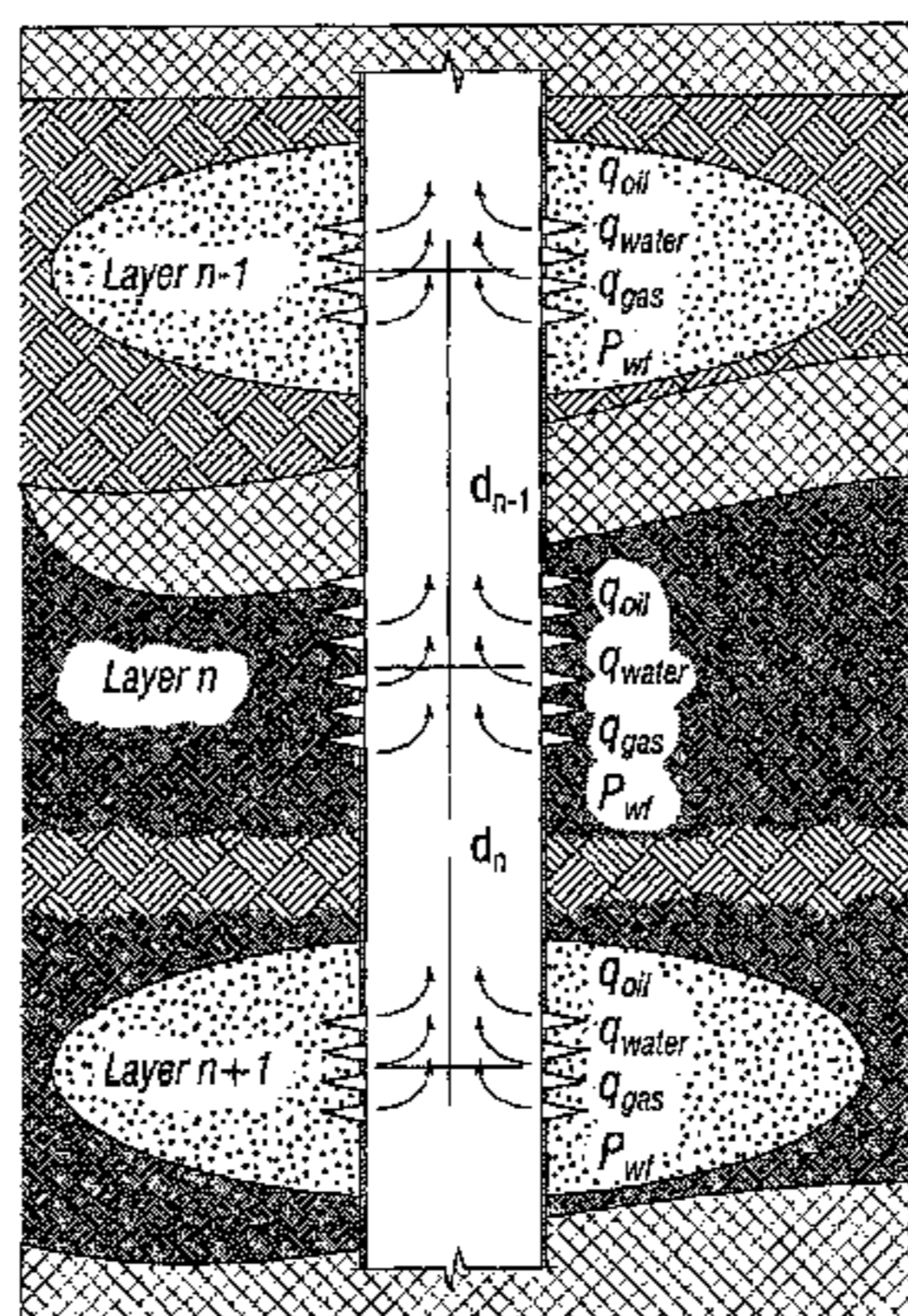
INDIVIDUAL RESERVOIR INTERVAL FLOW RATES AND WELLBORE PRESSURE TRAVERSES 10
