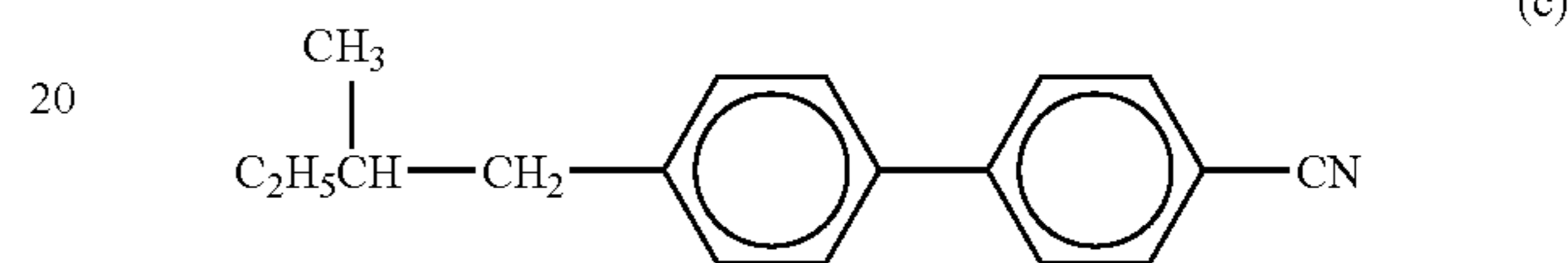
4-cyano-4'-n-pentylbiphenyl
