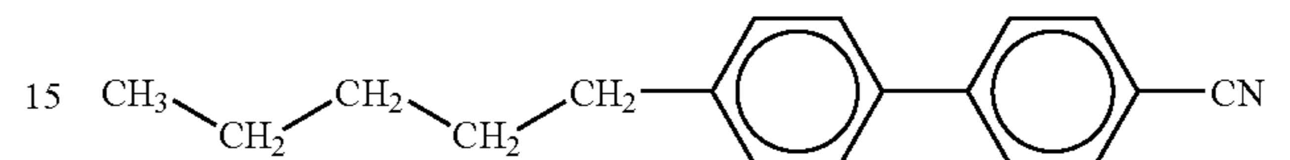
4-cyano-4'-n-pentylbiphenyl
