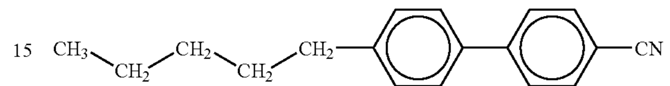
4-cyano-4'-n-pentylbiphenyl
