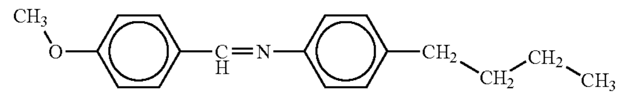
N-(4-methoxybenzylidene)-4'-n-butylaniline
