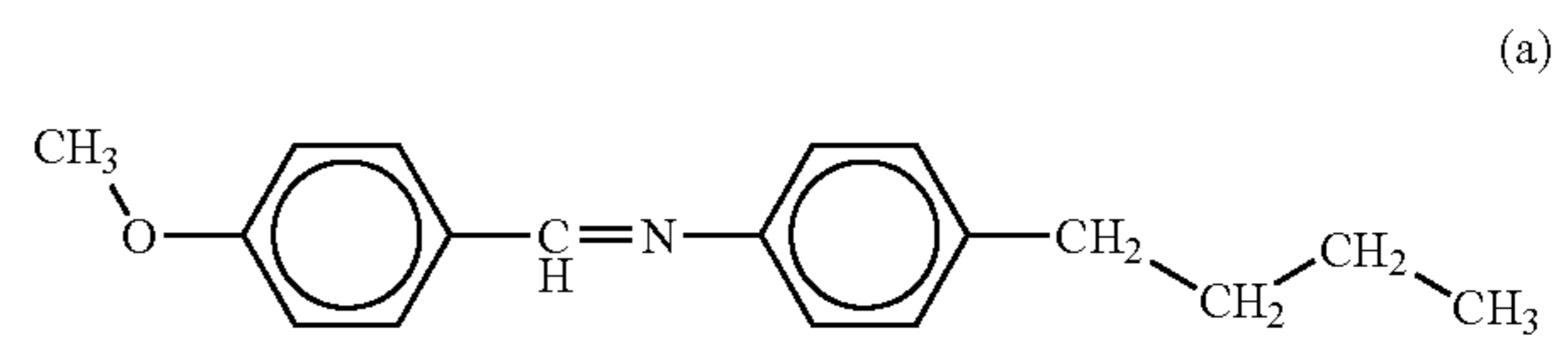
N-(4-methoxybenzylidene)-4'-n-butylaniline
