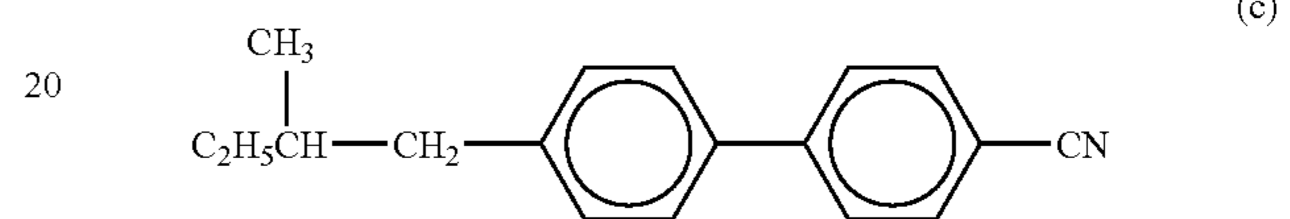
4-cyano-4'-n-pentylbiphenyl
