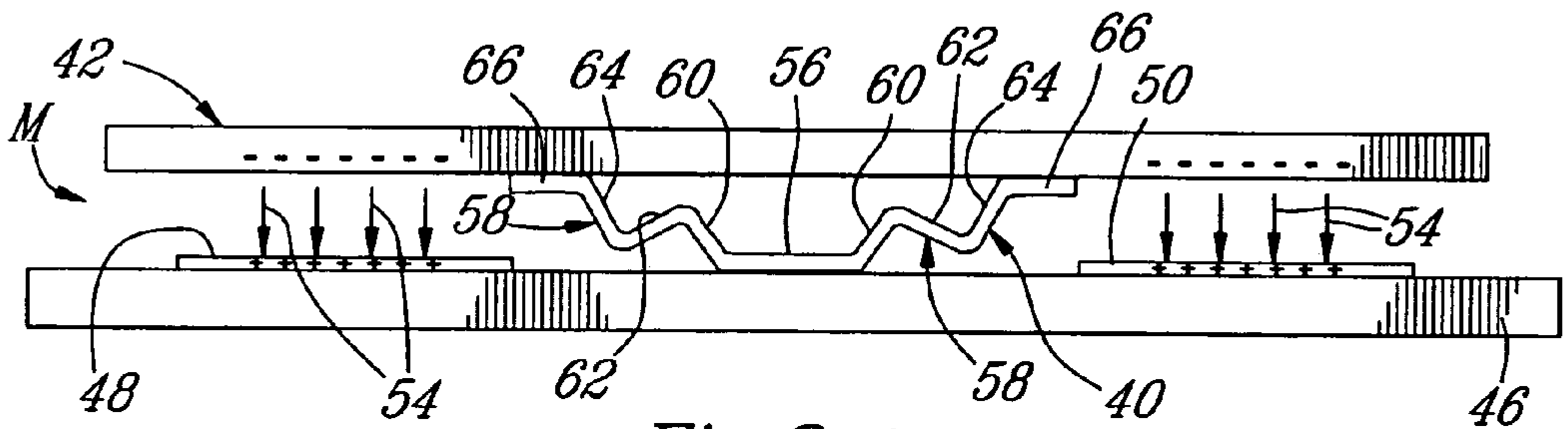
Fig. 3c (PRIOR ART)
