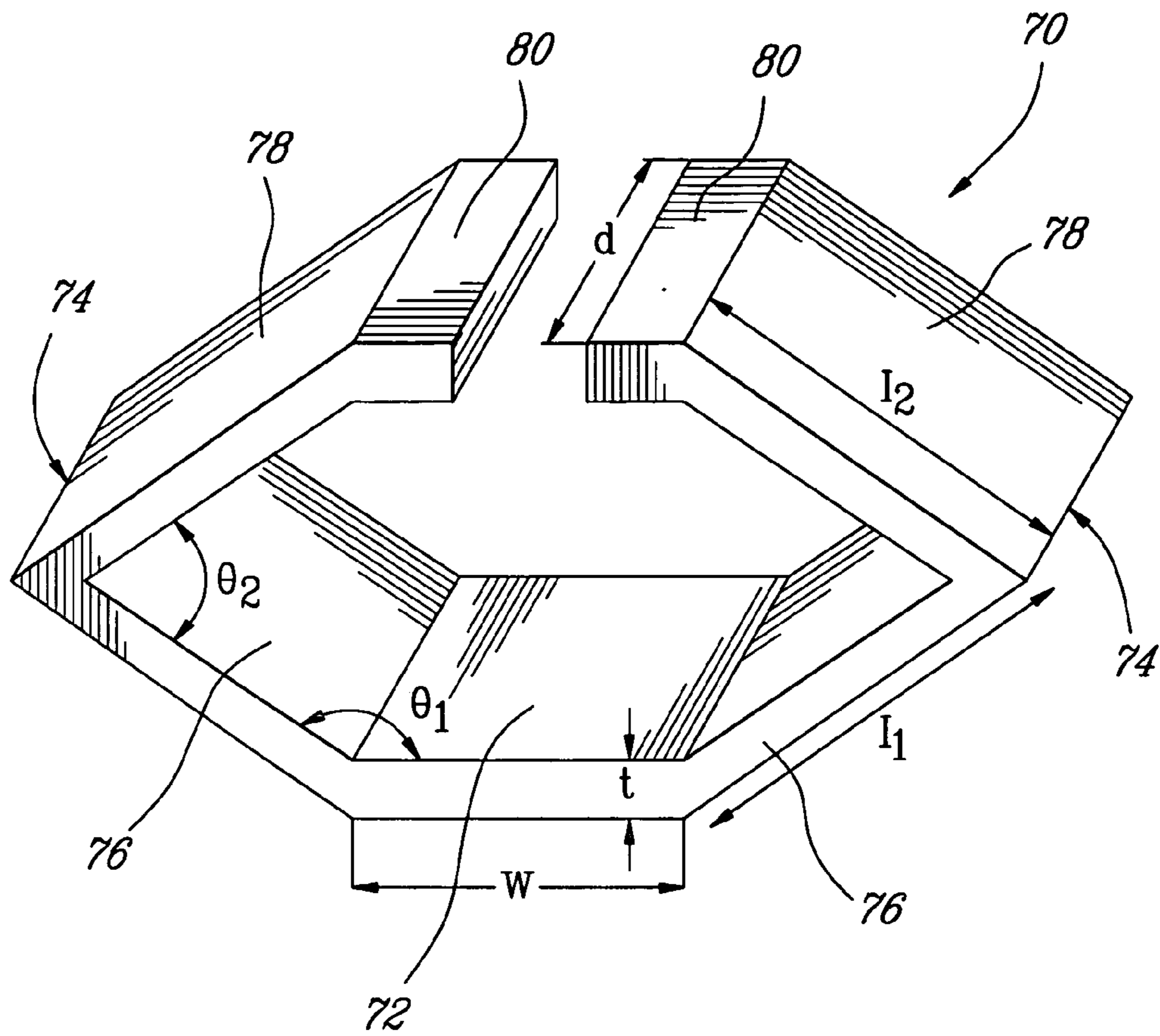
Fig. 7 (PRIOR ART)
