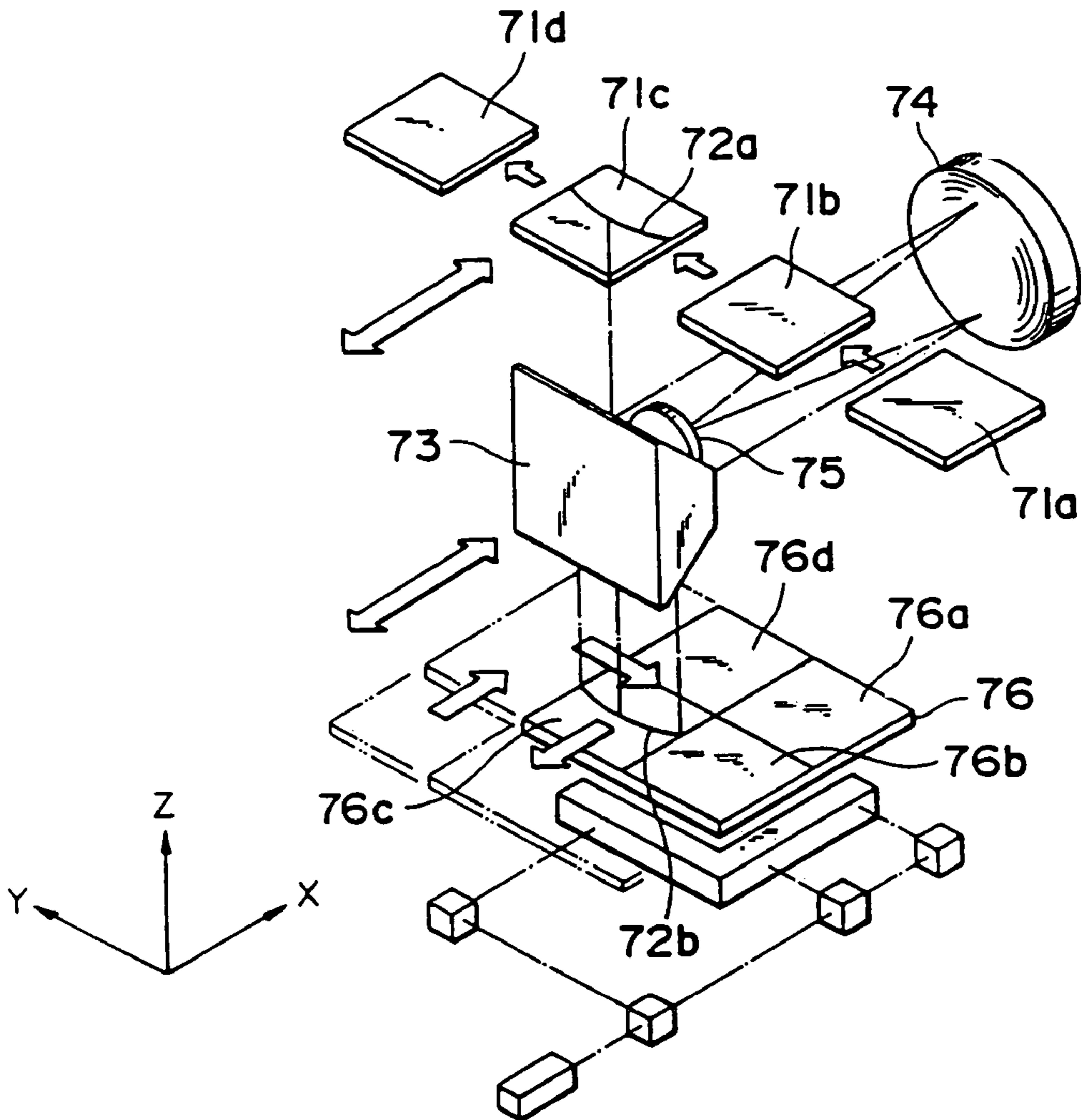
Fig. 1 PRIOR ART
