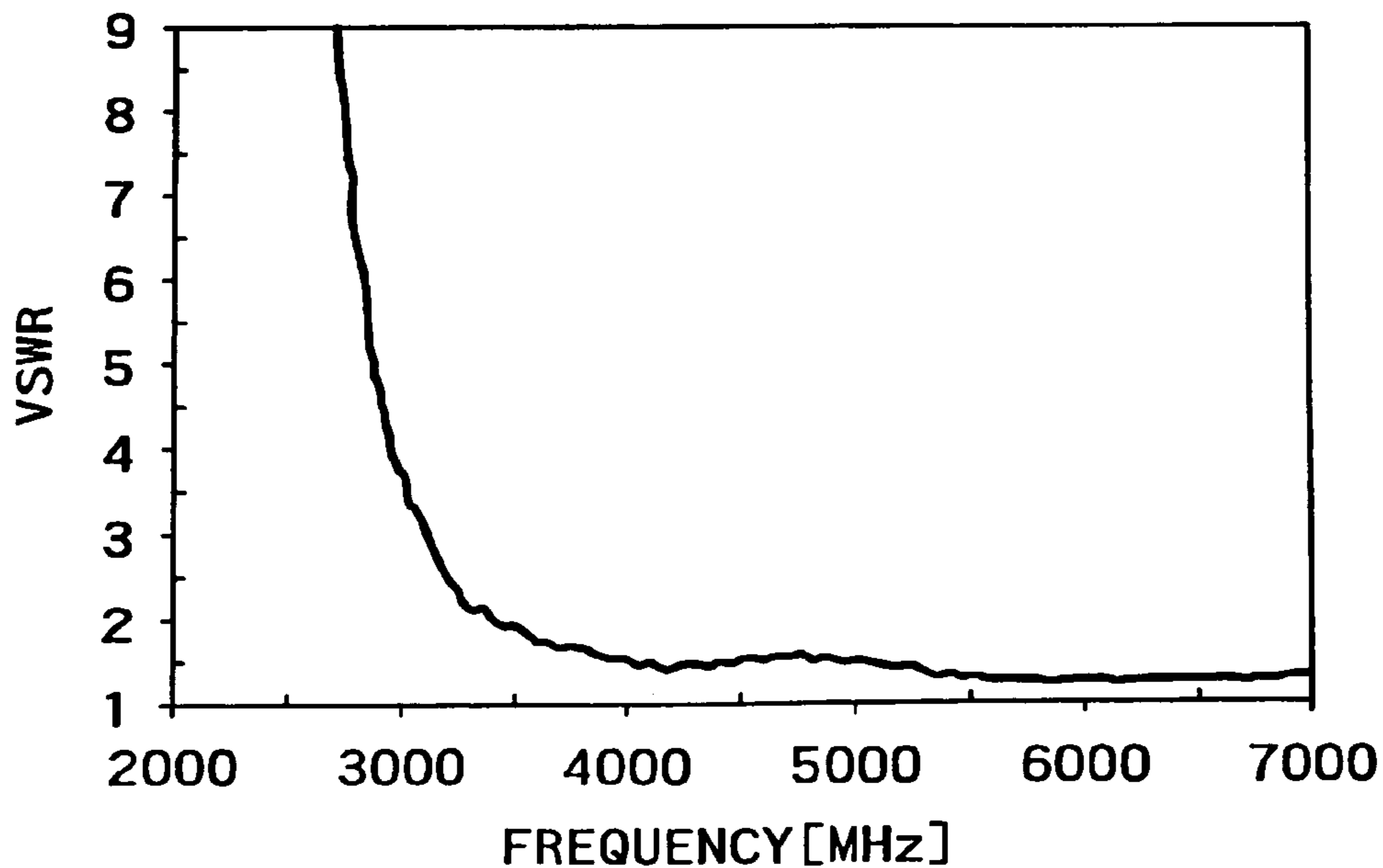
BENDED DISK MONOPOLE ANTENNA (h=23.5mm)
