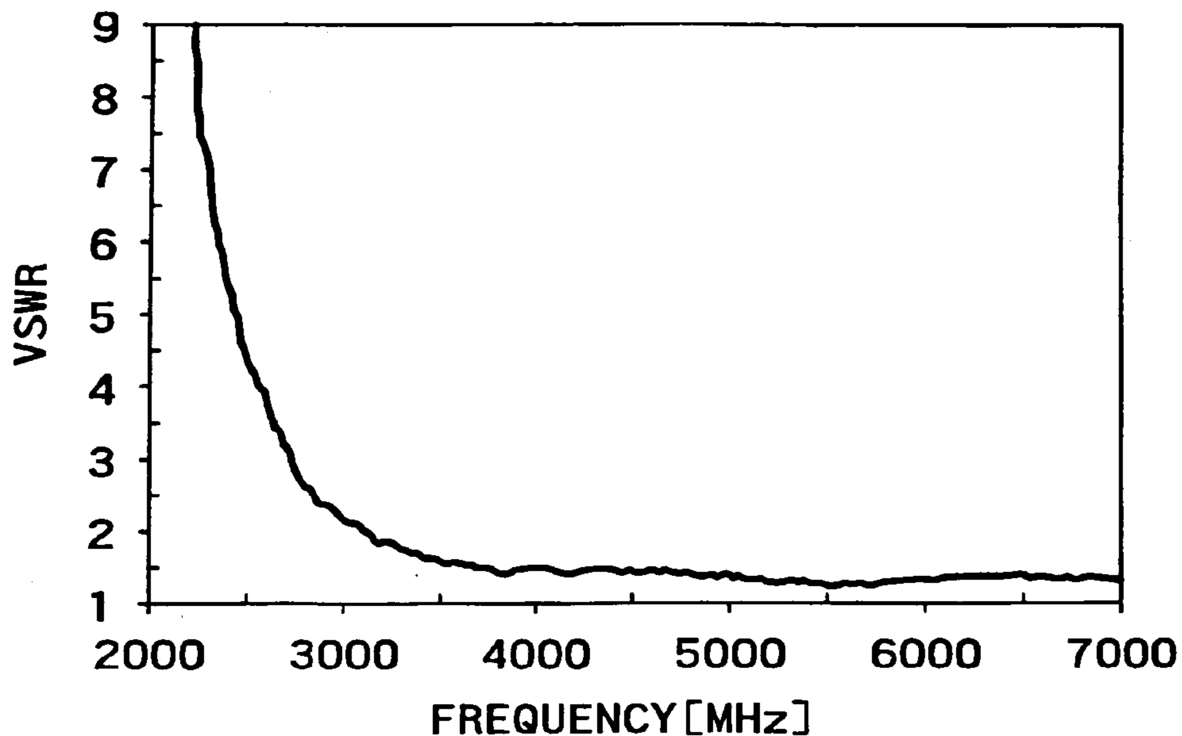
DISK MONOPOLE ANTENNA (h=23.5mm)
