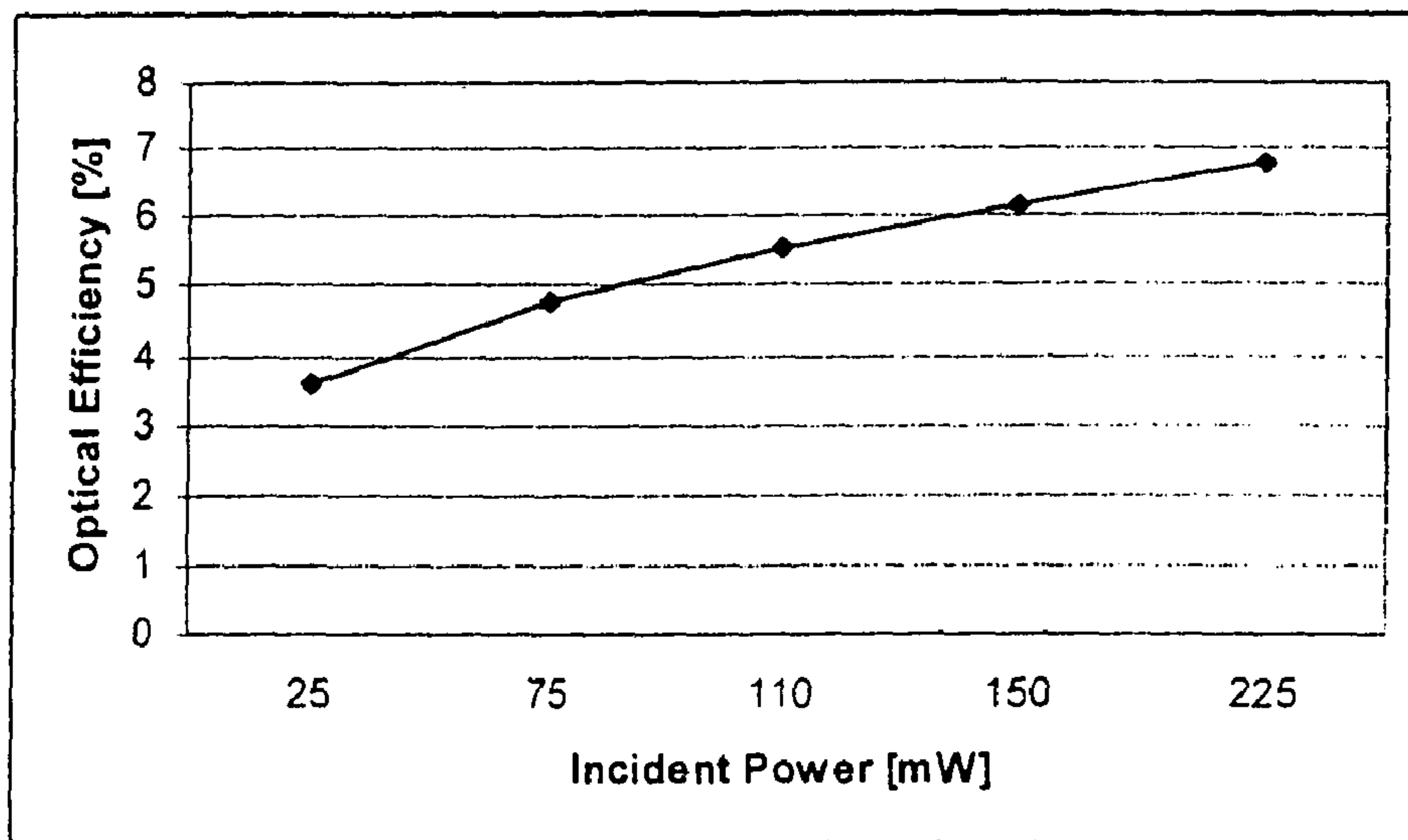
Figure 8. Optical efficiency of the YF_3:Yb,Er material scaled to the absorbed power.
