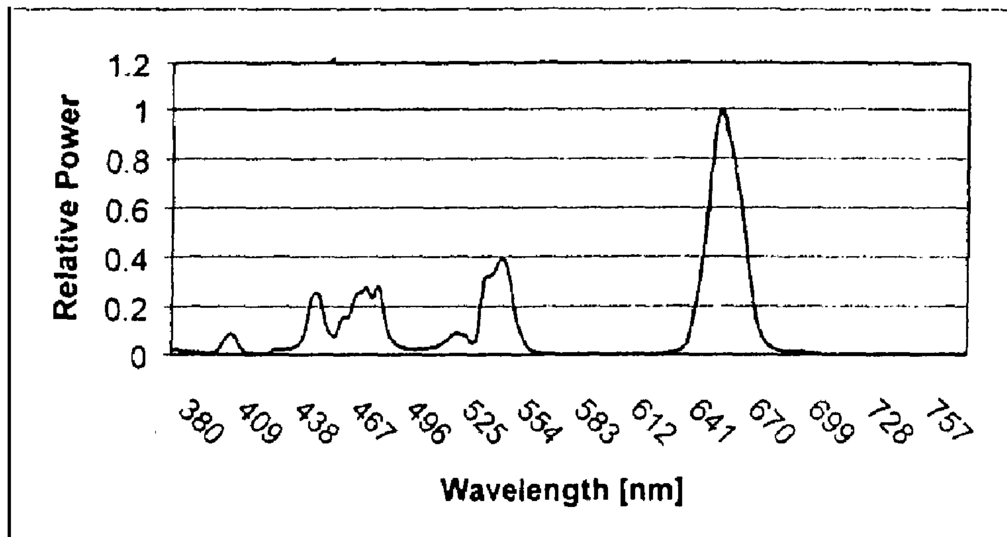
Figure 7. Additive mixture of emissions from YF_3:Yb,Er and LiYF_4:Th,Yb .
