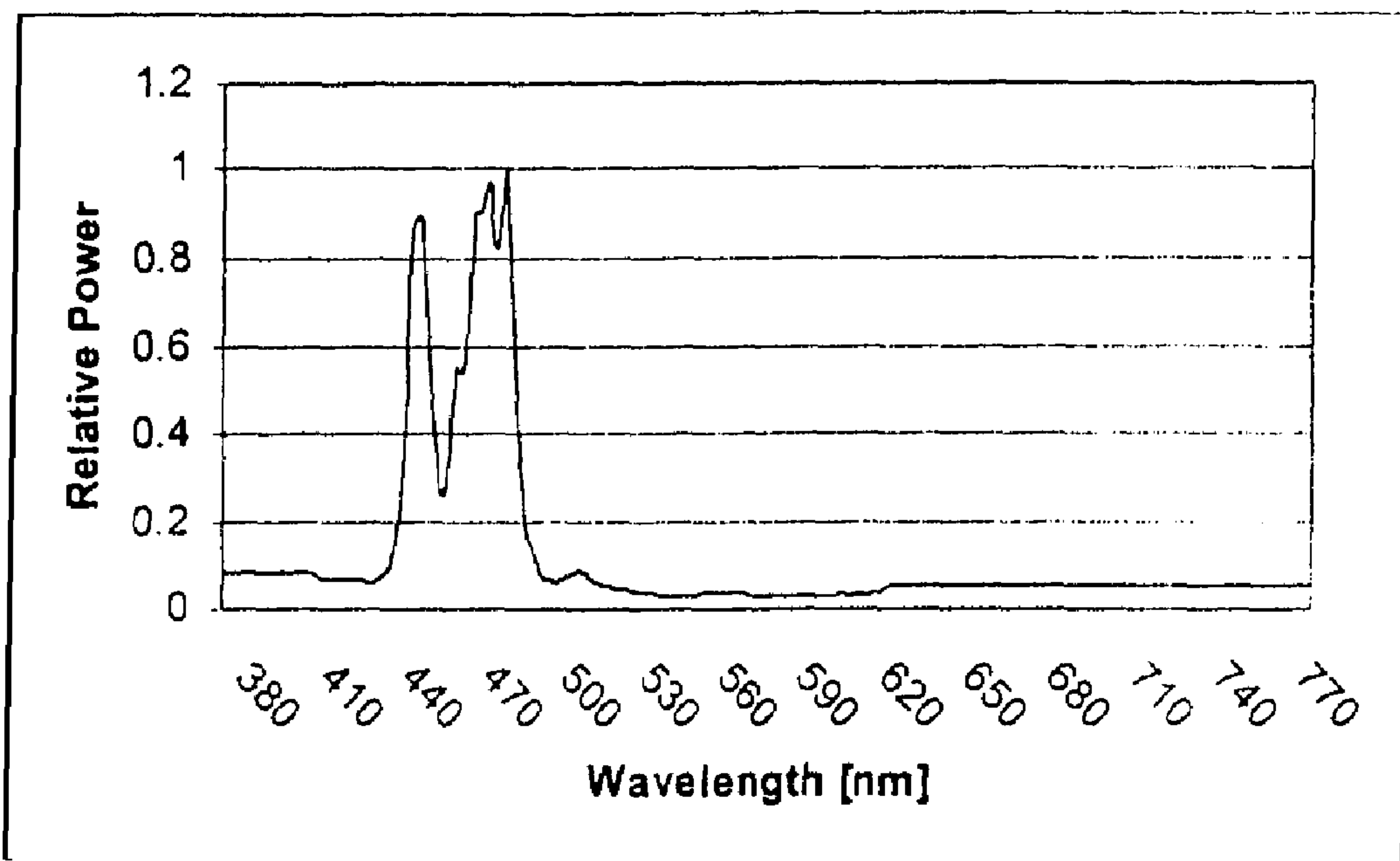
Figure 6. Emission from LiYF 4 : Th, Yb with continuous 980 pump.
