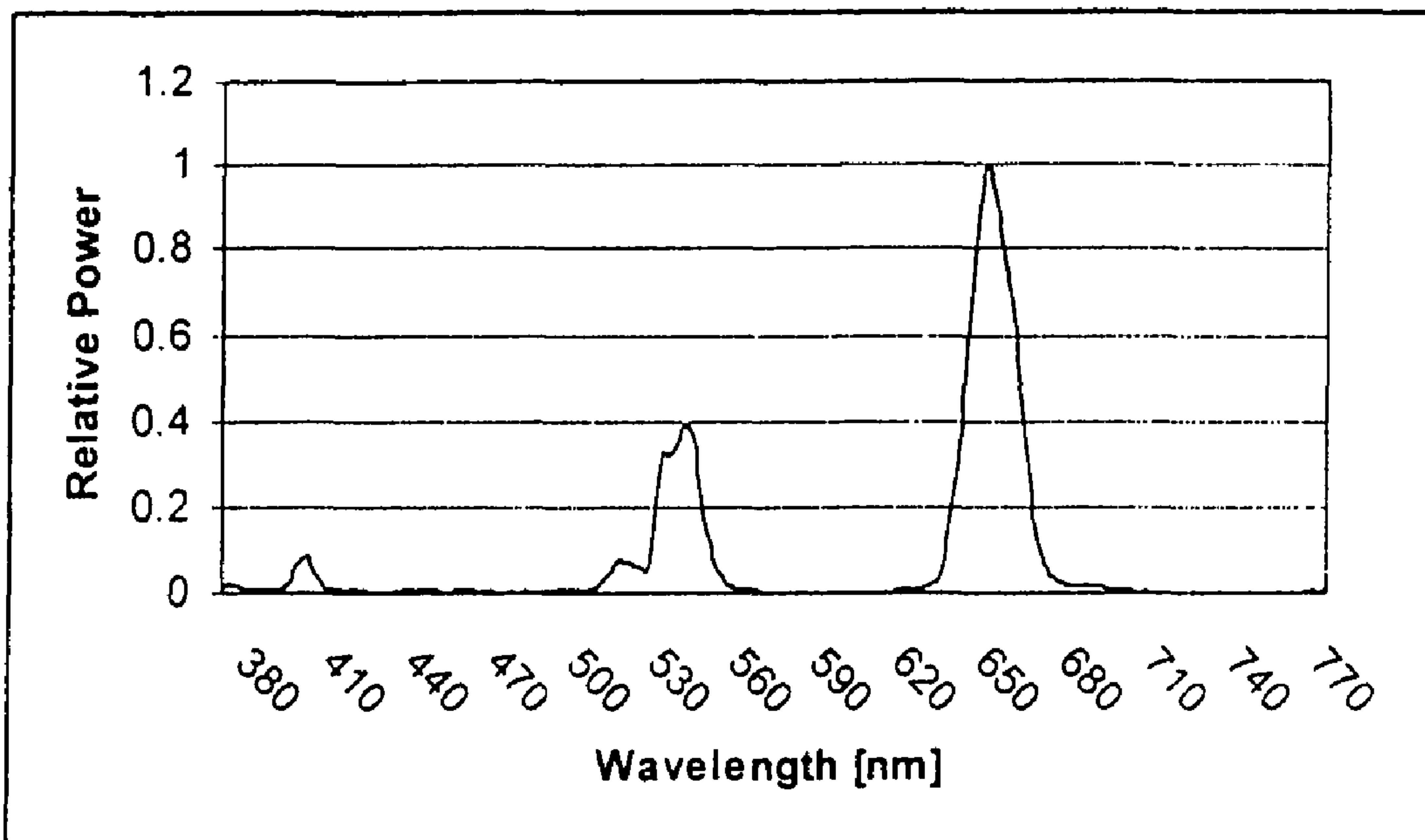
Figure 5. Emission from YF 3 :Yb,Er with continuous 980nm pump.
