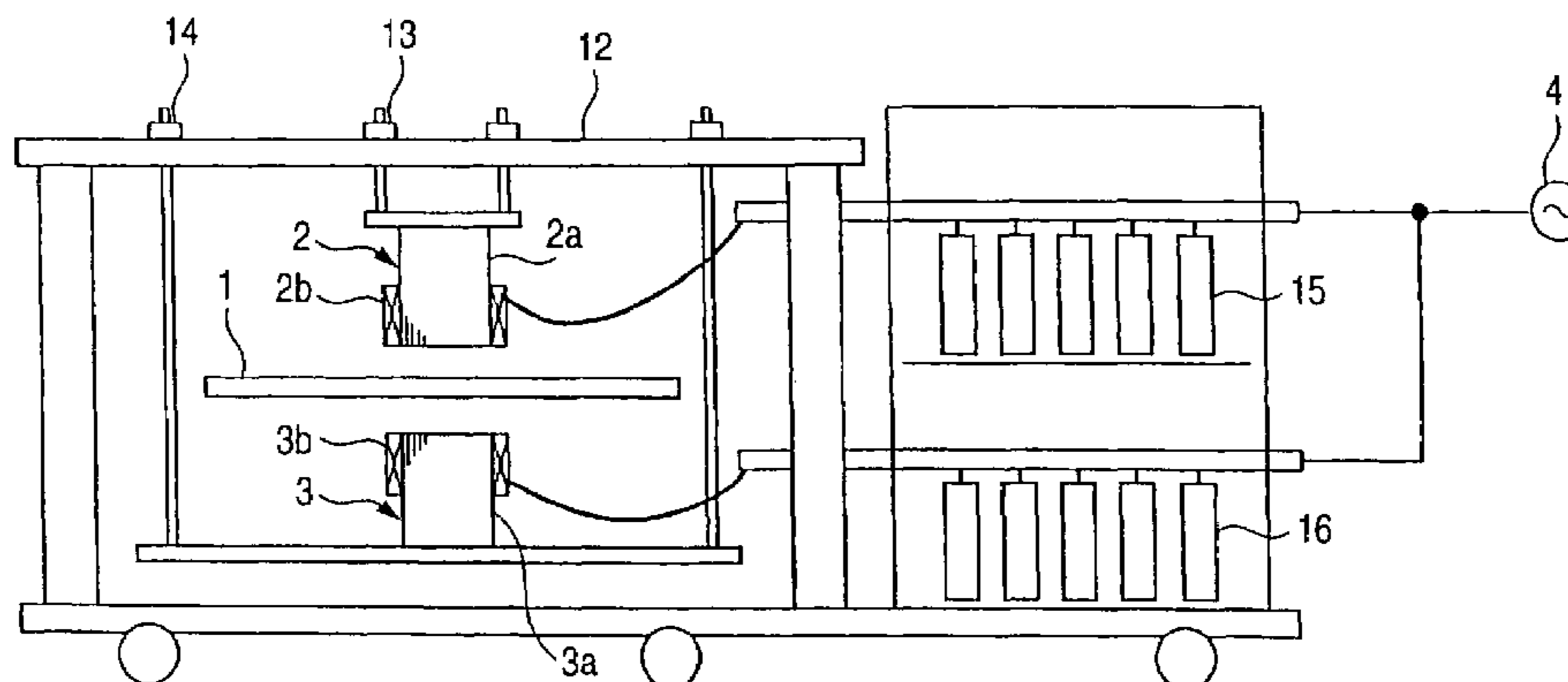
12,13 : LIFTING AND LOWERING MEANS
