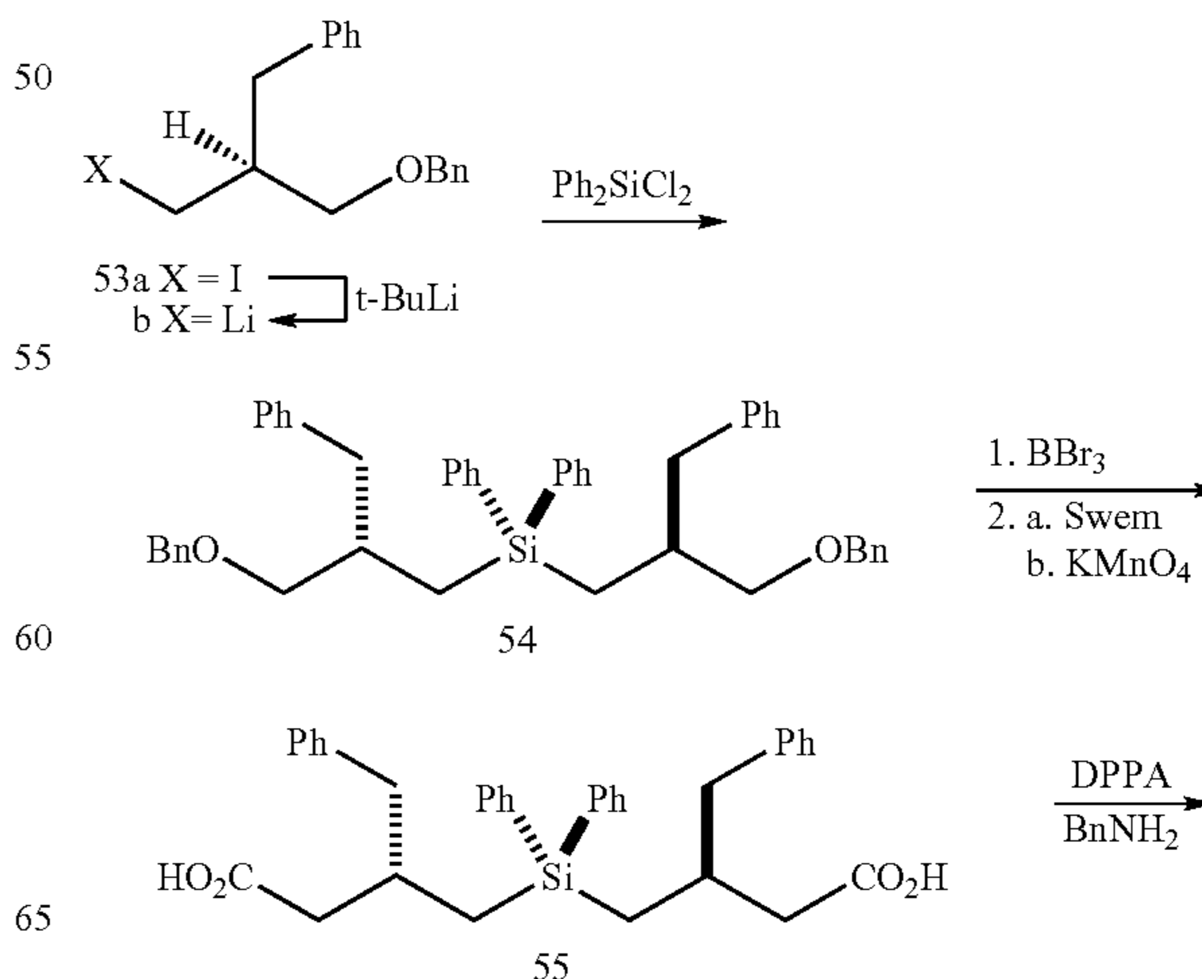
Scheme 9 Synthesis of Dibenzyloxy-2-(S)-6-(S)- dibenzyloxy-4,4-dihydroxy-4-silaheptanediamide (9a)
