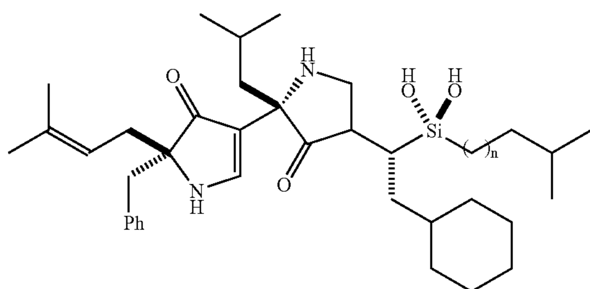
n = 0 6-Cyclohexyl-4,4-dihydroxy-3-(R)-[5'-(S)-5' isobutyl-5-[5''-(S)-5''-(3-methyl-2-butenyl)-5''-benzyl 3''-pyrrolin-4'' one]-3'-pyrrolin-4'-one]-4-sila-hexane
