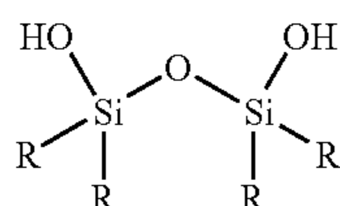
1,3-dihydroxy-1,1,3,3-tetra(3-[2-(S)-2-phenylmethylpropionyl])-disiloxane tetra(N-phenylmethylamide)
