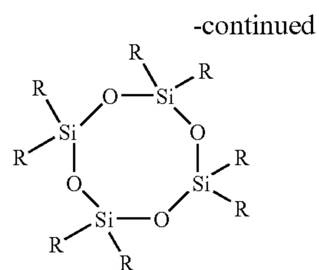
1,1,3,3,5,5,7,7-octa(3-[2-(S)-2-phenylmethylpropionyl])-cyclotetrasiloxane octa(N-phenylmethylamide)
