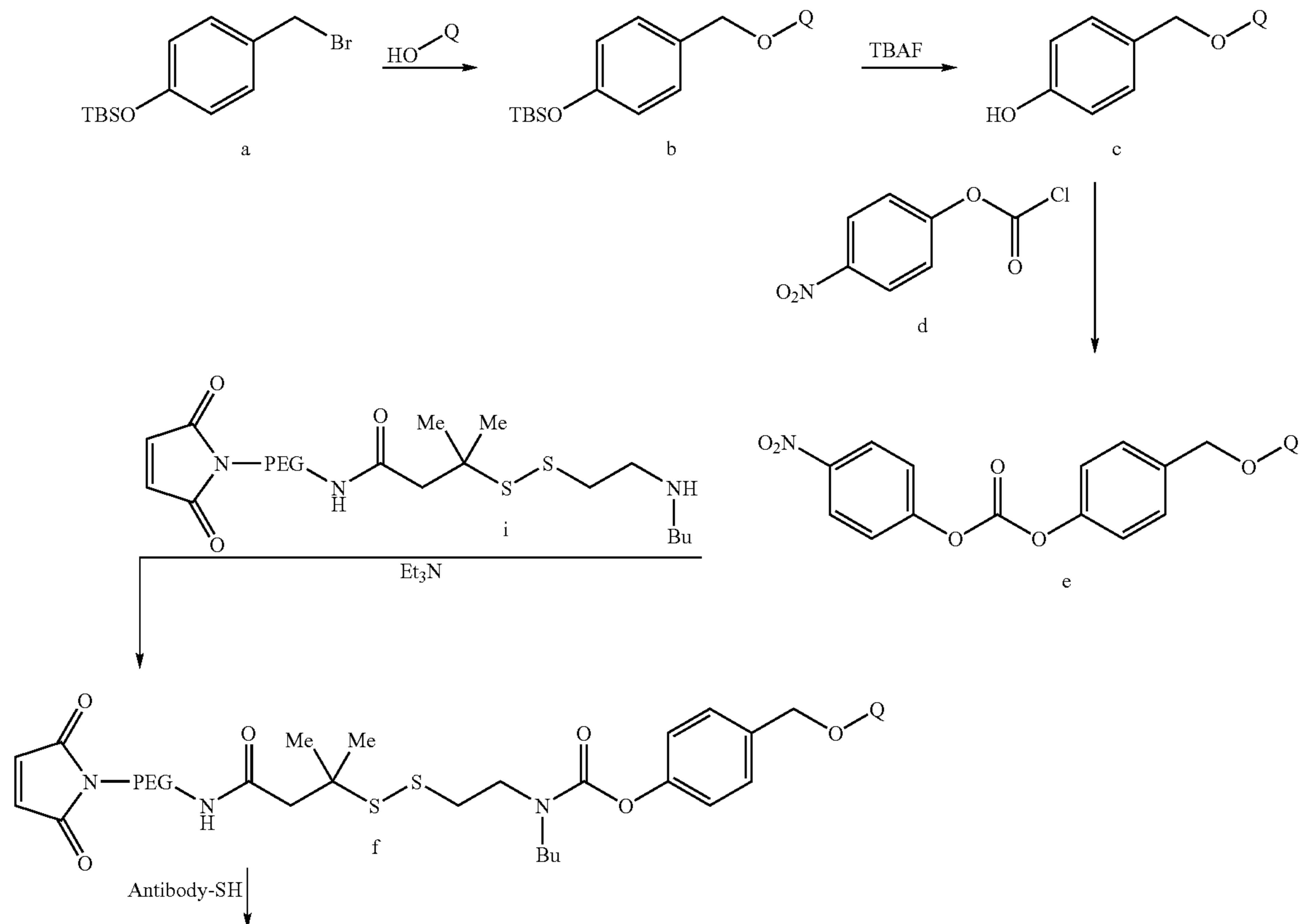
Scheme 6
