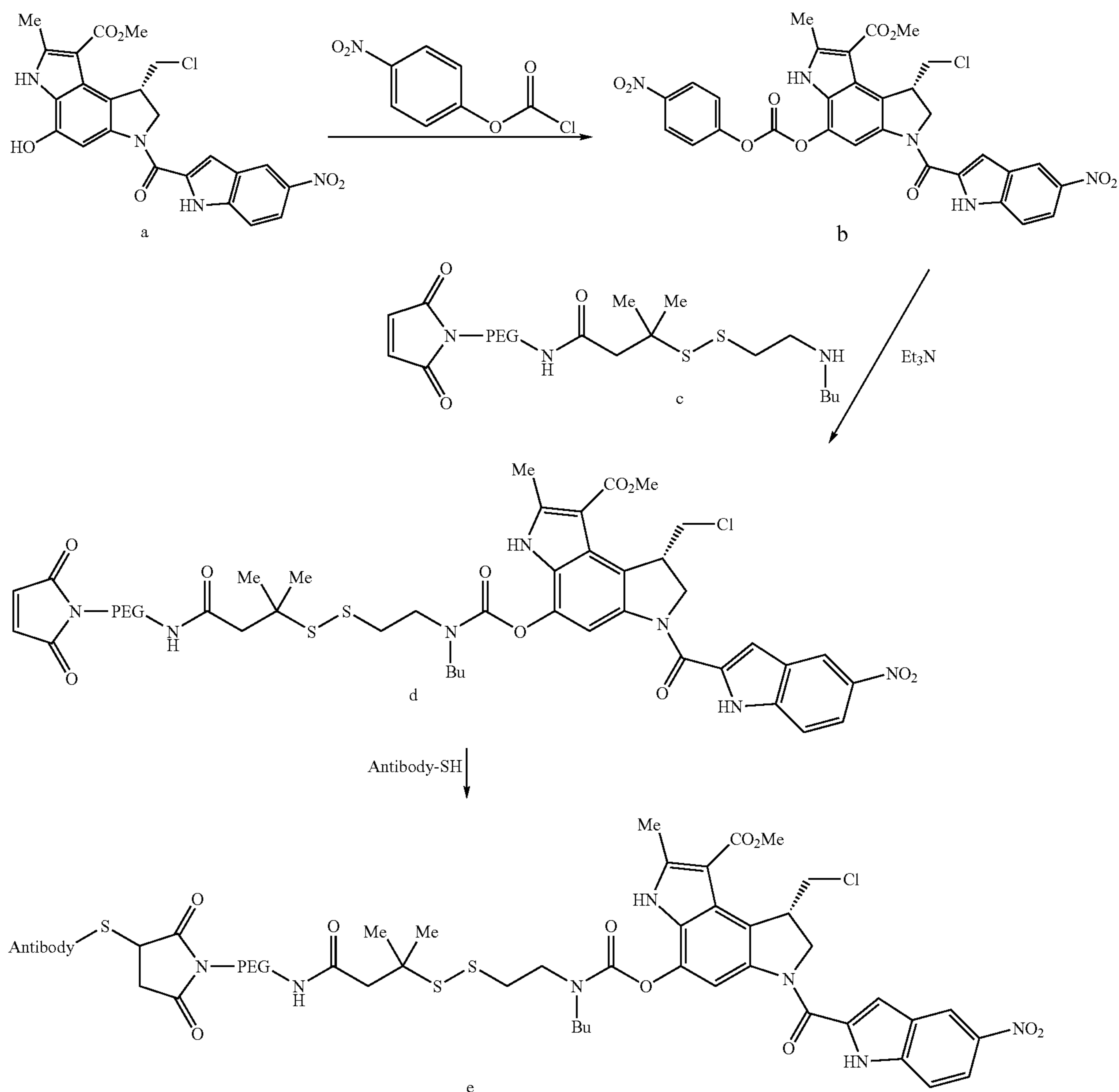
Scheme 7
