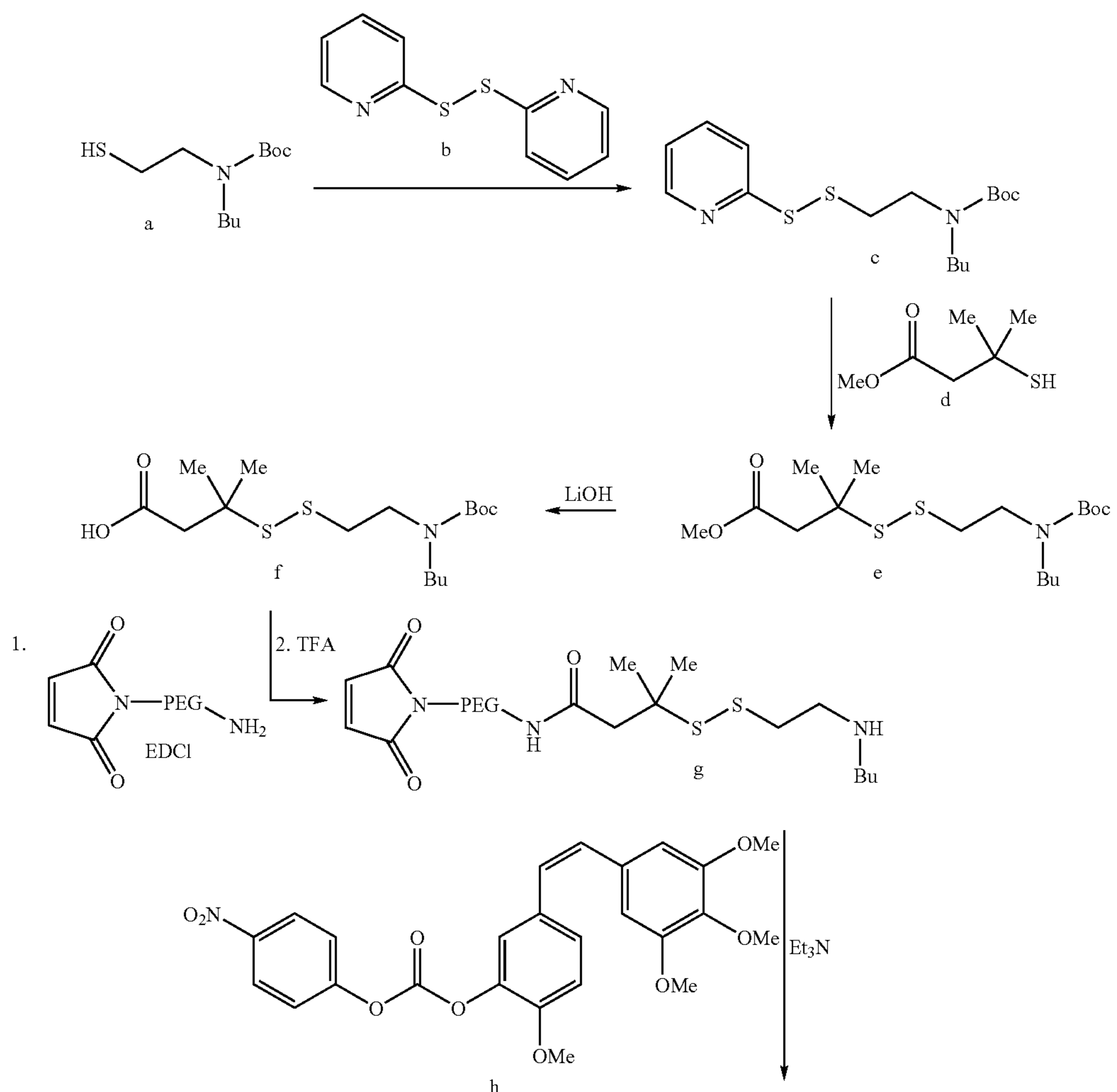
Scheme 5
