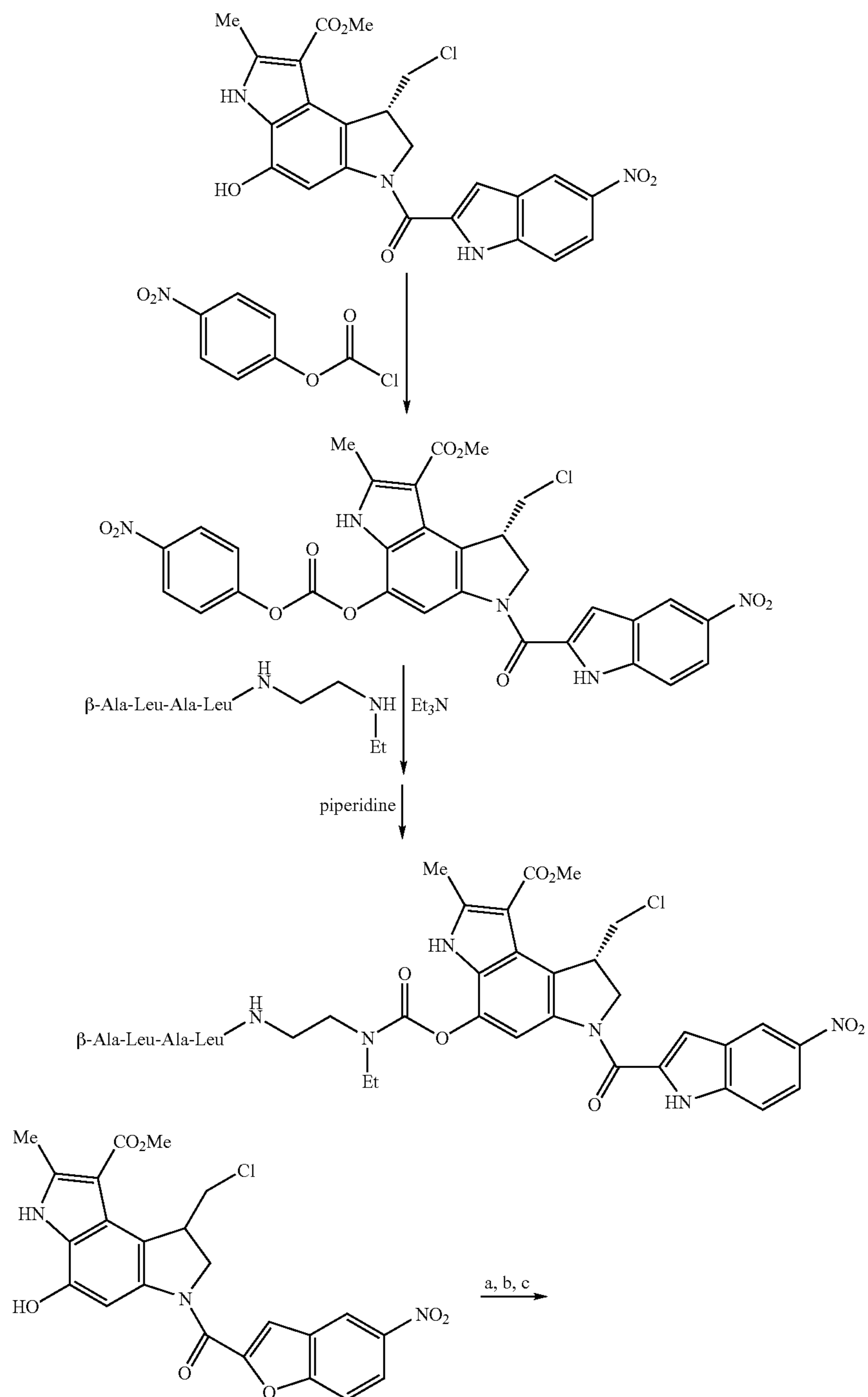
Scheme 4
