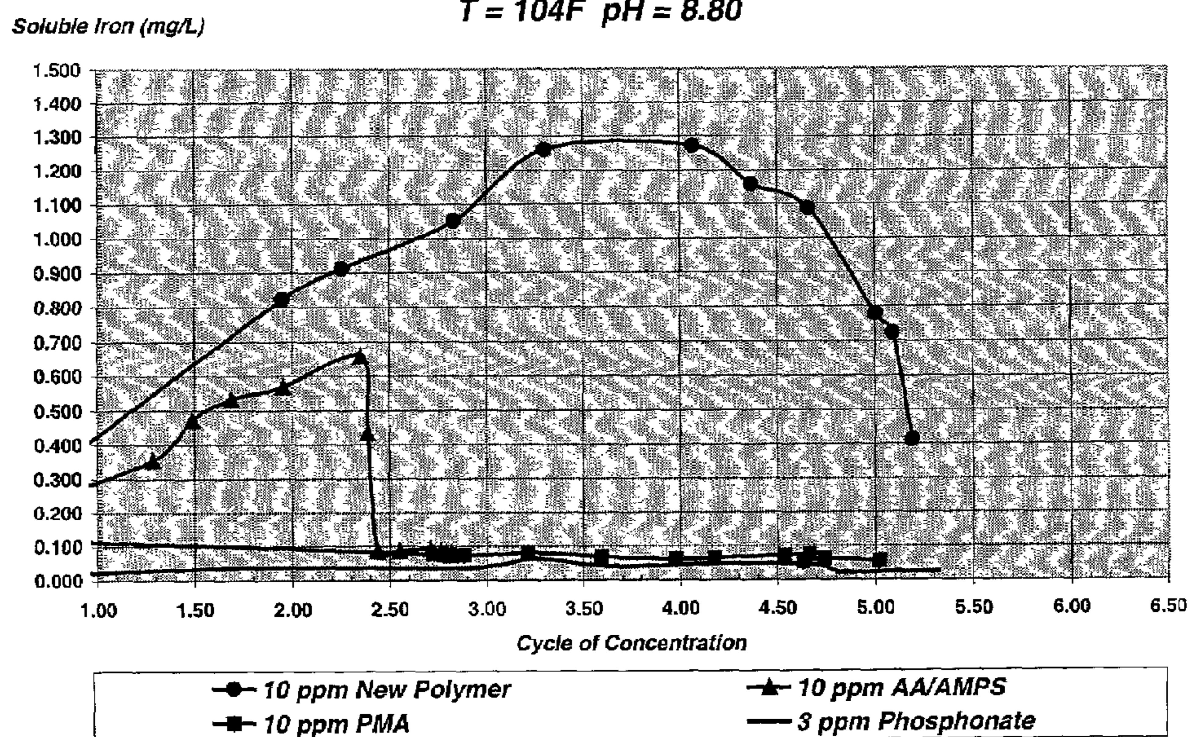
Figure 6: Soluble Iron Concentrations T = 104F pH = 8.80
