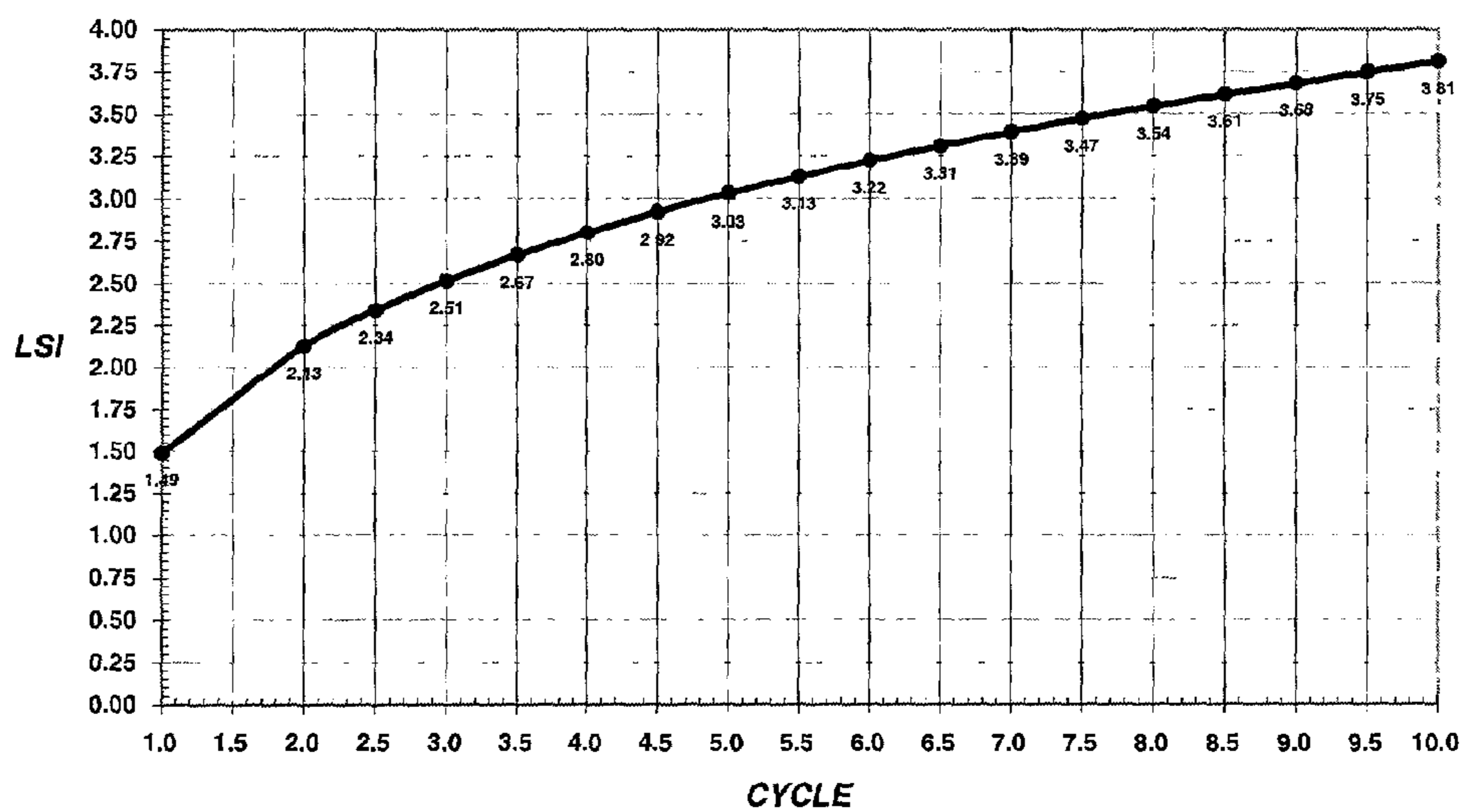
Figure 3: LSI Values Per Cycle of Concentration
