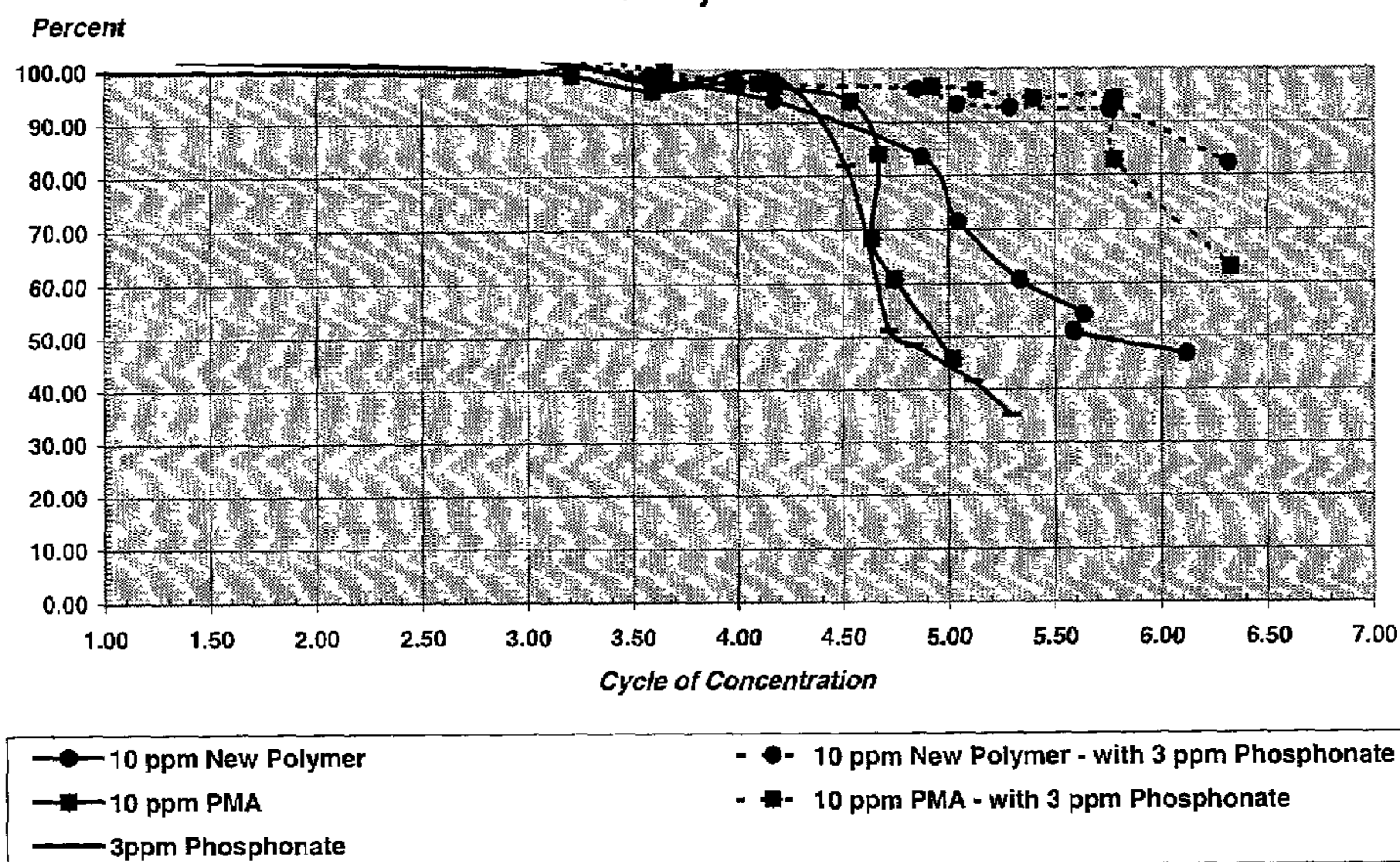
Figure 5: Calcium Threshold Inhibition T = 104F pH = 8.80
