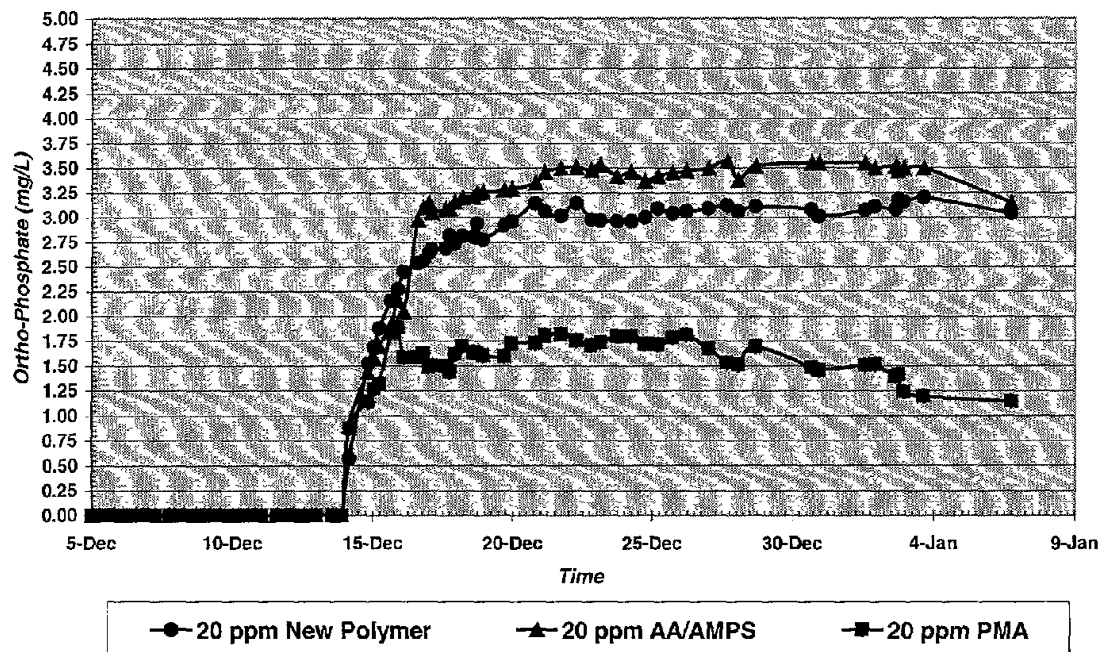
Figure 7: Achieved Ortho-Phosphate Concentrations with a 3.0 mg/L Feed
