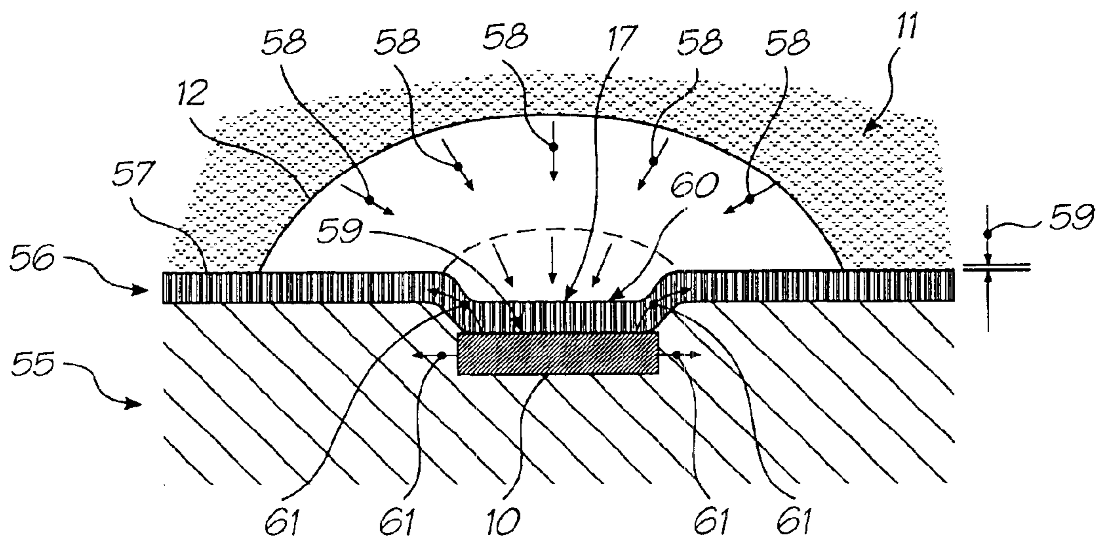
FIG. 47 (PRIOR ART)
