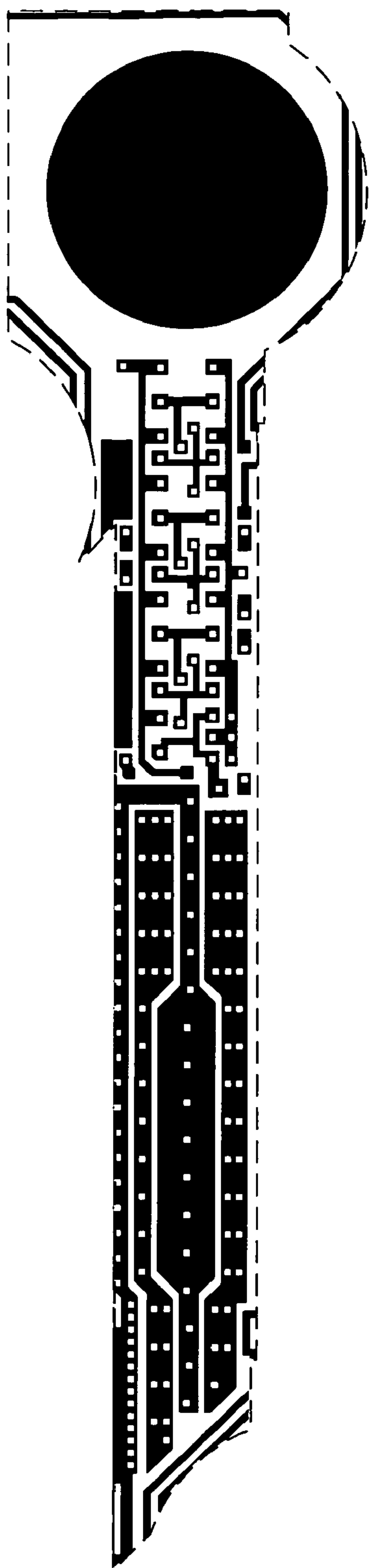
Metal 1 mask
