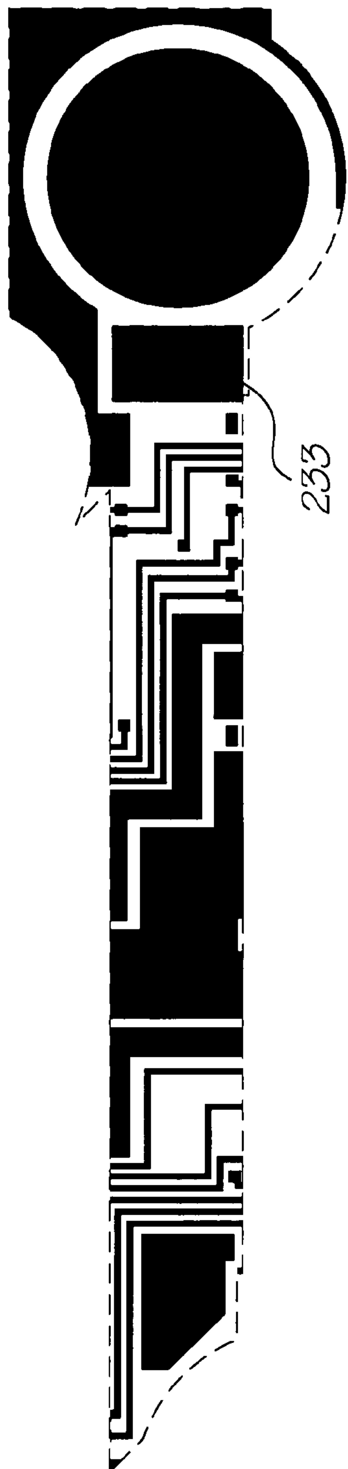
Metal 2 mask
