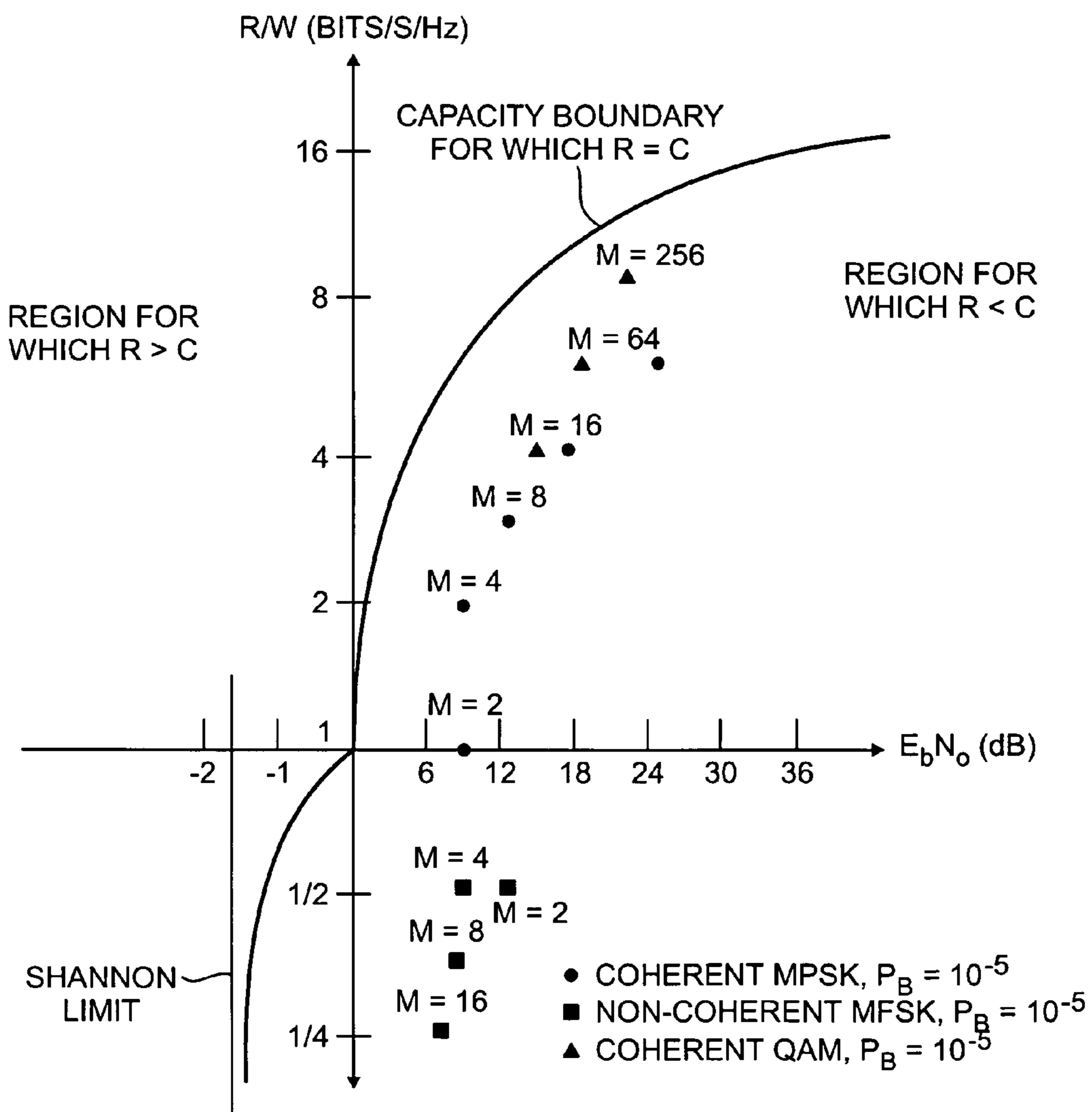
FIG. 3 (PRIOR ART)
