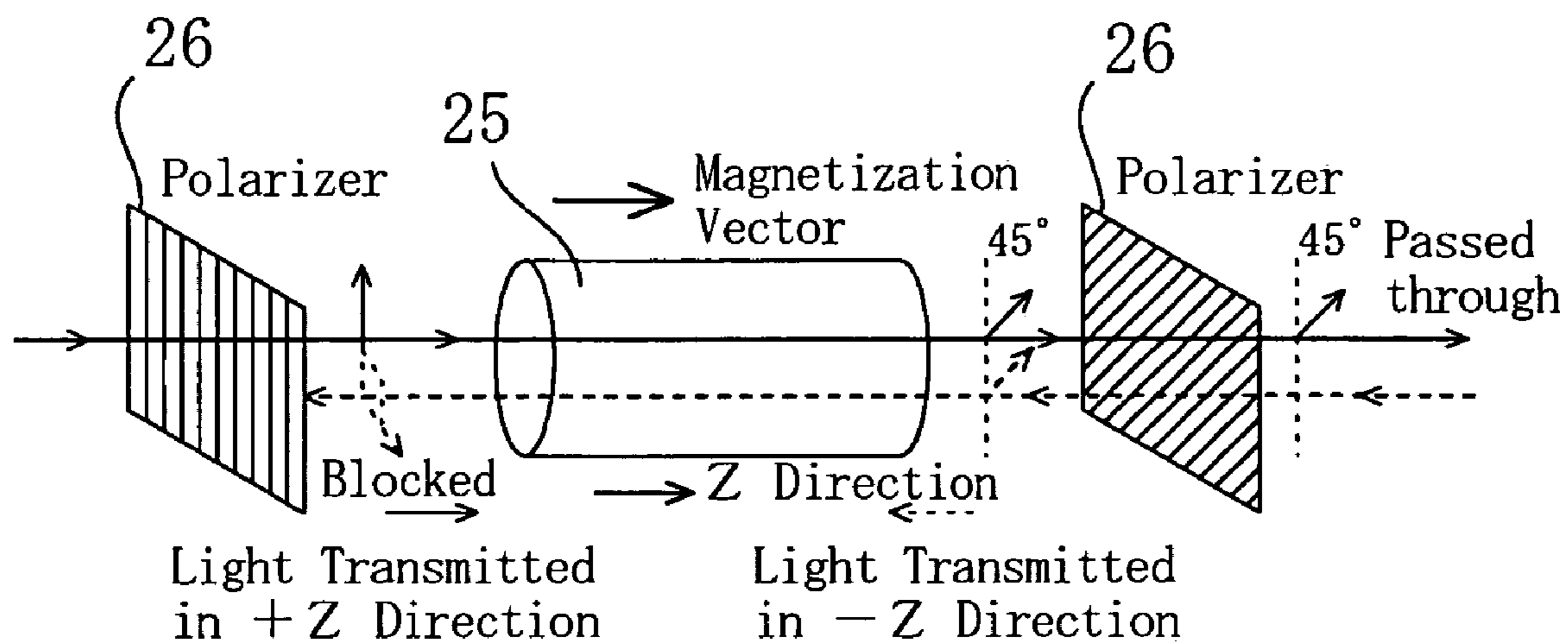
FIG. 10 PRIOR ART
