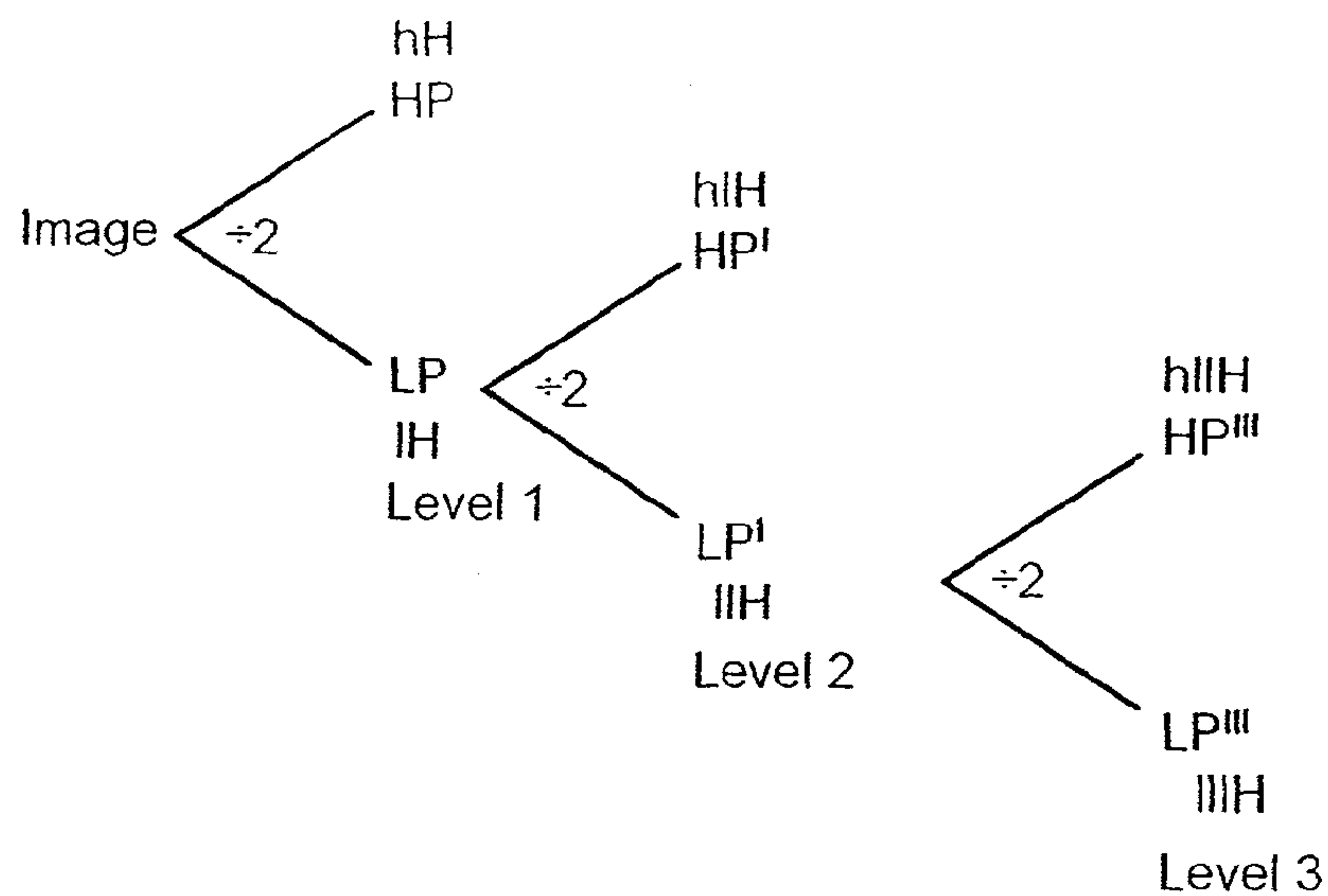
FIG. 3 Schematic of Wavelet Transform
