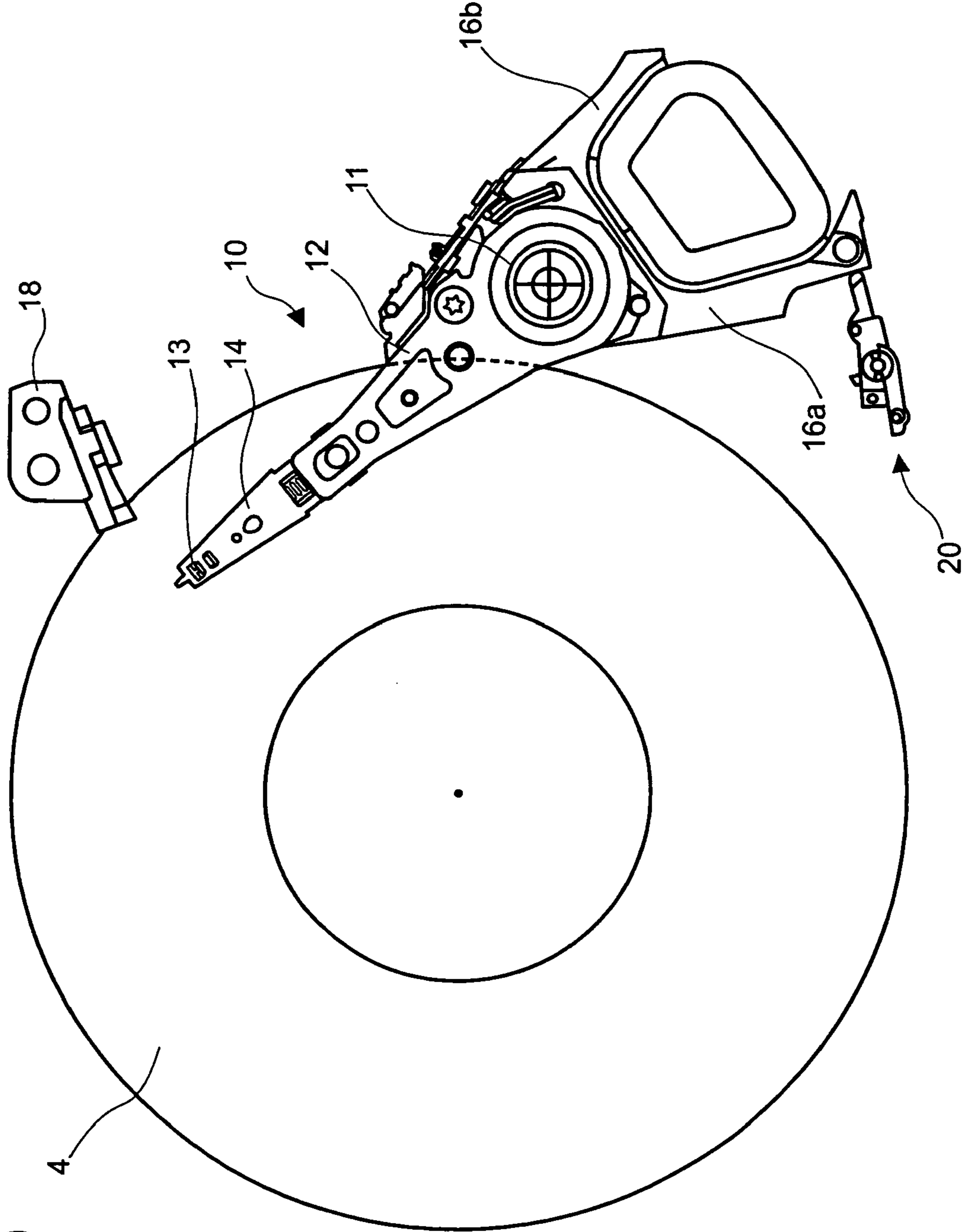
FIG.10 (Prior Art)
