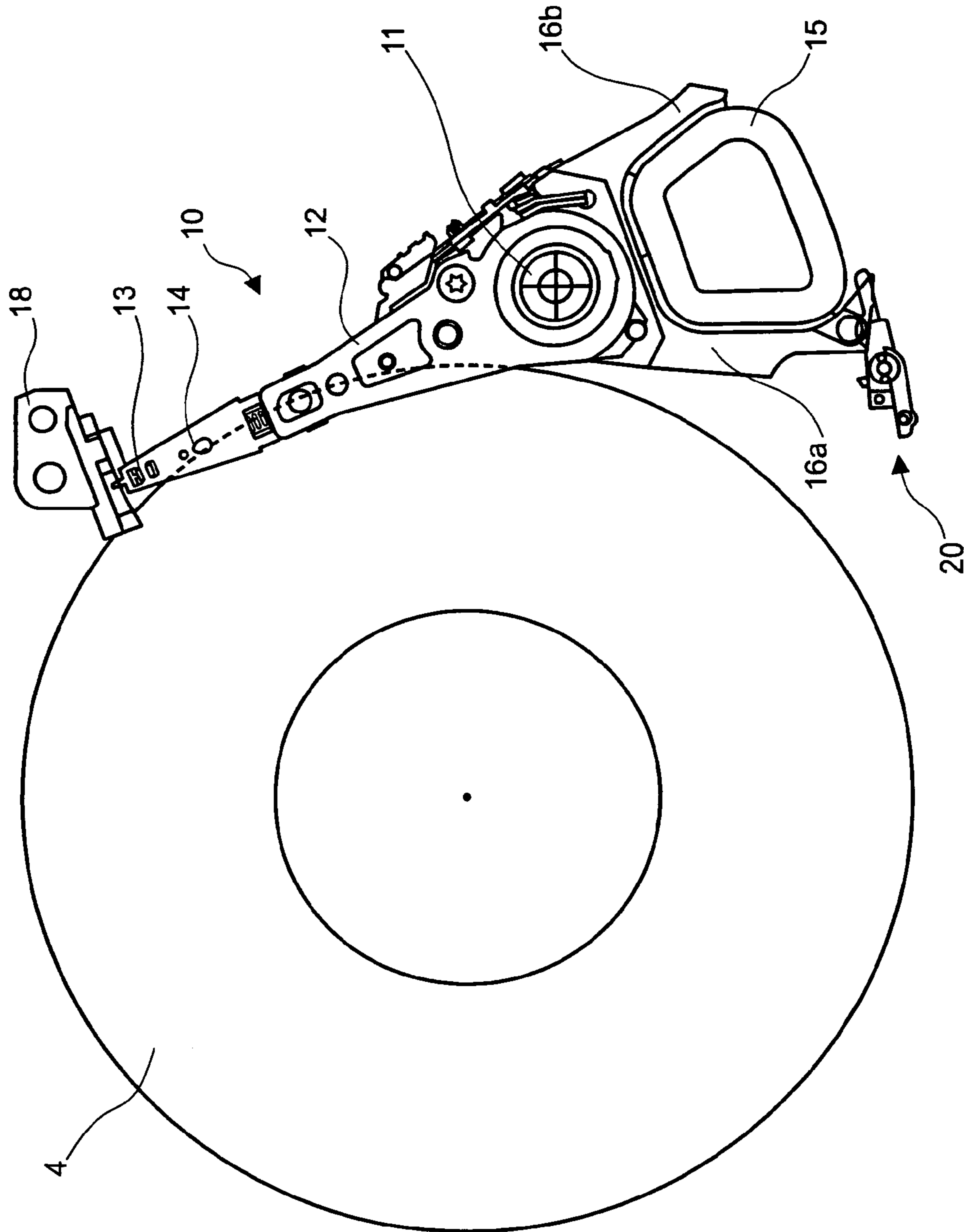
FIG.8 (Prior Art)
