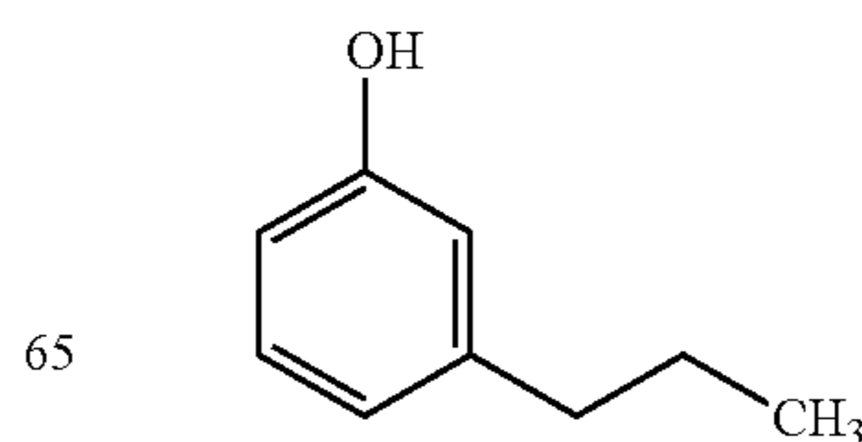
3-propyl phenol
