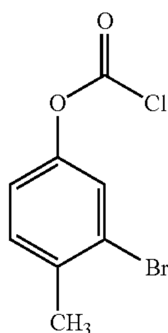
3-bromo-4-methyl-phenyl chloroformate
