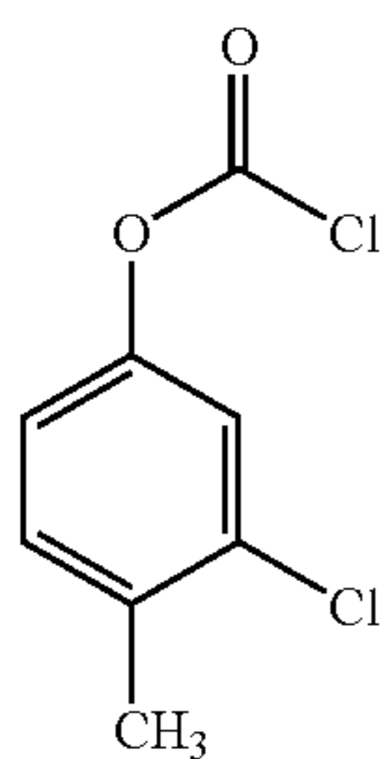
3-chloro-4-methyl-phenyl chloroformate
