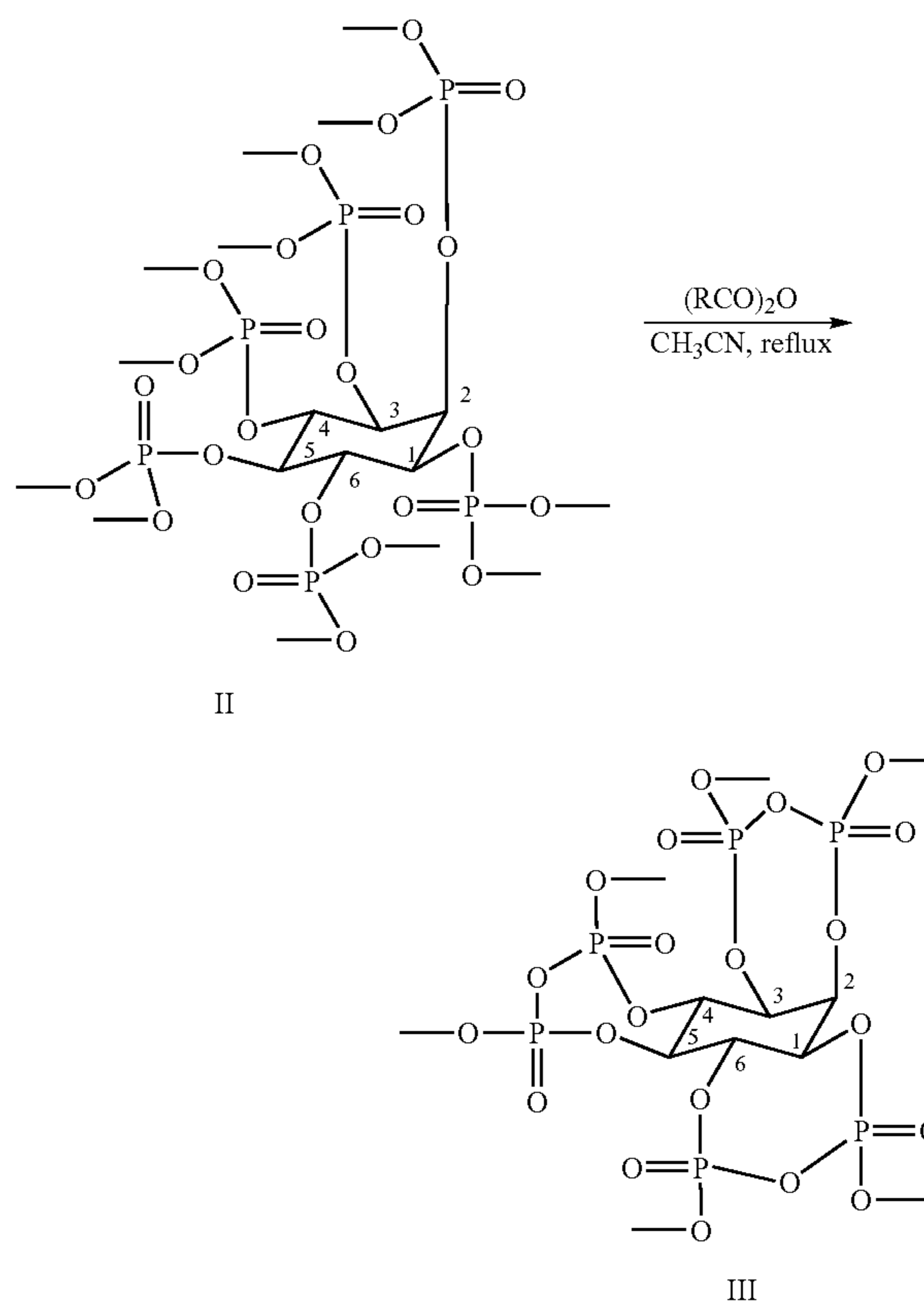
Scheme 1. Synthesis of IHP-tripyrophosphate.
