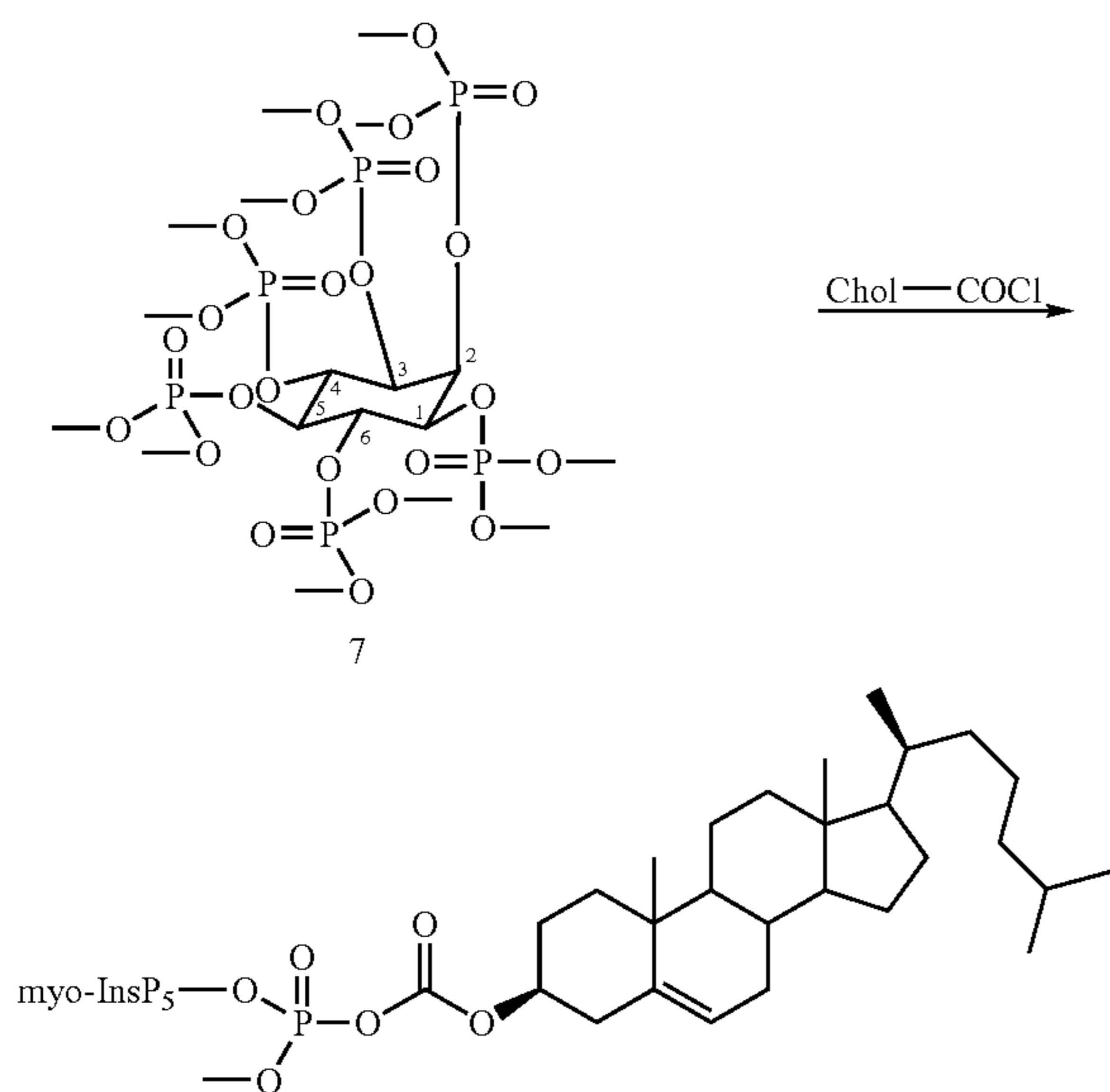
Scheme 7. Synthesis of IHP-Cholesteryloxy carbonyl hepta N,N-dimethyl-cyclohexyl-ammonium salt.
