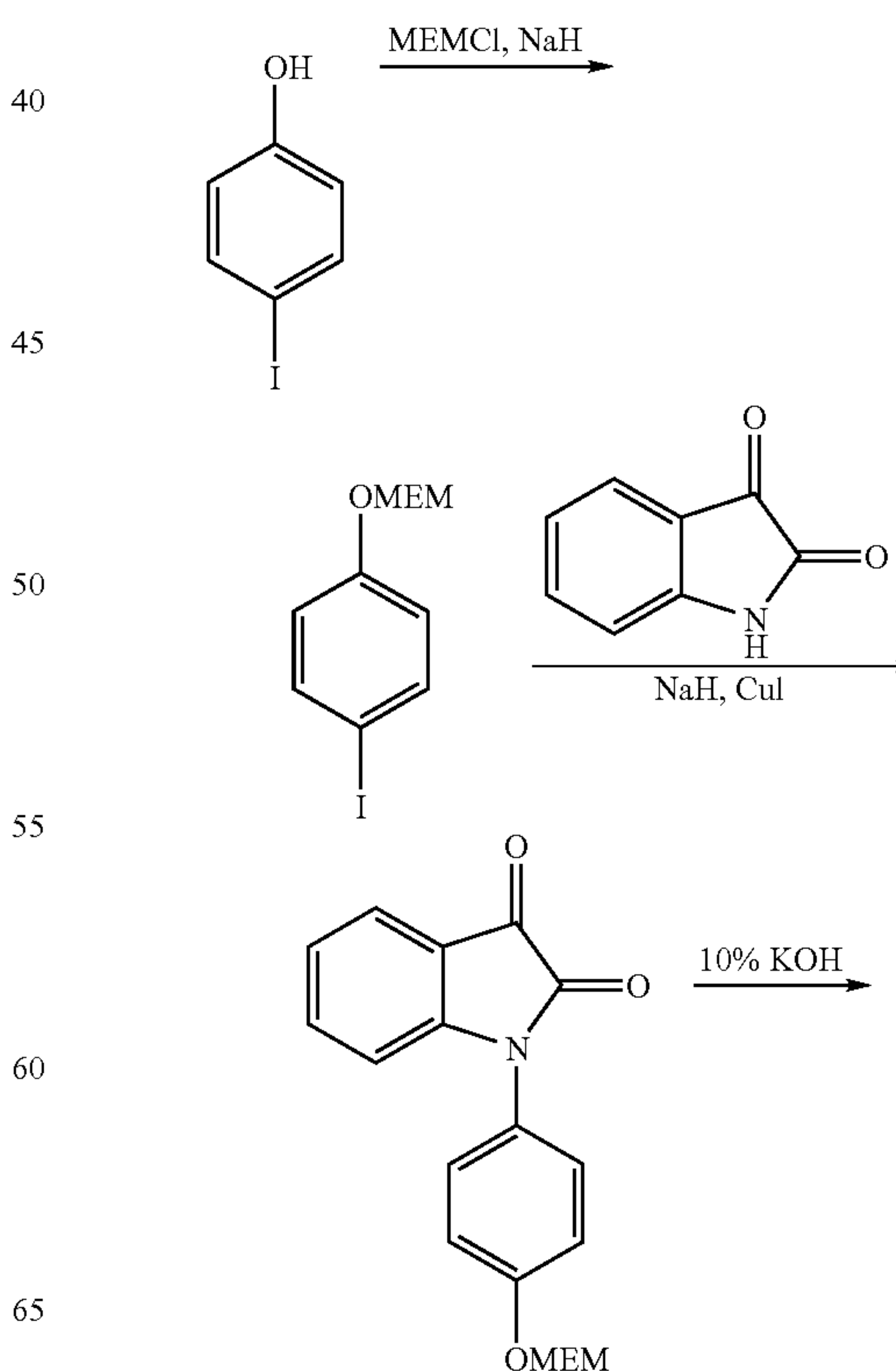
Scheme 4. Synthesis of 2-OH-DMAE
