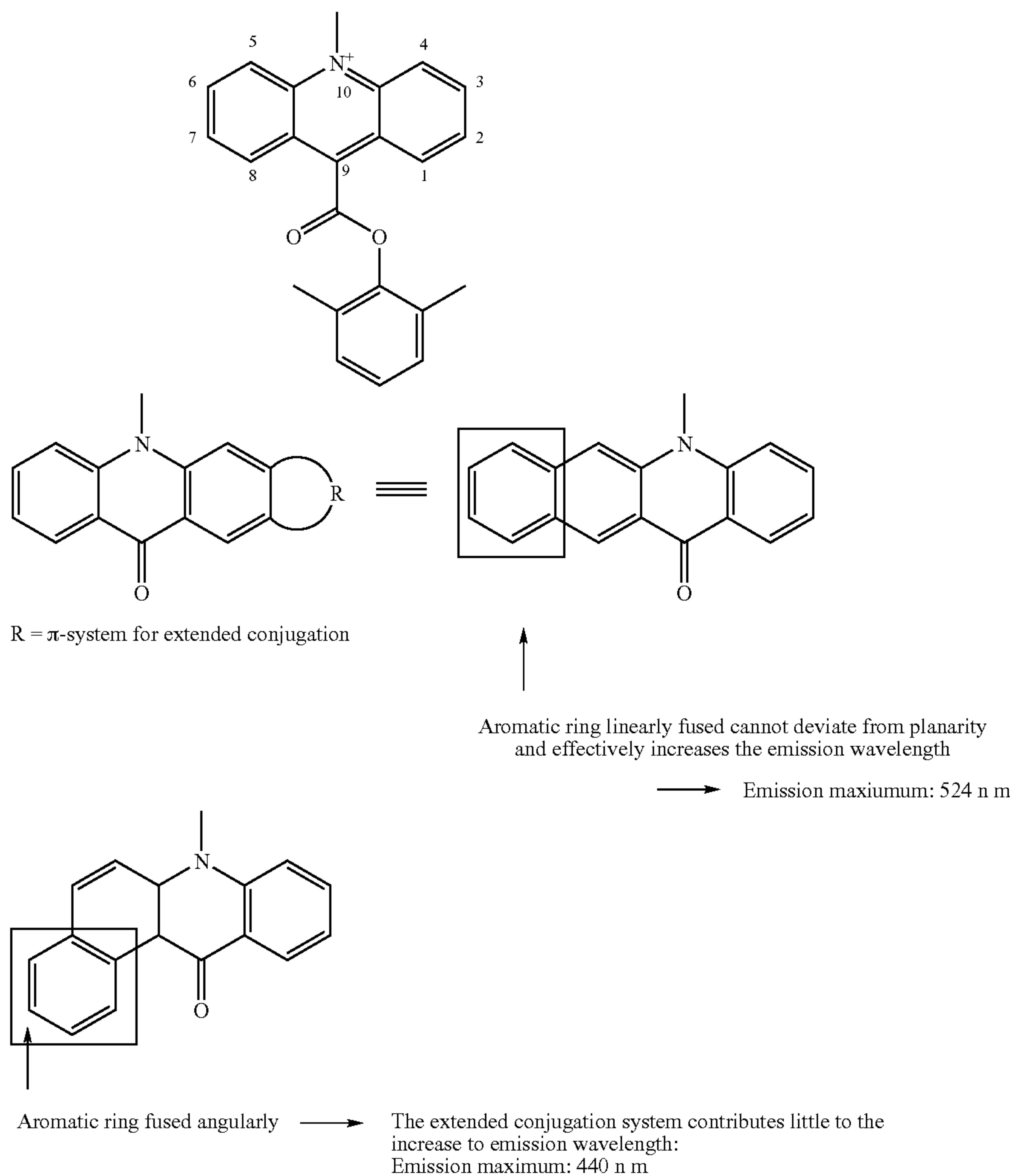
Numbering System for Acridinium Nucleus
