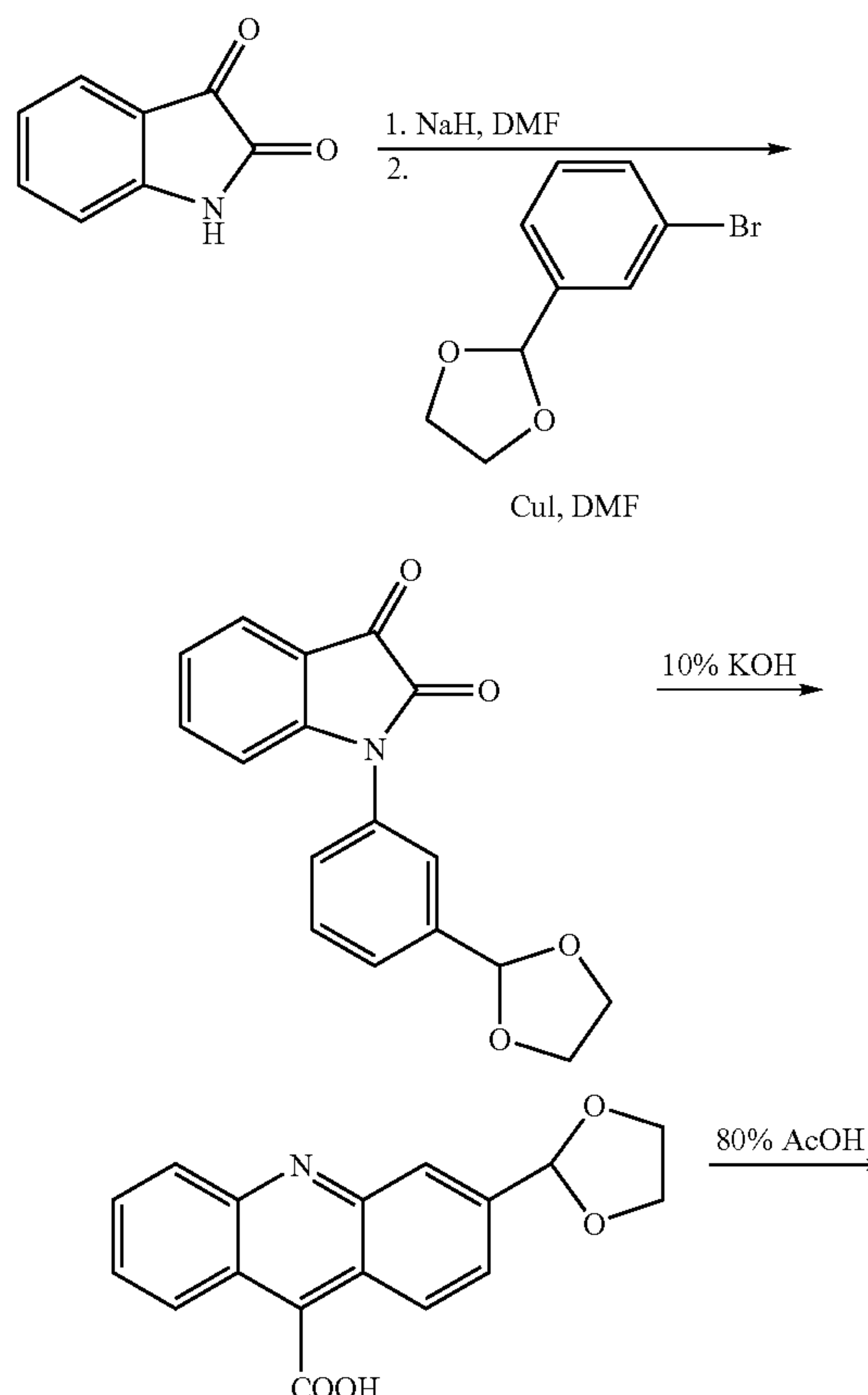
Scheme 1. Synthesis of 3-Substituted AE Derivatives
