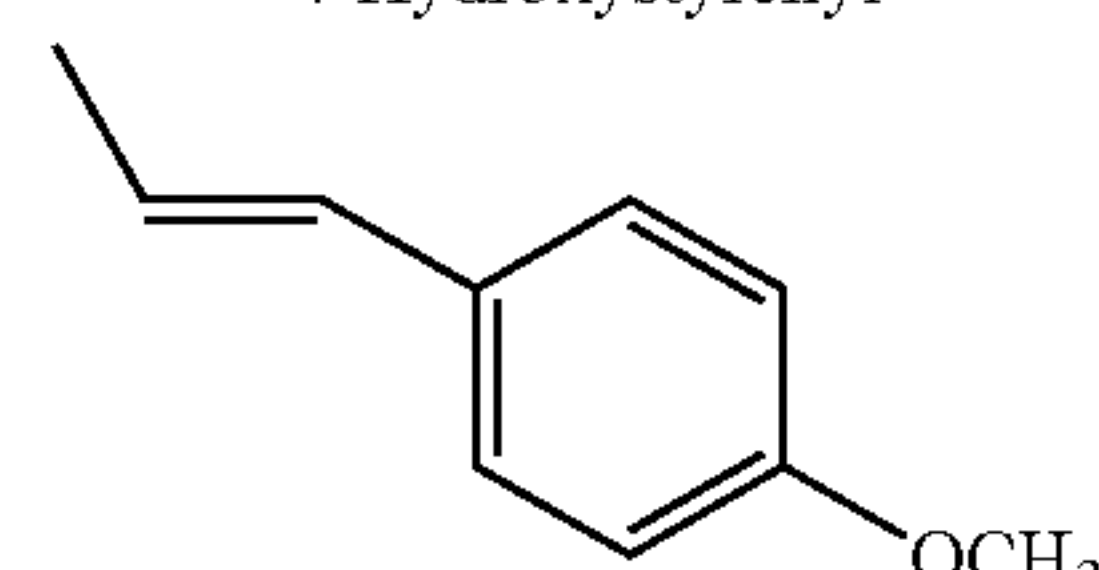
4-Methoxystyrenyl
