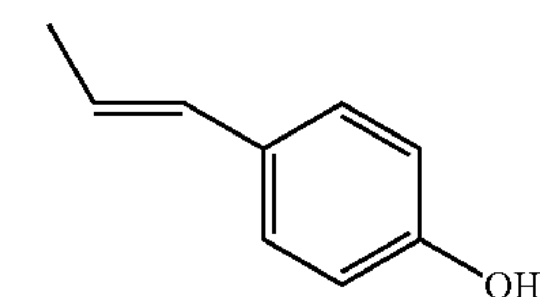
4-Hydroxystyrenyl
