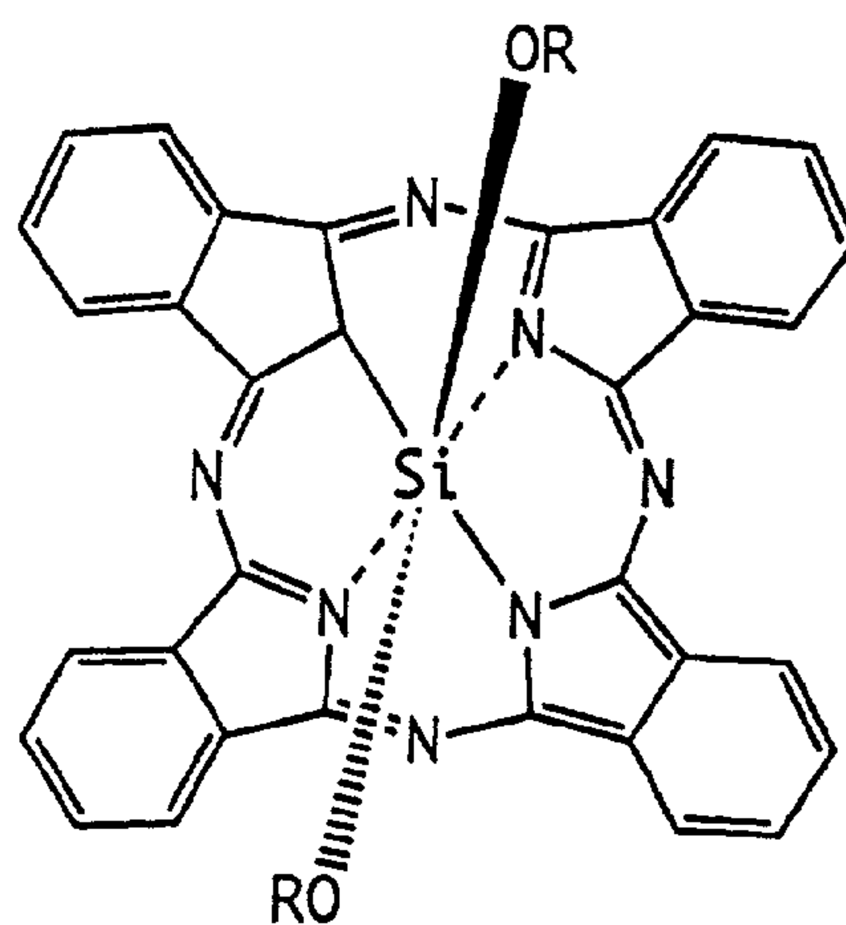
SILICON PHTHALOCYANINE
