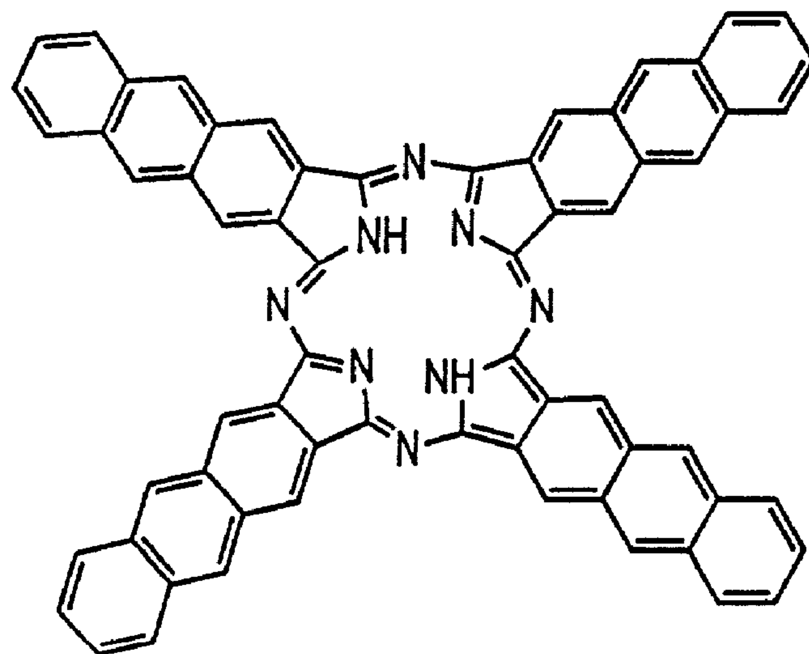
ANTHRANYLOCYANINE
