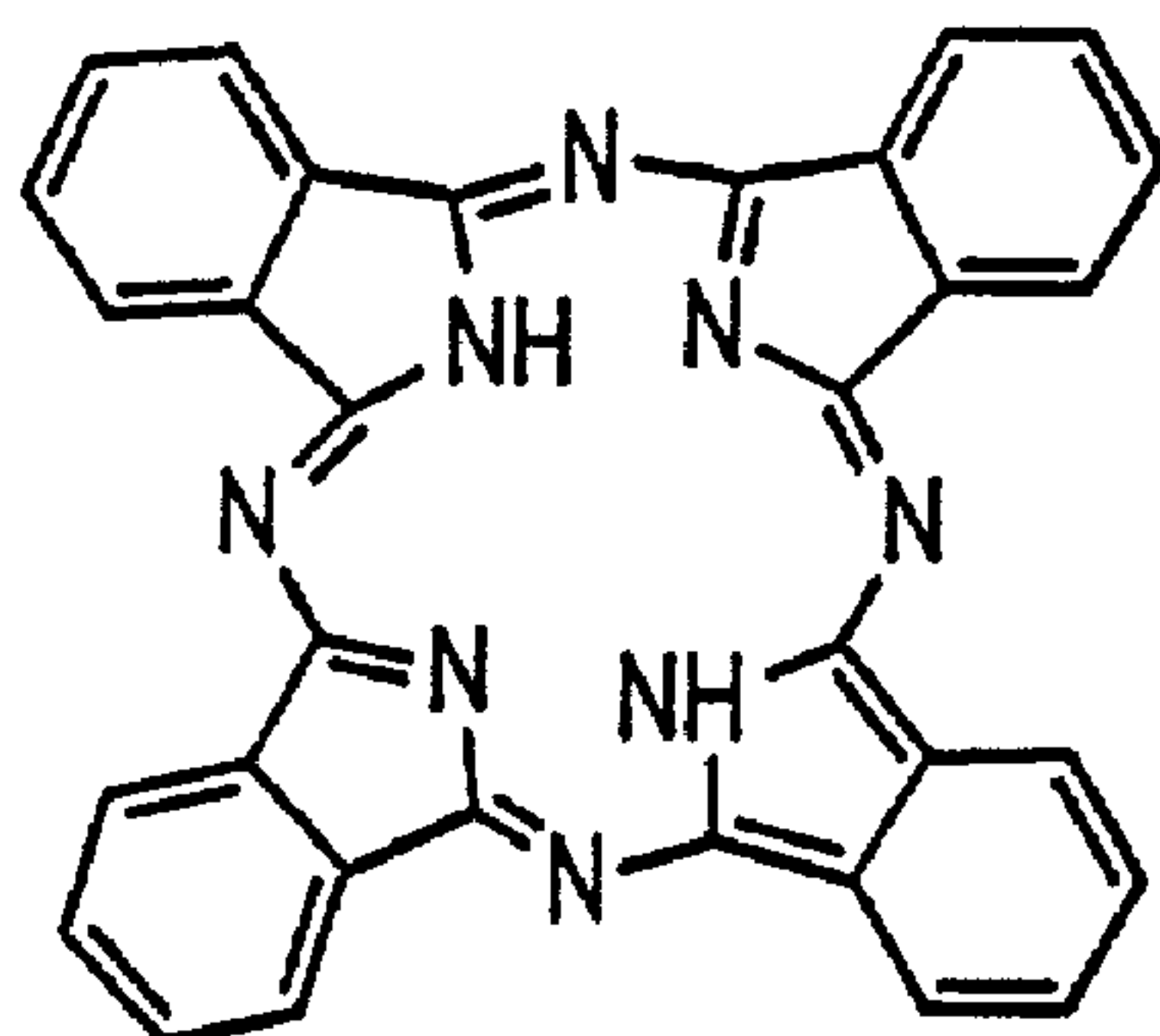
PHTHALOCYANINE
