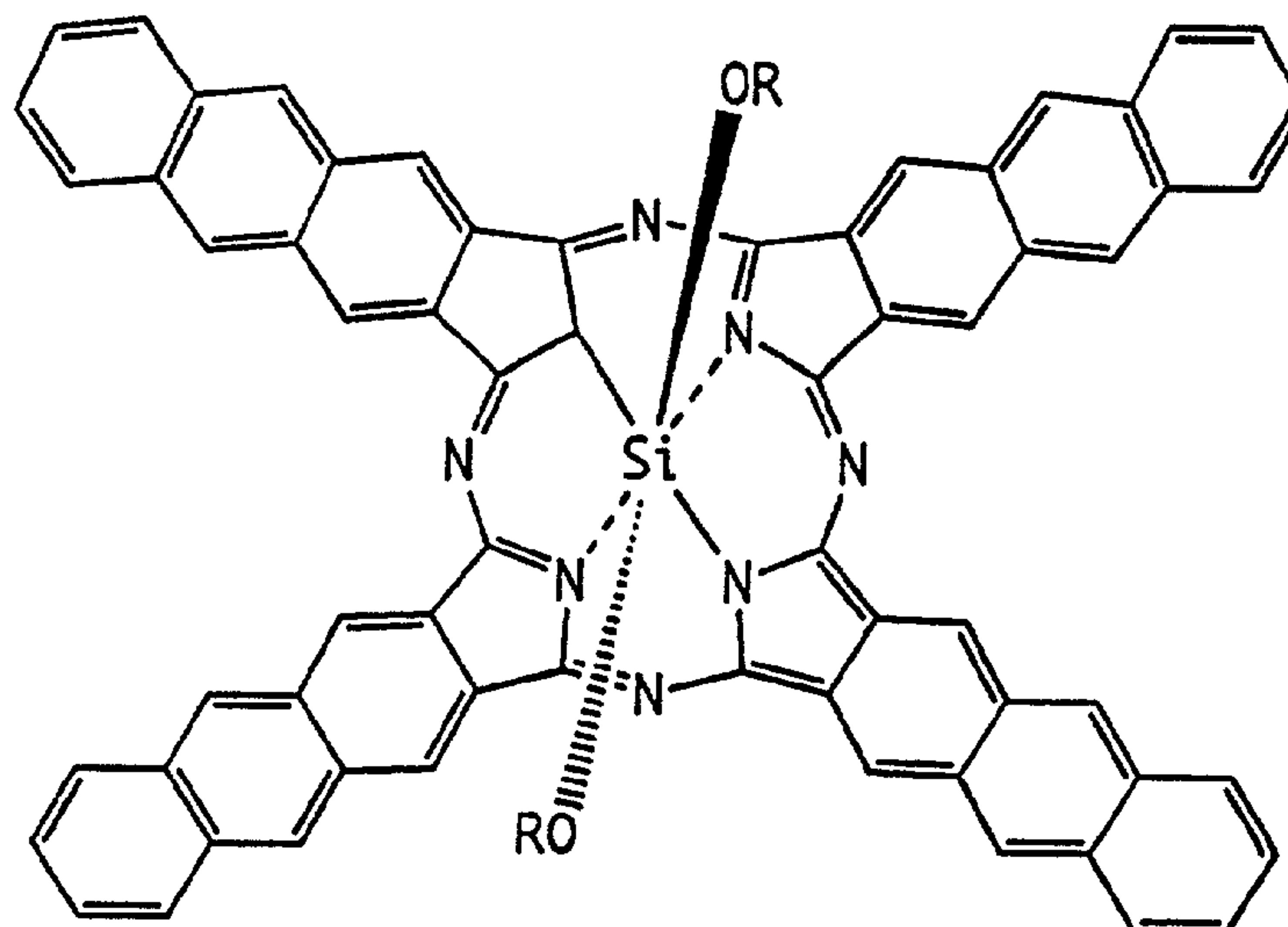
SILICON ANTHRACYANINE
