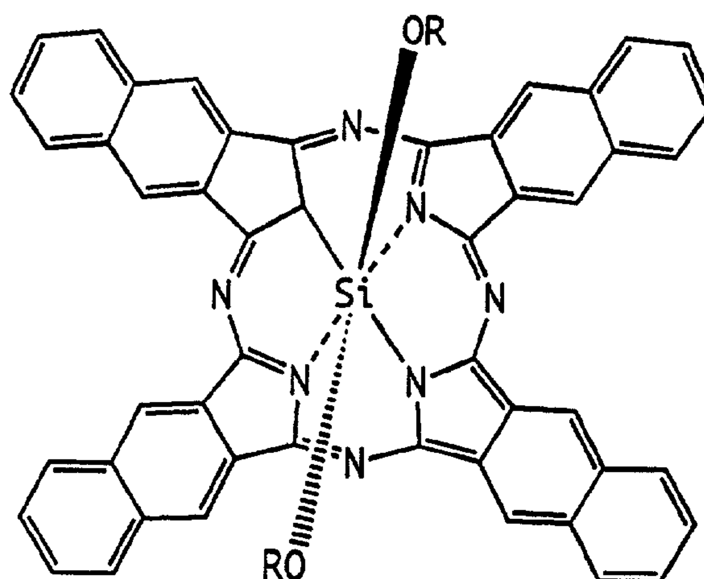
SILICON NAPHTHALOCYANINE
