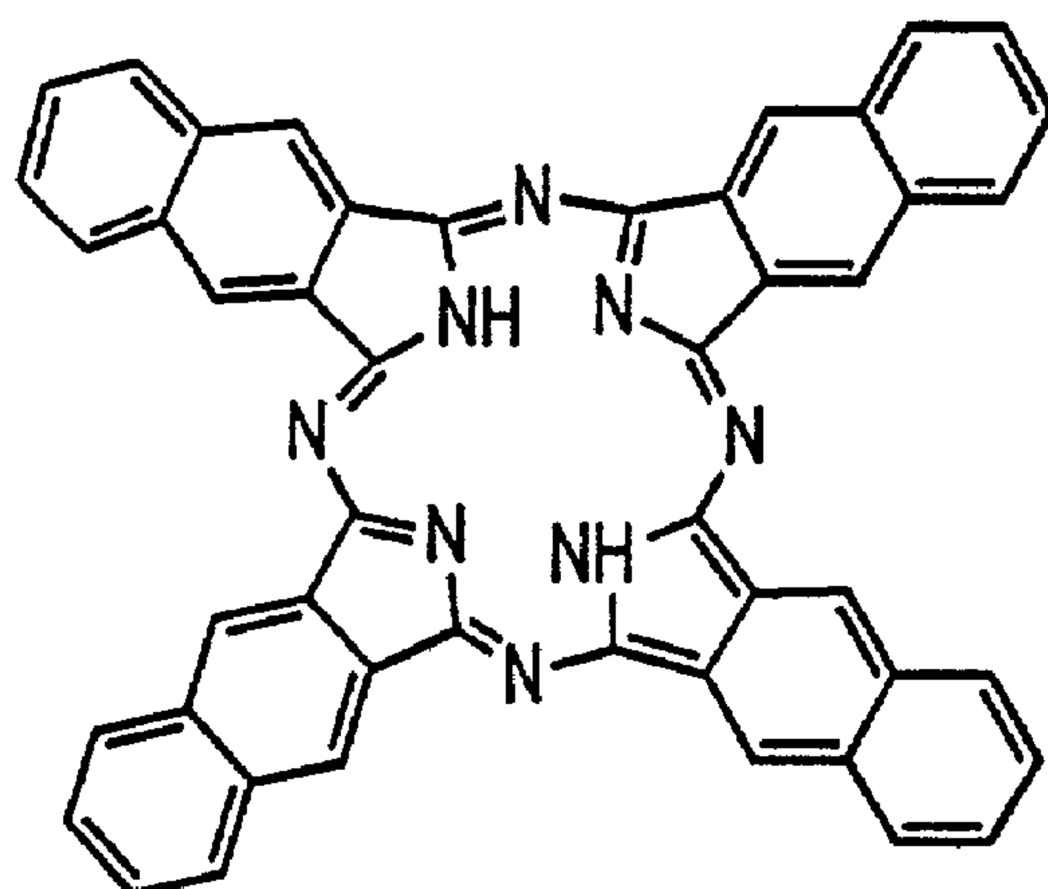
NAPHTHALOCYANINE
