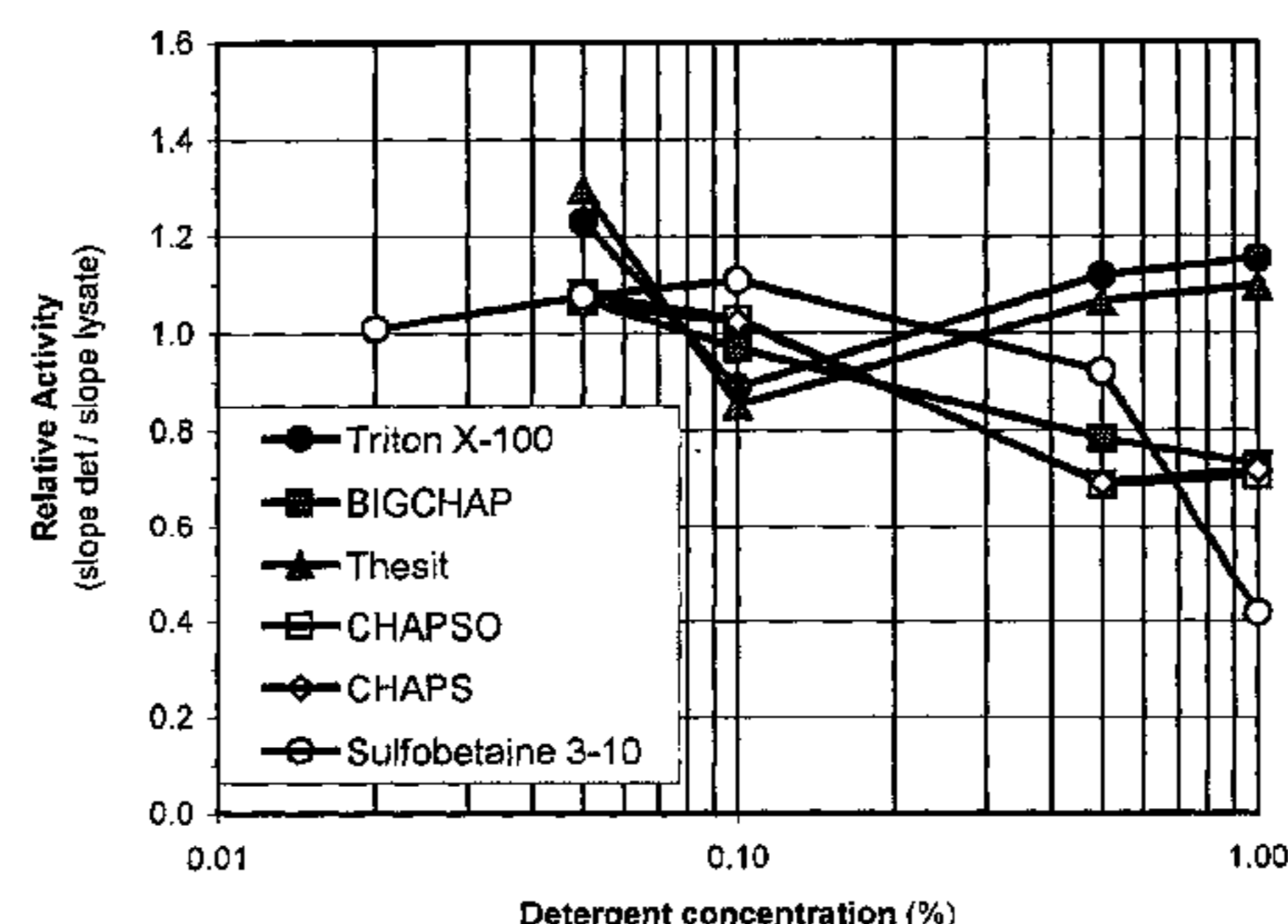
ATPase inhibition using nonionic and zwitterionic detergents
