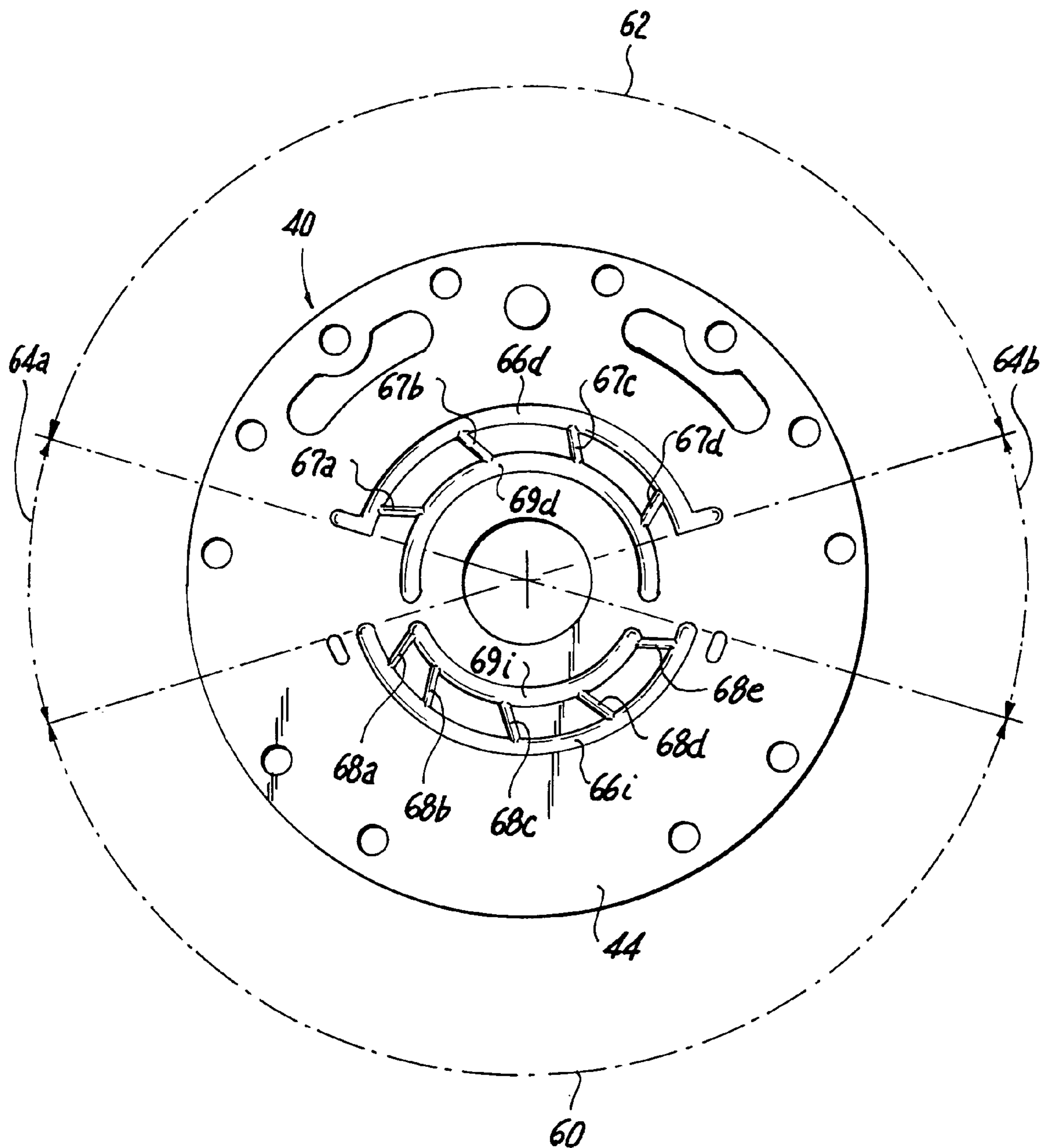
Fig. 3 (Prior Art)
