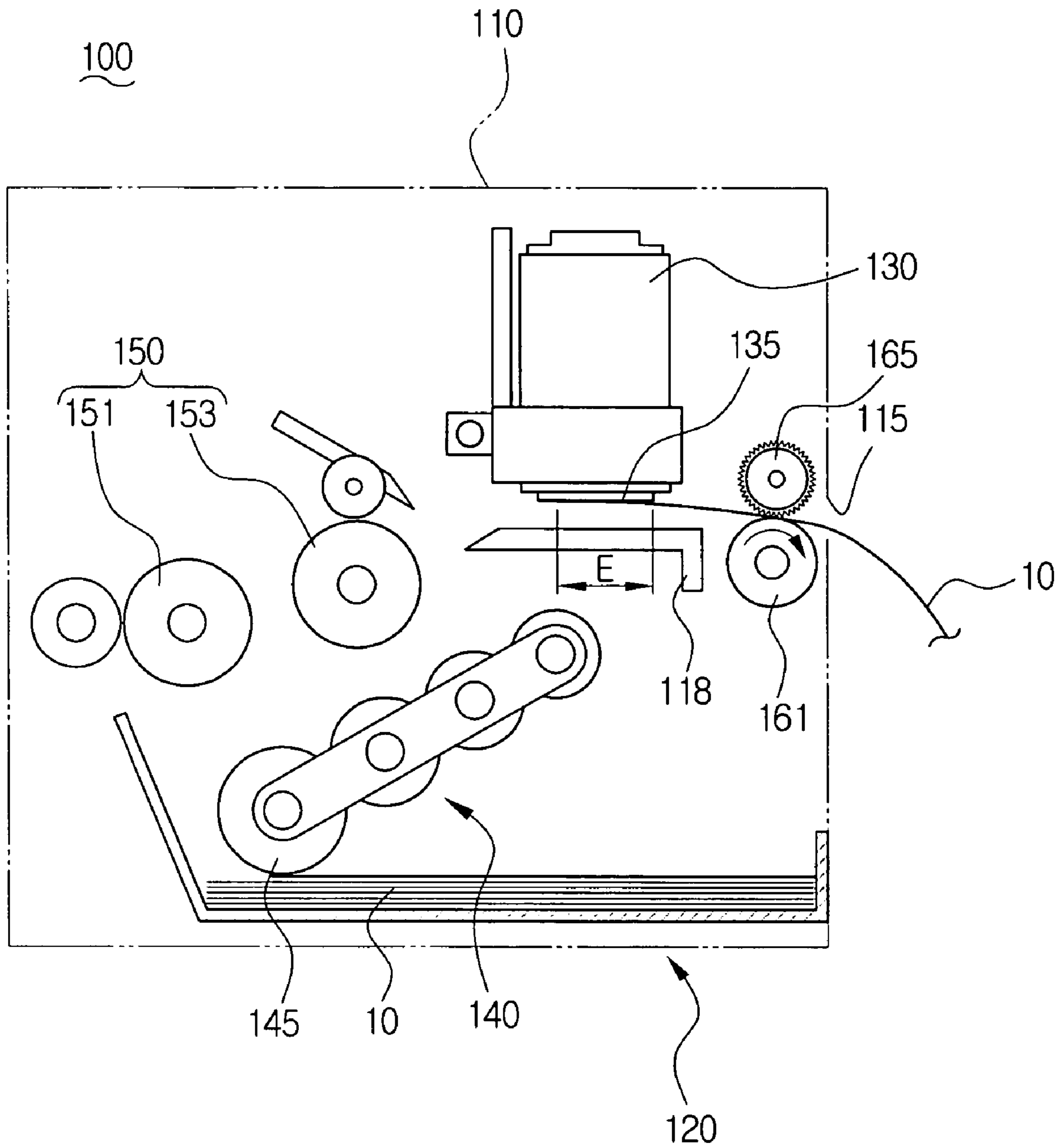
FIG. 1 (PRIOR ART)
