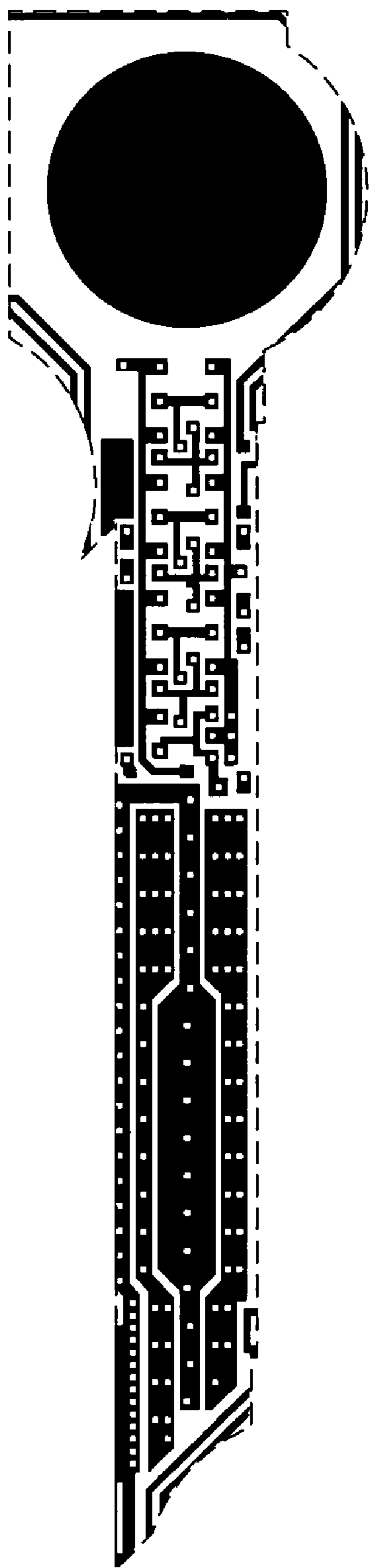
Metal 1 mask
