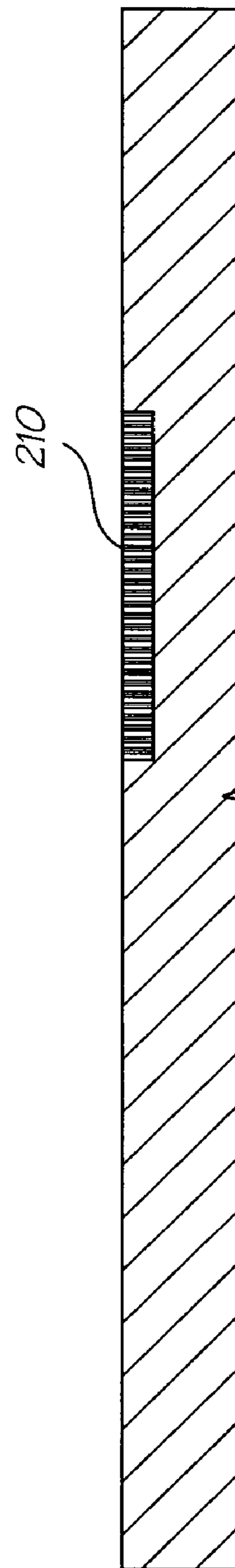
Implant N-Well
